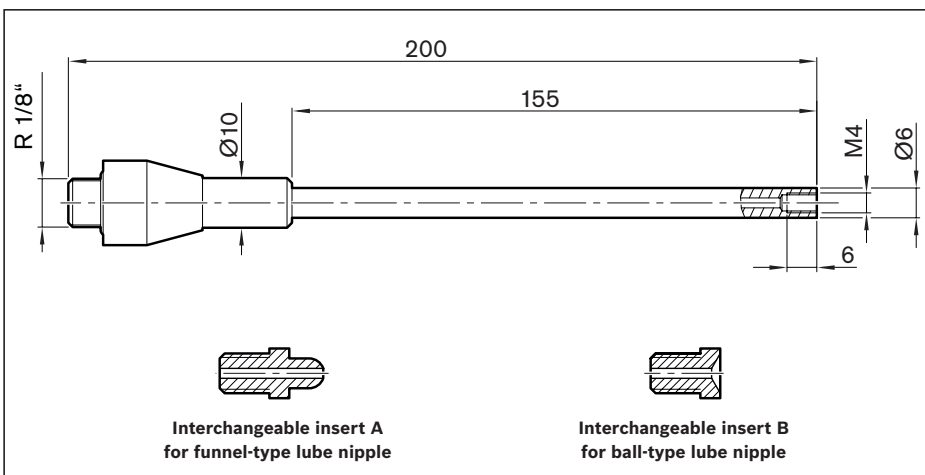
Nozzle pipe
