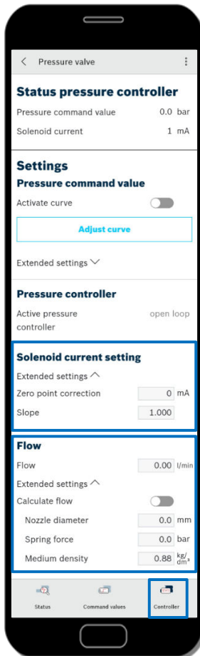
Fig. 46: Solenoid current control in "easy2connect"
