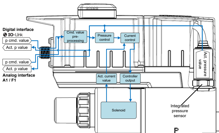
Fig. 3: Overview of DBETA with integrated pressure sensor
