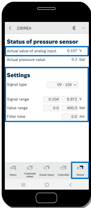
Fig. 38: Pressure settings via "easy2connect"
