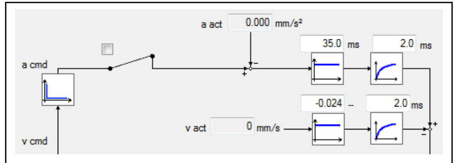
Fig. 7-121: State controller
