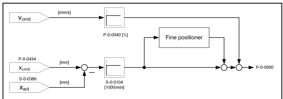
Fig. 6-13: Position controller
