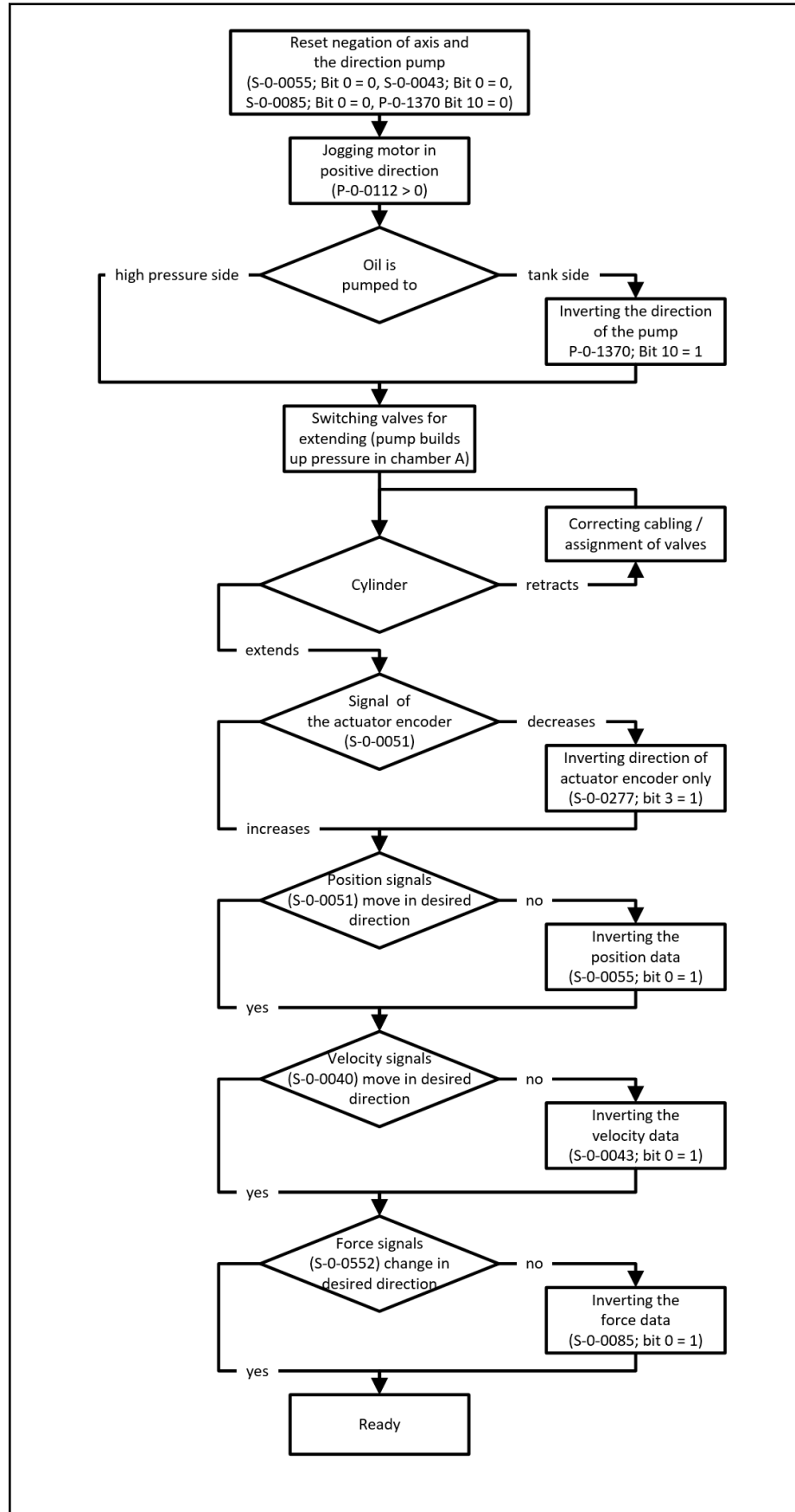
Fig. 7-40: Scaling configuration if direction is input via valves
