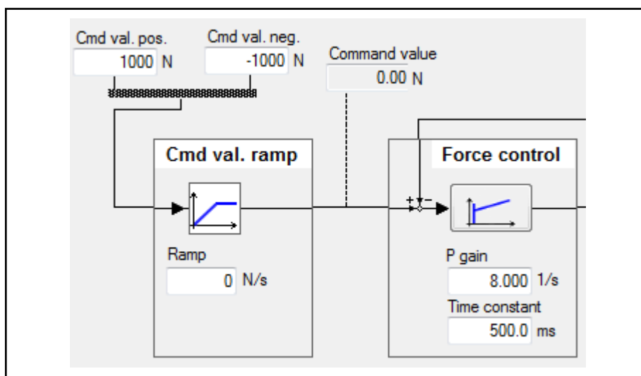
Fig. 7-129: Force controller overview
