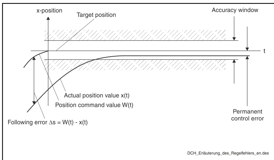
Fig. 6-14: Explanation of the control error
