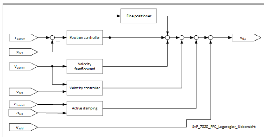
Fig. 6-12: Position controller overview
