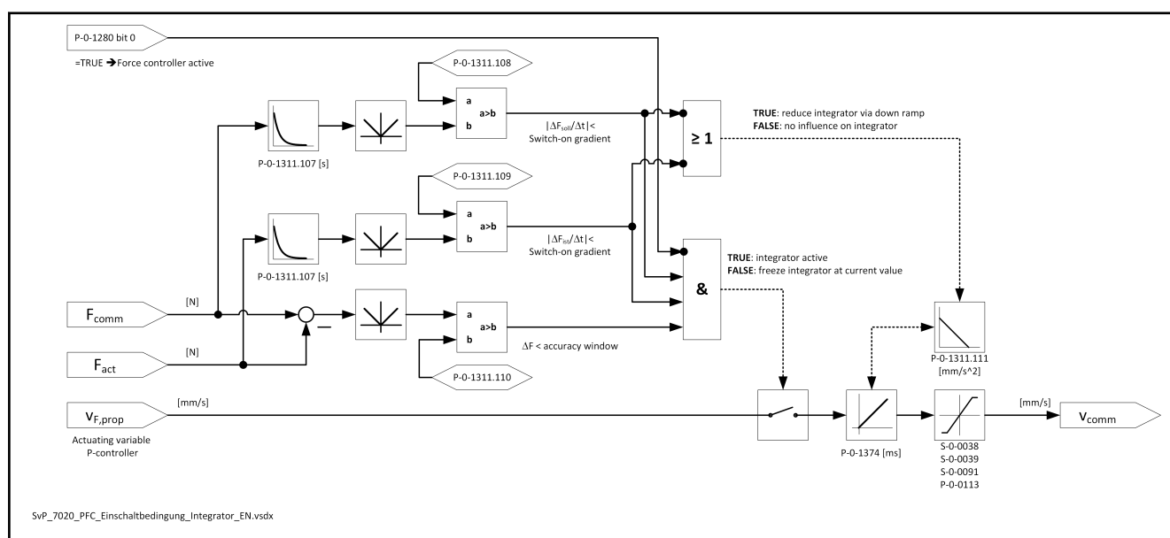
Fig. 6-19: Switch-on condition for integrator
