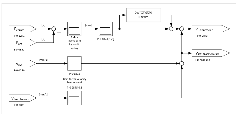
Fig. 6-18: Controller structure using the example of force
