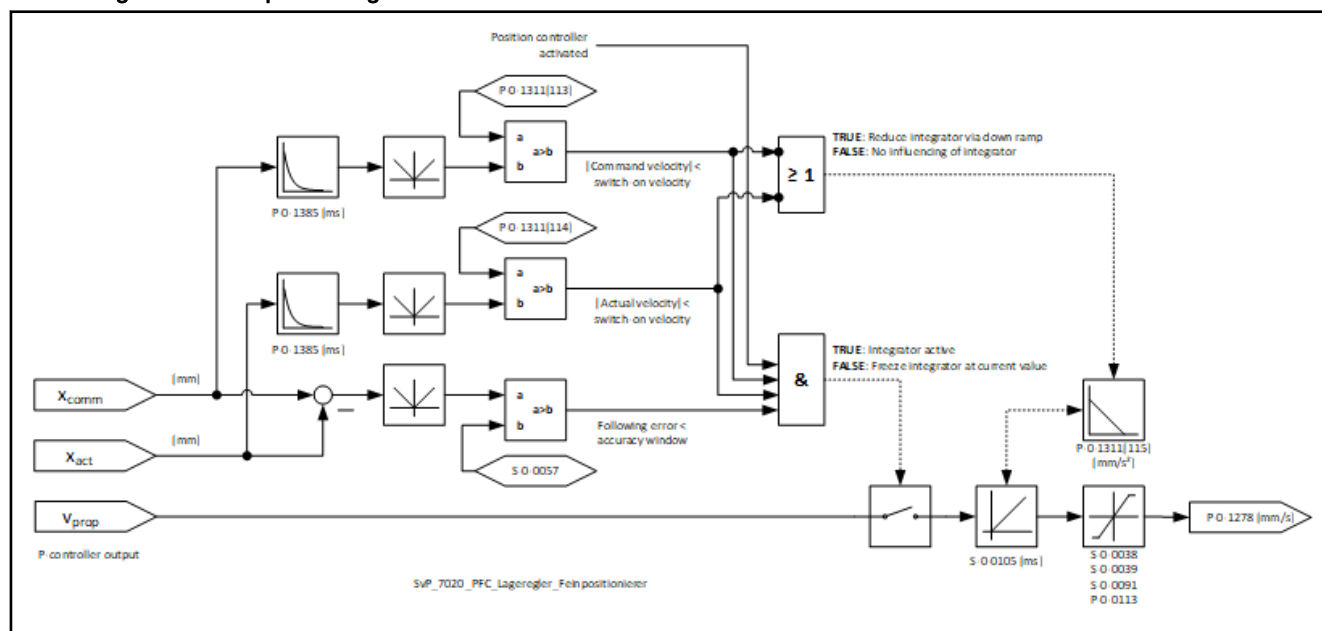
Fig. 6-15: Fine positioner
