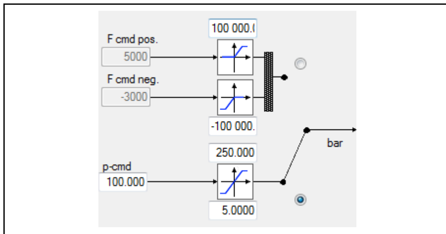
Fig. 7-133: Switching to force control
