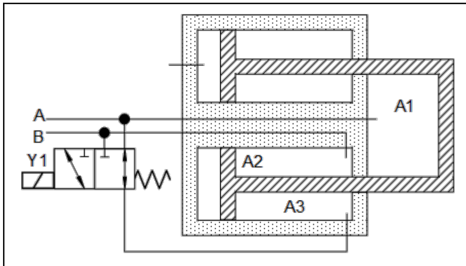
Fig. 6-5: Double rod multiple-chamber cylinder with A/B connections and A1/A2/A3 areas
