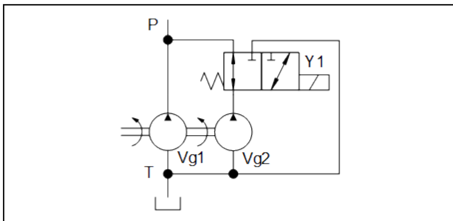
Fig. 6-10: Double pump
