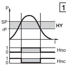
Fig. 1 Normally open
