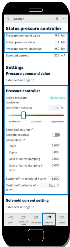
Fig. 51: 29283-FK_Closed-loop pressure control 2
