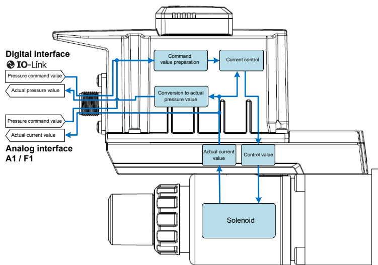
Fig. 1: Overview_(Z)3DREE
