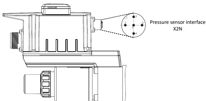
Fig. 34: Pressure sensor
