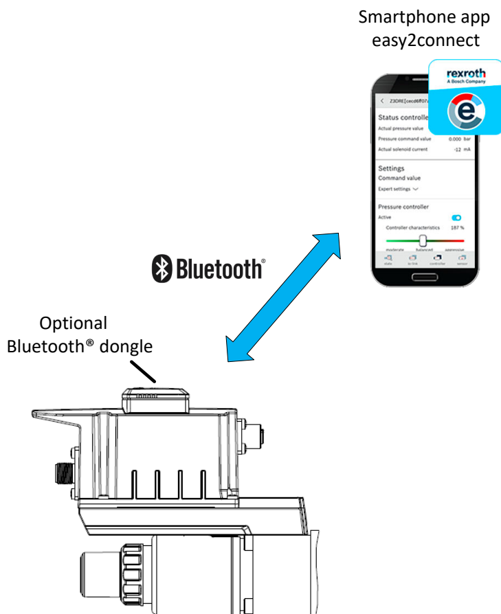
Fig. 4: Overview_BluetoothDongle
