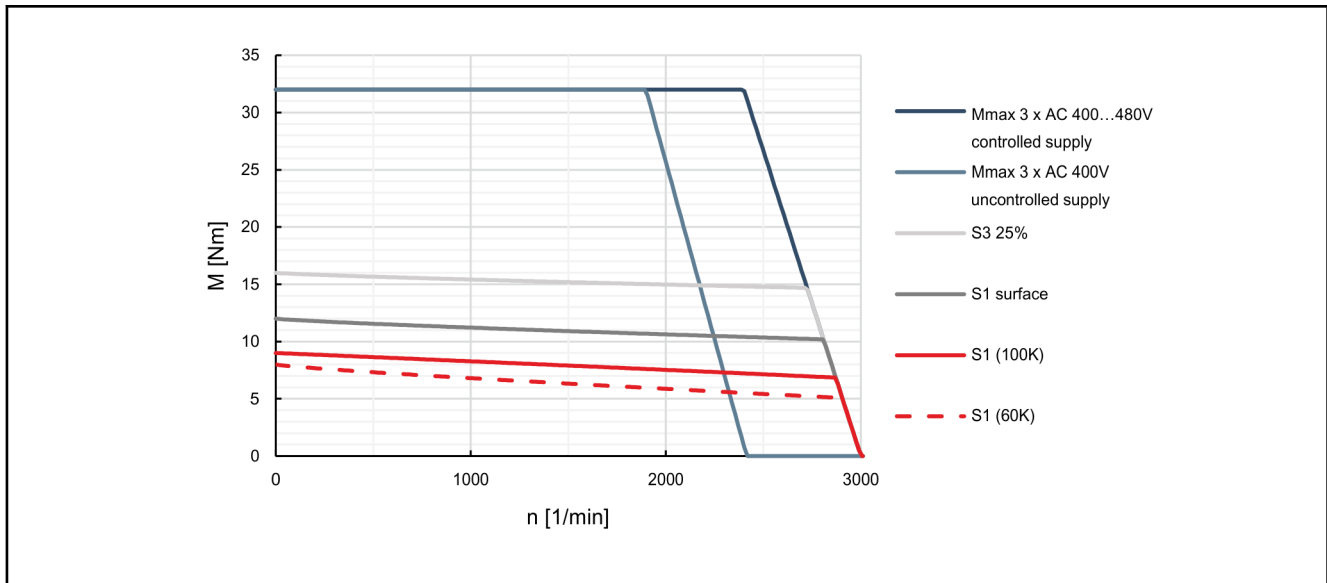
Fig. 4-21: Characteristic curves of motor MSK061C-0200
