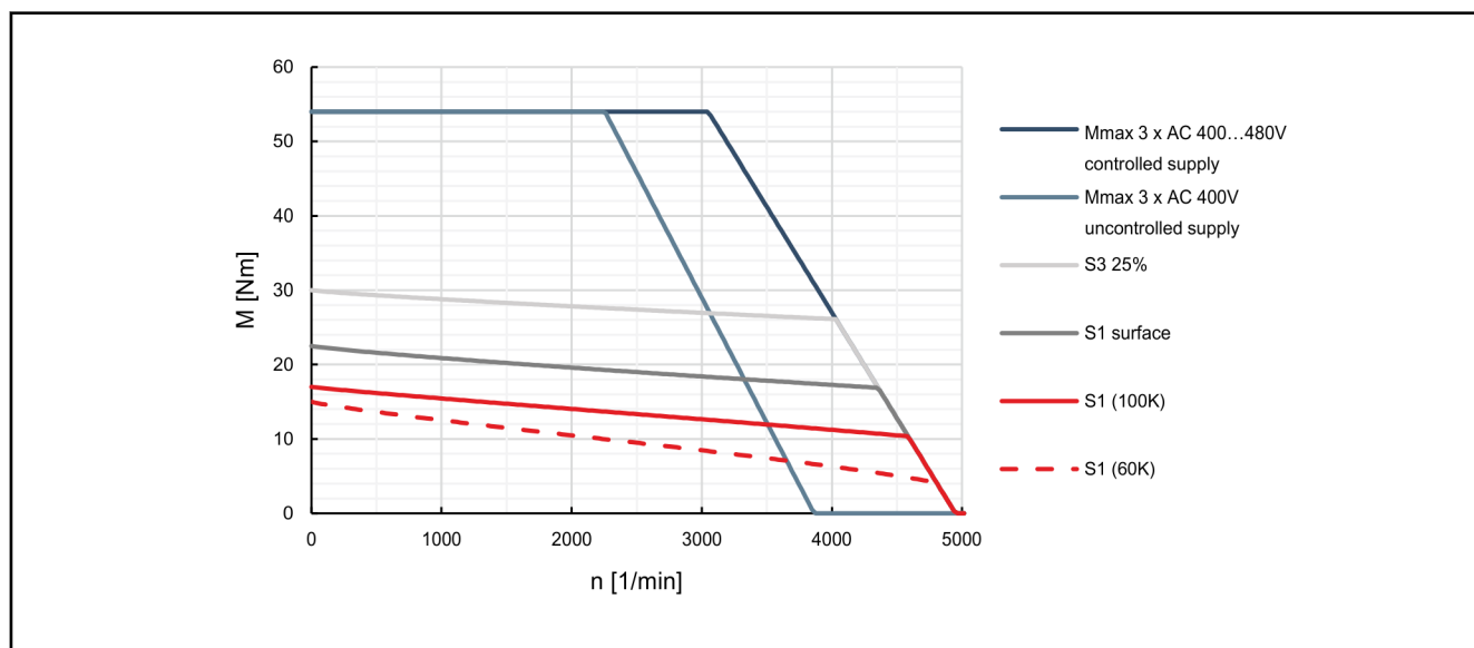
Fig. 4-54: Characteristic curves of motor MSK100A-0300
