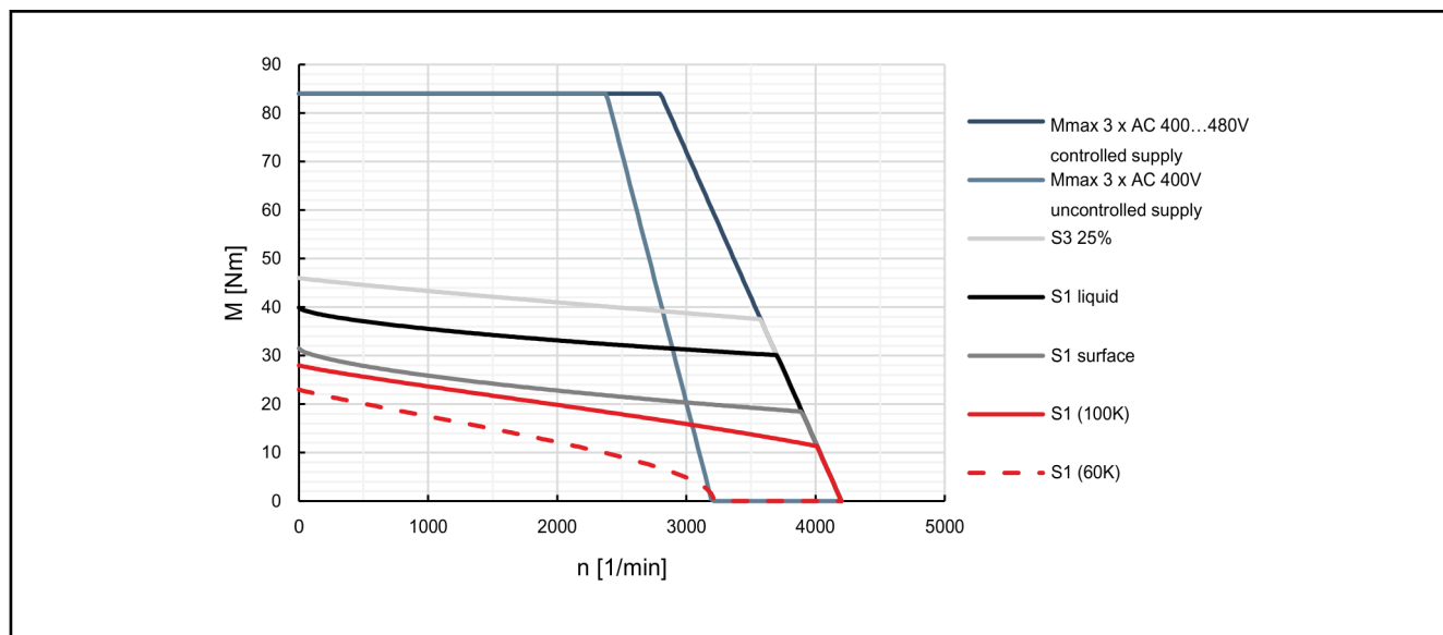
Fig. 4-40: Characteristic curves of motor MSK071E-0300
