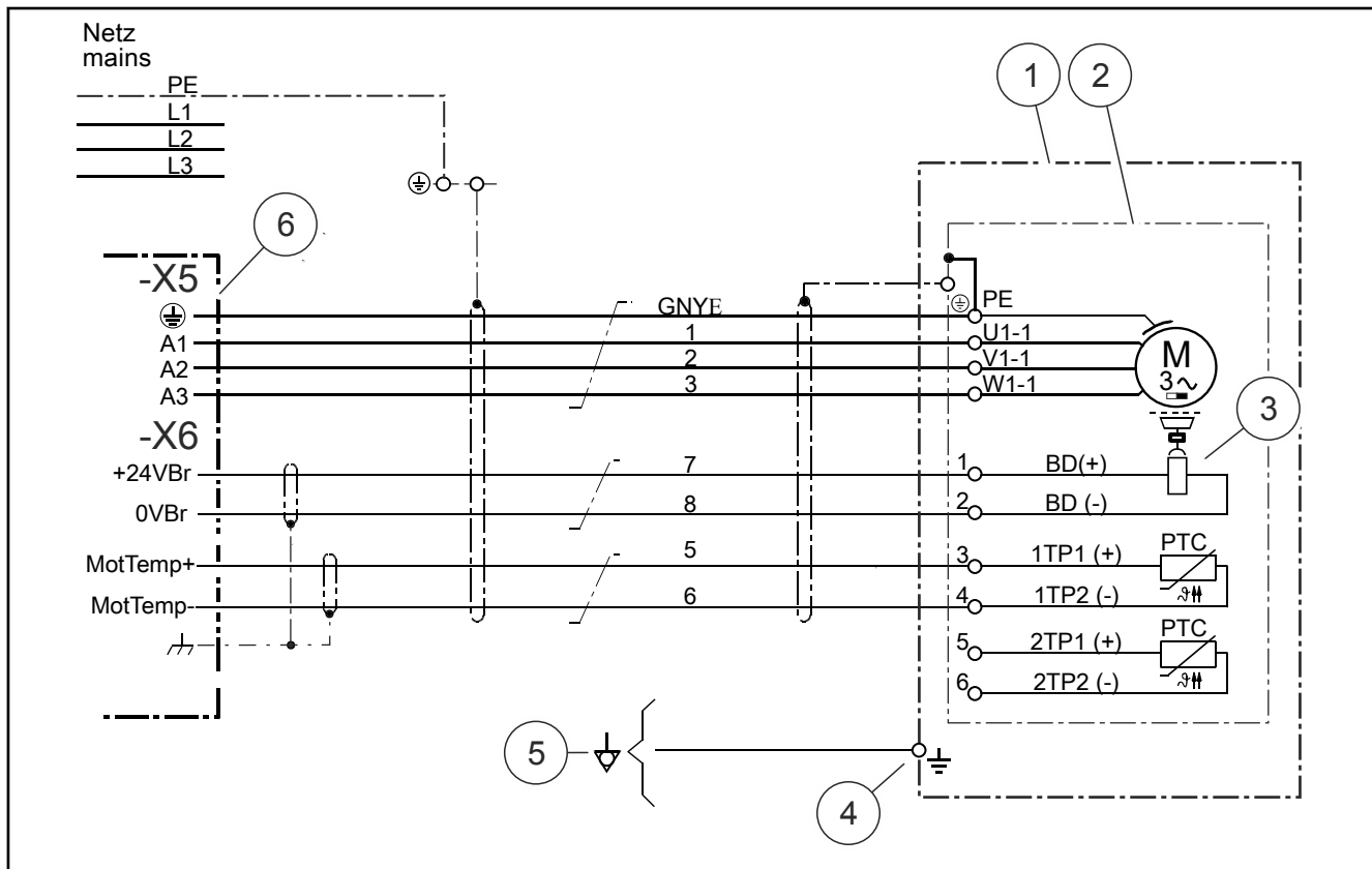
Fig. 12-3: Connection points
