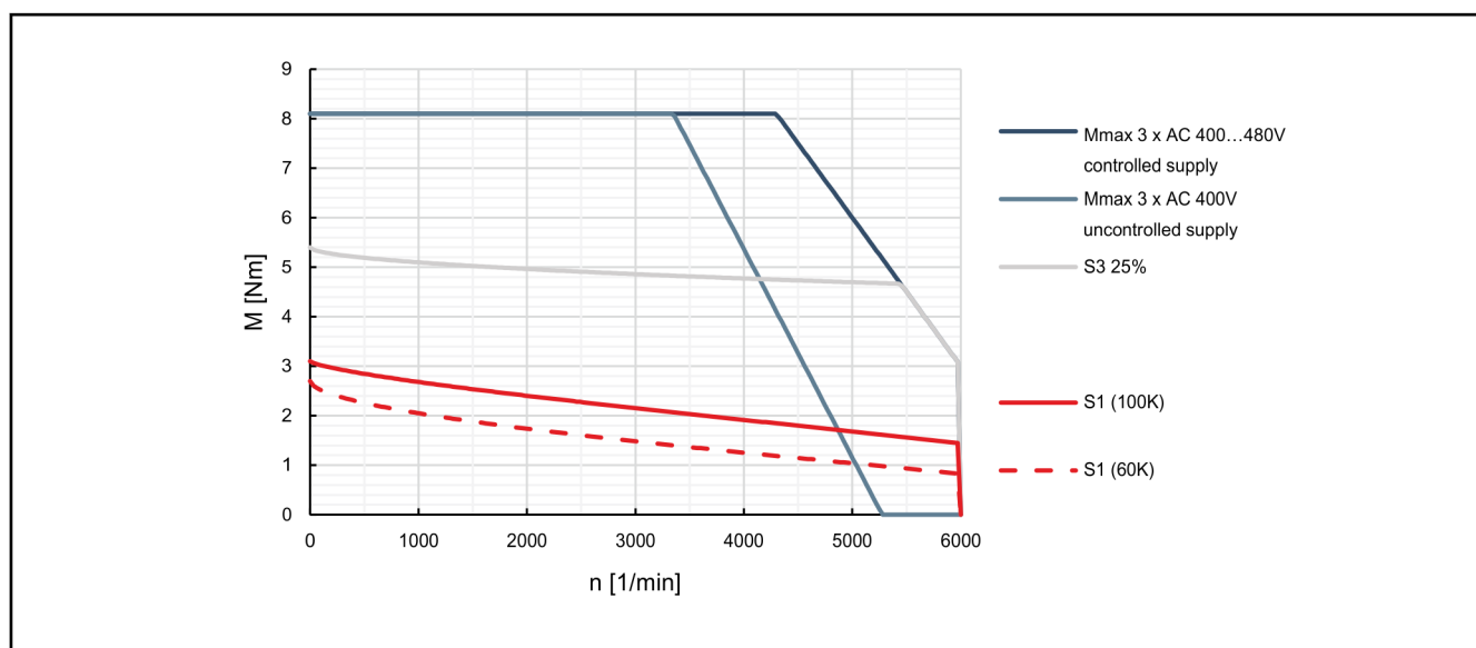
Fig. 4-7: Characteristic curves of motor MSK040C-0450
