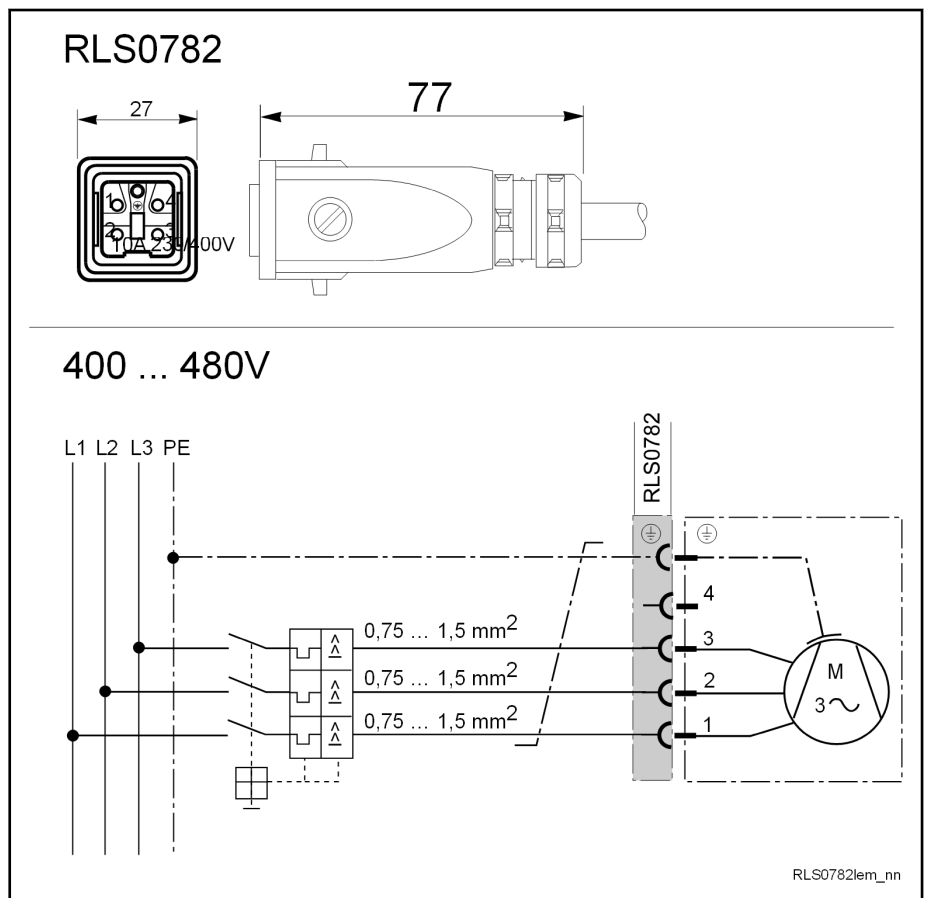
Fig. 7-4: 3-phase fan connection with protective switch
