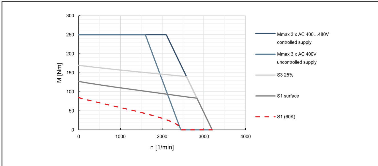
Fig. 4-78: Characteristic curves of motor MSK131B-0200
