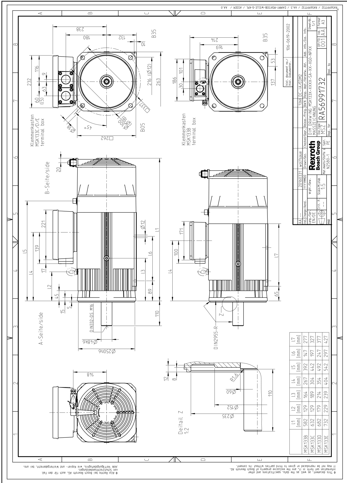
Fig. 5-35: Specifications MSK133
