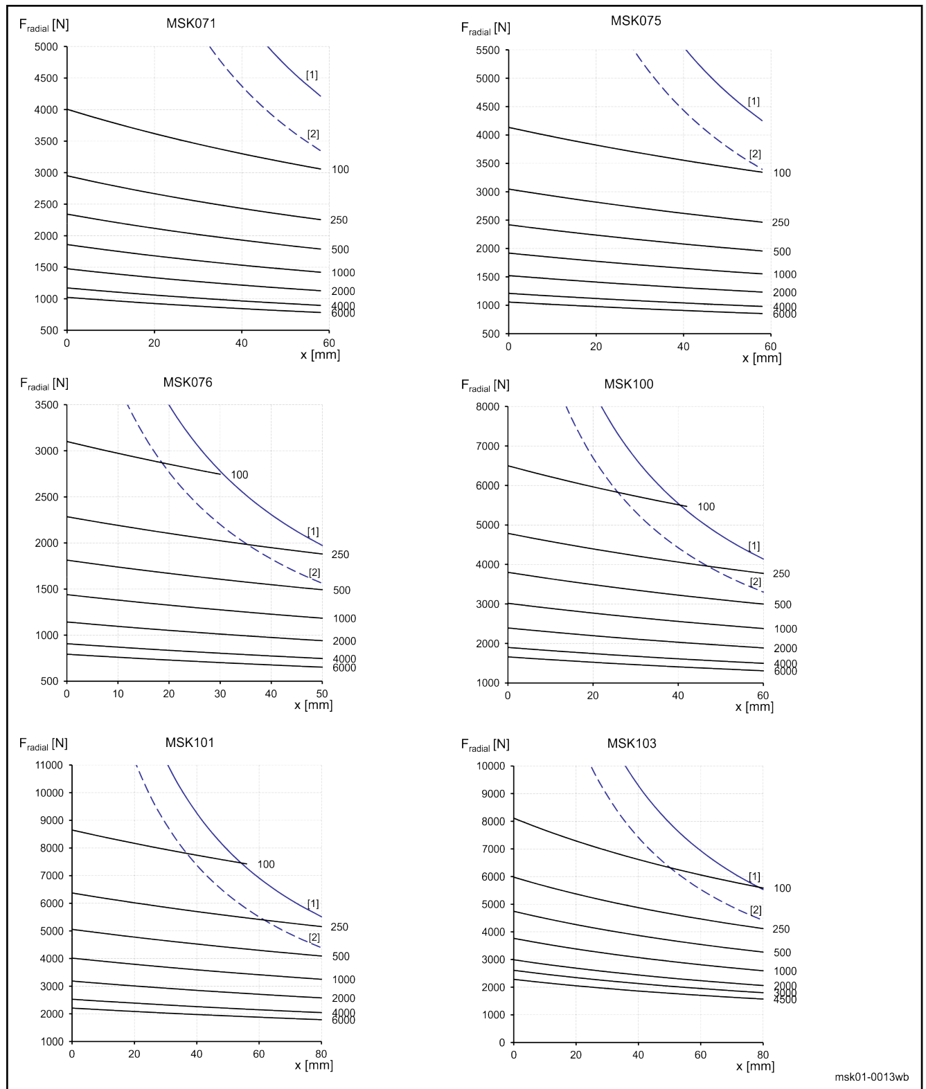
[1] Shaft plain [2] Shaft with keyway n [ \text{min}^{-1} ] Average speed Fig. 9-9: Radial force F_{radial}(2)
