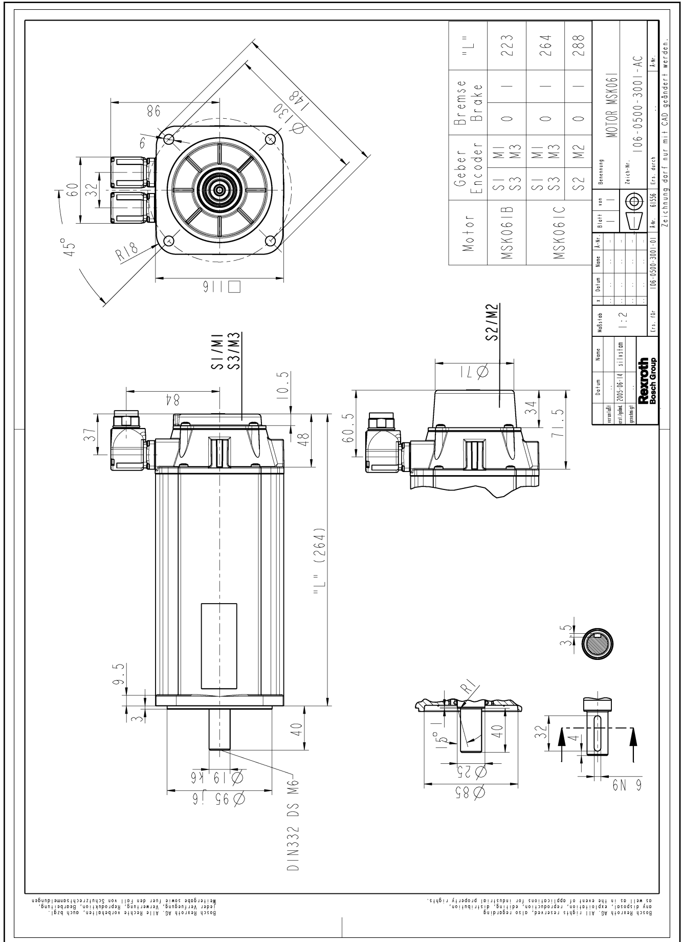
Fig. 5-8: MSK061 specification
