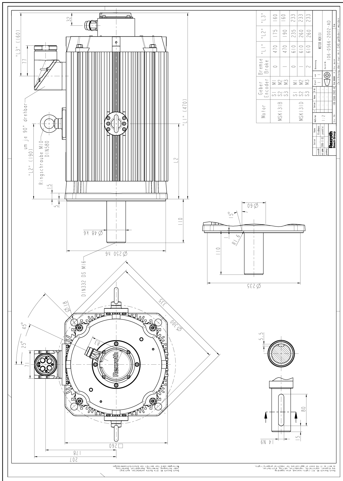
Fig. 5-33: MSK131 specification
