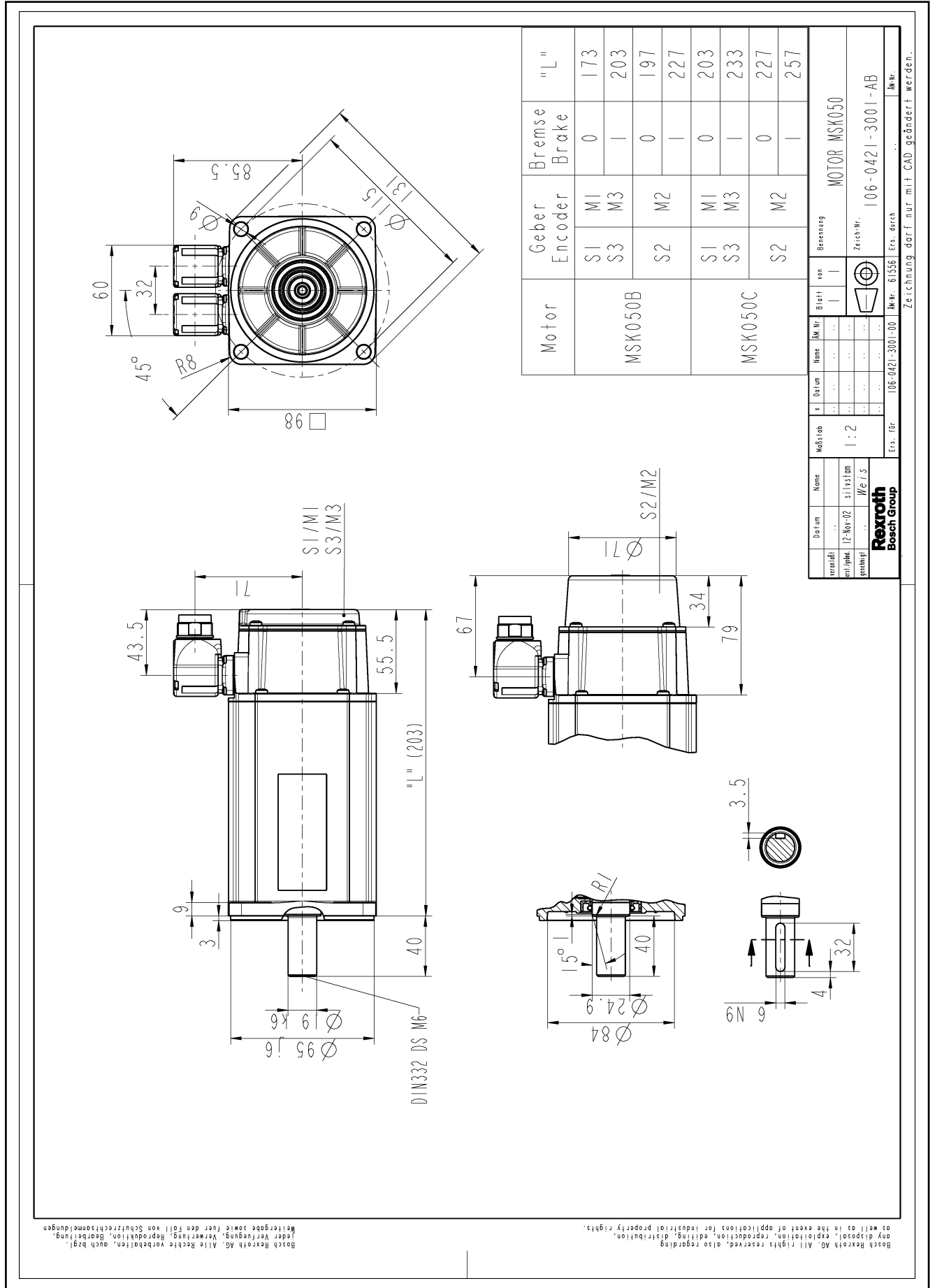
Fig. 5-4: MSK050 specification
