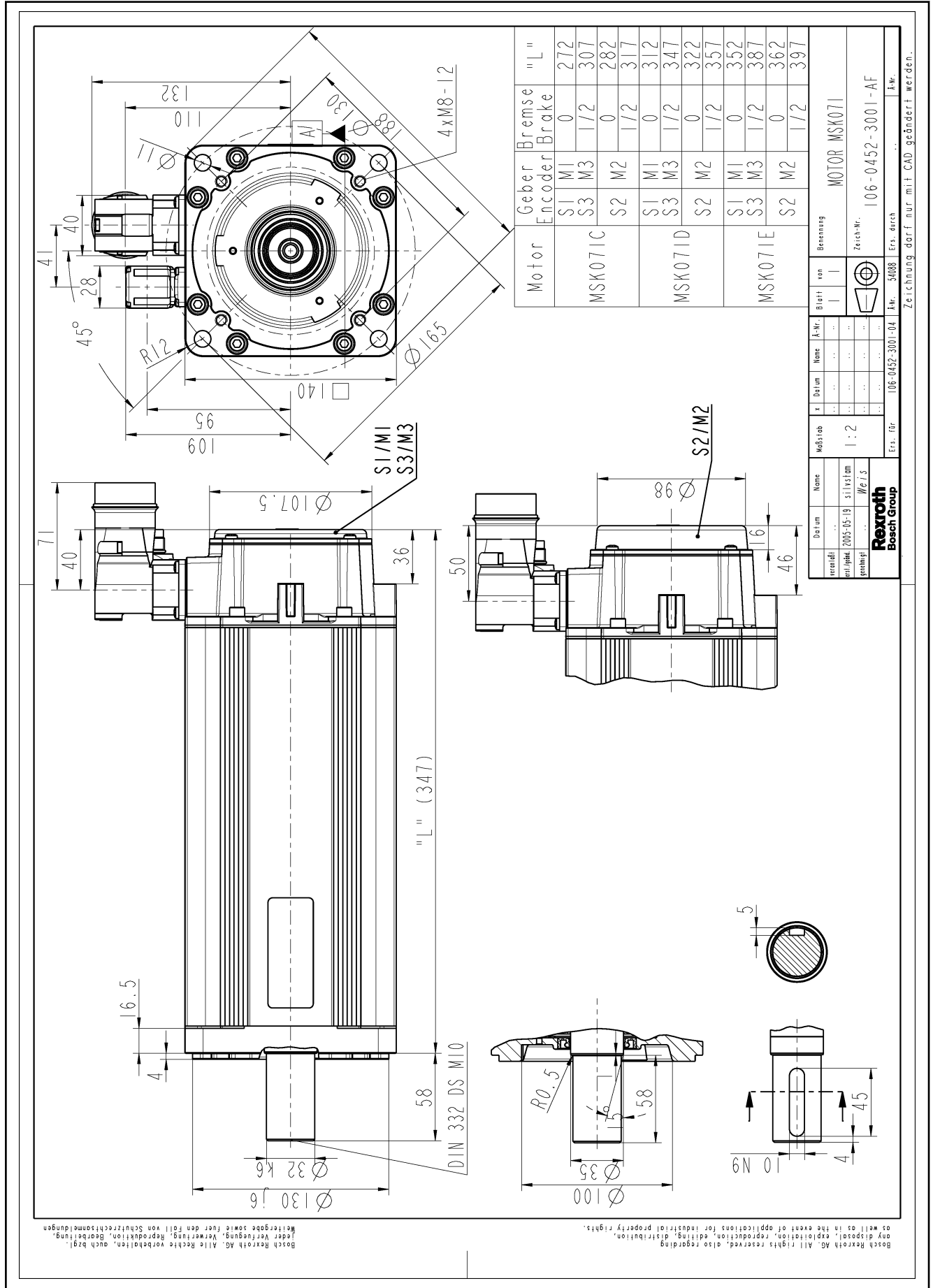
Fig. 5-14: MSK071...NN specification
