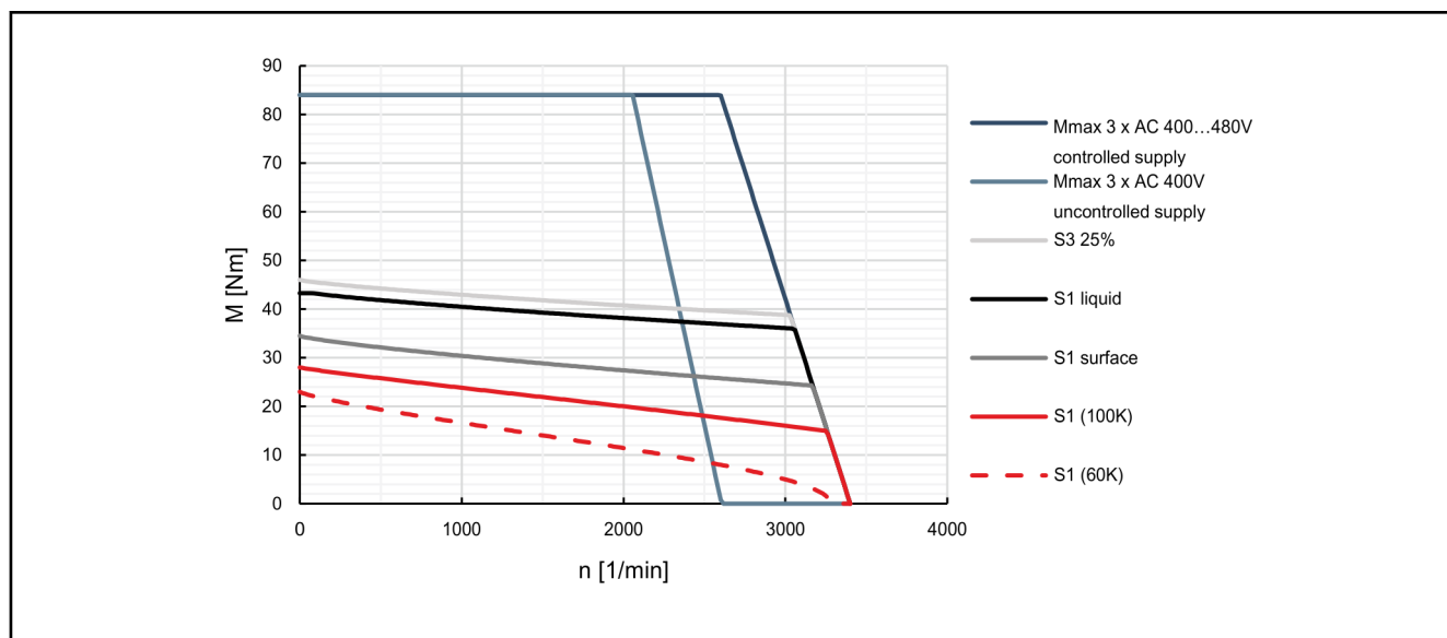
Fig. 4-39: Characteristic curves of motor MSK071E-0200
