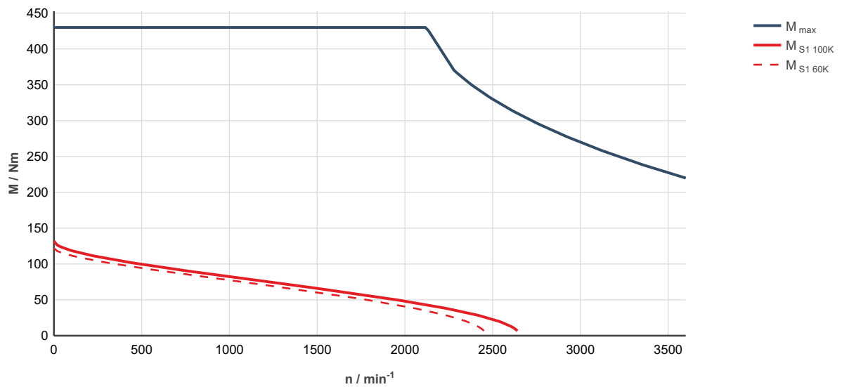
Fig. 309: MS2N13-C1BNN-___0-___-_, ctrIX DRIVE, uncontrolled supply 3 × AC 400 V M max : Characteristic curve applies to maximum torque 20 °C (cold)
