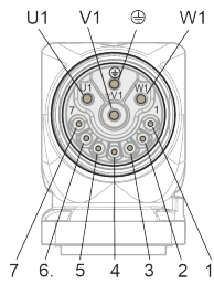
Fig. 379: Connector view of M23 single cable connector
