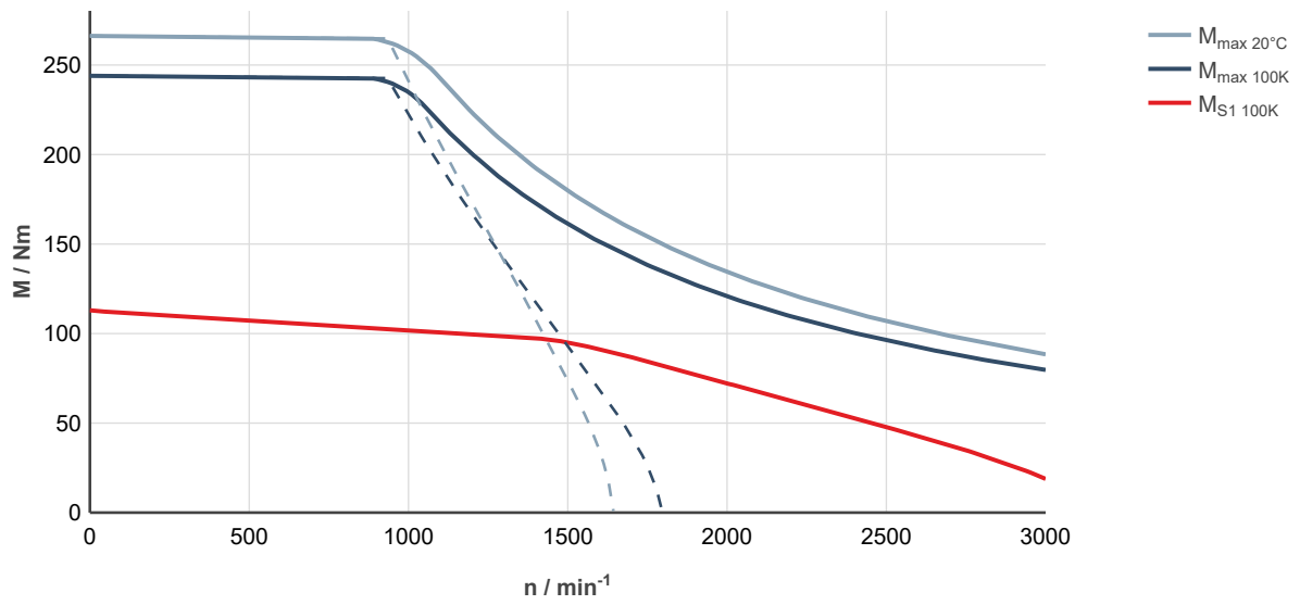
Fig. 249: MS2N10-E1BFA-___0-___-___, ctrlX DRIVE, uncontrolled supply 3 × AC 400 V
