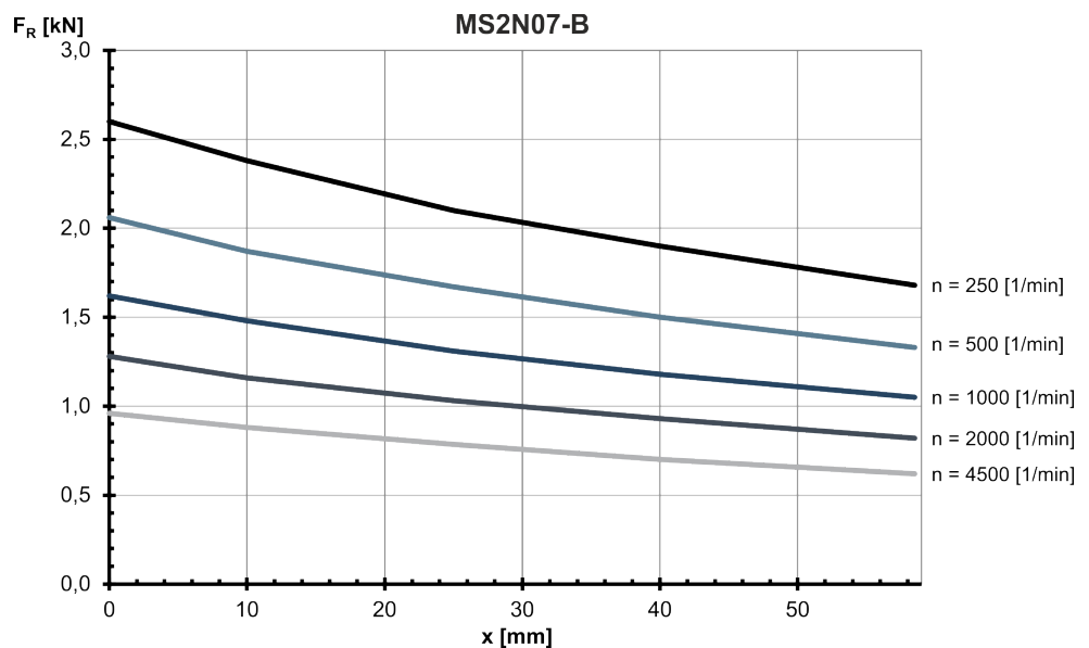
Fig. 189: MS2N07-B: Radial force in distance x from the shaft shoulder at a nominal bearing service life of L_{h10} = 30000 h
