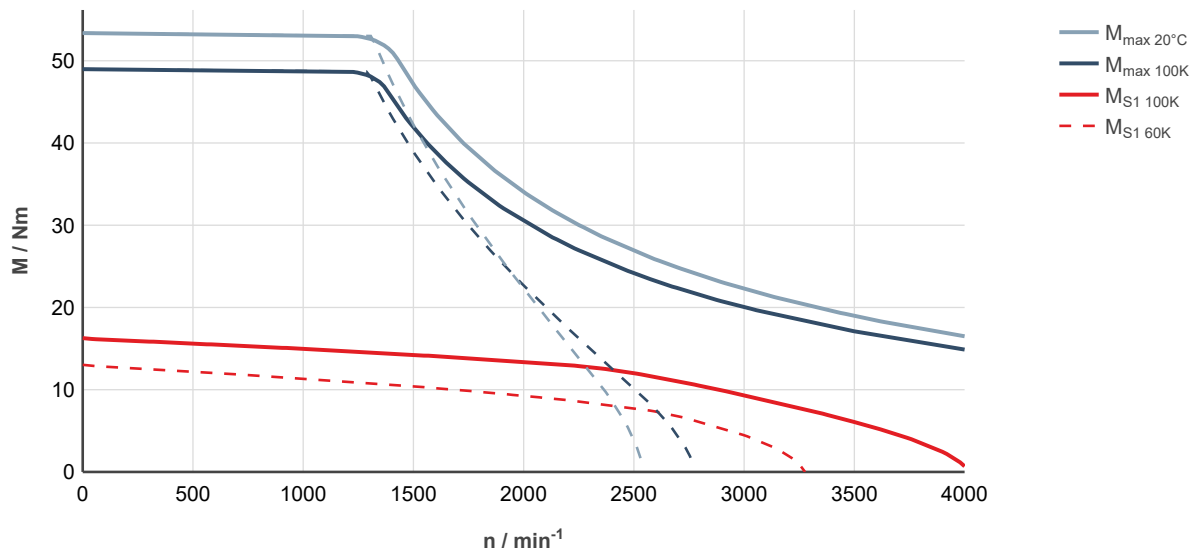
Fig. 81: MS2N06-E0BHN-___0-___-___, ctrlX DRIVE, uncontrolled supply 3 × AC 400 V
