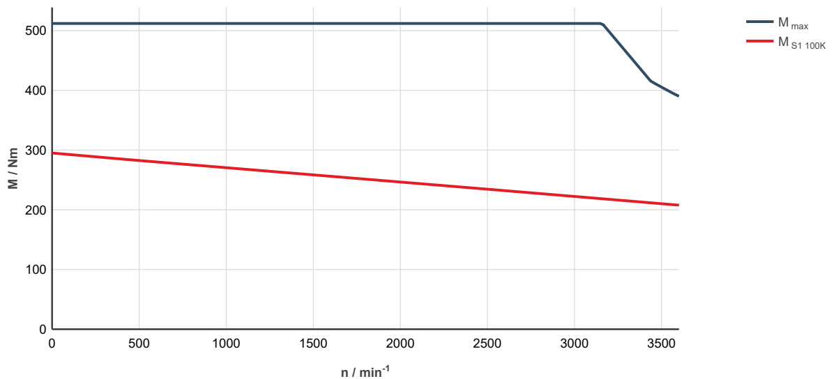
Fig. 346: MS2N13-D1BNL-___0-___-__, ctrlX DRIVE, controlled supply 3 x AC 400 ... 480 V M_{\text{max}} : Characteristic curve applies to maximum torque 20 °C (cold)
