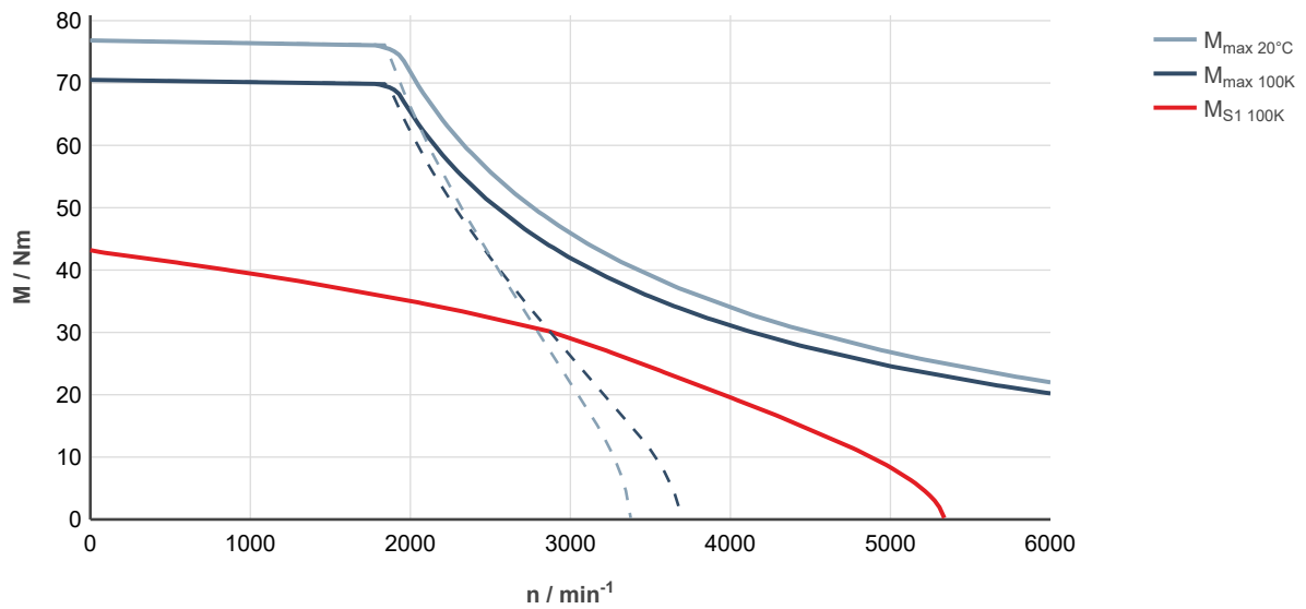
Fig. 231: MS2N10-C0BNA-___0-___-_, ctrlX DRIVE, uncontrolled supply 3 × AC 400 V
