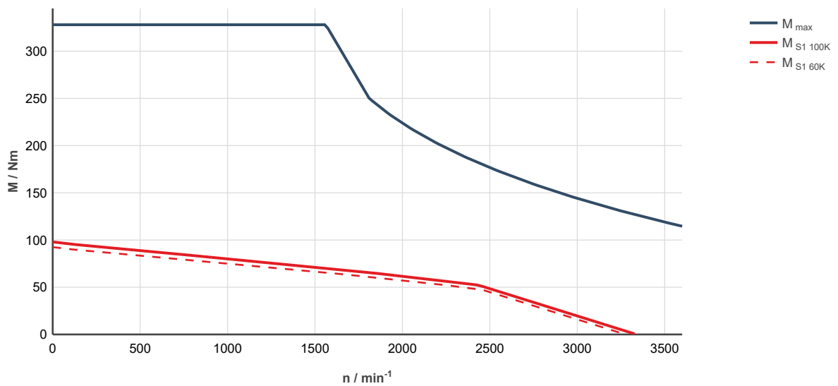
Fig. 303: MS2N13-B1BHN-___0-___-__ (modified), ctrlX DRIVE, uncontrolled supply 3 × AC 400 V M max : Characteristic curve applies to maximum torque 20 °C (cold)
