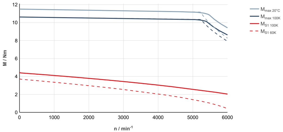
Fig. 55: MS2N05-B0BTN-___0-___-_, ctrlIX DRIVE, controlled supply 3 × AC 400 ... 480 V
