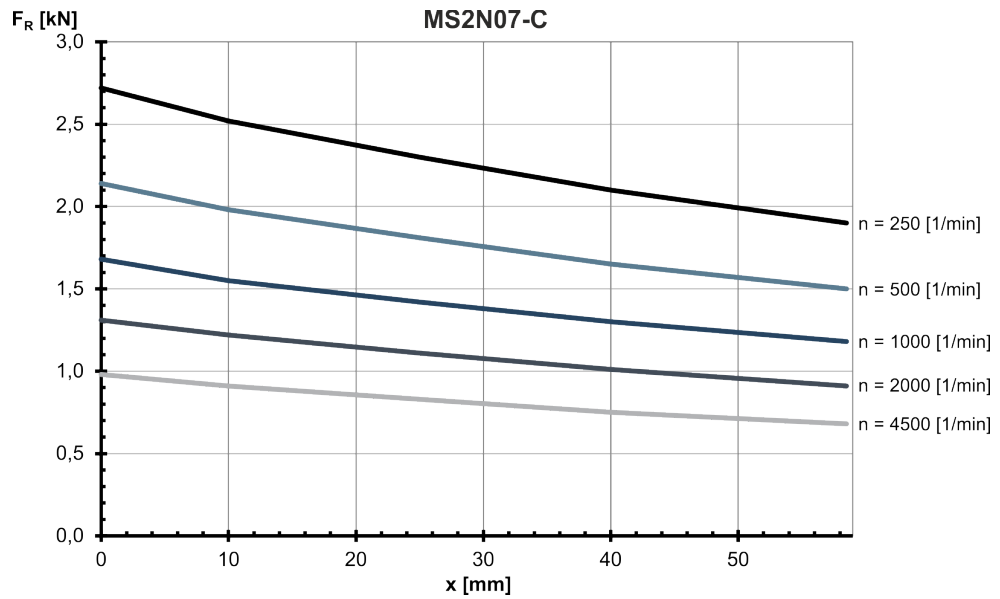
Fig. 190: MS2N07-C: Radial force in distance x from the shaft shoulder at a nominal bearing service life of L_{h10} = 30000 h
