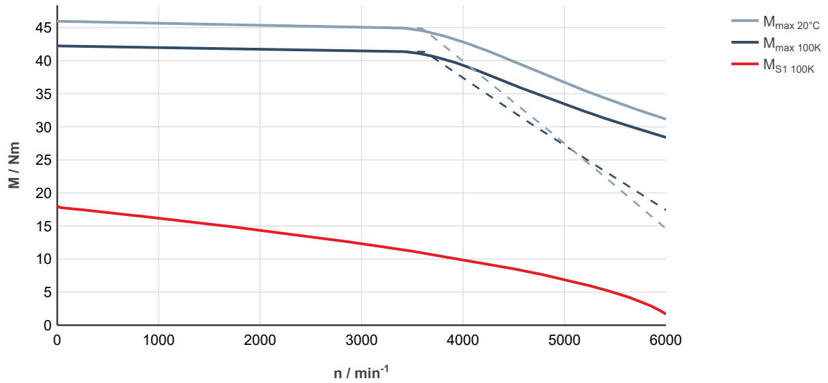
Fig. 135: MS2N07-C1BRA-___0-___-__, ctrlX DRIVE, controlled supply 3 × AC 400 ... 480 V
