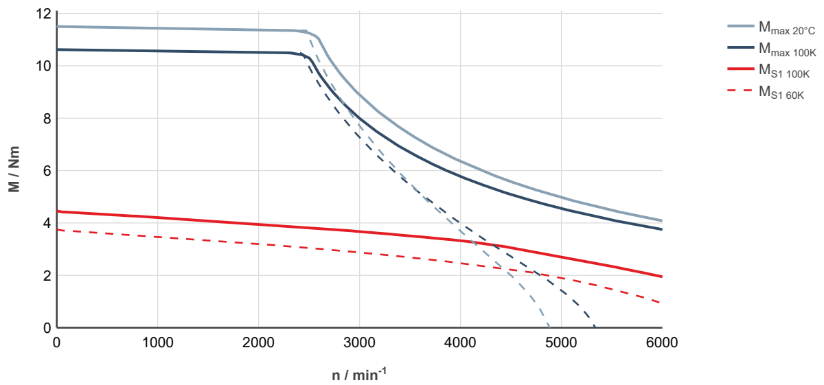
Fig. 53: MS2N05-B0BNN-___0-___-___, ctrlX DRIVE, controlled supply 3 × AC 400 ... 480 V
