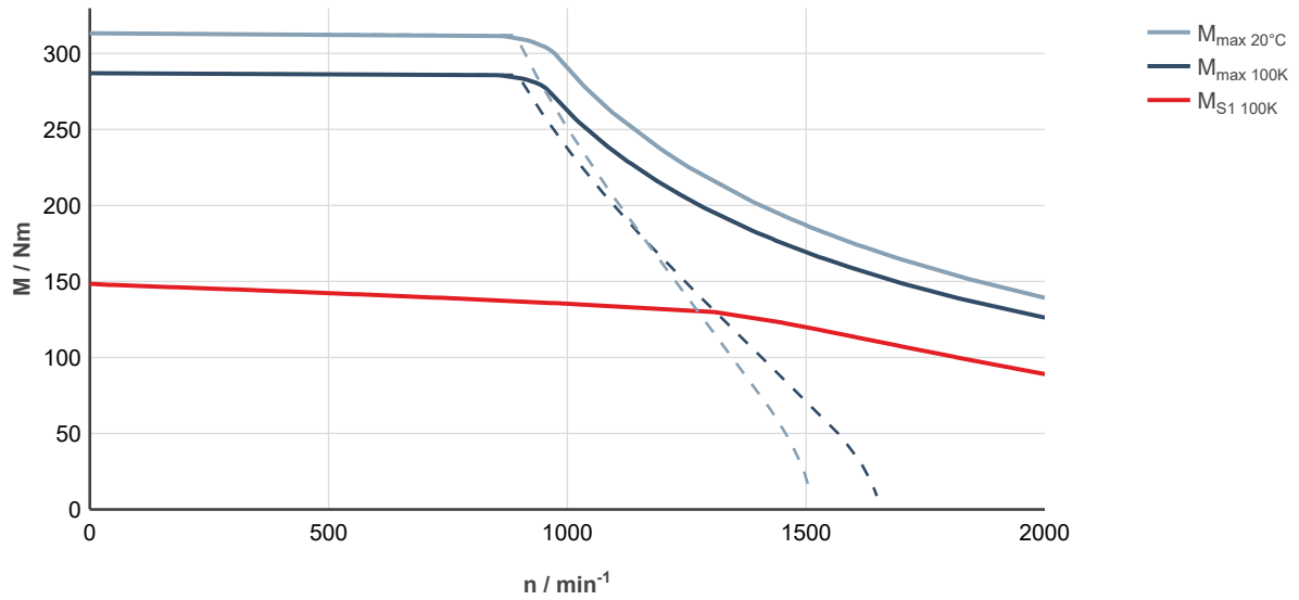
Fig. 254: MS2N10-F0BDA-___0-___-__, ctrlX DRIVE, controlled supply 3 × AC 400 ... 480 V
