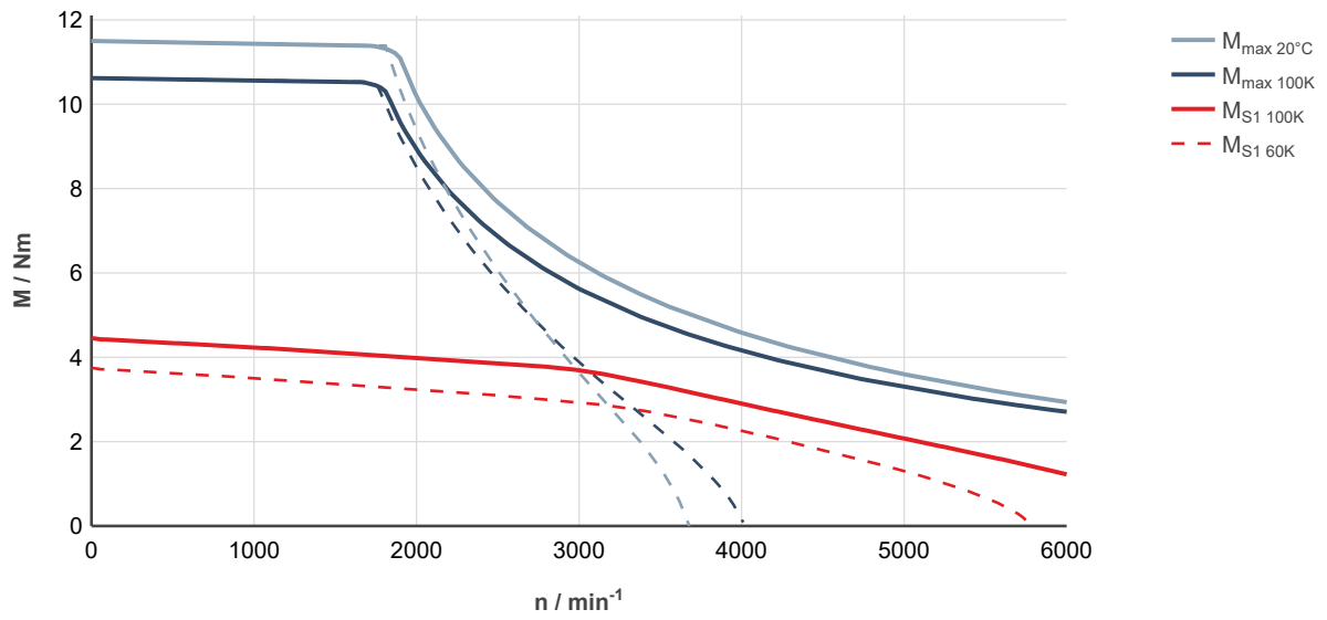
Fig. 52: MS2N05-B0BNN-___0-___-___, ctrlX DRIVE, uncontrolled supply 3 × AC 400 V
