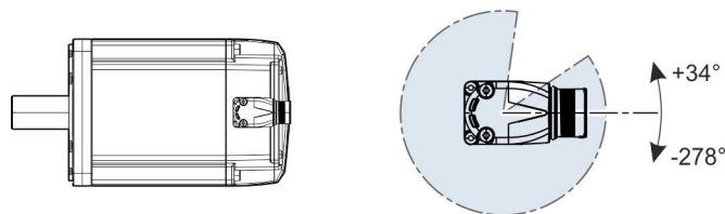
Fig. 380: Rotating area electrical connection "S"
