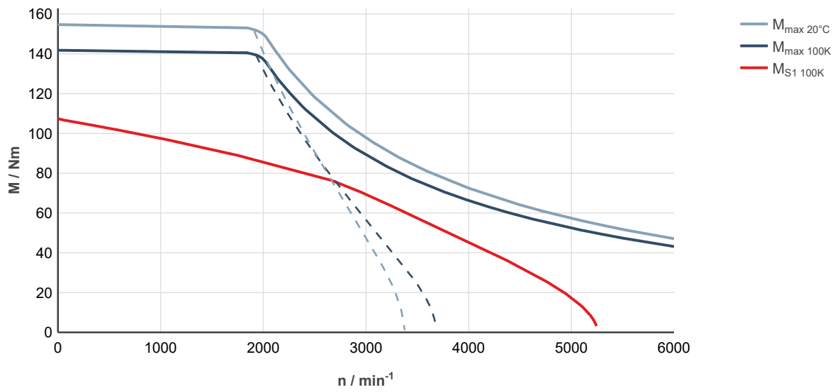
Fig. 271: MS2N10-D0BNL-___0-___-___, ctrIX DRIVE, uncontrolled supply 3 × AC 400 V
