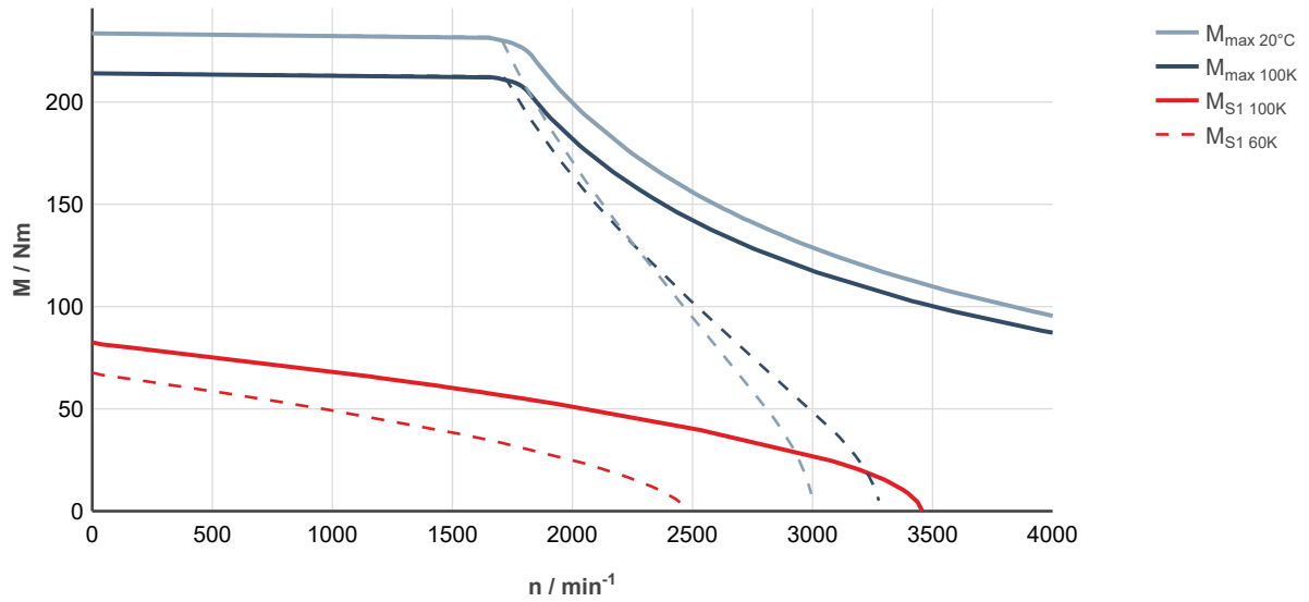
Fig. 212: MS2N10-E0BHN-___0-___-_, ctrlX DRIVE, controlled supply 3 × AC 400 ... 480 V
