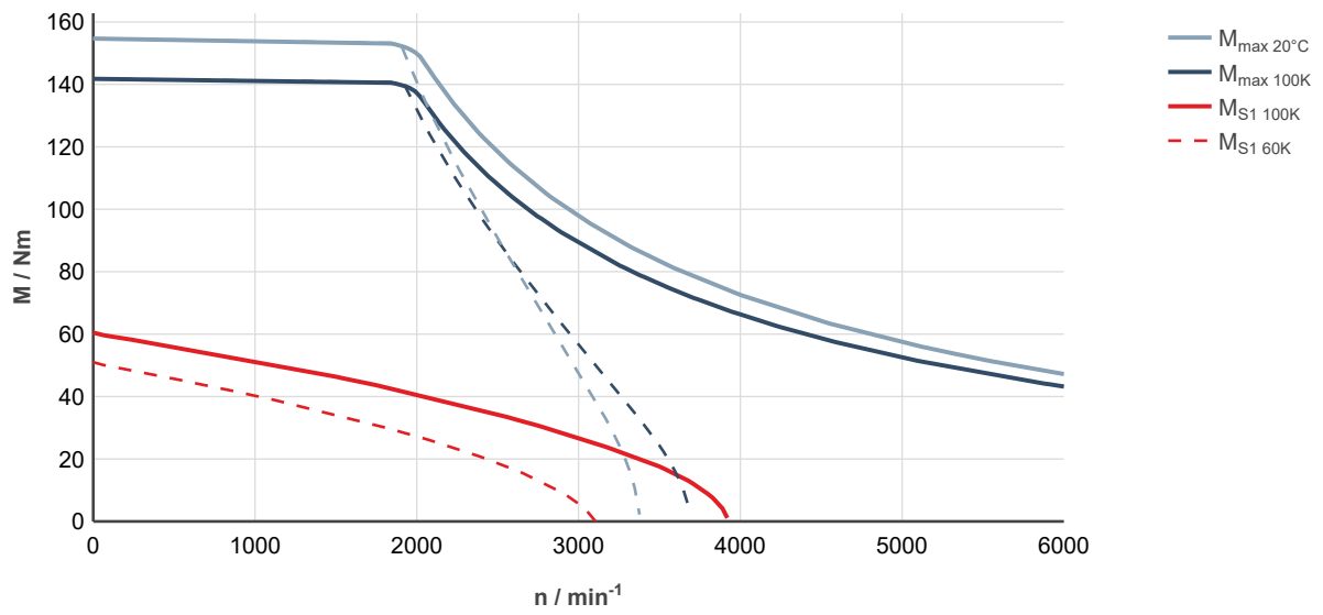
Fig. 205: MS2N10-D0BNN-___0-___-, ctrlX DRIVE, uncontrolled supply 3 × AC 400 V
