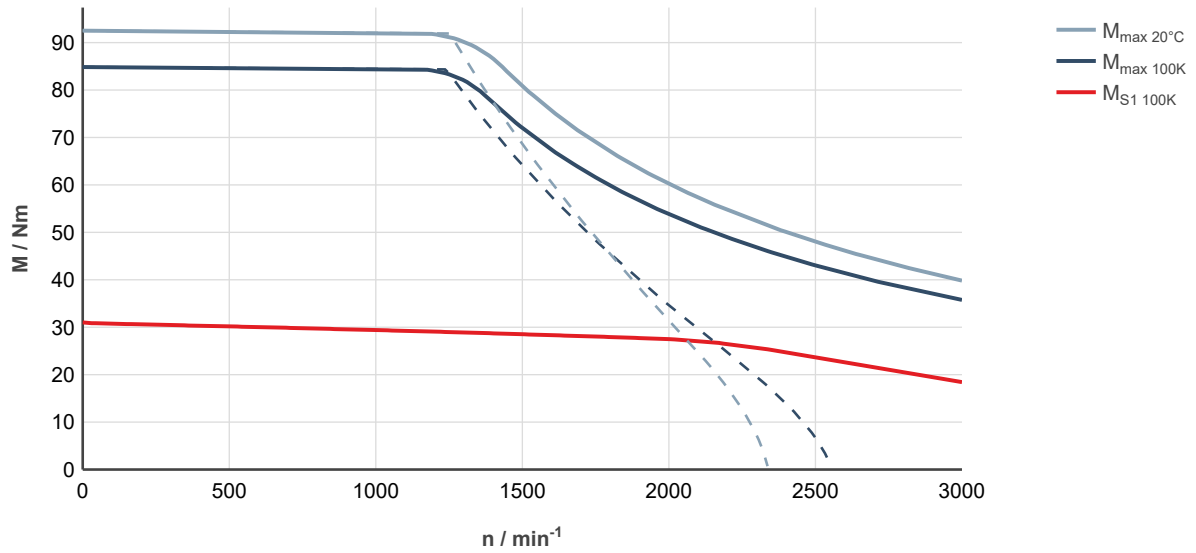
Fig. 145: MS2N07-D1BFA-___0-___-__, ctrlX DRIVE, controlled supply 3 × AC 400 ... 480 V
