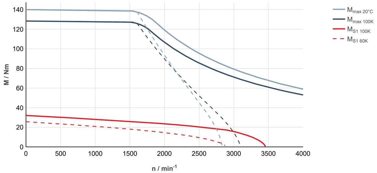
Fig. 125: MS2N07-E1BHN-___0-___-_, ctrlX DRIVE, controlled supply 3 × AC 400 ... 480 V
