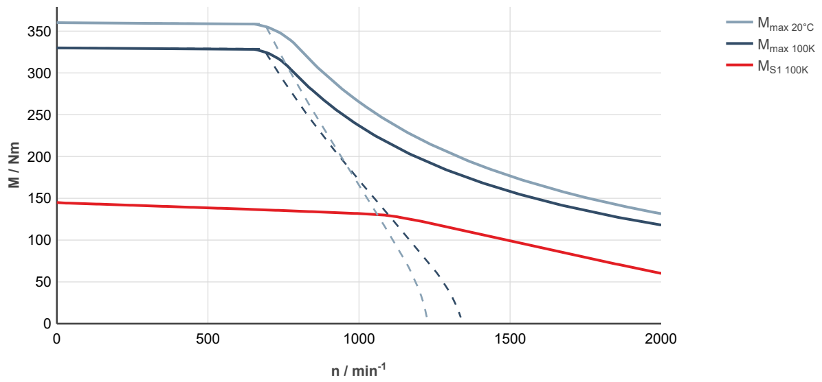
Fig. 257: MS2N10-F1BDA-___0-___-__, ctrlX DRIVE, uncontrolled supply 3 × AC 400 V
