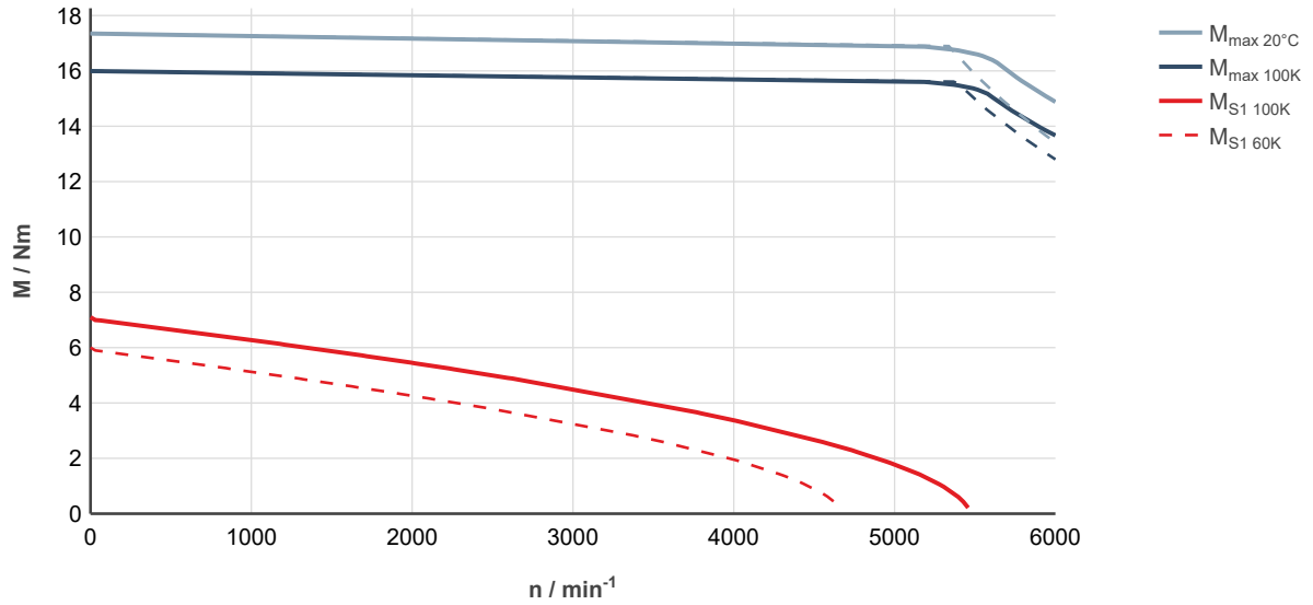
Fig. 74: MS2N06-C0BTN-___0-___-__, ctrlX DRIVE, controlled supply 3 × AC 400 ... 480 V
