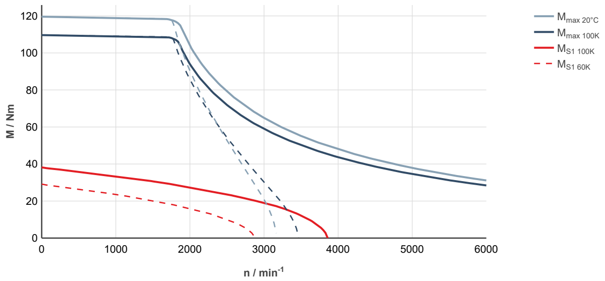
Fig. 118: MS2N07-E0BNN-___0-___-_, ctrlX DRIVE, uncontrolled supply 3 × AC 400 V
