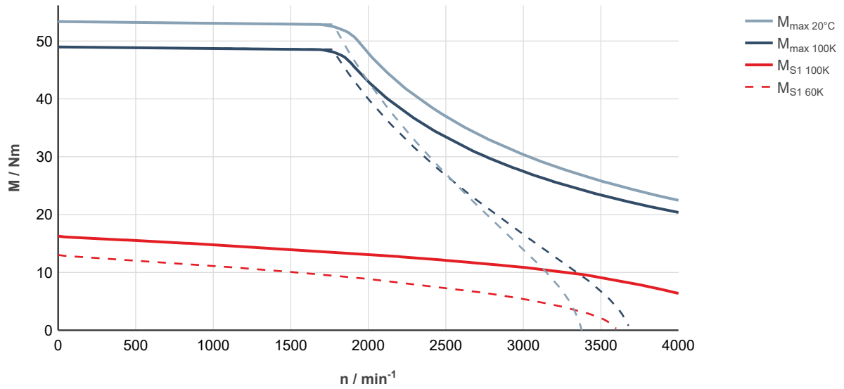
Fig. 82: MS2N06-E0BHN-___0-___-___, ctrlX DRIVE, controlled supply 3 × AC 400 ... 480 V
