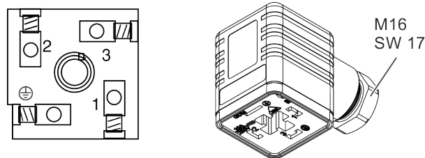
Fig. 387: RLSxxxx_Single components fan connector
