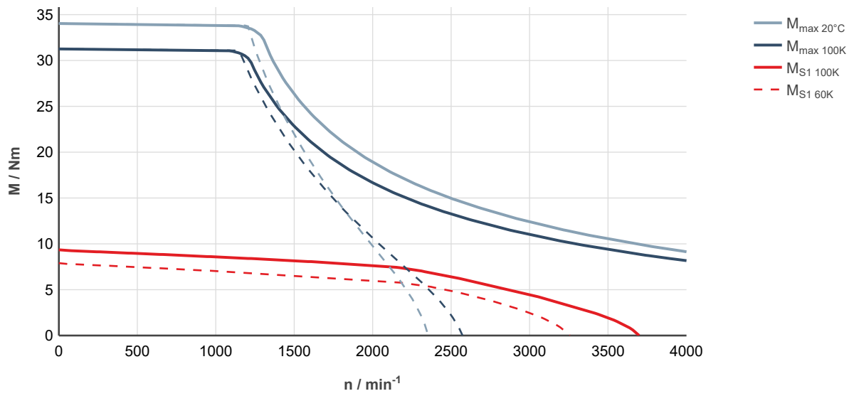
Fig. 60: MS2N05-D0BHN-___0-___-_, ctrIX DRIVE, uncontrolled supply 3 x AC 400 V
