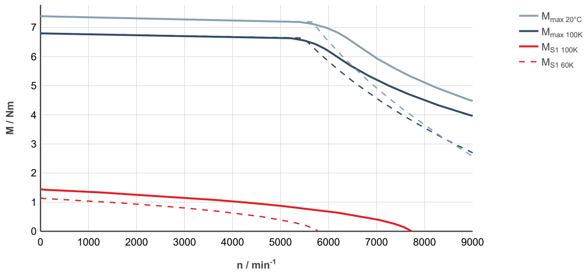
Fig. 28: MS2N03-D0BYN-___0-___-__, ctrlX DRIVE, uncontrolled supply 3 × AC 400 V
