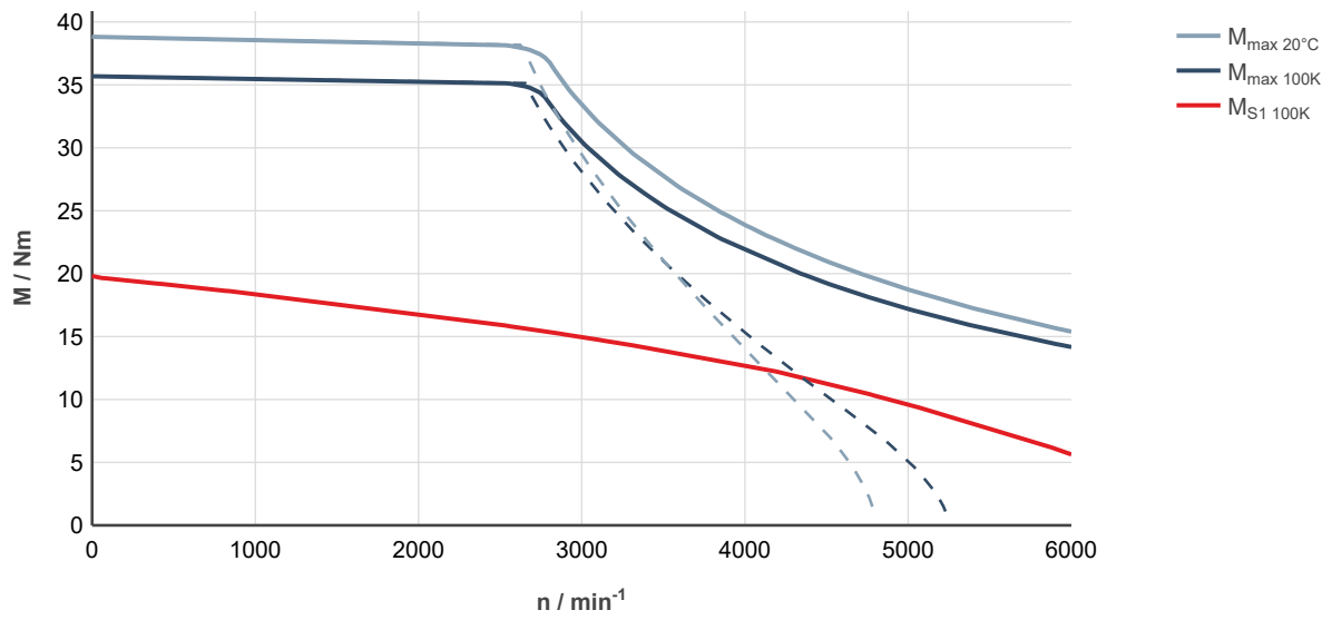
Fig. 130: MS2N07-C0BQA-___0-___-_, ctrlIX DRIVE, uncontrolled supply 3 × AC 400 V
