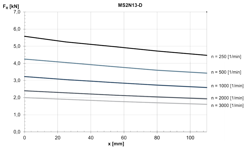
Fig. 356: MS2N13-D: Radial force in distance x from the shaft shoulder at a nominal bearing service life of L_{h10} = 30000 h
