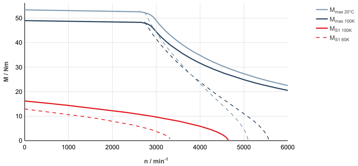
Fig. 83: MS2N06-E0BRN-___0-___-___, ctrlX DRIVE, uncontrolled supply 3 × AC 400 V
