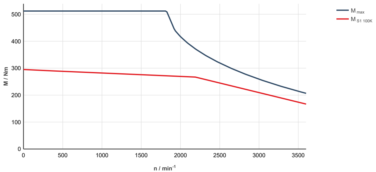
Fig. 343: MS2N13-D1BHL-___0-___-__, ctrlX DRIVE, uncontrolled supply 3 × AC 400 V M_{\text{max}} : Characteristic curve applies to maximum torque 20 °C (cold)
