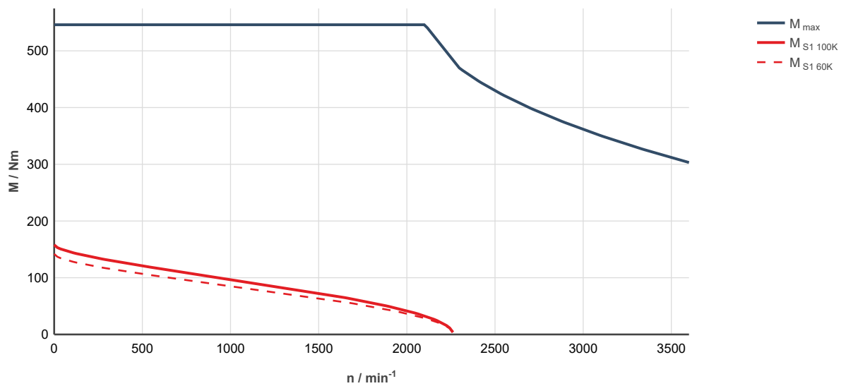
Fig. 313: MS2N13-D1BNN-___0-___-_, ctrlX DRIVE, uncontrolled supply 3 × AC 400 V M max : Characteristic curve applies to maximum torque 20 °C (cold)
