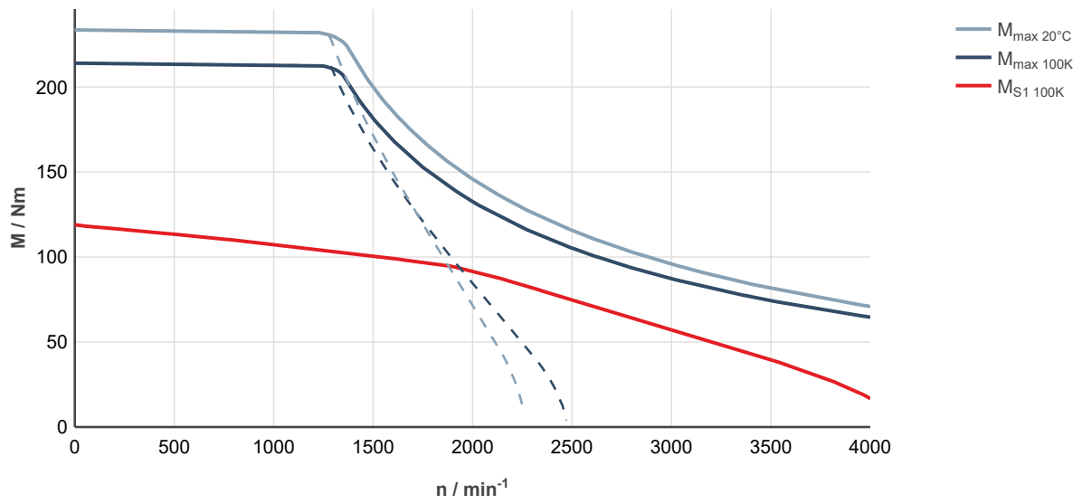
Fig. 245: MS2N10-E0BHA-___0-___-_, ctrIX DRIVE, uncontrolled supply 3 × AC 400 V
