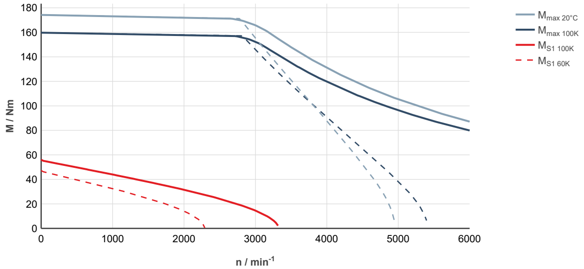
Fig. 210: MS2N10-D1BNN-___0-___-_, ctrlX DRIVE, controlled supply 3 × AC 400 ... 480 V
