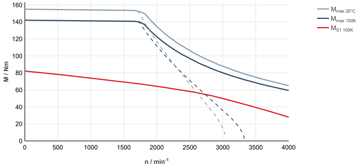
Fig. 238: MS2N10-D0BHA-___0-___-_, ctrlX DRIVE, controlled supply 3 × AC 400 ... 480 V
