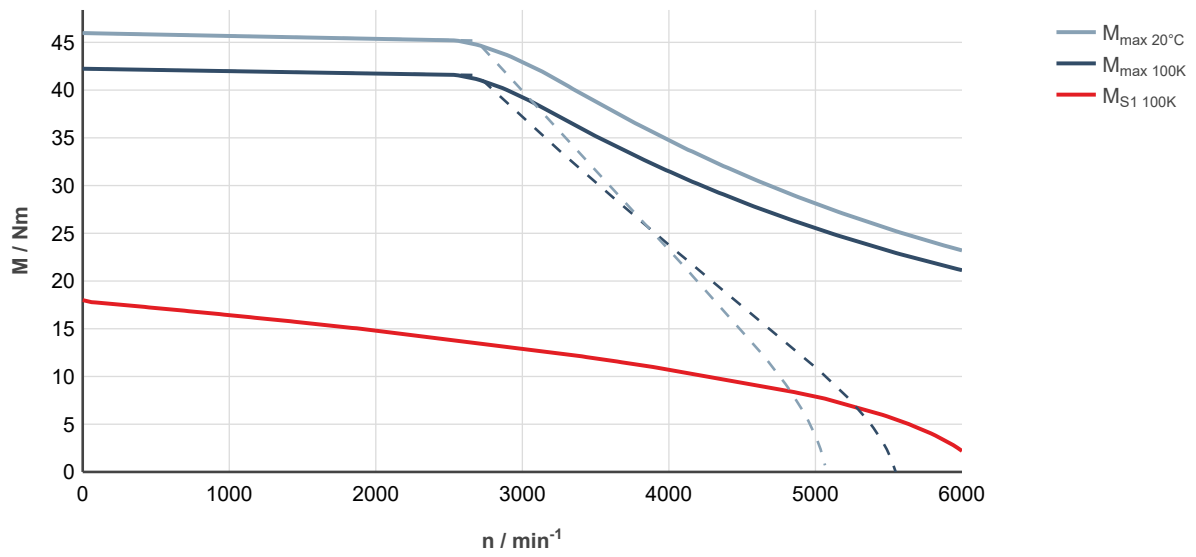
Fig. 134: MS2N07-C1BRA-___0-___-__, ctrlX DRIVE, uncontrolled supply 3 × AC 400 V
