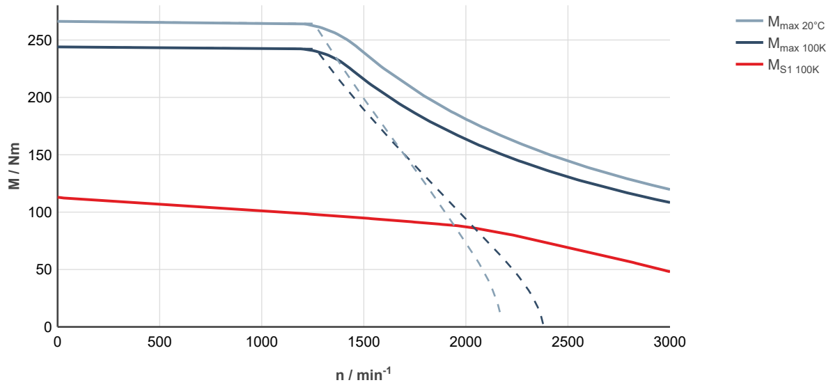
Fig. 250: MS2N10-E1BFA-___0-___-___, ctrlX DRIVE, controlled supply 3 × AC 400 ... 480 V
