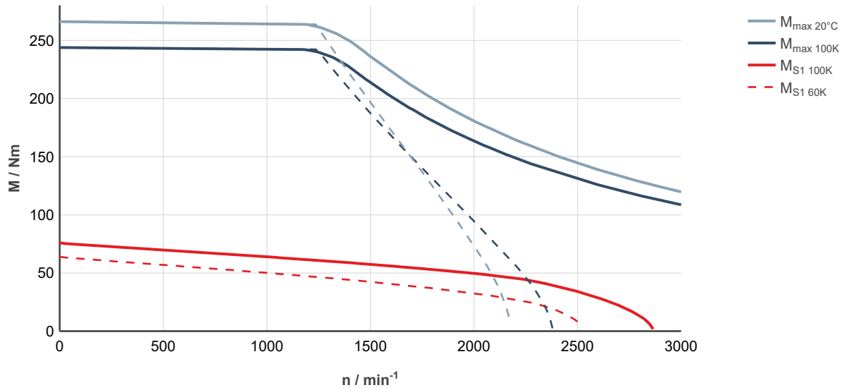
Fig. 216: MS2N10-E1BFN-___0-___-__, ctrlX DRIVE, controlled supply 3 × AC 400 ... 480 V
