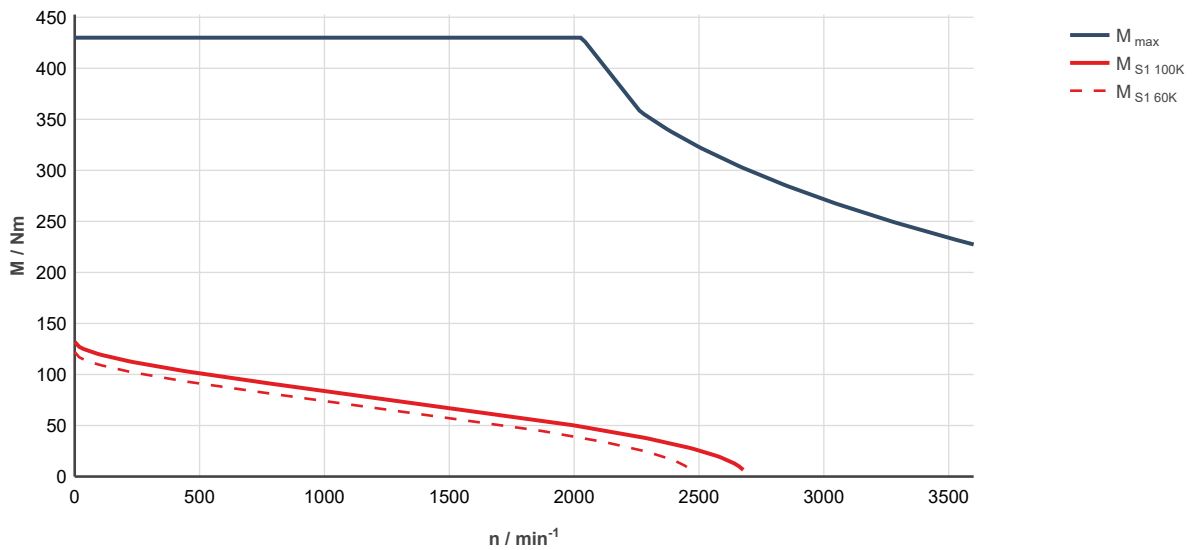
Fig. 308: MS2N13-C1BHN-___0-___-_, ctrIX DRIVE, controlled supply 3 x AC 400 ... 480 V M_{max} : Characteristic curve applies to maximum torque 20 °C (cold)
