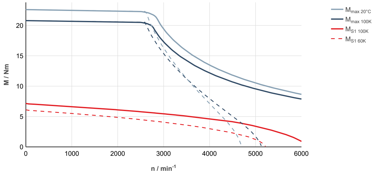
Fig. 57: MS2N05-C0BNN-___0-___-_, ctrlX DRIVE, controlled supply 3 × AC 400 ... 480 V
