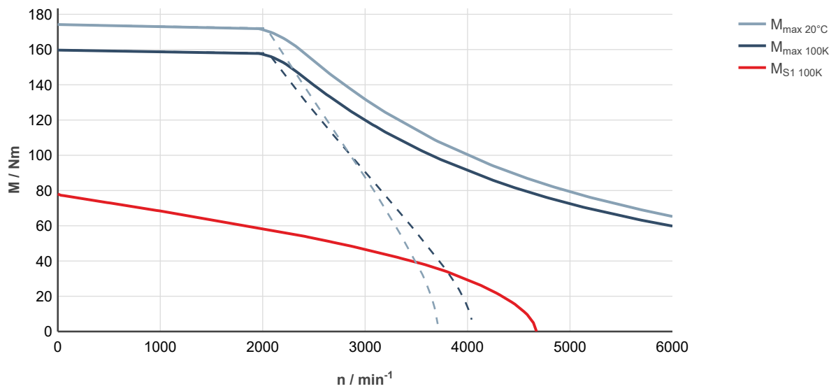
Fig. 243: MS2N10-D1BNA-___0-___-_, ctrlX DRIVE, uncontrolled supply 3 × AC 400 V
