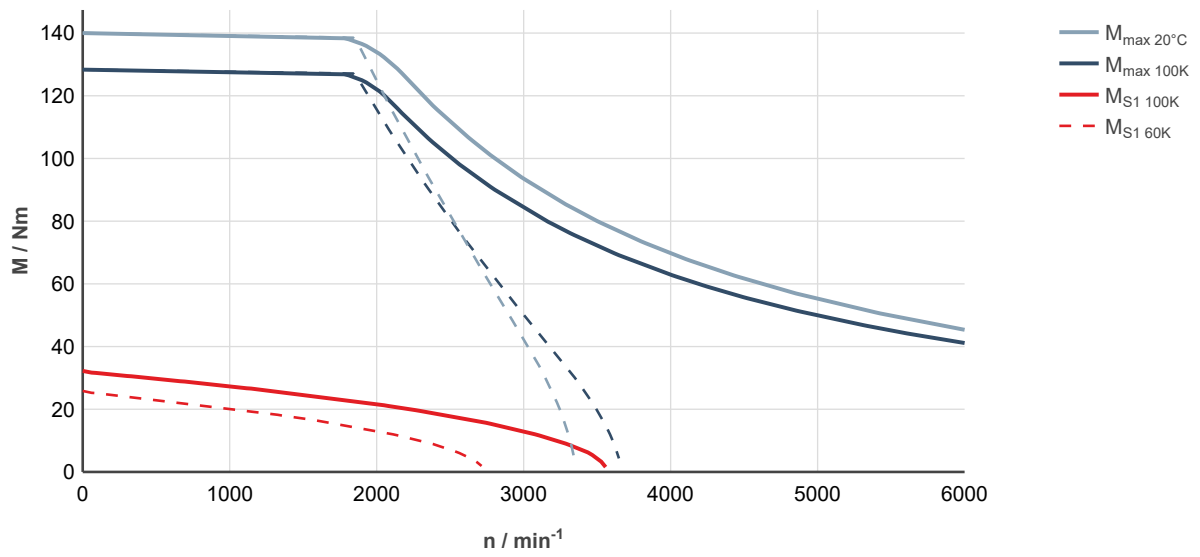
Fig. 126: MS2N07-E1BNN-___0-___-_, ctrlX DRIVE, uncontrolled supply 3 × AC 400 V
