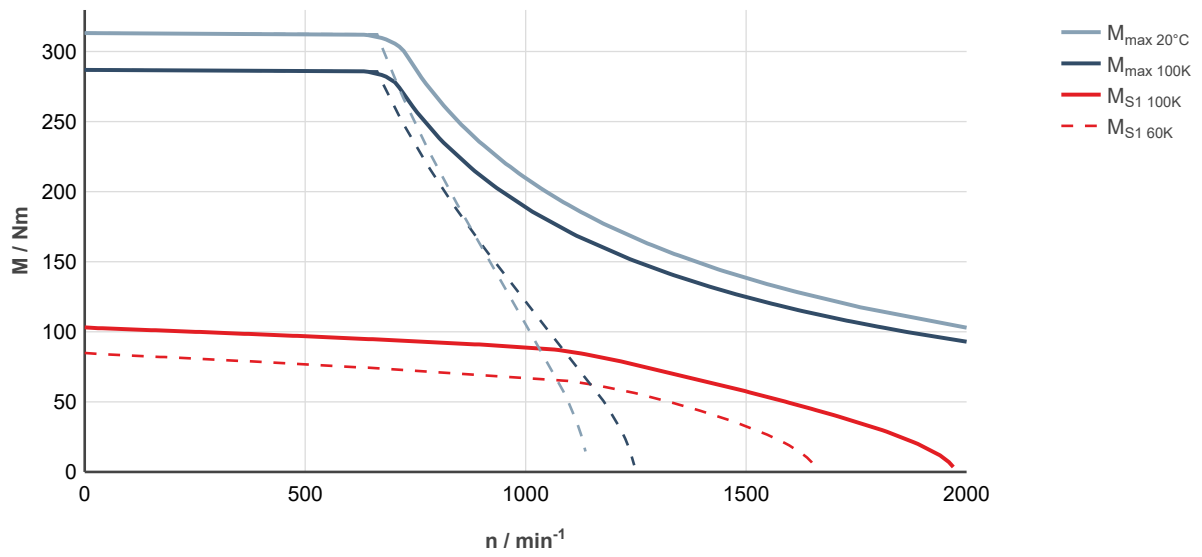
Fig. 219: MS2N10-F0BDN-___0-___-_, ctrlX DRIVE, uncontrolled supply 3 × AC 400 V
