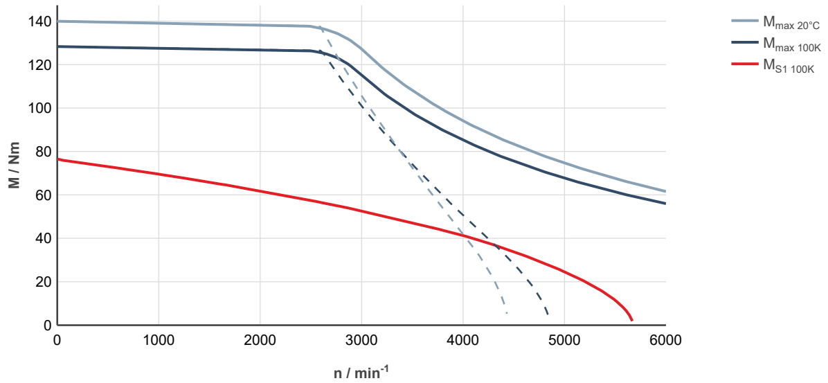
Fig. 185: MS2N07-E1BNL-__0-__-__, ctrlX DRIVE, controlled supply 3 × AC 400 ... 480 V
