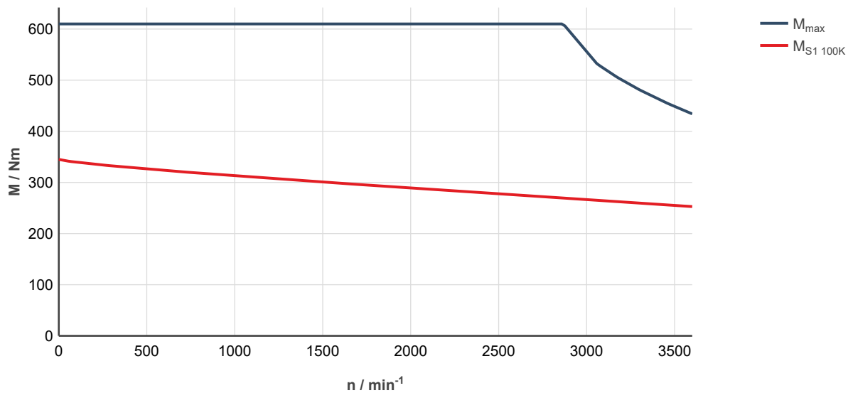
Fig. 350: MS2N13-E1BNL-__0-__-__, ctrlX DRIVE, controlled supply 3 × AC 400 ... 480 V M_{\text{max}} : Characteristic curve applies to maximum torque 20 °C (cold)
