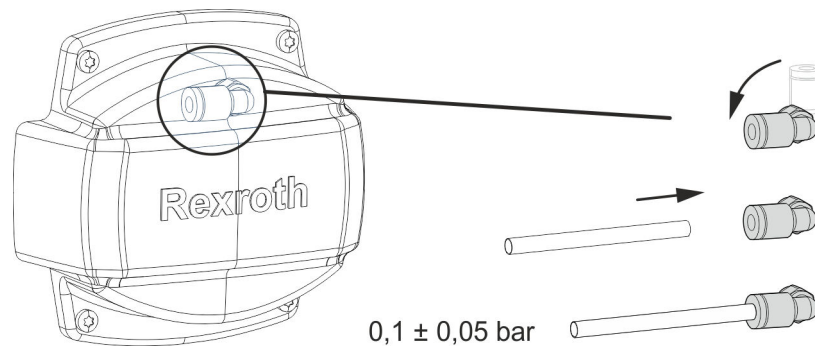
Fig. 398: Connection compressed air hose for using sealing air.
