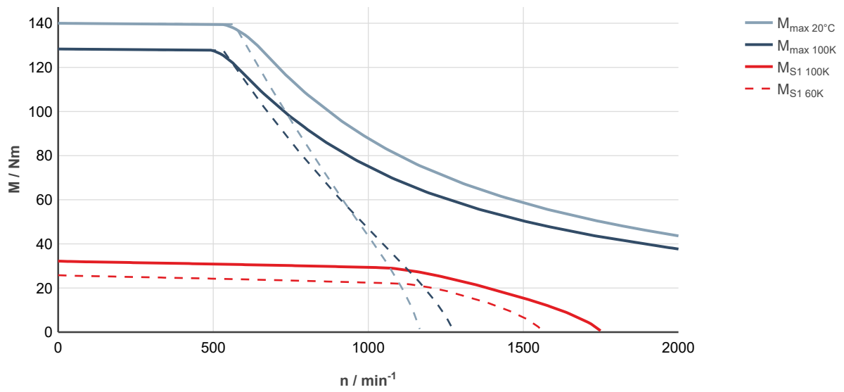
Fig. 122: MS2N07-E1BDN-___0-___-_, ctrlX DRIVE, uncontrolled supply 3 × AC 400 V
