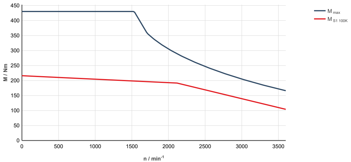
Fig. 323: MS2N13-C1BHC-___0-___-_, ctrIX DRIVE, uncontrolled supply 3 × AC 400 V M_{\text{max}} Characteristic curve applies to maximum torque 20 °C (cold)
