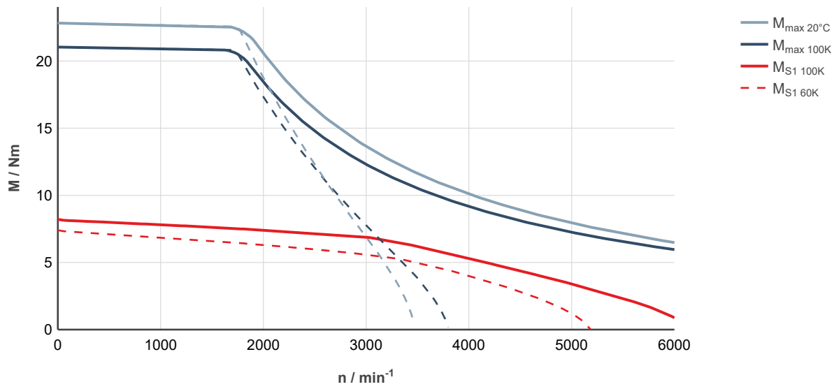
Fig. 90: MS2N07-B1BNN-___0-___-, ctrlX DRIVE, uncontrolled supply 3 × AC 400 V
