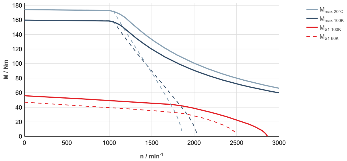
Fig. 207: MS2N10-D1BFN-___0-___-_, ctrlX DRIVE, uncontrolled supply 3 × AC 400 V
