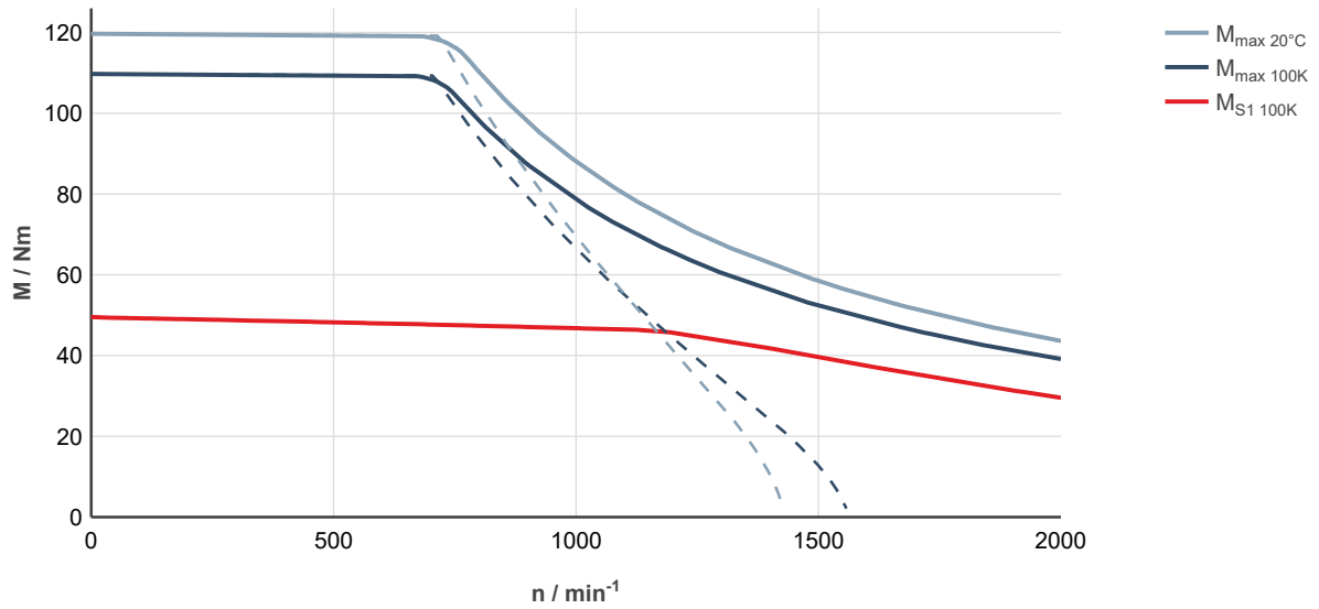
Fig. 151: MS2N07-E0BDA-___0-___-___, ctrlX DRIVE, controlled supply 3 × AC 400 ... 480 V
