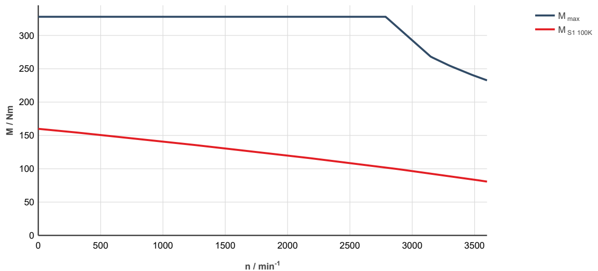
Fig. 322: MS2N13-B1BNC-___0-___-_, ctrIX DRIVE, controlled supply 3 x AC 400 ... 480 V M_{\text{max}} : Characteristic curve applies to maximum torque 20 °C (cold)
