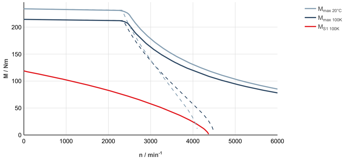
Fig. 248: MS2N10-E0BNA-___0-___-_, ctrIX DRIVE, controlled supply 3 × AC 400 ... 480 V
