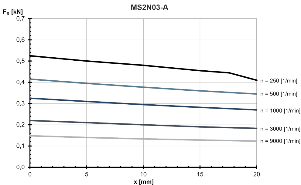
Fig. 32: MS2N03-A: Radial force in distance x from the shaft shoulder at a nominal bearing service life of L_{h10} = 30000 h
