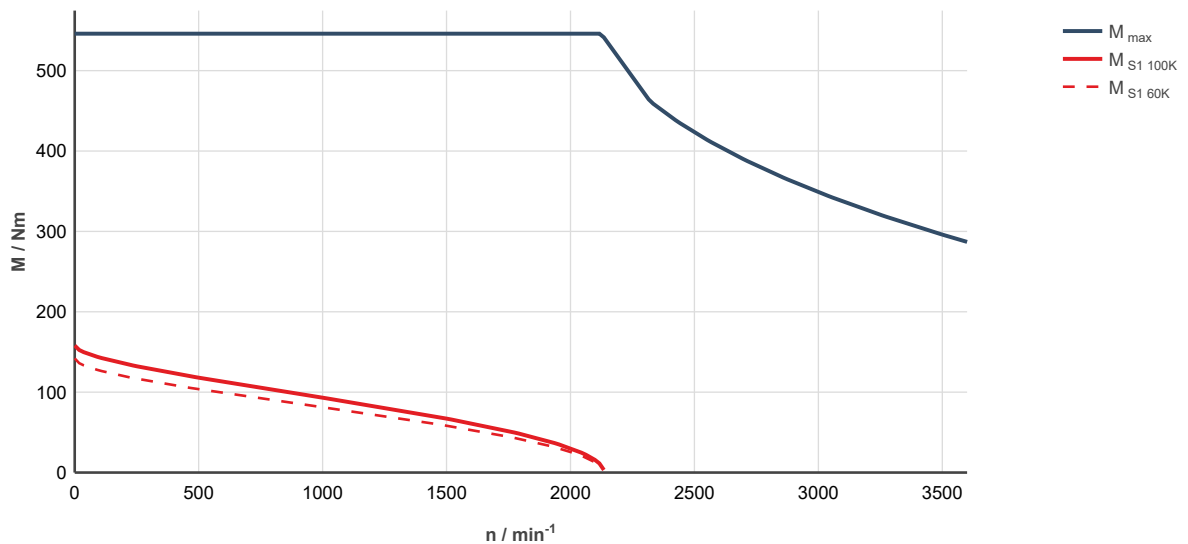
Fig. 312: MS2N13-D1BHN-___0-___-_, ctrIX DRIVE, controlled supply 3 x AC 400 ... 480 V M_{\max} : Characteristic curve applies to maximum torque 20 °C (cold)
