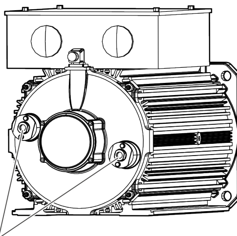
Fig. 395: Coolant connection MS2N13-__L__E__
