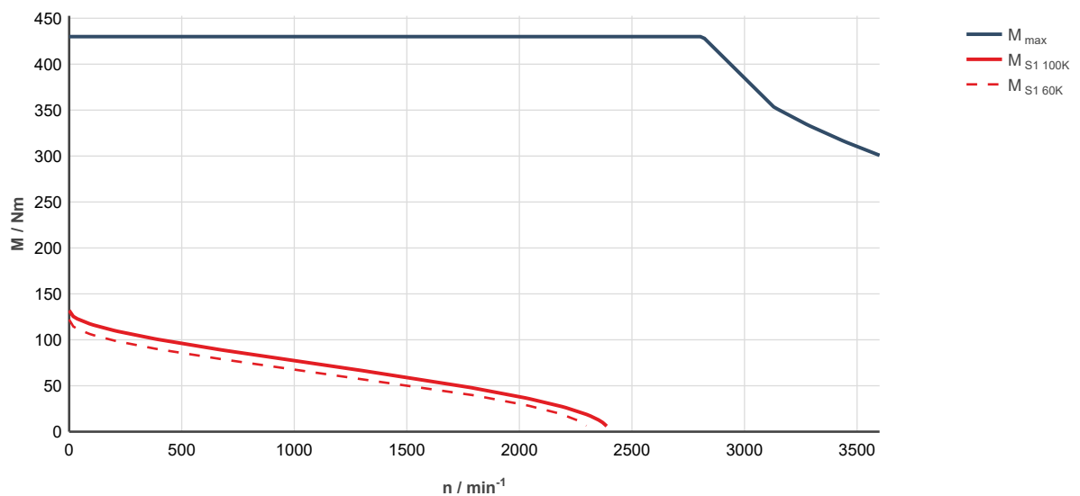
Fig. 310: MS2N13-C1BNN-___0-___-_, ctrIX DRIVE, controlled supply 3 x AC 400 ... 480 V M max : Characteristic curve applies to maximum torque 20 °C (cold)
