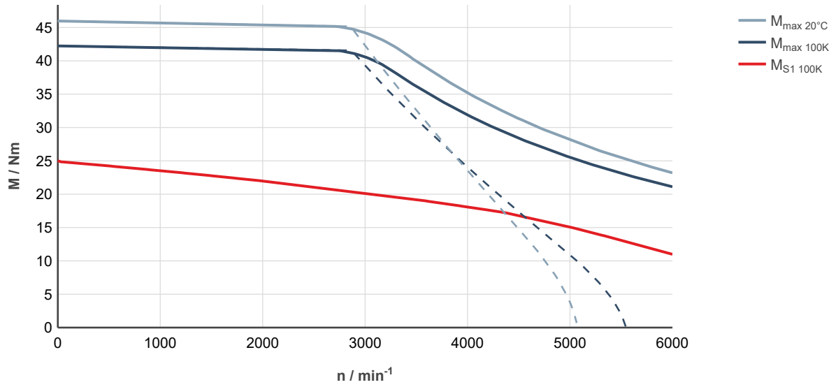
Fig. 168: MS2N07-C1BRL-___0-___-___, ctrIX DRIVE, uncontrolled supply 3 × AC 400 V
