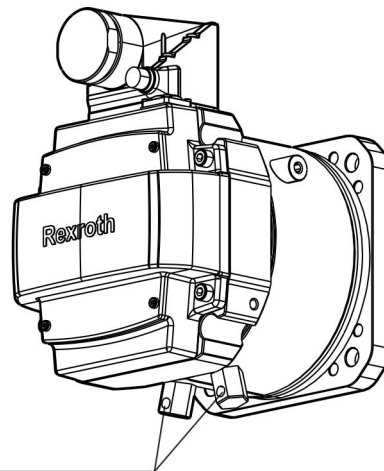
Fig. 391: Coolant connection MS2N10-__L__B__
