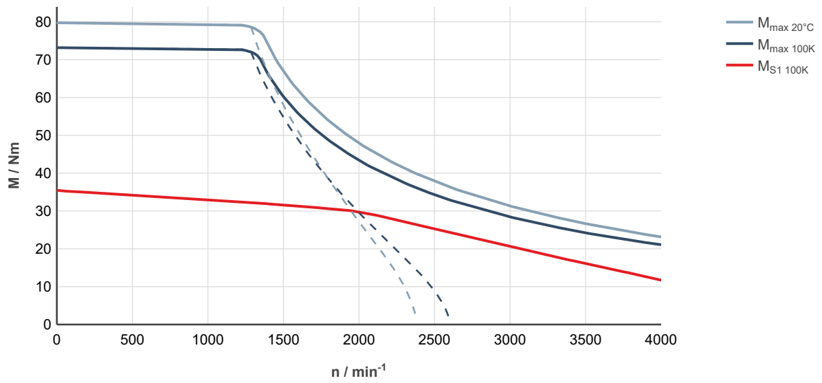
Fig. 138: MS2N07-D0BHA-___0-___-_, ctrlX DRIVE, uncontrolled supply 3 × AC 400 V
