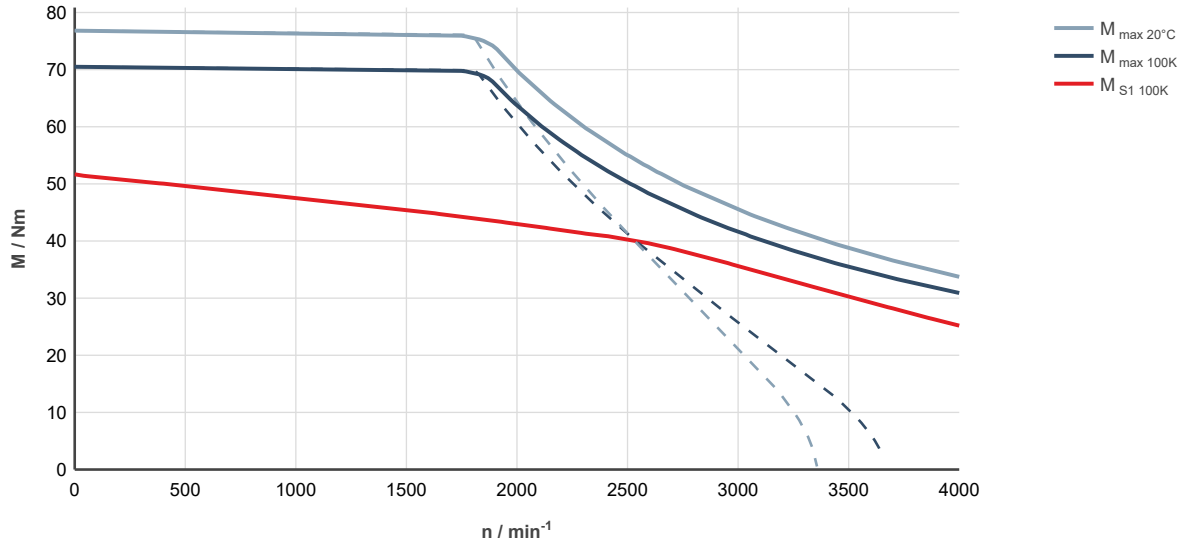
Fig. 264: MS2N10-C0BHL-___0-___-_0, ctrlX DRIVE, controlled supply 3 x AC 400 ... 480 V
