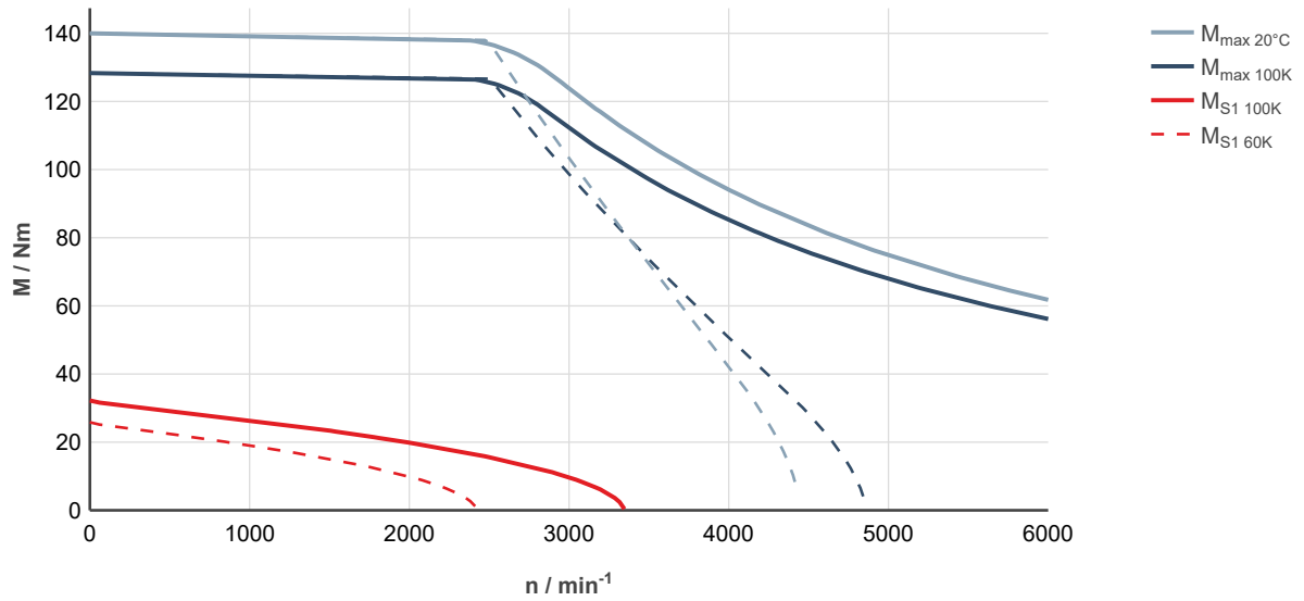
Fig. 127: MS2N07-E1BNN-___0-___-_, ctrlX DRIVE, controlled supply 3 × AC 400 ... 480 V
