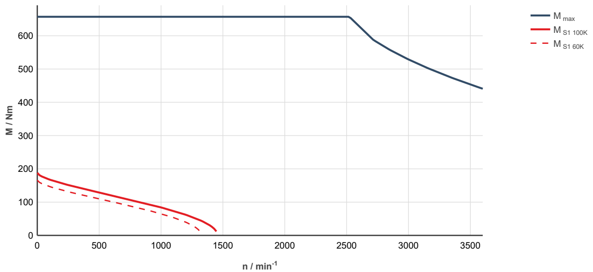
Fig. 318: MS2N13-E1BNN-___0-___-_, ctrlX DRIVE, controlled supply 3 x AC 400 ... 480 V M_{max} : Characteristic curve applies to maximum torque 20 °C (cold)
