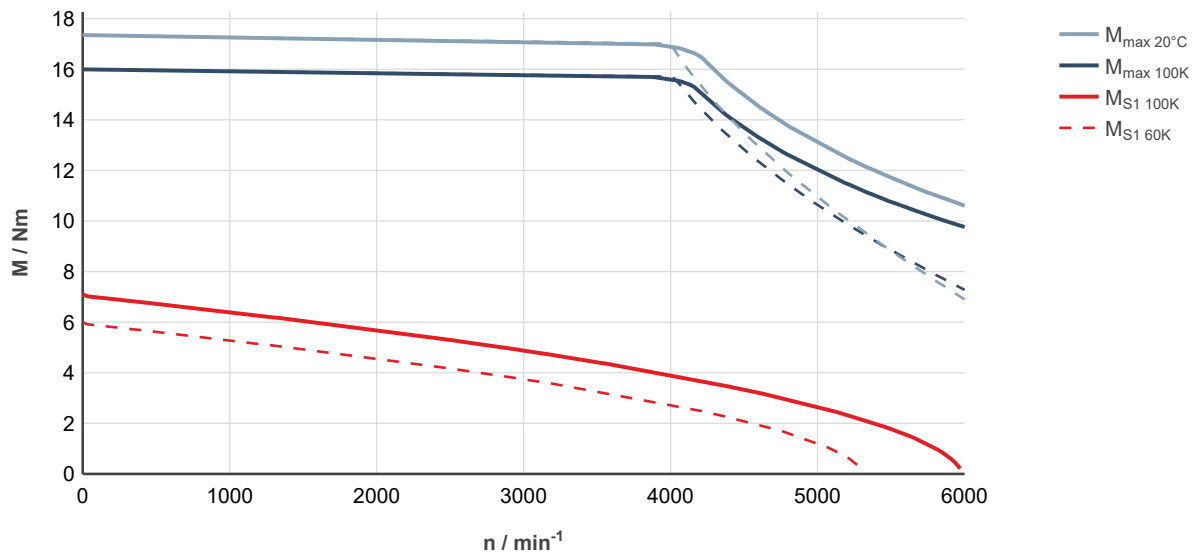
Fig. 73: MS2N06-C0BTN-___0-___-__, ctrlX DRIVE, uncontrolled supply 3 × AC 400 V
