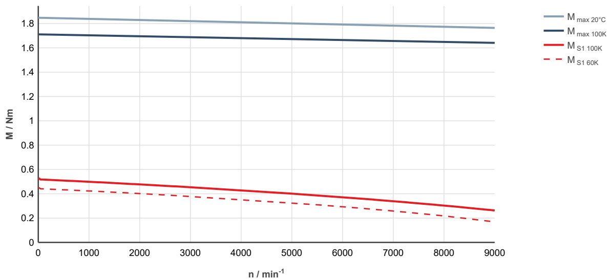
Fig. 25: MS2N03-A0BYN-___0-___-___, ctrlX DRIVE, controlled supply 3 x AC 400 ... 480 V
