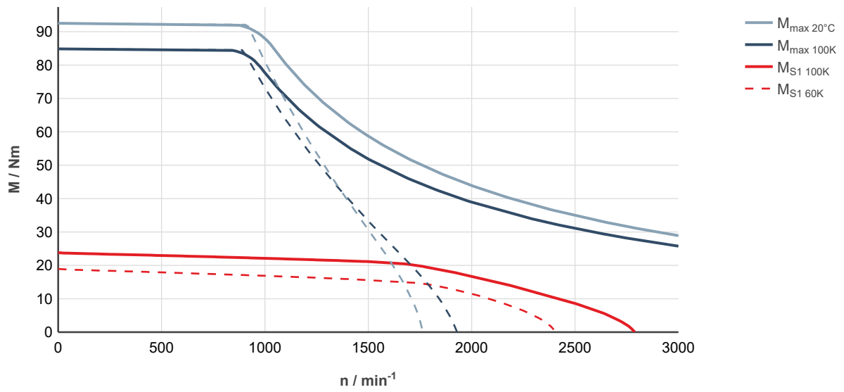
Fig. 108: MS2N07-D1BFN-___0-___-__, ctrlX DRIVE, uncontrolled supply 3 × AC 400 V
