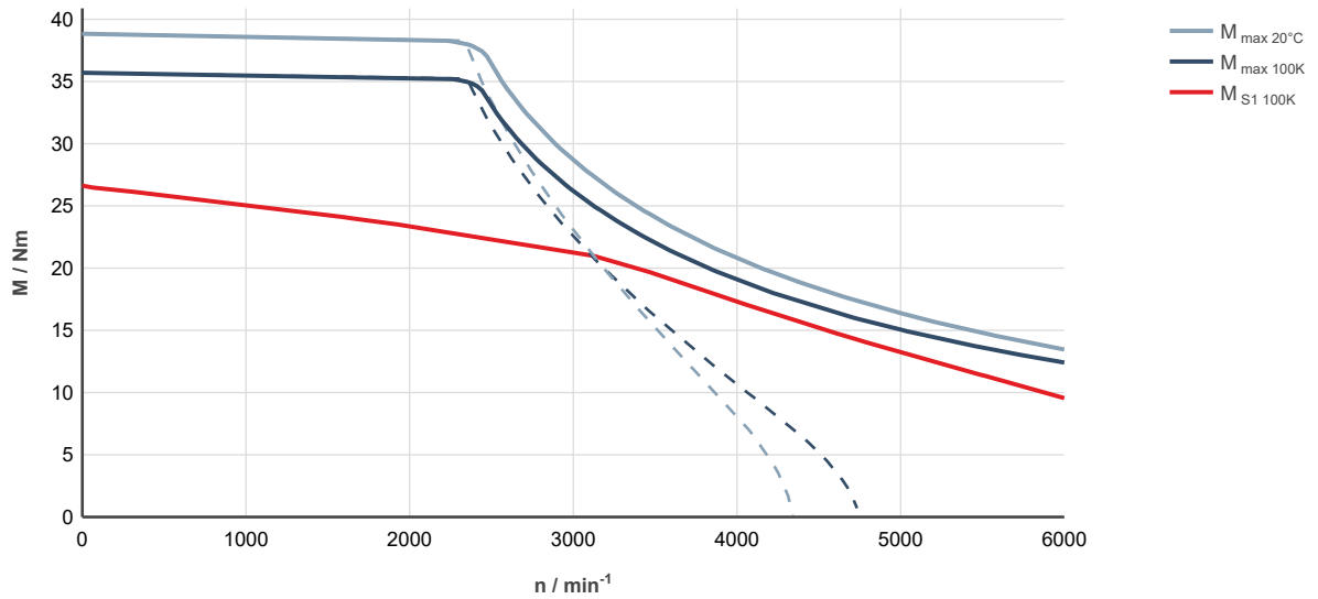
Fig. 165: MS2N07-C0BNL-___0-___-___, ctrlX DRIVE, controlled supply 3 x AC 400 ... 480 V
