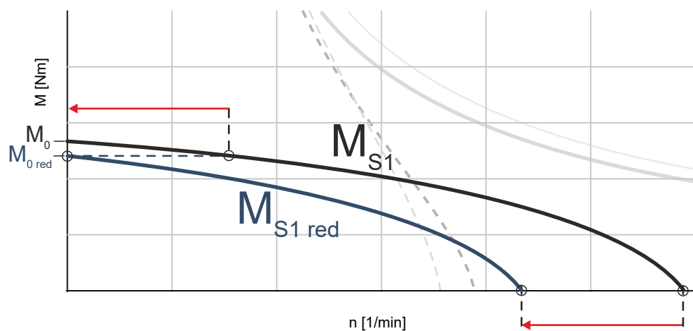
Fig. 400: Determine S1-characteristic curve M_{S1\ red} with derating factor f_{TH}
