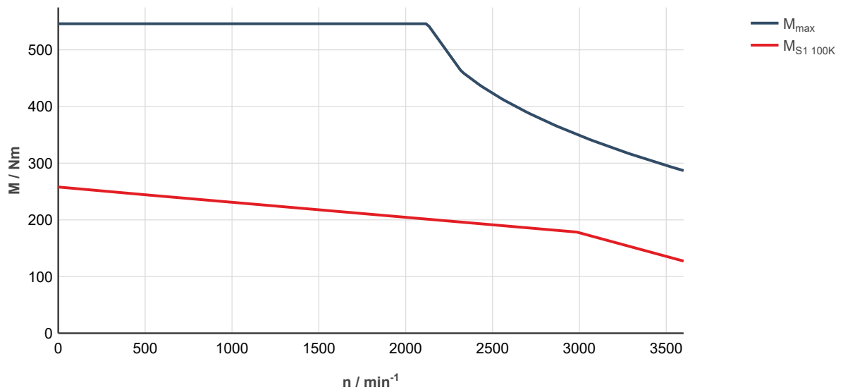
Fig. 328: MS2N13-D1BHC-___0-___-_, ctrlX DRIVE, controlled supply 3 x AC 400 ... 480 V M_{\text{max}} Characteristic curve applies to maximum torque 20 °C (cold)
