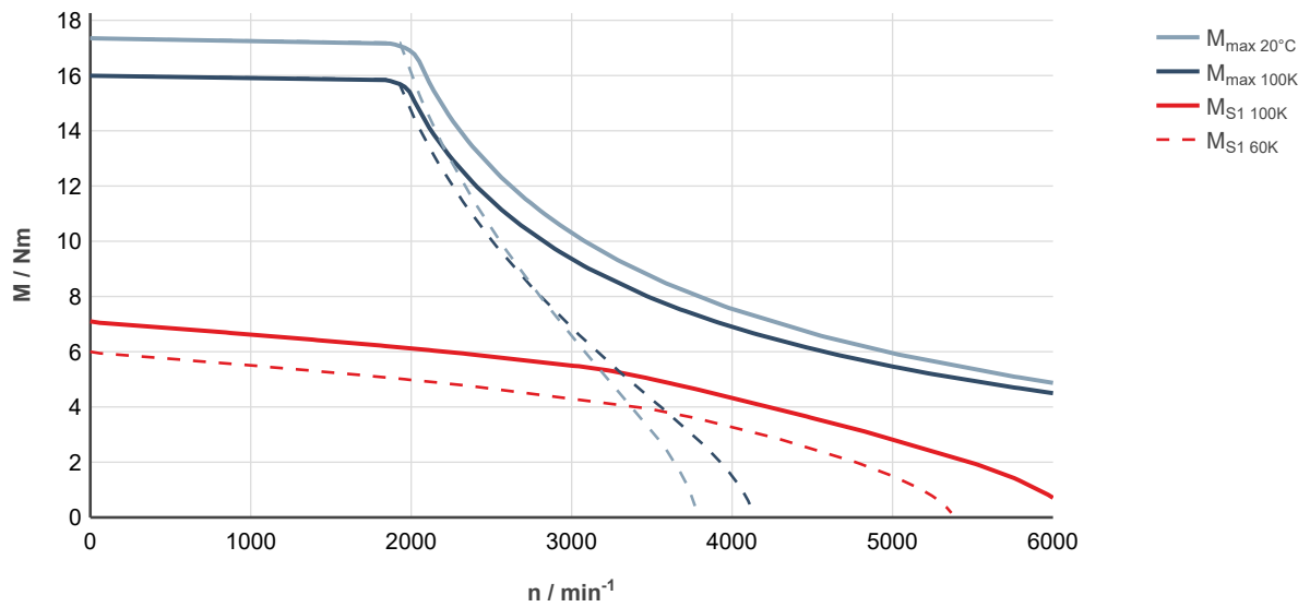
Fig. 71: MS2N06-C0BNN-___0-___-__, ctrlX DRIVE, uncontrolled supply 3 × AC 400 V
