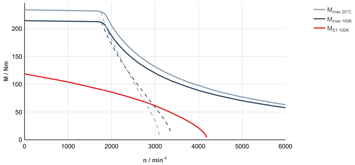
Fig. 247: MS2N10-E0BNA-___0-___-_, ctrIX DRIVE, uncontrolled supply 3 × AC 400 V
