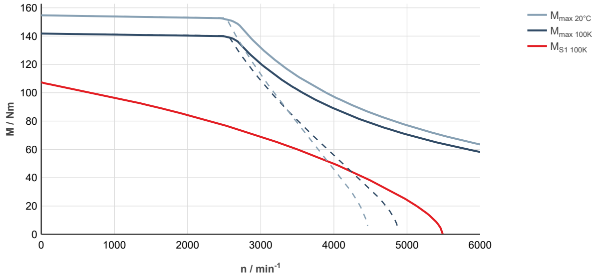
Fig. 272: MS2N10-D0BNL-___0-___-___, ctrIX DRIVE, controlled supply 3 × AC 400 ... 480 V
