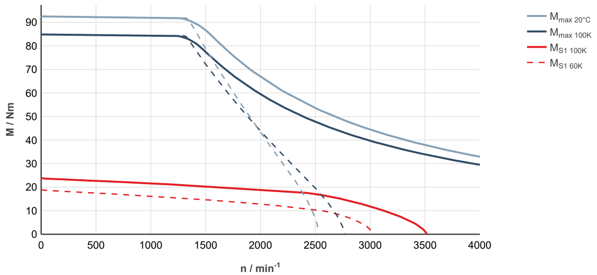
Fig. 110: MS2N07-D1BHN-___0-___-, ctrlX DRIVE, uncontrolled supply 3 × AC 400 V
