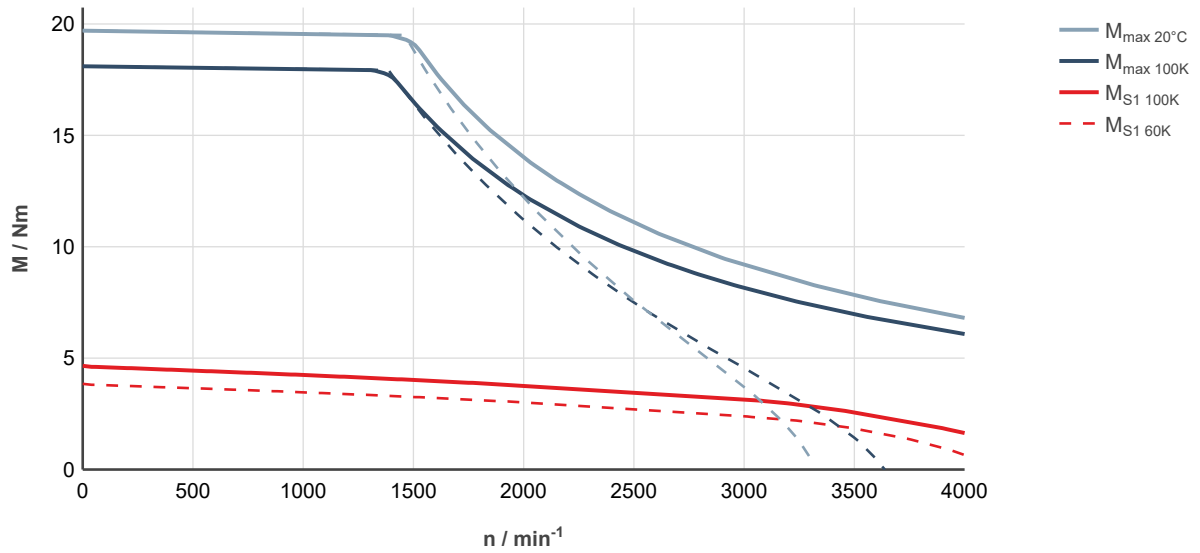
Fig. 44: MS2N04-D0BHN-___0-___-_, ctrlX DRIVE, controlled supply 3 × AC 400 ... 480 V
