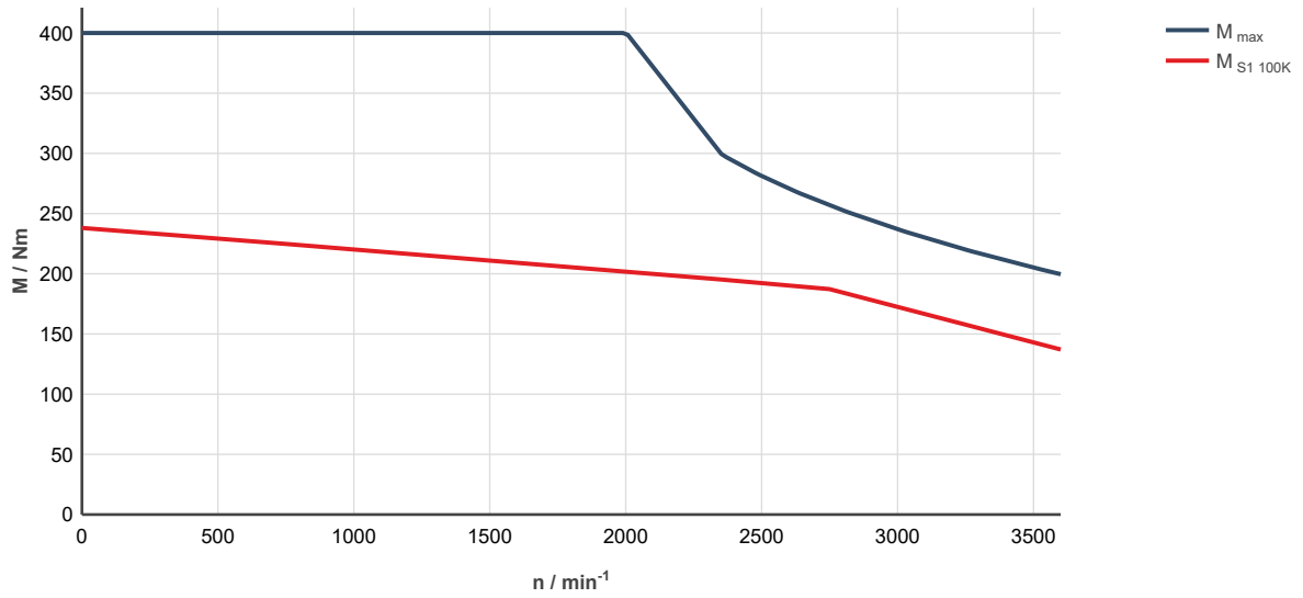
Fig. 341: MS2N13-C1BNL-___0-___-__, ctrlX DRIVE, uncontrolled supply 3 × AC 400 V M_{\text{max}} : Characteristic curve applies to maximum torque 20 °C (cold)
