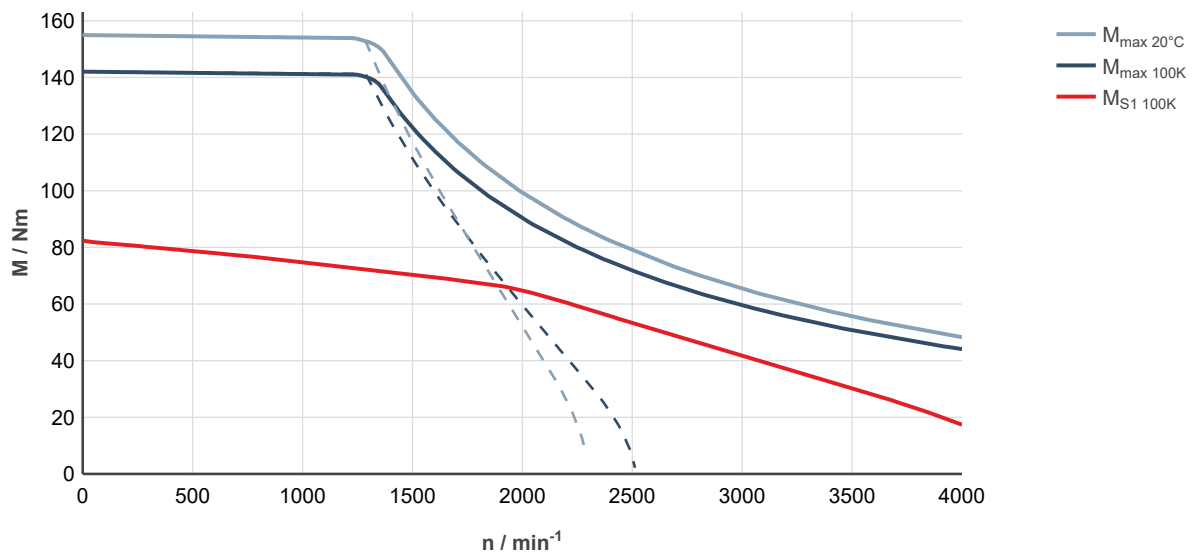
Fig. 237: MS2N10-D0BHA-___0-___-_, ctrlX DRIVE, uncontrolled supply 3 × AC 400 V
