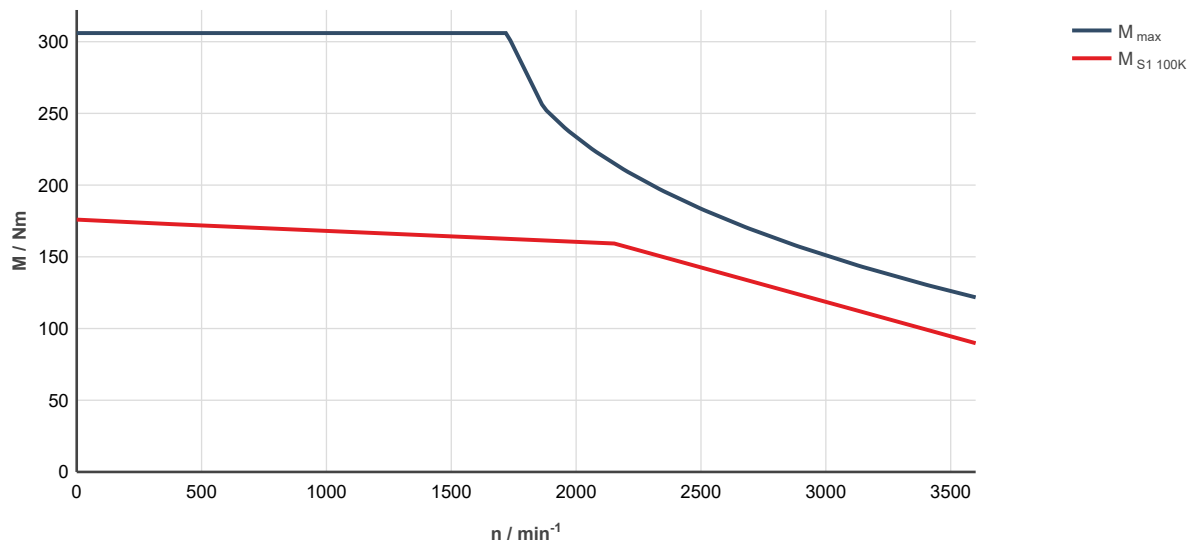
Fig. 335: MS2N13-B1BHL-__0-__-__, ctrlX DRIVE, uncontrolled supply 3 × AC 400 V M_{\text{max}} : Characteristic curve applies to maximum torque 20 °C (cold)
