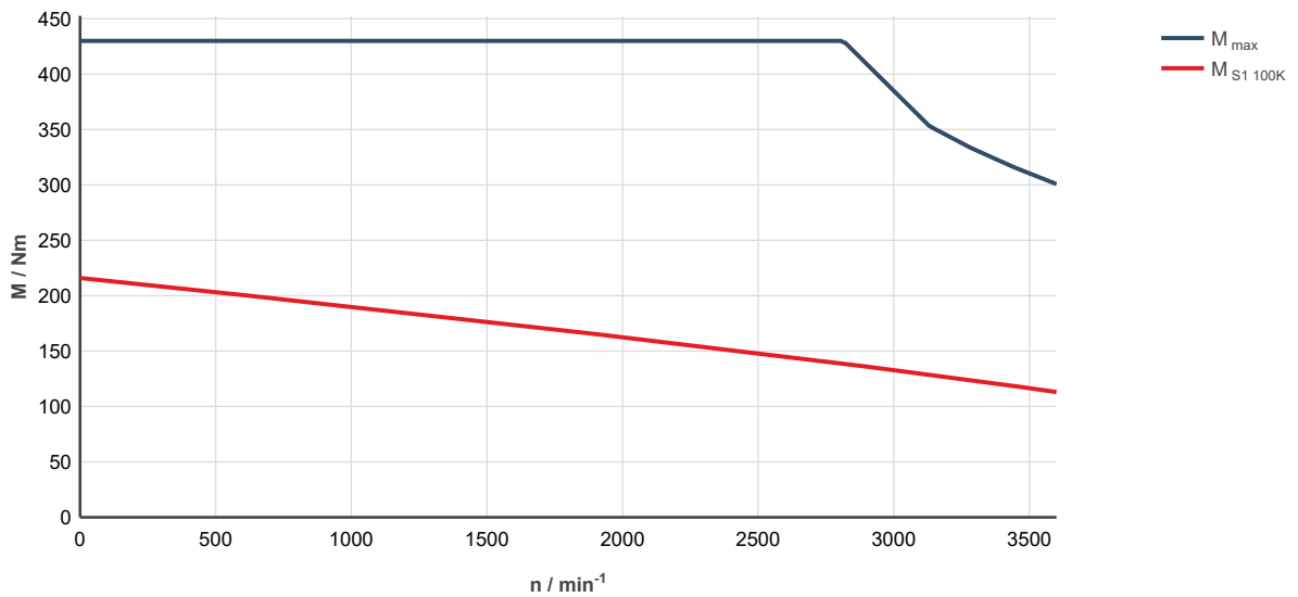
Fig. 326: MS2N13-C1BNC-___0-N___-__, ctrlX DRIVE, controlled supply 3 x AC 400 ... 480 V M_{\text{max}} : Characteristic curve applies to maximum torque 20 °C (cold)
