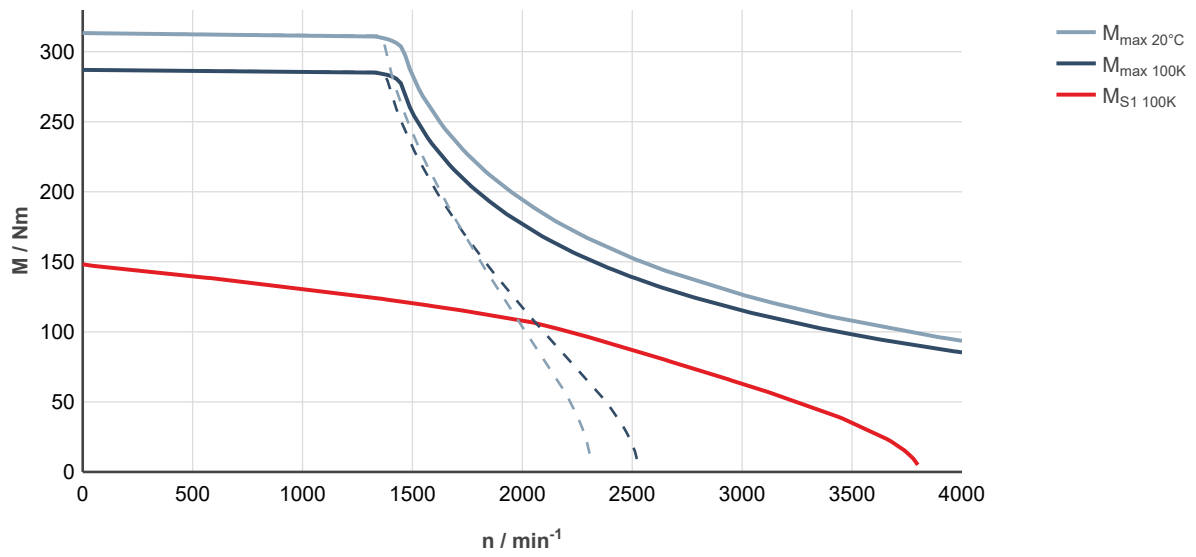
Fig. 255: MS2N10-F0BHA-___0-___-_, ctrlX DRIVE, uncontrolled supply 3 × AC 400 V
