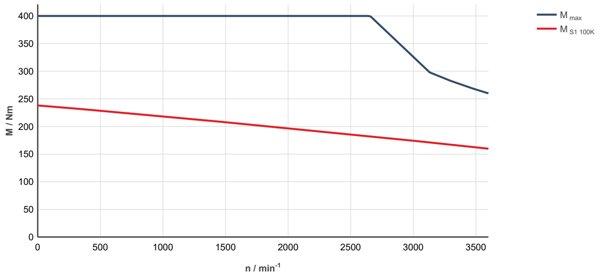
Fig. 342: MS2N13-C1BNL-___0-___-__, ctrlX DRIVE, controlled supply 3 x AC 400 ... 480 V M_{\text{max}} : Characteristic curve applies to maximum torque 20 °C (cold)
