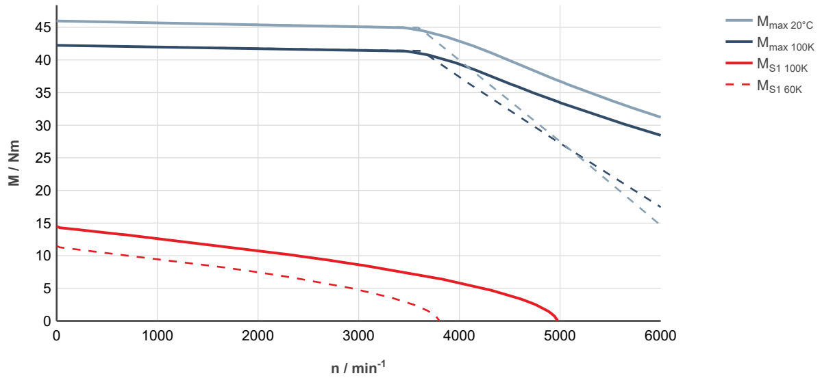
Fig. 99: MS2N07-C1BRN-___0-___-__, ctrlX DRIVE, controlled supply 3 × AC 400 ... 480 V
