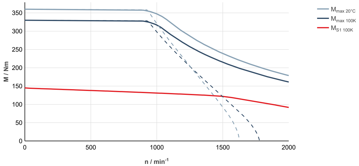
Fig. 258: MS2N10-F1BDA-___0-___-__, ctrlX DRIVE, controlled supply 3 × AC 400 ... 480 V
