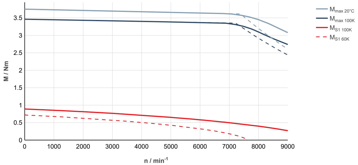
Fig. 27: MS2N03-B0BYN-___0-___-_, ctrlX DRIVE, controlled supply 3 × AC 400 ... 480 V
