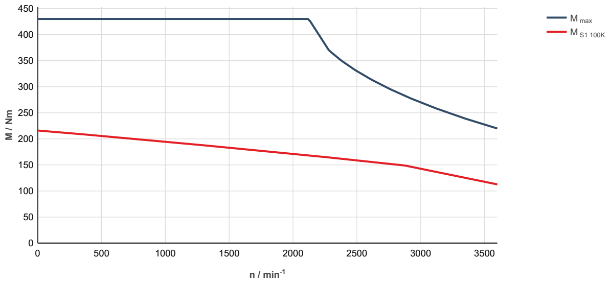
Fig. 325: MS2N13-C1BNC-___0-N___-__, ctrlX DRIVE, uncontrolled supply 3 × AC 400 V M_{\text{max}} : Characteristic curve applies to maximum torque 20 °C (cold)
