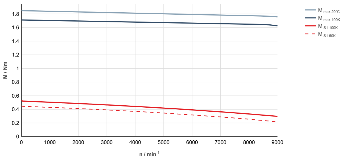
Fig. 24: MS2N03-A0BYN-___0-___-___, ctrlX DRIVE, uncontrolled supply 3 × AC 400 V
