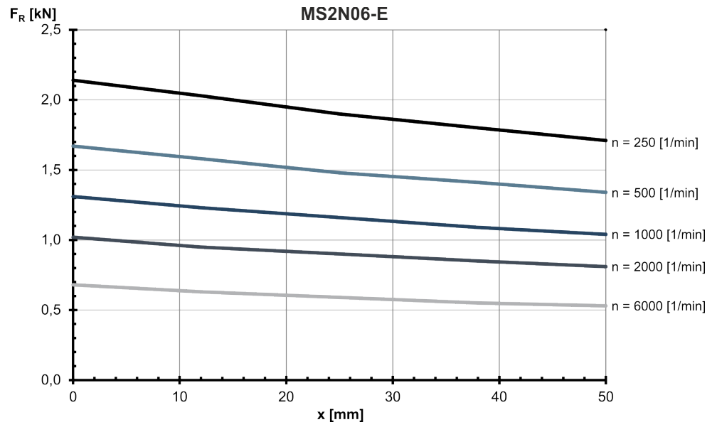
Fig. 89: MS2N06-E: Radial force in distance x from the shaft shoulder at a nominal bearing service life of L_{h10} = 30000 h
