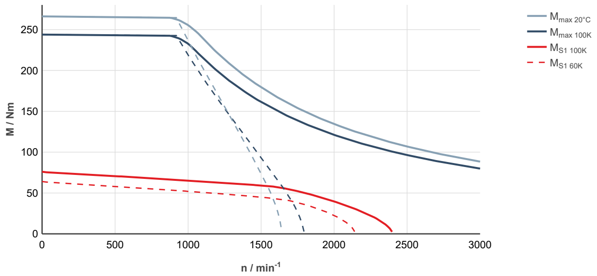
Fig. 215: MS2N10-E1BFN-___0-___-__, ctrlX DRIVE, uncontrolled supply 3 × AC 400 V
