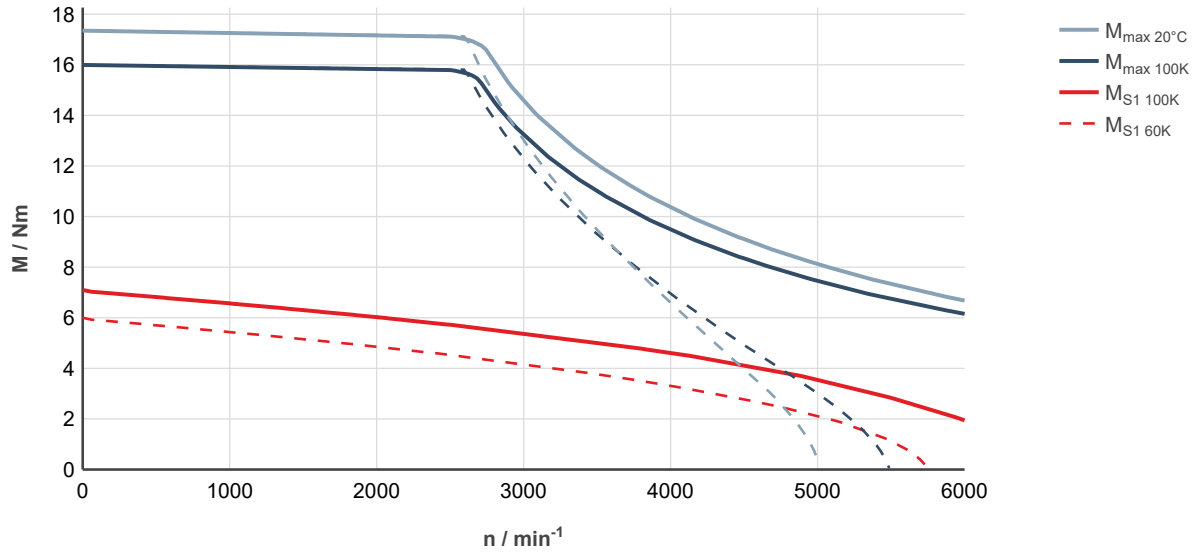
Fig. 72: MS2N06-C0BNN-___0-___-__, ctrlX DRIVE, controlled supply 3 × AC 400 ... 480 V
