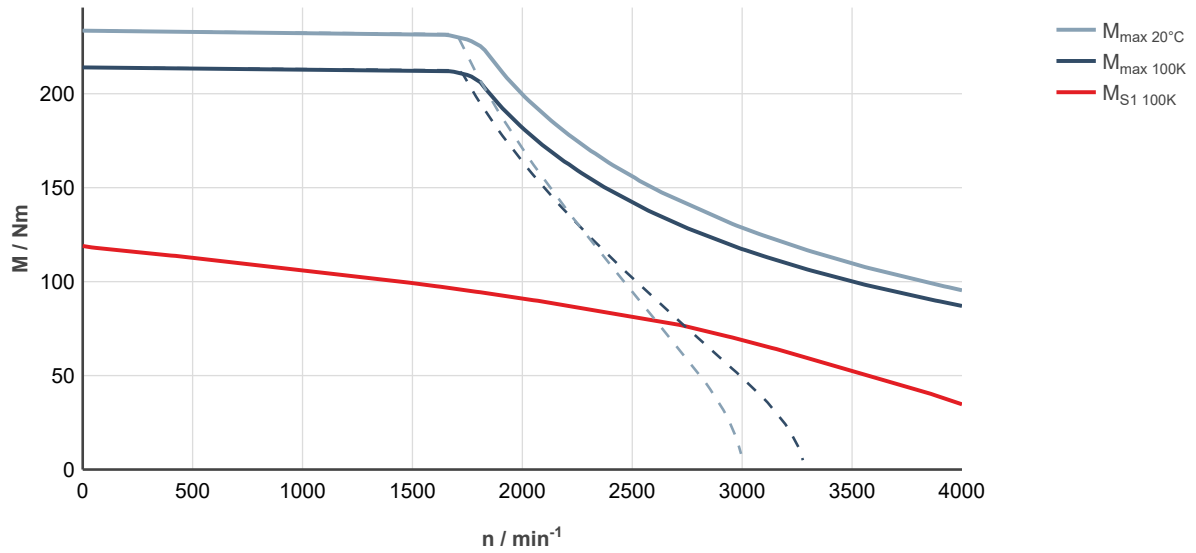
Fig. 246: MS2N10-E0BHA-___0-___-_, ctrIX DRIVE, controlled supply 3 × AC 400 ... 480 V
