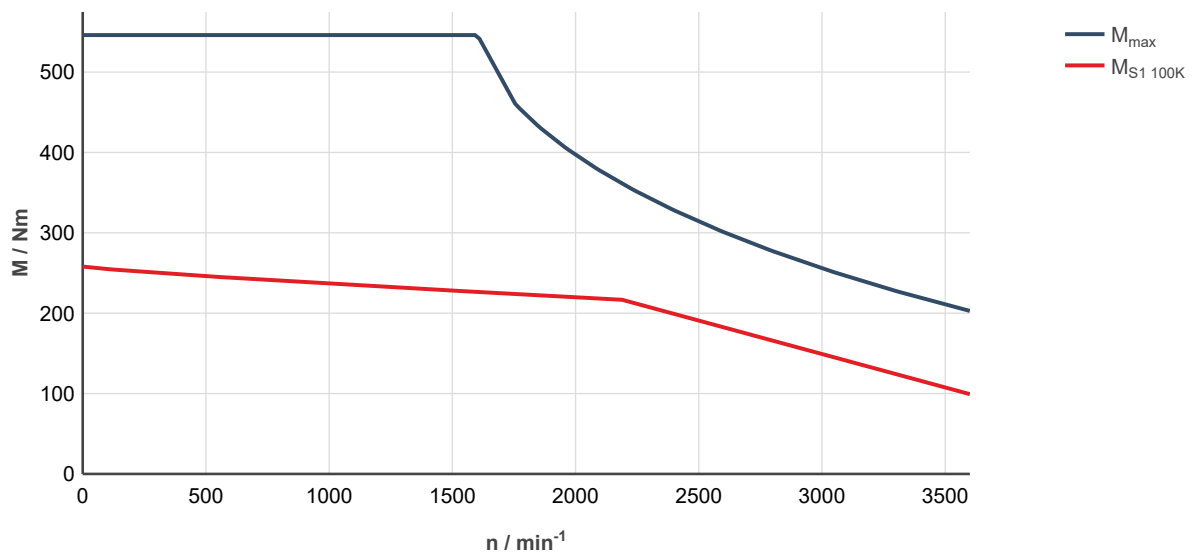
Fig. 327: MS2N13-D1BHC-___0-___-_, ctrlX DRIVE, uncontrolled supply 3 × AC 400 V(1) M_{\text{max}} Characteristic curve applies to maximum torque 20 °C (cold)
