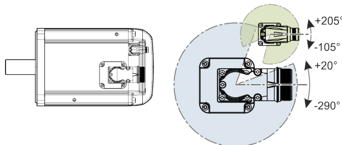
Fig. 384: : Rotating area electrical connection "V"
