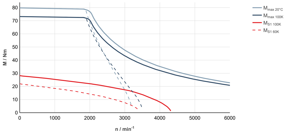
Fig. 104: MS2N07-D0BNN-___0-___-, ctrlX DRIVE, uncontrolled supply 3 × AC 400 V
