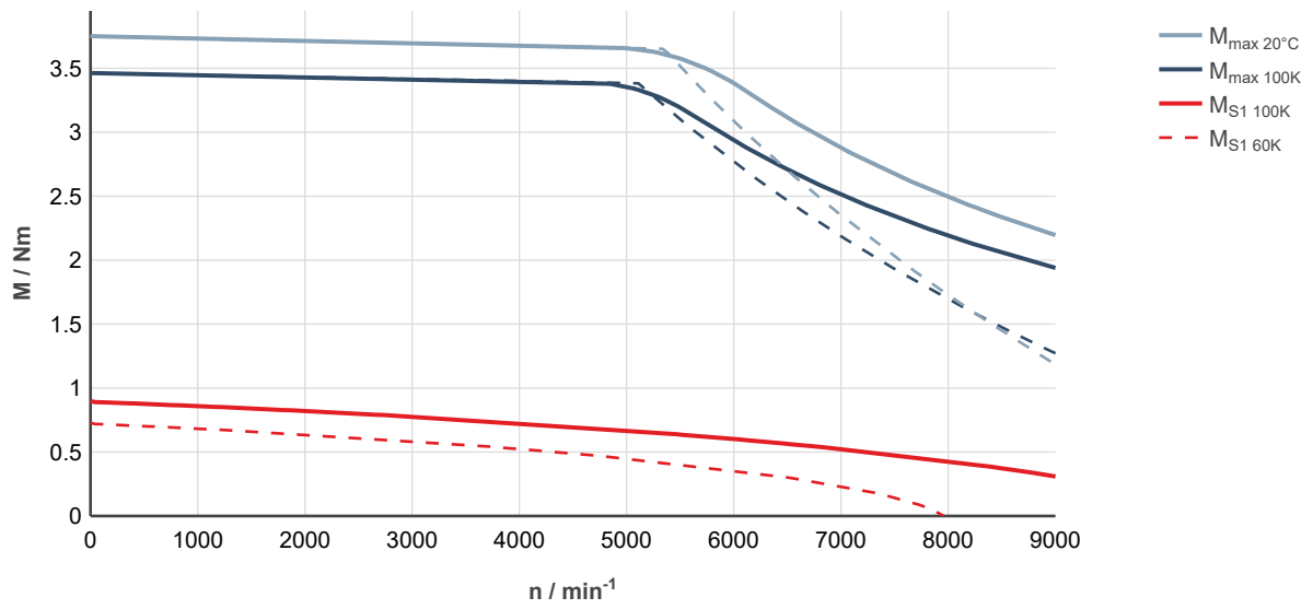
Fig. 26: MS2N03-B0BYN-___0-___-_, ctrlX DRIVE, uncontrolled supply 3 × AC 400 V
