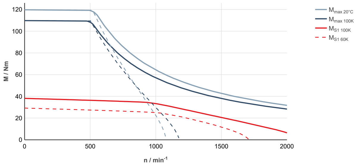
Fig. 114: MS2N07-E0BDN-___0-___-_, ctrlX DRIVE, uncontrolled supply 3 × AC 400 V
