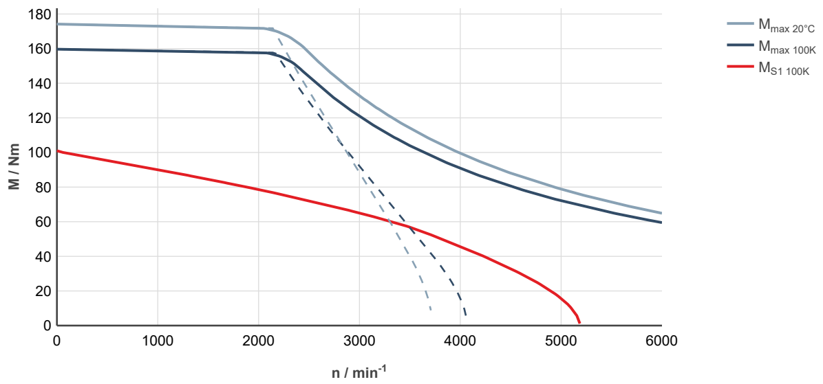
Fig. 273: MS2N10-D1BNL-___0-___-___, ctrIX DRIVE, uncontrolled supply 3 × AC 400 V
