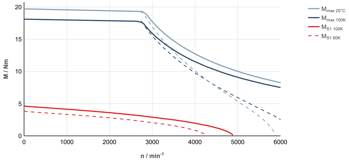
Fig. 46: MS2N04-D0BQN-___0-___-_, ctrlX DRIVE, controlled supply 3 × AC 400 ... 480 V
