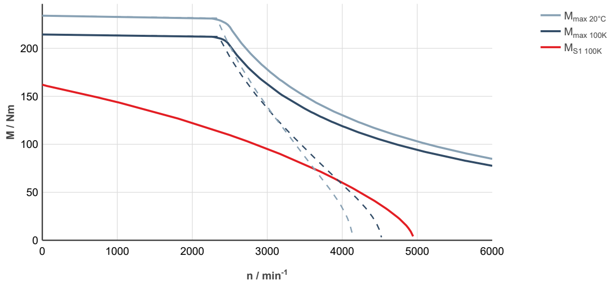
Fig. 278: MS2N10-E0BNL-___0-___-___, ctrlX DRIVE, controlled supply 3 × AC 400 ... 480 V
