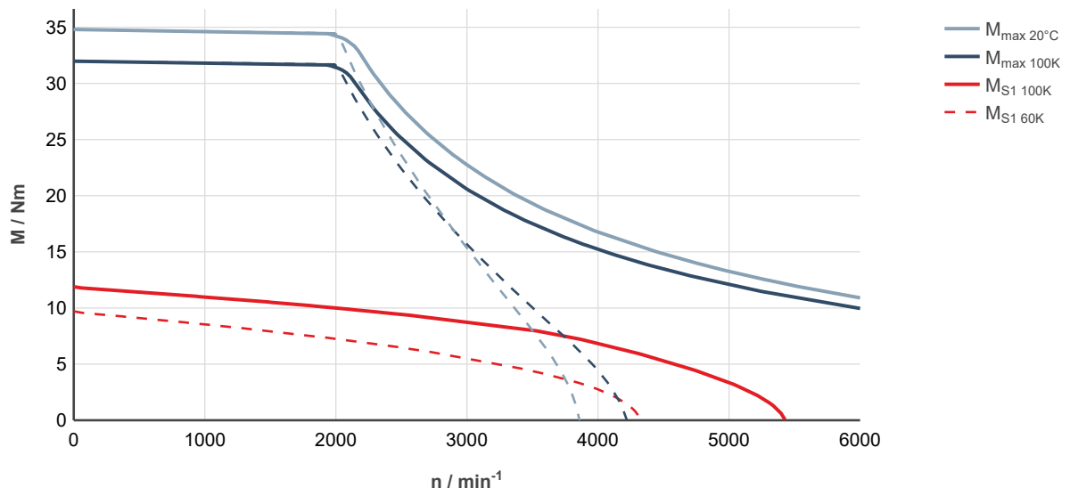
Fig. 75: MS2N06-D0BNN-___0-___-_, ctrlX DRIVE, uncontrolled supply 3 × AC 400 V
