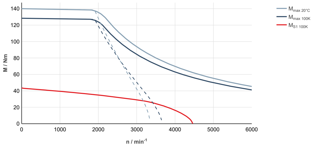
Fig. 162: MS2N07-E1BNA-___0-___-__, ctrlX DRIVE, uncontrolled supply 3 × AC 400 V
