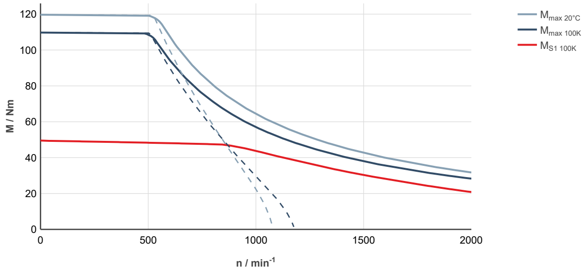
Fig. 150: MS2N07-E0BDA-___0-___-___, ctrlX DRIVE, uncontrolled supply 3 × AC 400 V
