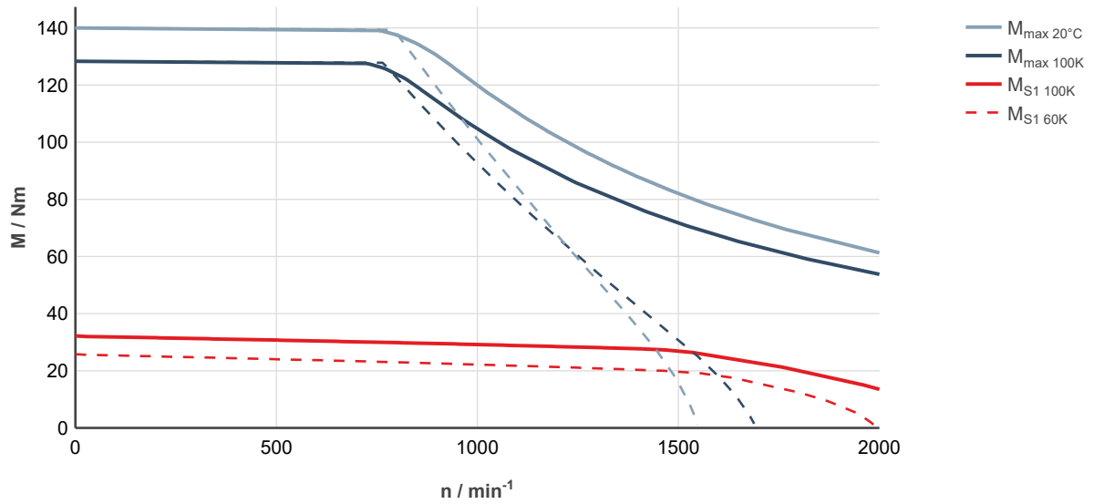
Fig. 123: MS2N07-E1BDN-___0-___-_, ctrlX DRIVE, controlled supply 3 × AC 400 ... 480 V
