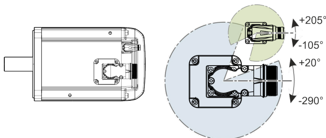
Fig. 369: Rotating area electrical connection "V"
