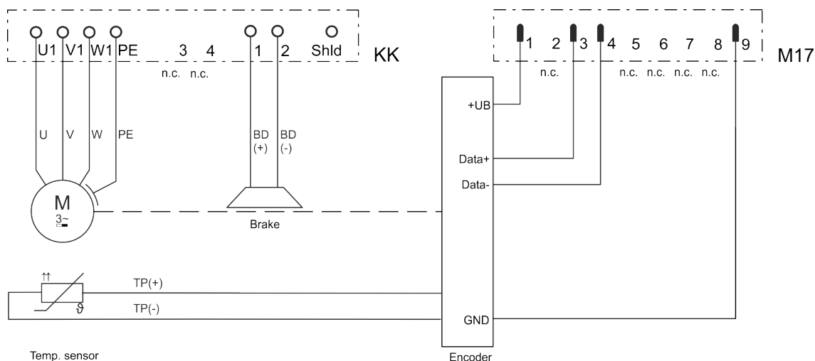
Fig. 363: Double cable connection terminal boxes, digital encoder C and D, brake optional
