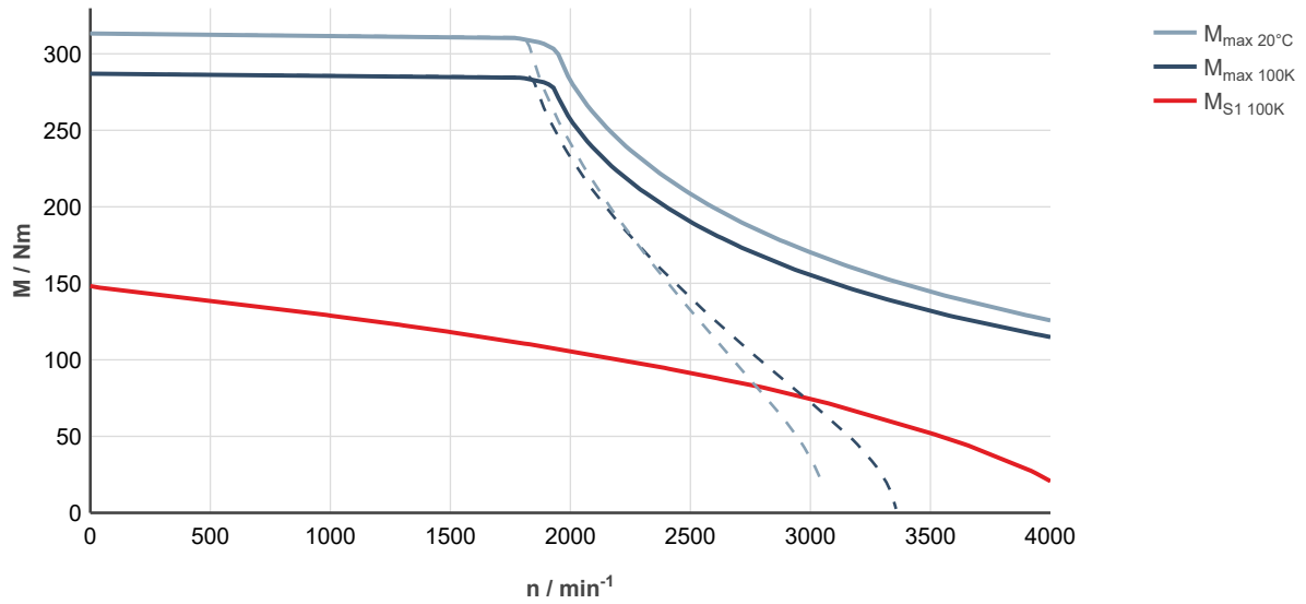
Fig. 256: MS2N10-F0BHA-___0-___-_, ctrlX DRIVE, controlled supply 3 × AC 400 ... 480 V
