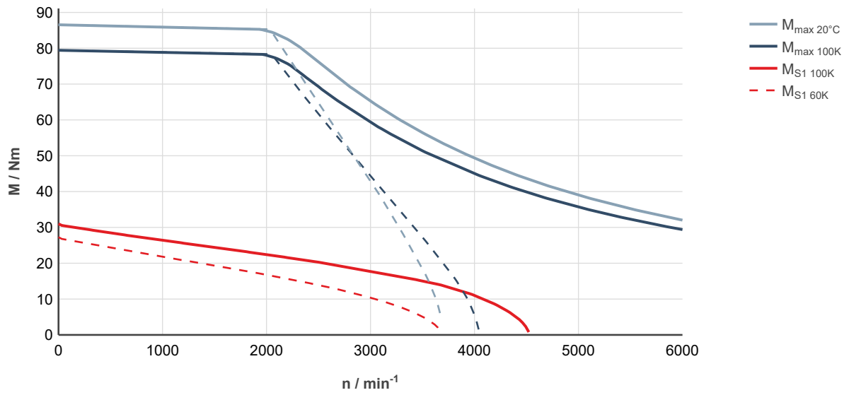
Fig. 201: MS2N10-C1BNN-___0-___-_, ctrlX DRIVE, uncontrolled supply 3 × AC 400 V
