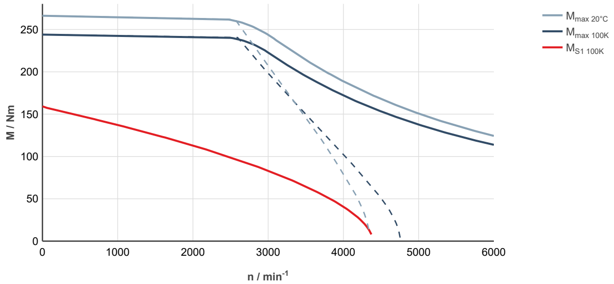
Fig. 280: MS2N10-E1BNL-___0-___-___, ctrlX DRIVE, controlled supply 3 × AC 400 ... 480 V
