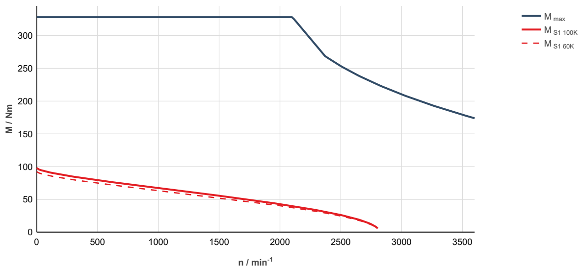
Fig. 305: MS2N13-B1BNN-___0-___-_, ctrIX DRIVE, uncontrolled supply 3 × AC 400 V M_{\text{max}} : Characteristic curve applies to maximum torque 20 °C (cold)
