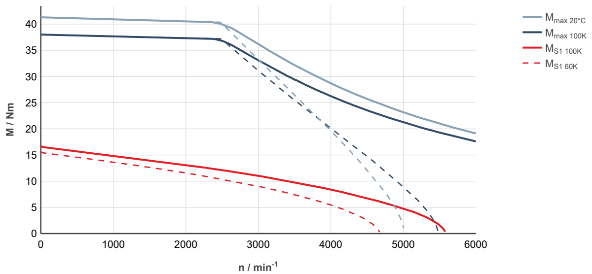
Fig. 193: MS2N10-B1BQN-___0-___-, ctrlX DRIVE, uncontrolled supply 3 × AC 400 V
