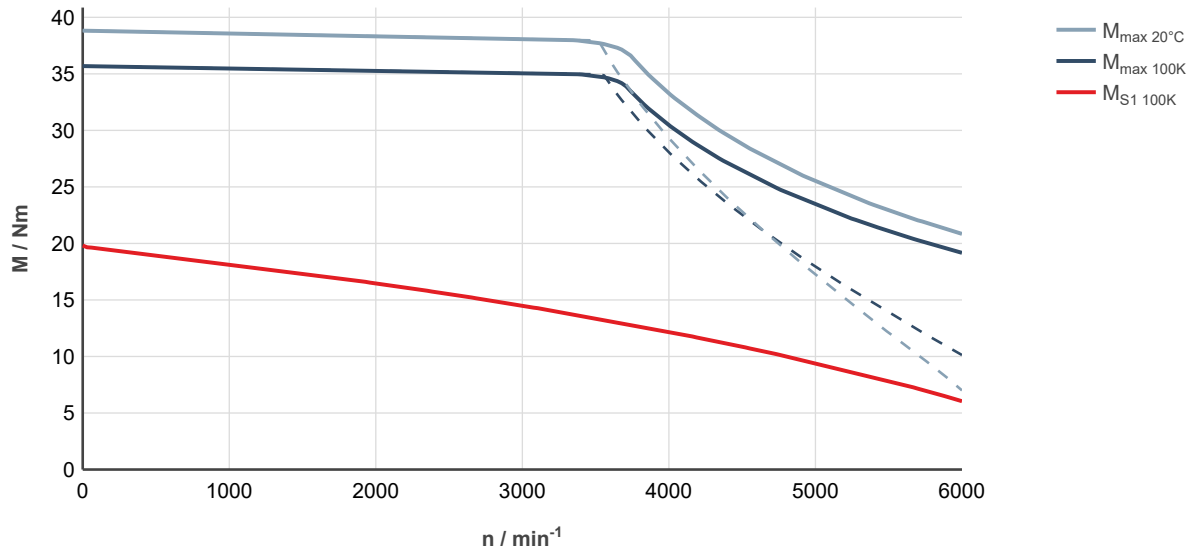
Fig. 131: MS2N07-C0BQA-___0-___-_, ctrlIX DRIVE, controlled supply 3 × AC 400 ... 480 V
