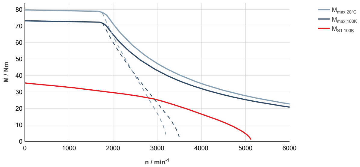
Fig. 140: MS2N07-D0BNA-___0-___-_, ctrlX DRIVE, uncontrolled supply 3 × AC 400 V
