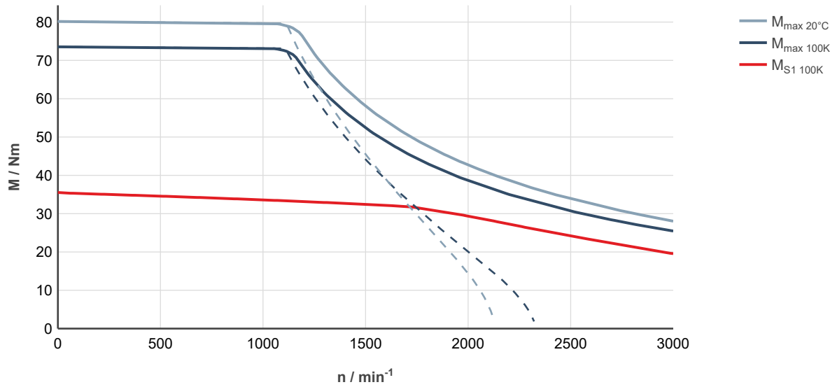
Fig. 137: MS2N07-D0BFA-___0-___-___, ctrlX DRIVE, controlled supply 3 × AC 400 ... 480 V
