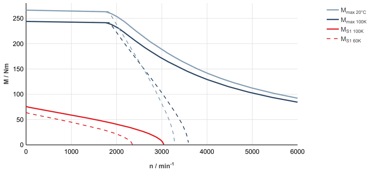
Fig. 217: MS2N10-E1BNN-___0-___-_, ctrlX DRIVE, uncontrolled supply 3 × AC 400 V
