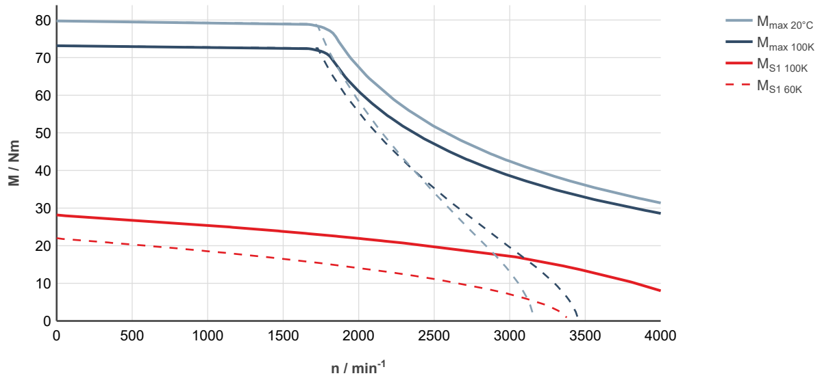
Fig. 103: MS2N07-D0BHN-___0-___-_, ctrlX DRIVE, controlled supply 3 × AC 400 ... 480 V
