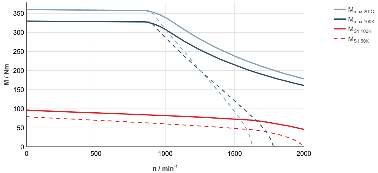
Fig. 224: MS2N10-F1BDN-___0-___-_, ctrlX DRIVE, controlled supply 3 × AC 400 ... 480 V
