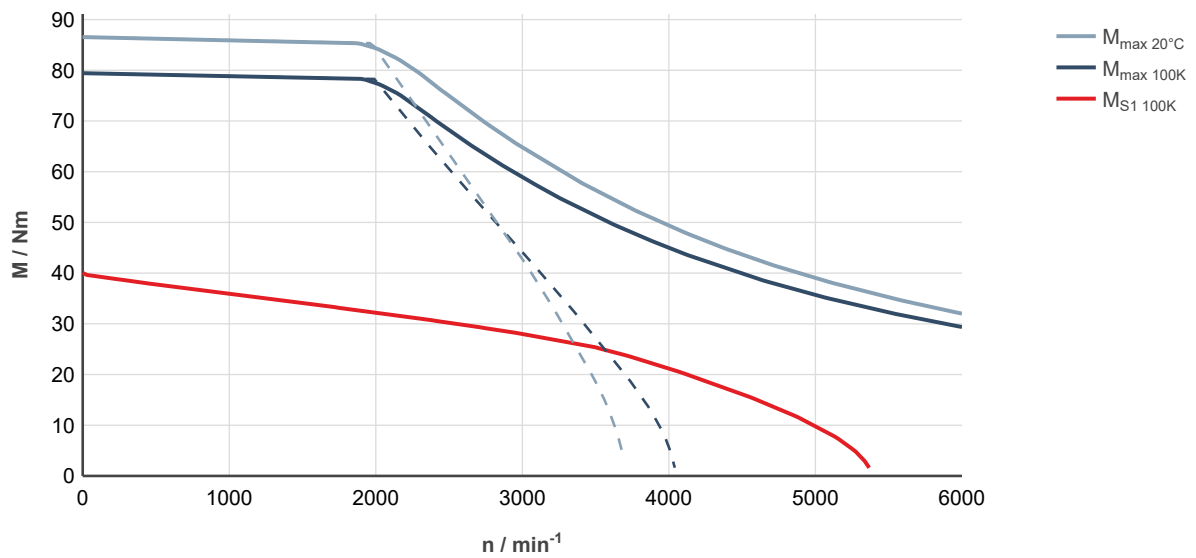
Fig. 235: MS2N10-C1BNA-___0-___-_, ctrlX DRIVE, uncontrolled supply 3 × AC 400 V
