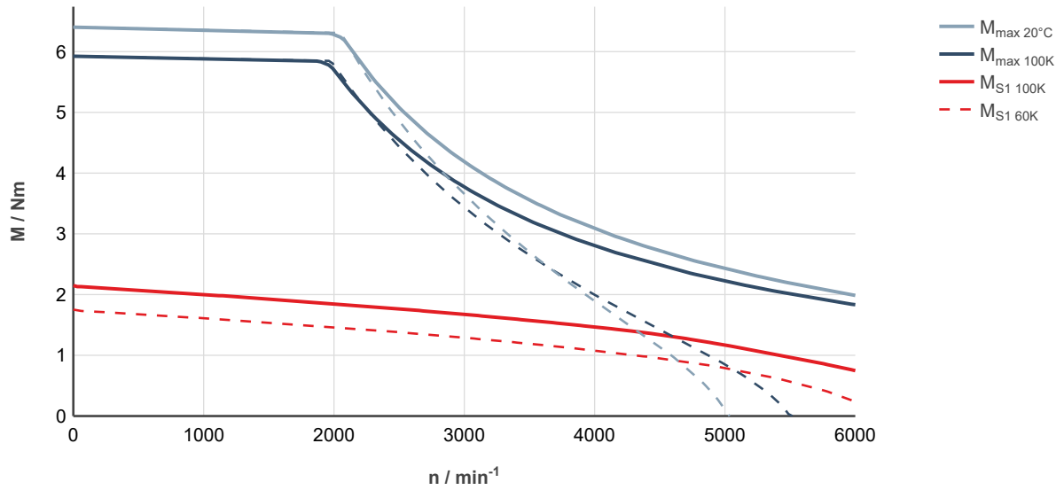
Fig. 36: MS2N04-B0BNN-___0-___-___, ctrlX DRIVE, controlled supply 3 × AC 400 ... 480 V
