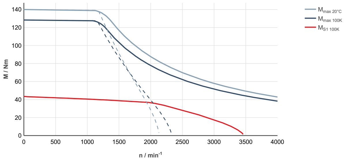
Fig. 160: MS2N07-E1BHA-___0-___-_, ctrIX DRIVE, uncontrolled supply 3 x AC 400 V
