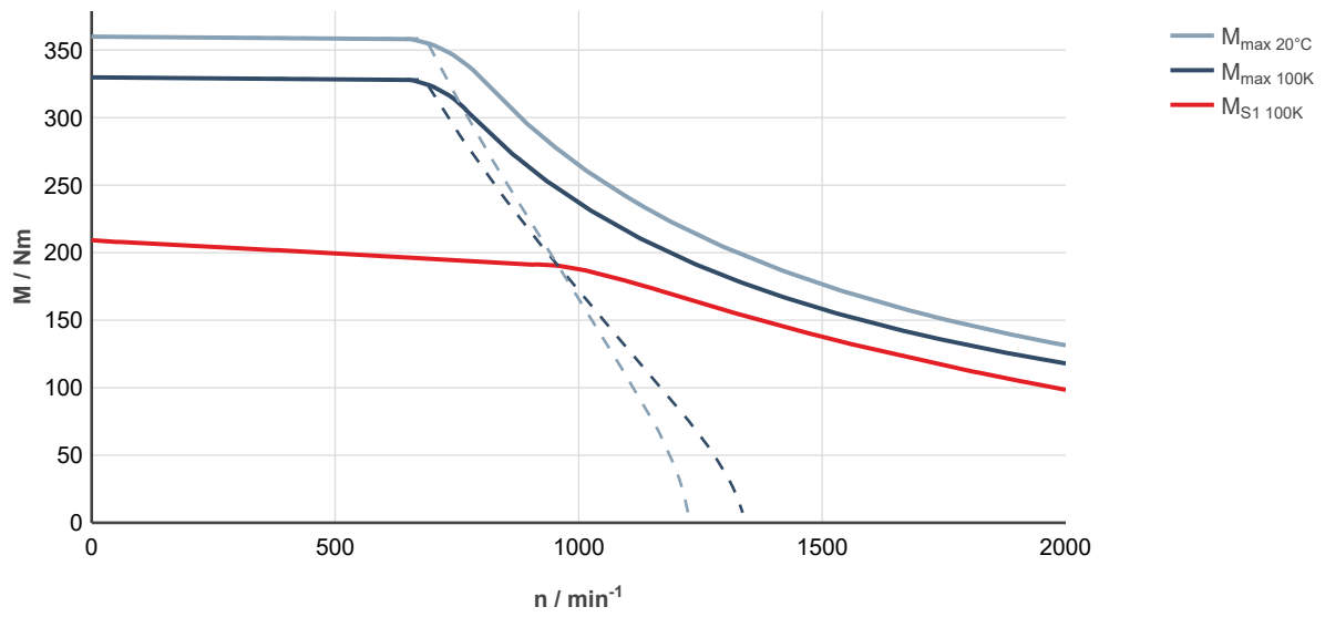
Fig. 283: MS2N10-F1BDL-___0-___-___, ctrlX DRIVE, uncontrolled supply 3 × AC 400 V
