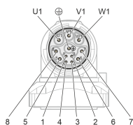
Fig. 377: Connector view of M17 single cable connector
