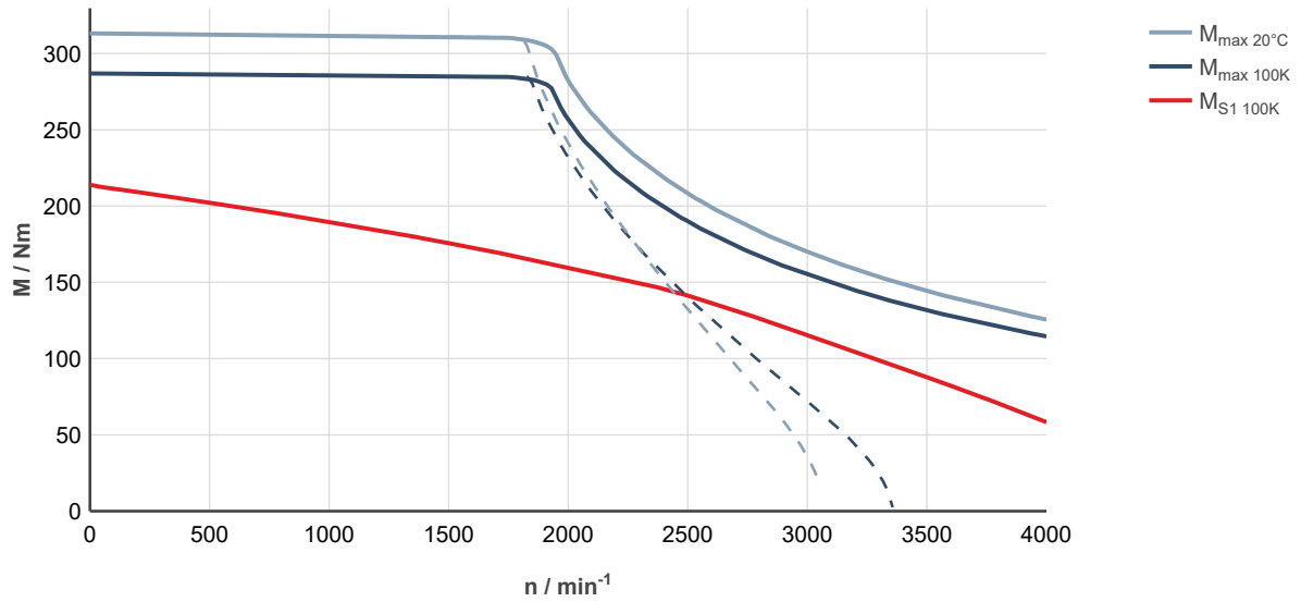
Fig. 282: MS2N10-F0BHL-___0-___-___, ctrlX DRIVE, controlled supply 3 × AC 400 ... 480 V
