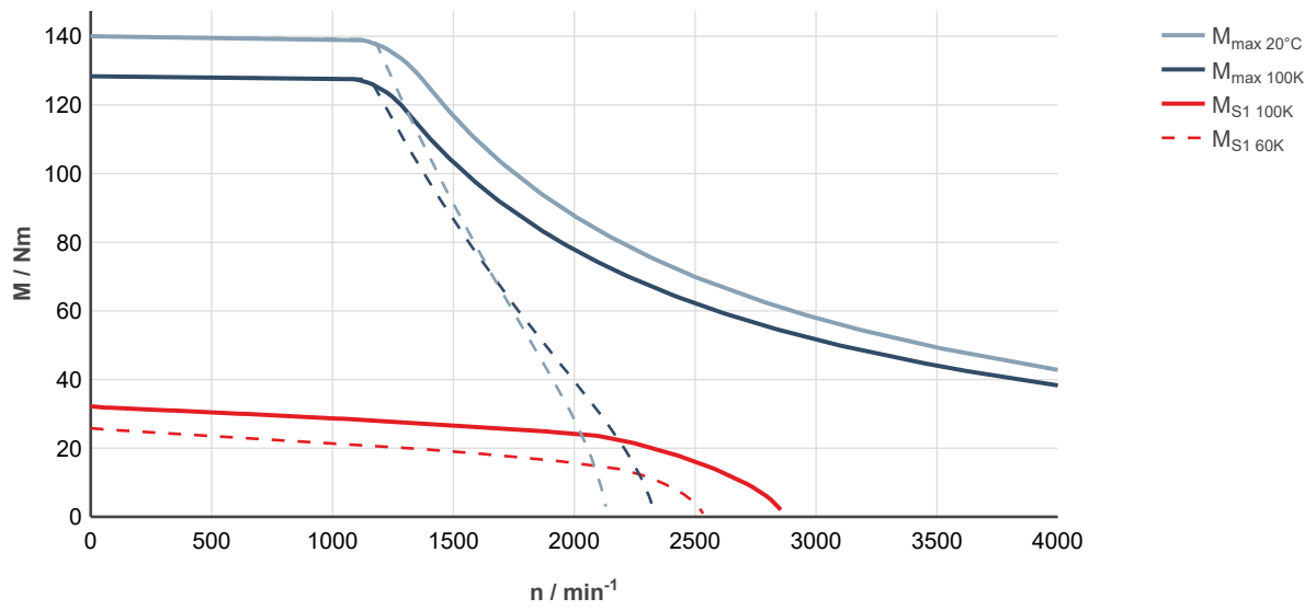
Fig. 124: MS2N07-E1BHN-___0-___-_, ctrlX DRIVE, uncontrolled supply 3 × AC 400 V
