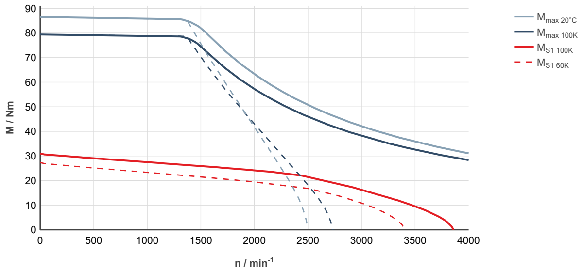
Fig. 199: MS2N10-C1BHN-___0-___-_, ctrlX DRIVE, uncontrolled supply 3 × AC 400 V
