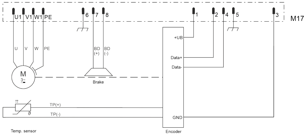
Fig. 358: M17 Single cable connection, digital encoder C, D, H, optional brake
