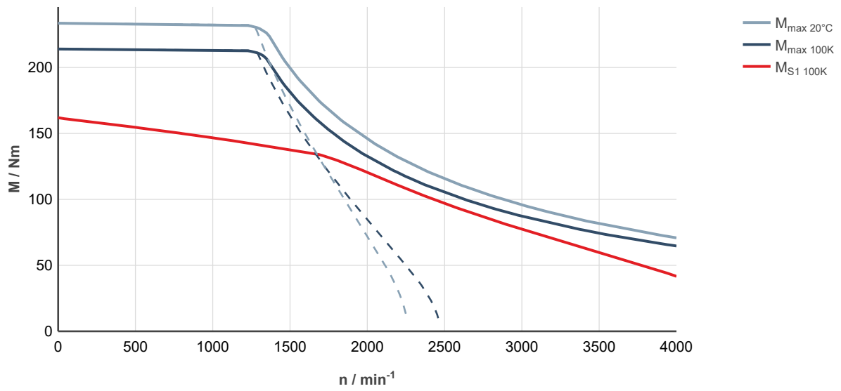
Fig. 275: MS2N10-E0BHL-___0-___-___, ctrlX DRIVE, uncontrolled supply 3 × AC 400 V
