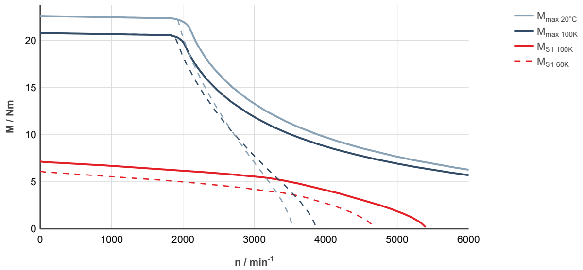
Fig. 56: MS2N05-C0BNN-___0-___-_, ctrlX DRIVE, uncontrolled supply 3 × AC 400 V
