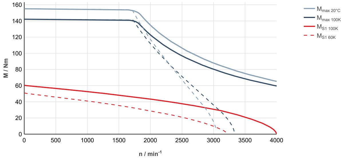
Fig. 204: MS2N10-D0BHN-___0-___-_, ctrlX DRIVE, controlled supply 3 × AC 400 ... 480 V
