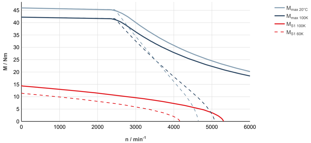
Fig. 97: MS2N07-C1BNN-___0-___-__, ctrlX DRIVE, controlled supply 3 × AC 400 ... 480 V
