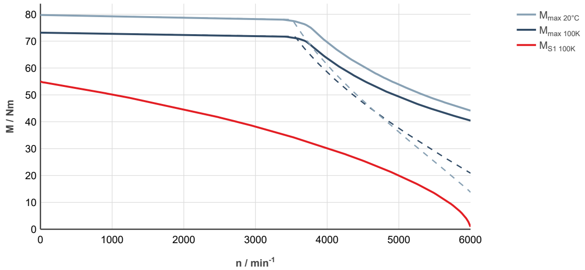
Fig. 175: MS2N07-D0BRL-___0-___-___, ctrlX DRIVE, controlled supply 3 × AC 400 ... 480 V
