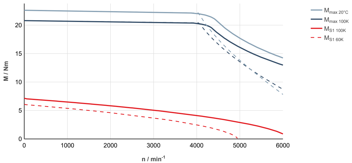
Fig. 58: MS2N05-C0BTN-___0-___-__, ctrlX DRIVE, uncontrolled supply 3 × AC 400 V
