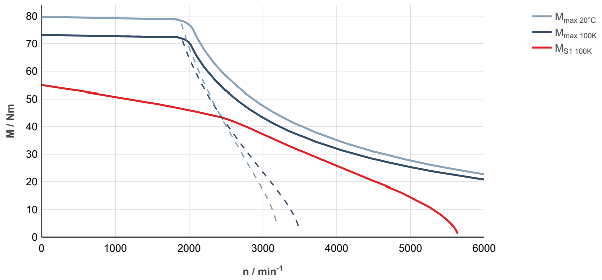
Fig. 172: MS2N07-D0BNL-___0-___-___, ctrIX DRIVE, uncontrolled supply 3 × AC 400 V
