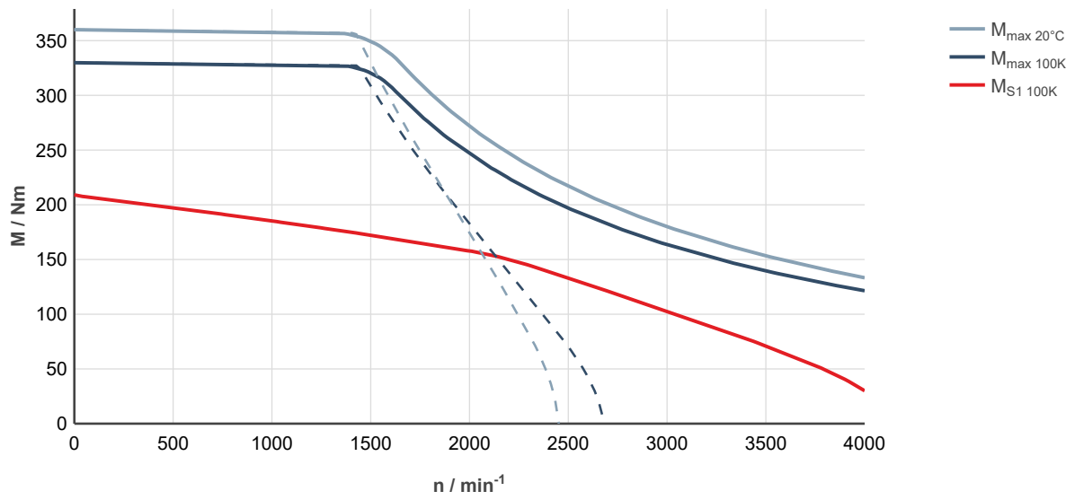
Fig. 285: MS2N10-F1BHL-___0-___-___, ctrlX DRIVE, uncontrolled supply 3 × AC 400 V
