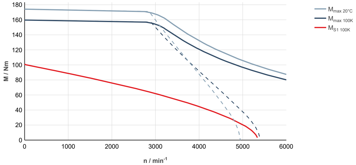
Fig. 274: MS2N10-D1BNL-___0-___-___, ctrIX DRIVE, controlled supply 3 × AC 400 ... 480 V
