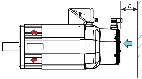
Fig. 3: Minimum distance
