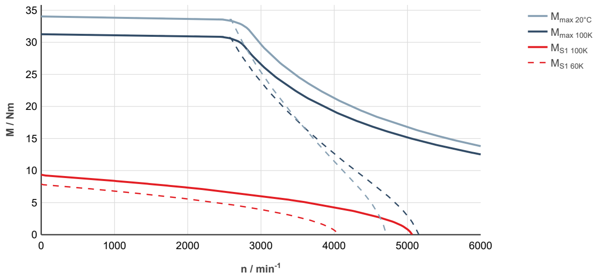
Fig. 62: MS2N05-D0BRN-___0-___-___, ctrlX DRIVE, uncontrolled supply 3 × AC 400 V
