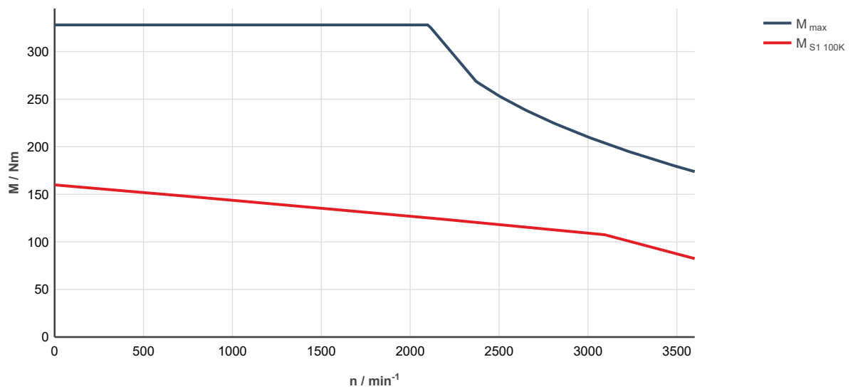
Fig. 321: MS2N13-B1BNC-___0-___-_, ctrIX DRIVE, uncontrolled supply 3 × AC 400 V M_{\text{max}} : Characteristic curve applies to maximum torque 20 °C (cold)
