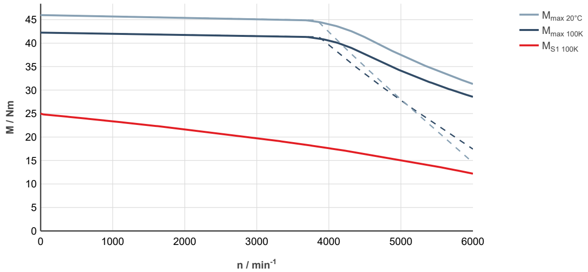
Fig. 169: MS2N07-C1BRL-___0-___-___, ctrIX DRIVE, controlled supply 3 × AC 400 ... 480 V
