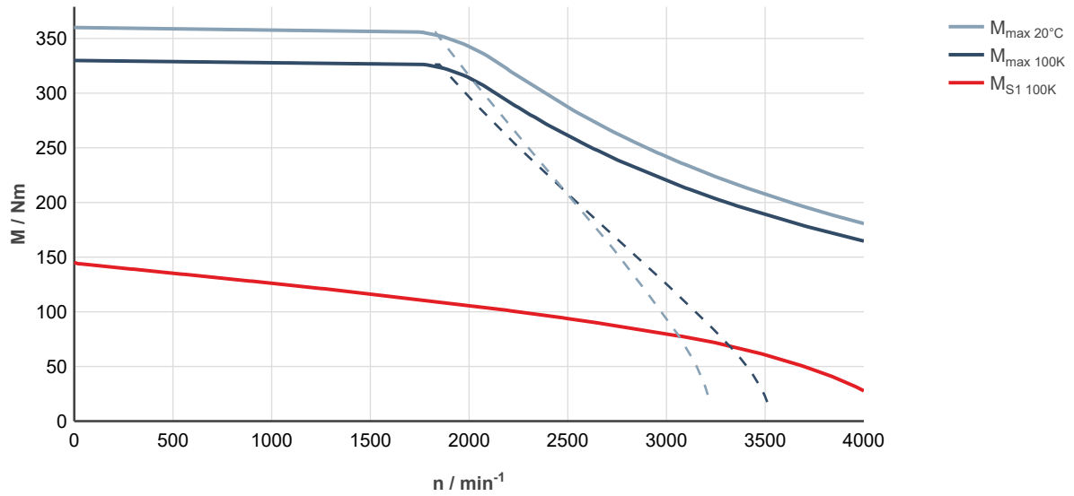
Fig. 260: MS2N10-F1BHA-___0-___-__, ctrlX DRIVE, controlled supply 3 × AC 400 ... 480 V
