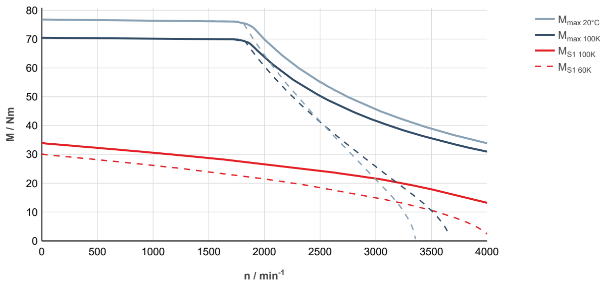
Fig. 196: MS2N10-C0BHN-___0-___-_, ctrlX DRIVE, controlled supply 3 × AC 400 ... 480 V
