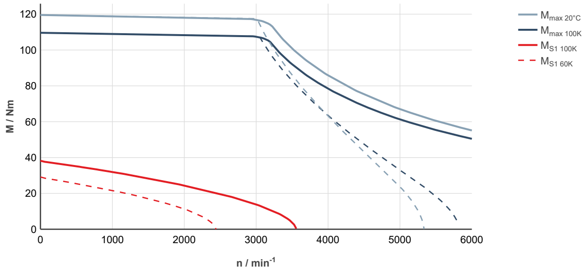
Fig. 121: MS2N07-E0BQN-___0-___- , ctrlX DRIVE, controlled supply 3 × AC 400 ... 480 V
