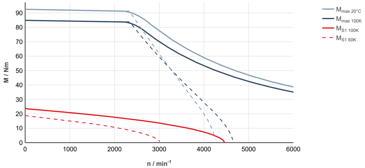
Fig. 113: MS2N07-D1BNN-___0-___-, ctrlX DRIVE, controlled supply 3 × AC 400 ... 480 V
