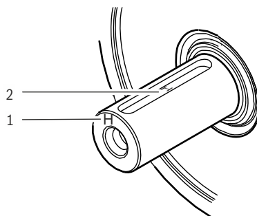
Fig. 5: Identification balancing
