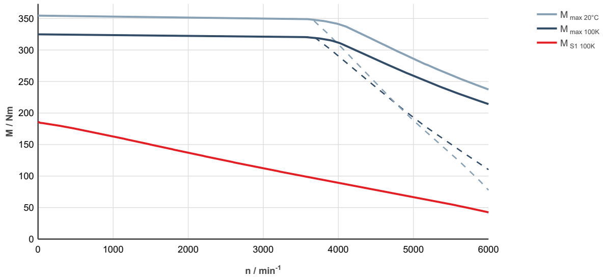
Fig. 290: MS2N10-R0BQL-___0-___-___, ctrlX DRIVE, controlled supply 3 x AC 400 ... 480 V
