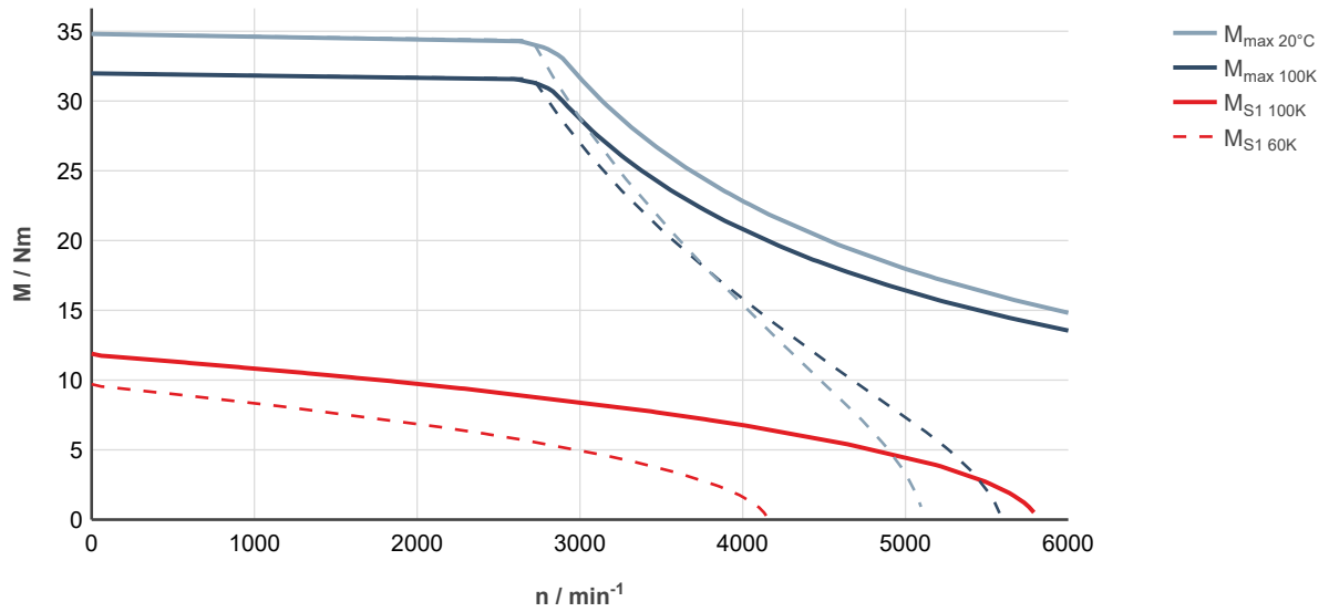
Fig. 76: MS2N06-D0BNN-___0-___-_, ctrlX DRIVE, controlled supply 3 × AC 400 ... 480 V
