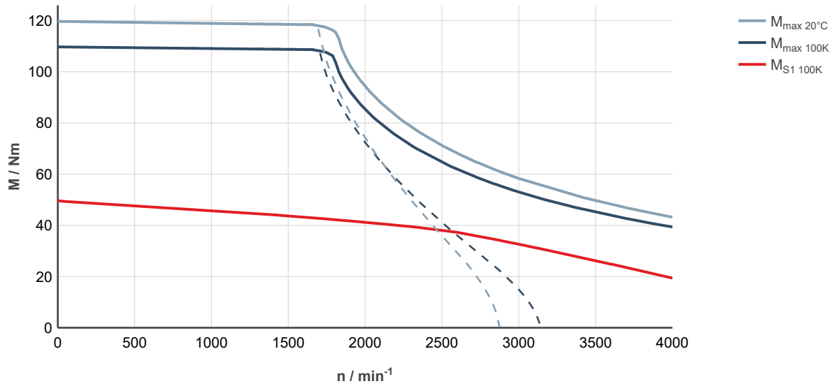
Fig. 153: MS2N07-E0BHA-___0-___-__, ctrlX DRIVE, controlled supply 3 × AC 400 ... 480 V
