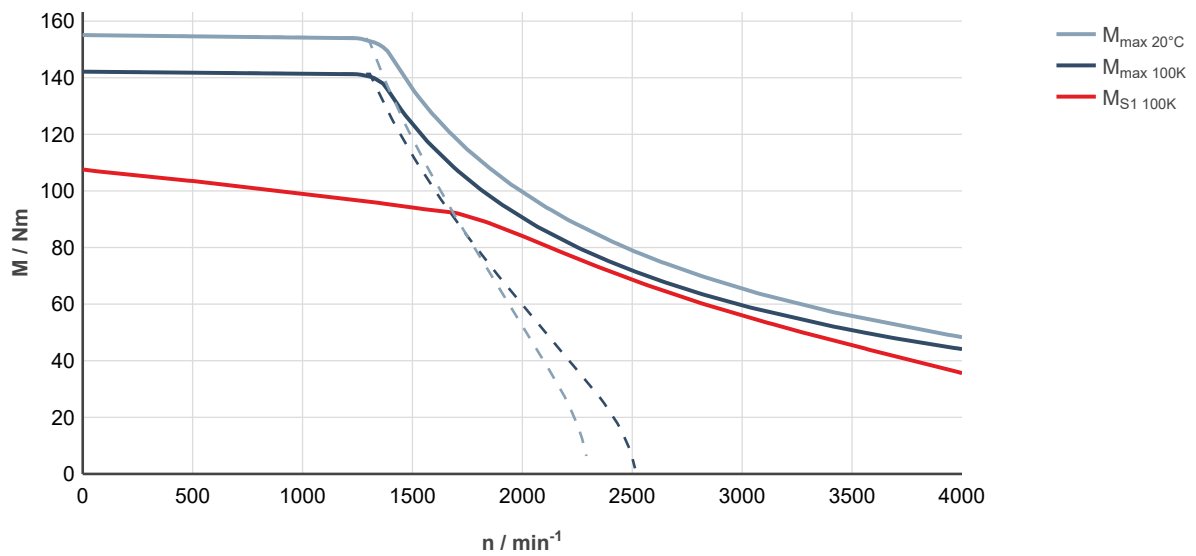
Fig. 269: MS2N10-D0BHL-___0-___-___, ctrIX DRIVE, uncontrolled supply 3 × AC 400 V
