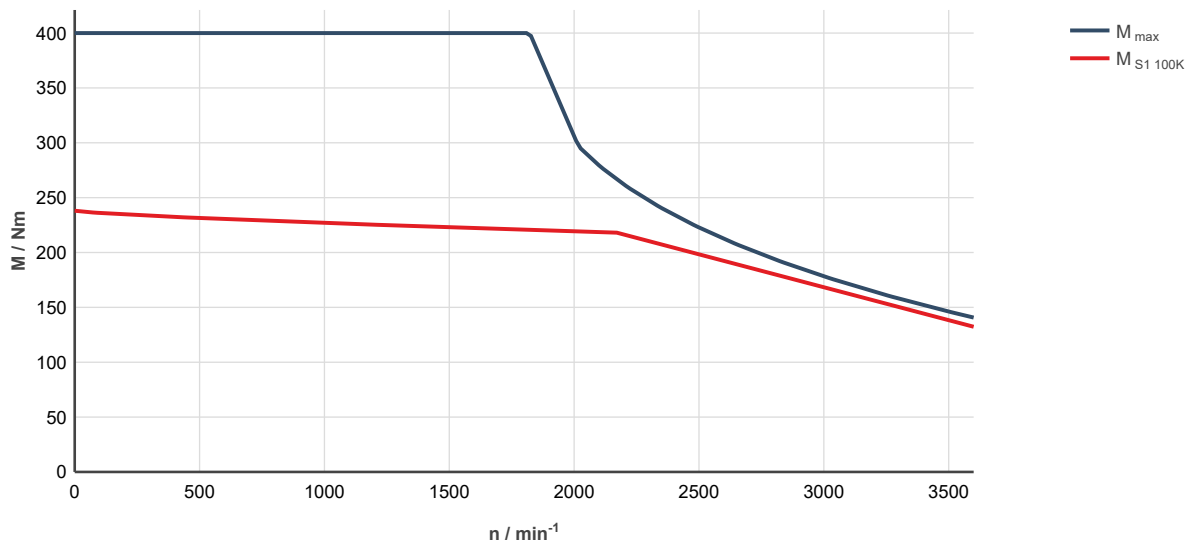
Fig. 339: MS2N13-C1BHL-___0-___-__, ctrlX DRIVE, uncontrolled supply 3 × AC 400 V M_{\text{max}} Characteristic curve applies to maximum torque 20 °C (cold)
