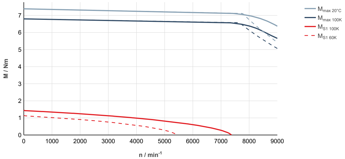
Fig. 29: MS2N03-D0BYN-___0-___-__, ctrlX DRIVE, controlled supply 3 × AC 400 ... 480 V
