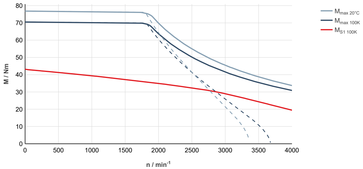
Fig. 230: MS2N10-C0BHA-___0-___-_, ctrlX DRIVE, controlled supply 3 × AC 400 ... 480 V
