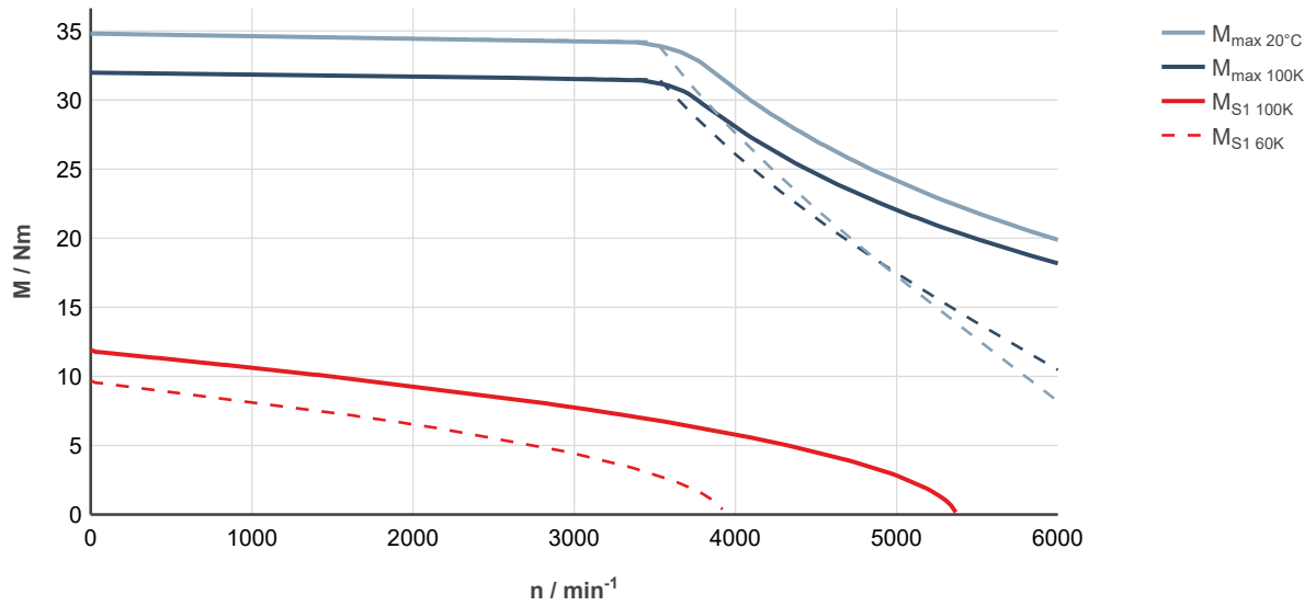
Fig. 78: MS2N06-D0BRN-___0-___-___, ctrlX DRIVE, controlled supply 3 × AC 400 ... 480 V
