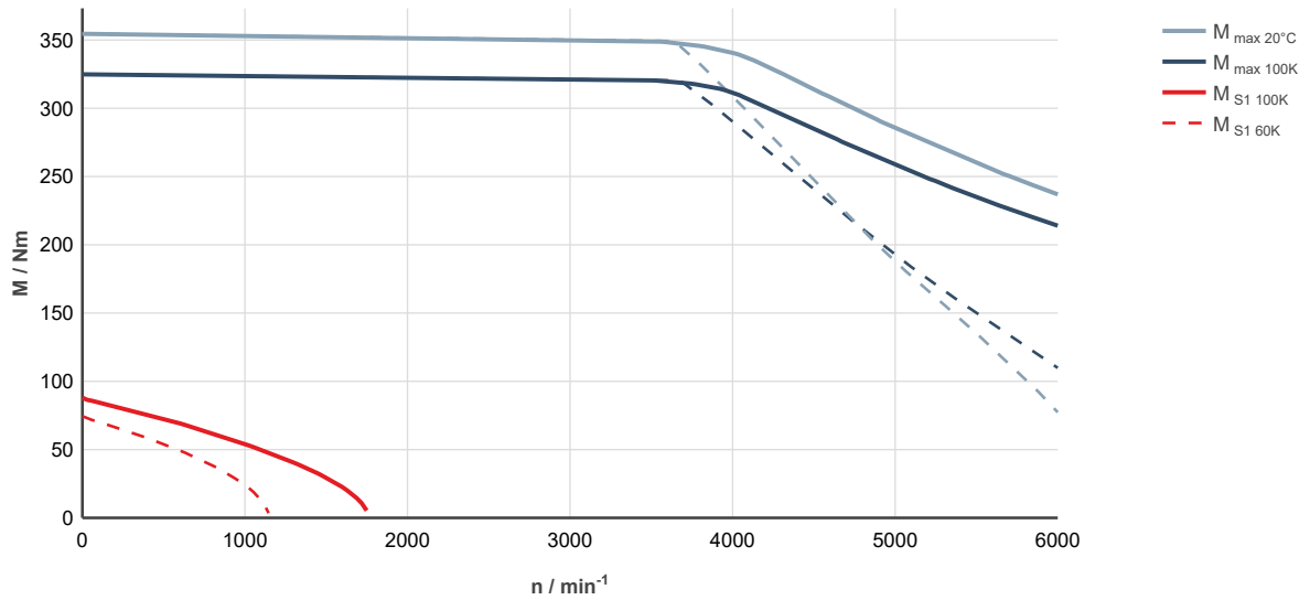
Fig. 228: MS2N10-R0BQN-___0-N___-_, ctrlX DRIVE, controlled supply 3 x AC 400 ... 480 V
