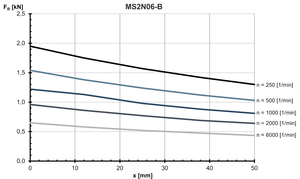
Fig. 86: MS2N06-B: Radial force in distance x from the shaft shoulder at a nominal bearing service life of L_{h10} = 30000 h
