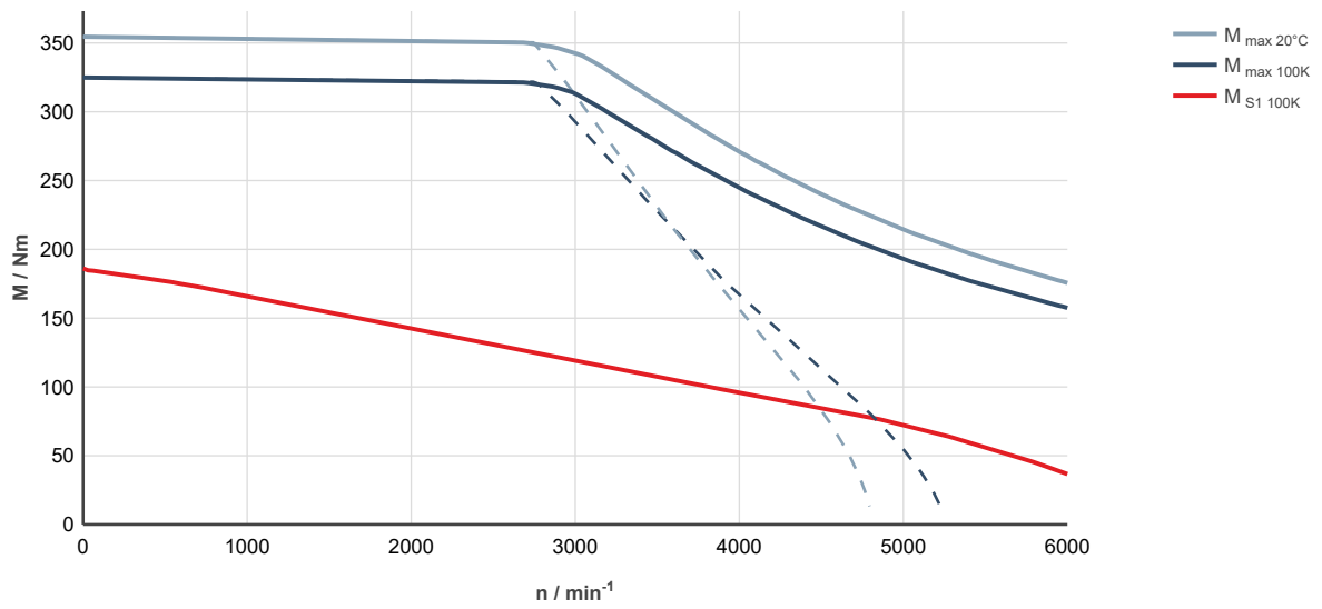
Fig. 289: MS2N10-R0BQL-___0-___-___, ctrlX DRIVE, uncontrolled supply 3 × AC 400 V
