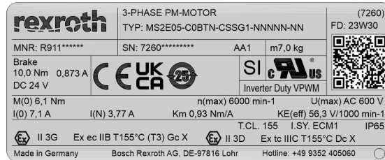
Fig. 1: Type plate MS2N (example)
