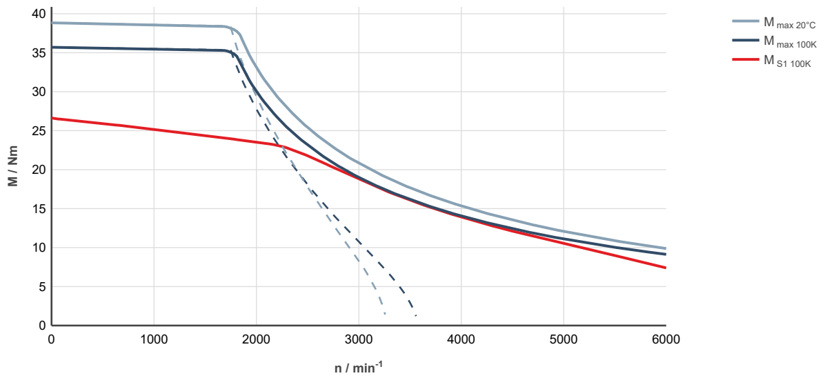
Fig. 164: MS2N07-C0BNL-___0-___-___, ctrlX DRIVE, uncontrolled supply 3 × AC 400 V
