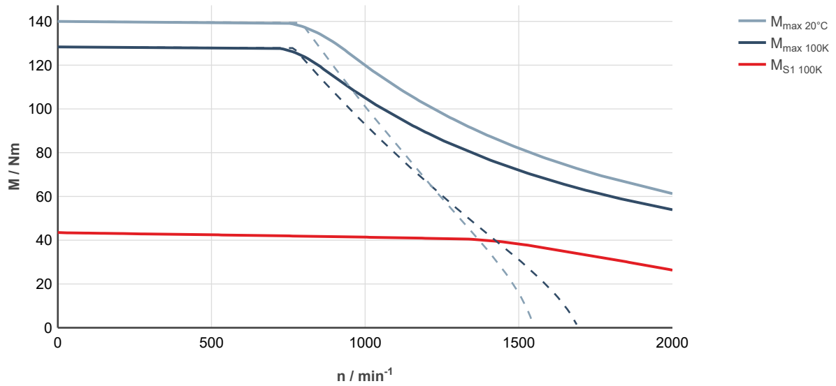
Fig. 159: MS2N07-E1BDA-___0-___-_, ctrlX DRIVE, controlled supply 3 × AC 400 ... 480 V
