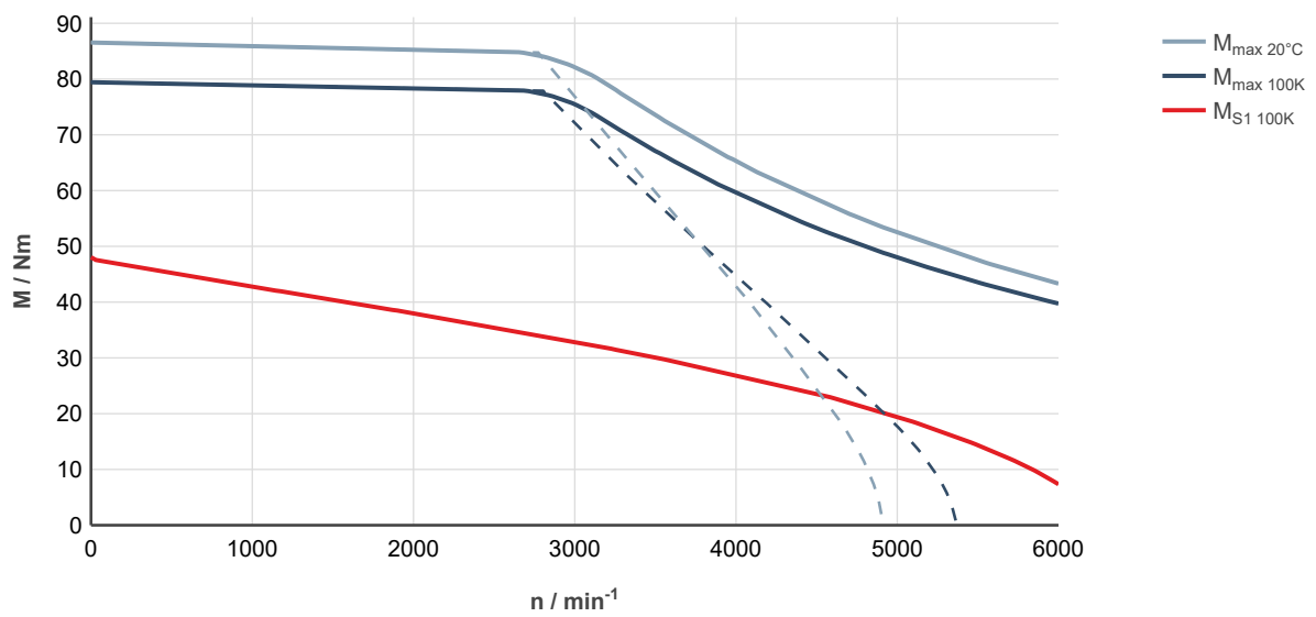
Fig. 268: MS2N10-C1BNL-___0-___-___, ctrIX DRIVE, controlled supply 3 × AC 400 ... 480 V
