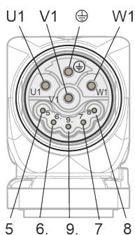
Fig. 381: Connector view of M23 performance connector
