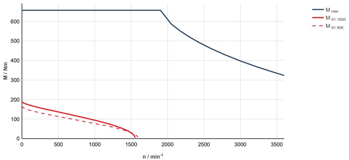
Fig. 317: MS2N13-E1BNN-___0-___-_, ctrlX DRIVE, uncontrolled supply 3 × AC 400 V M_{max} : Characteristic curve applies to maximum torque 20 °C (cold)
