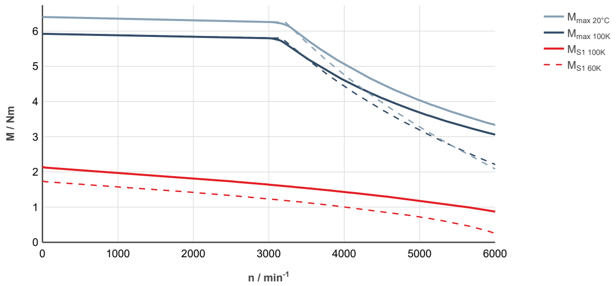
Fig. 37: MS2N04-B0BTN-___0-___-_, ctrlX DRIVE, uncontrolled supply 3 × AC 400 V
