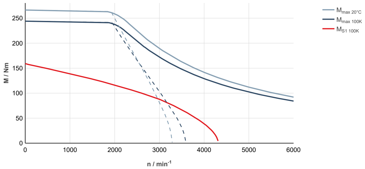
Fig. 279: MS2N10-E1BNL-___0-___-___, ctrlX DRIVE, uncontrolled supply 3 × AC 400 V
