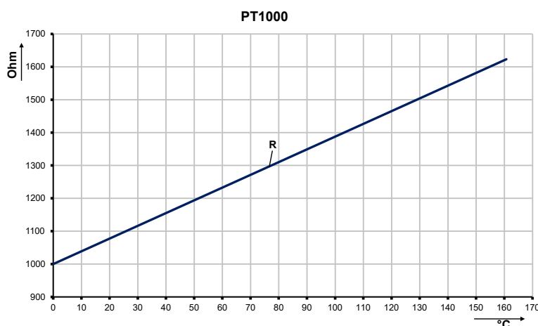
Fig. 2: Characteristic curve PT1000
