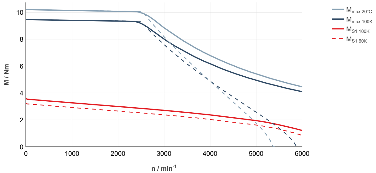
Fig. 70: MS2N06-B1BNN-___0-___-___, ctrlIX DRIVE, controlled supply 3 × AC 400 ... 480 V
