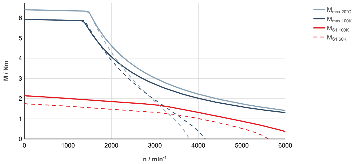
Fig. 35: MS2N04-B0BNN-___0-___-___, ctrlX DRIVE, uncontrolled supply 3 × AC 400 V
