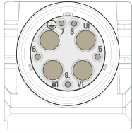
Fig. 385: Connector view of M58 performance connector
