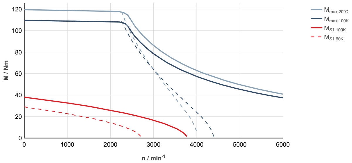
Fig. 120: MS2N07-E0BQN-___0-___- , ctrlX DRIVE, uncontrolled supply 3 × AC 400 V
