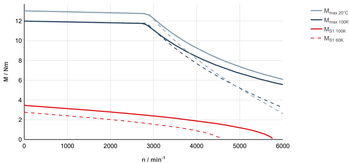
Fig. 41: MS2N04-C0BTN-___0-___-__, ctrlX DRIVE, uncontrolled supply 3 × AC 400 V
