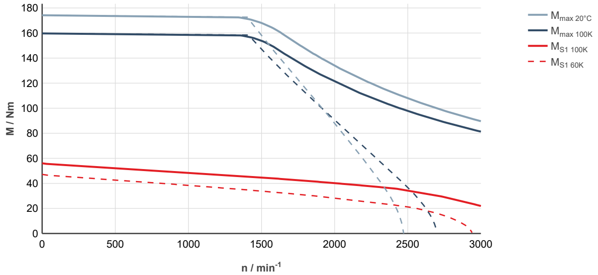
Fig. 208: MS2N10-D1BFN-___0-___-_, ctrlX DRIVE, controlled supply 3 × AC 400 ... 480 V
