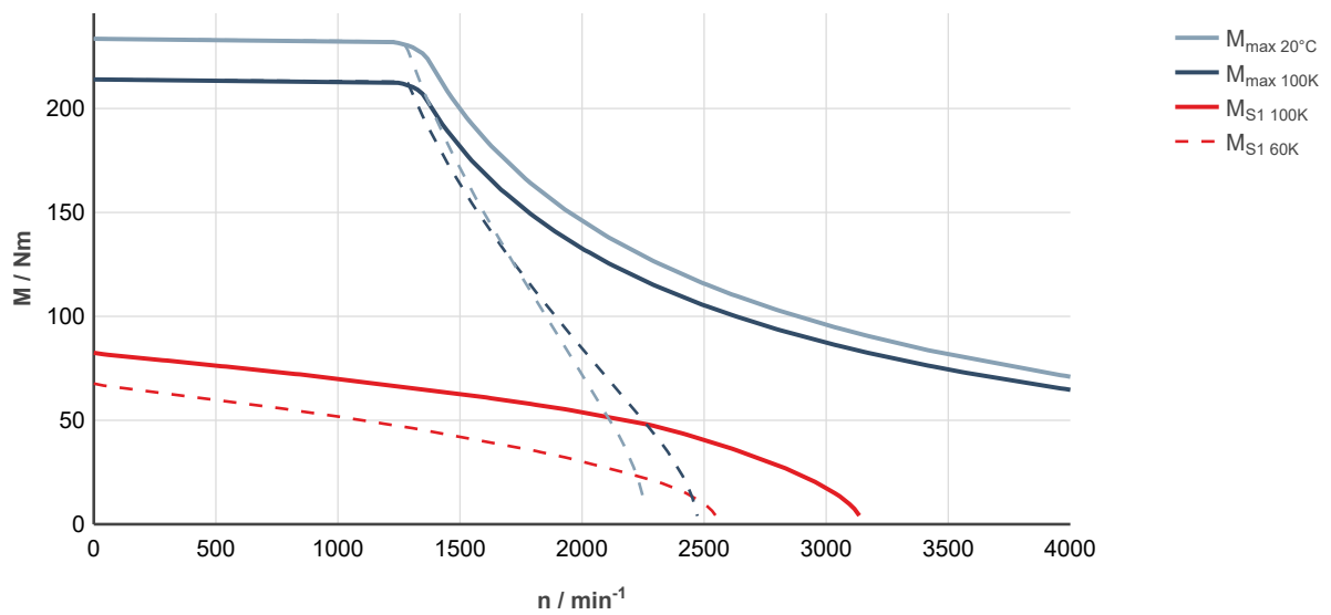
Fig. 211: MS2N10-E0BHN-___0-___-_, ctrlX DRIVE, uncontrolled supply 3 × AC 400 V
