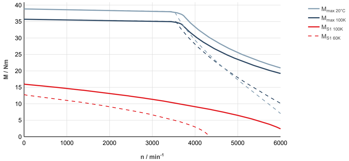
Fig. 95: MS2N07-C0BQN-___0-___-_, ctrlX DRIVE, controlled supply 3 × AC 400 ... 480 V
