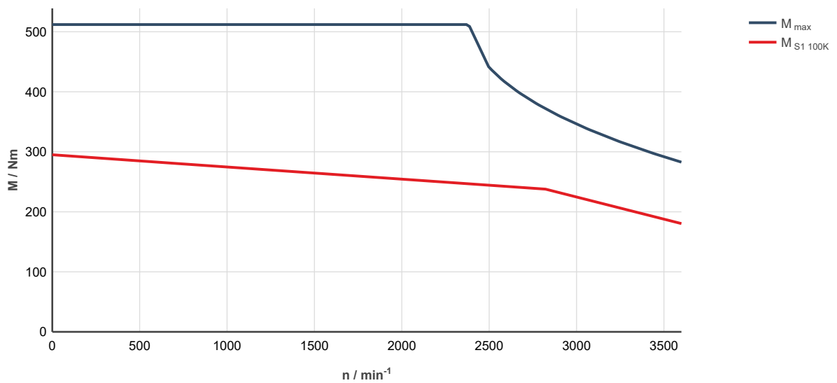
Fig. 345: MS2N13-D1BNL-___0-___-__, ctrlX DRIVE, uncontrolled supply 3 × AC 400 V M_{\text{max}} : Characteristic curve applies to maximum torque 20 °C (cold)
