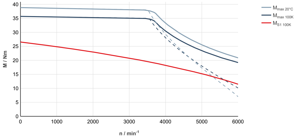
Fig. 167: MS2N07-C0BQL-__0-__-__, ctrlX DRIVE, controlled supply 3 × AC 400 ... 480 V
