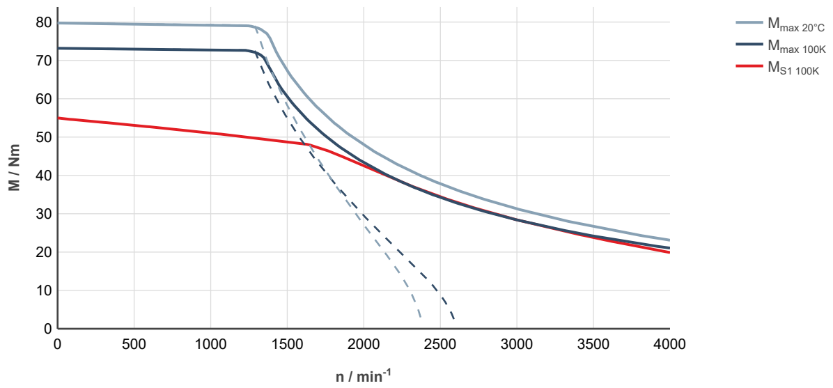
Fig. 170: MS2N07-D0BHL-___0-___-___, ctrIX DRIVE, uncontrolled supply 3 × AC 400 V
