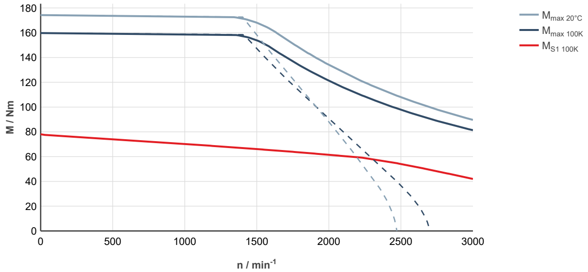
Fig. 242: MS2N10-D1BFA-___0-___-__, ctrlX DRIVE, controlled supply 3 × AC 400 ... 480 V
