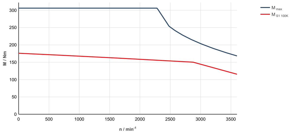
Fig. 336: MS2N13-B1BHL-__0-__-__, ctrlX DRIVE, controlled supply 3 x AC 400 ... 480 V M_{\text{max}} : Characteristic curve applies to maximum torque 20 °C (cold)
