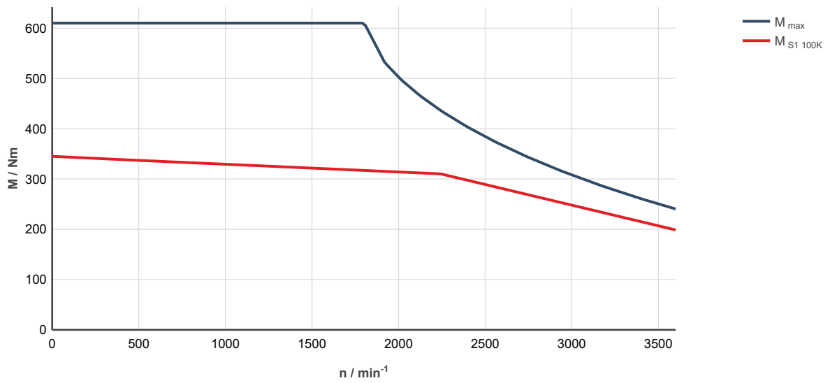
Fig. 347: MS2N13-E1BHL-__0-__-__, ctrlX DRIVE, uncontrolled supply 3 × AC 400 V M_{\text{max}} : Characteristic curve applies to maximum torque 20 °C (cold)
