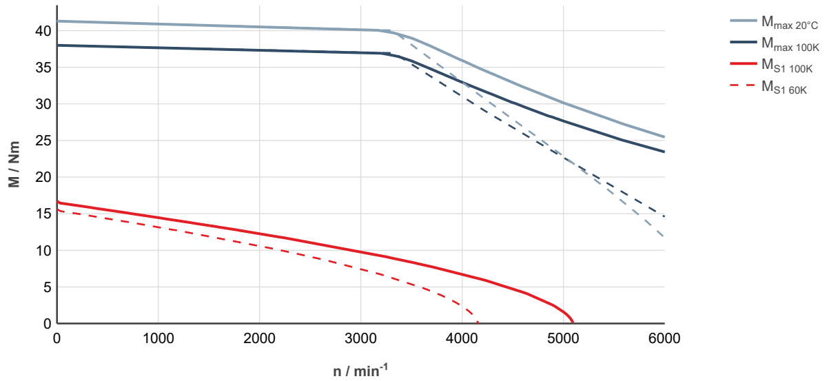
Fig. 194: MS2N10-B1BQN-___0-___-, ctrlX DRIVE, controlled supply 3 × AC 400 ... 480 V
