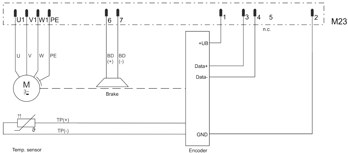
Fig. 359: M23 Single cable connection, digital encoder C, D, H, optional brake
