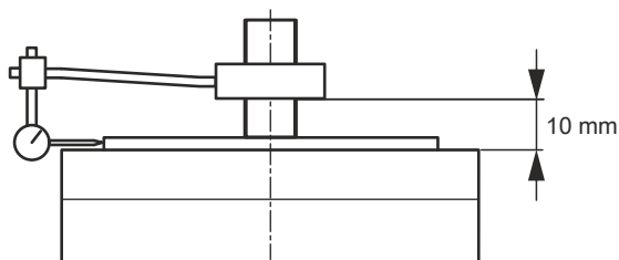
Fig. 15: Measuring system of coaxiality
