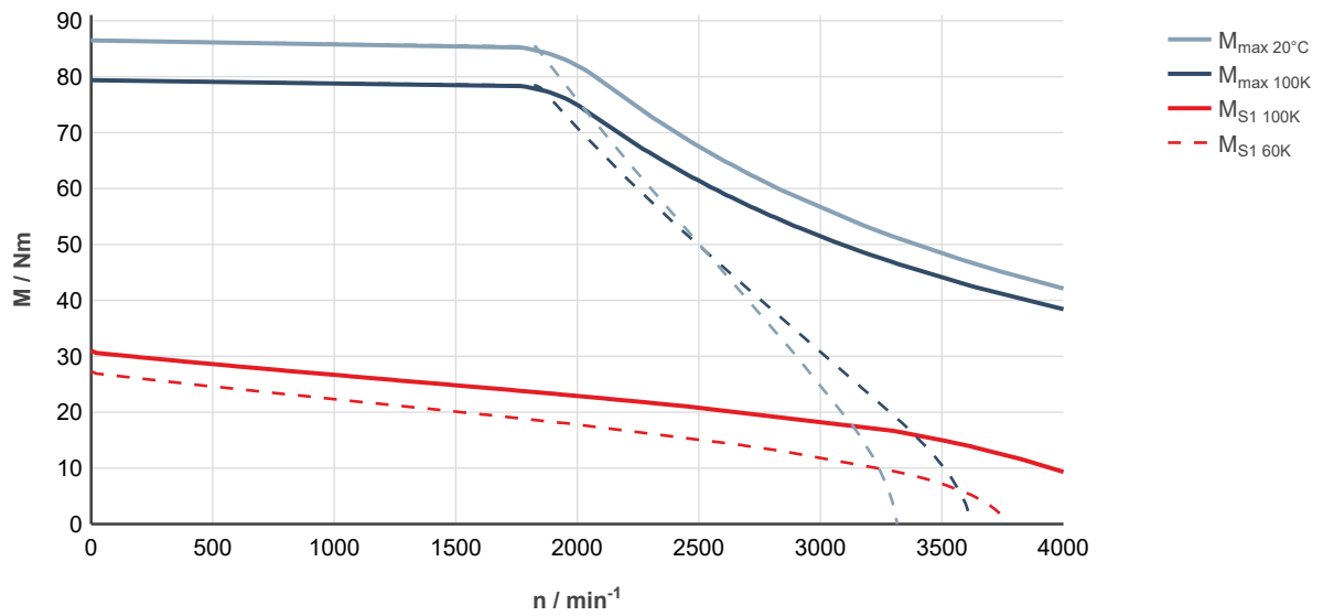
Fig. 200: MS2N10-C1BHN-___0-___-_, ctrlX DRIVE, controlled supply 3 × AC 400 ... 480 V
