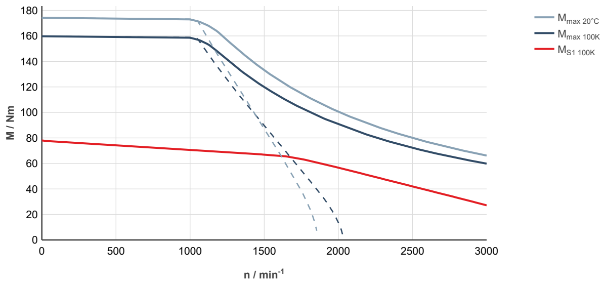
Fig. 241: MS2N10-D1BFA-___0-___-__, ctrlX DRIVE, uncontrolled supply 3 × AC 400 V
