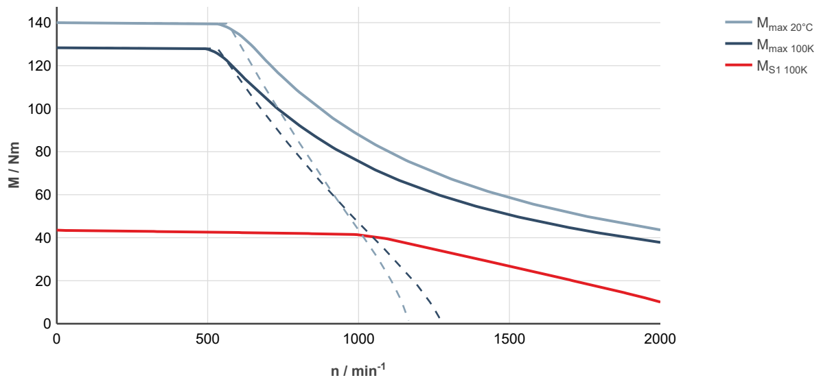
Fig. 158: MS2N07-E1BDA-___0-___-_, ctrlX DRIVE, uncontrolled supply 3 × AC 400 V
