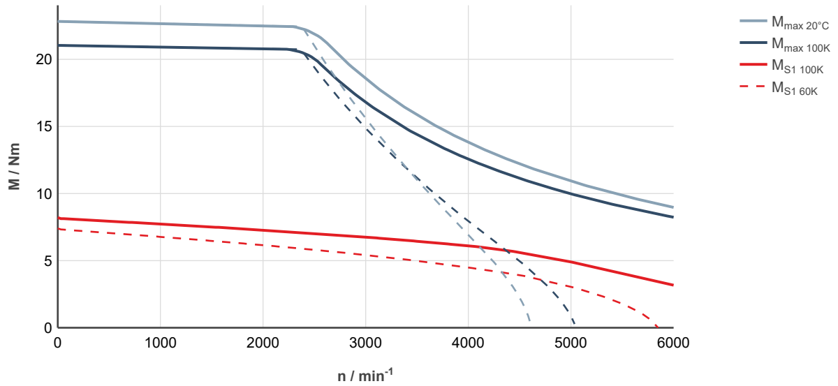
Fig. 91: MS2N07-B1BNN-___0-___-, ctrlX DRIVE, controlled supply 3 × AC 400 ... 480 V
