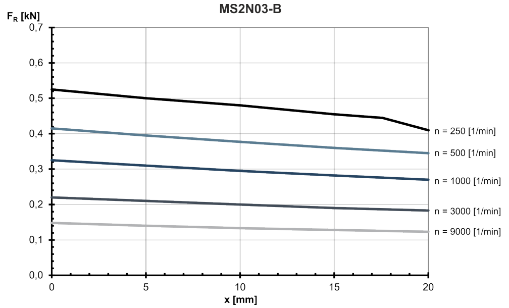
Fig. 33: MS2N03-B: Radial force in distance x from the shaft shoulder at a nominal bearing service life of L_{h10} = 30000 h
