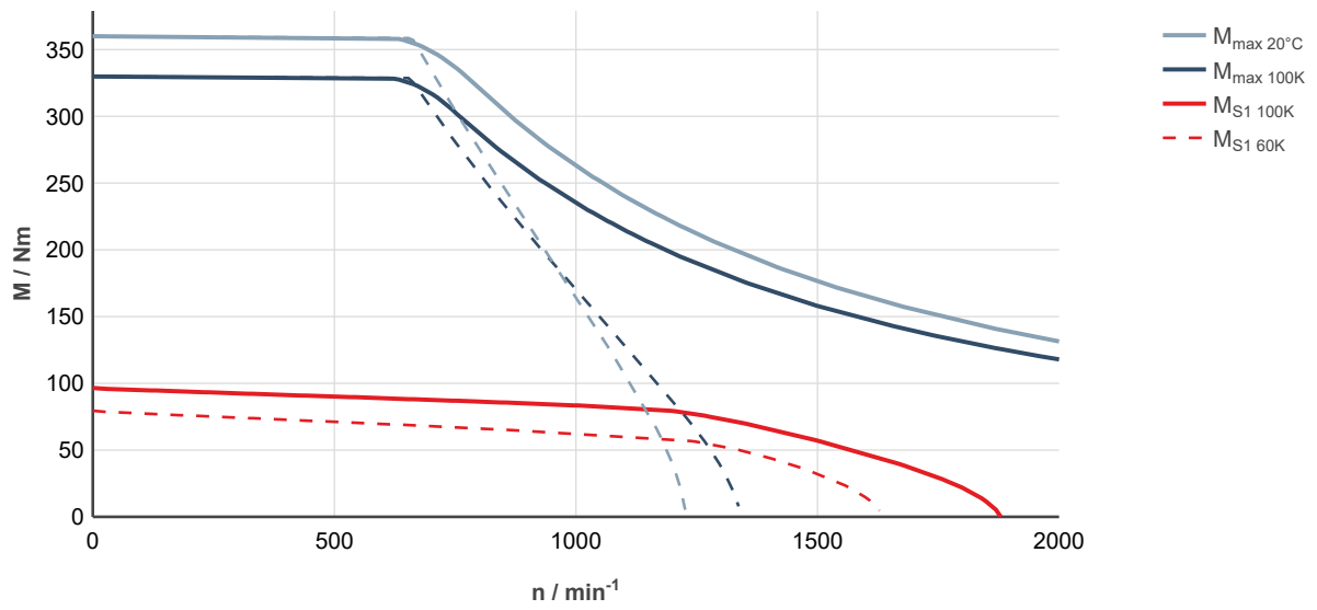
Fig. 223: MS2N10-F1BDN-___0-___-_, ctrlX DRIVE, uncontrolled supply 3 × AC 400 V
