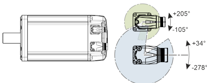
Fig. 368: Rotating area electrical connection "U"
