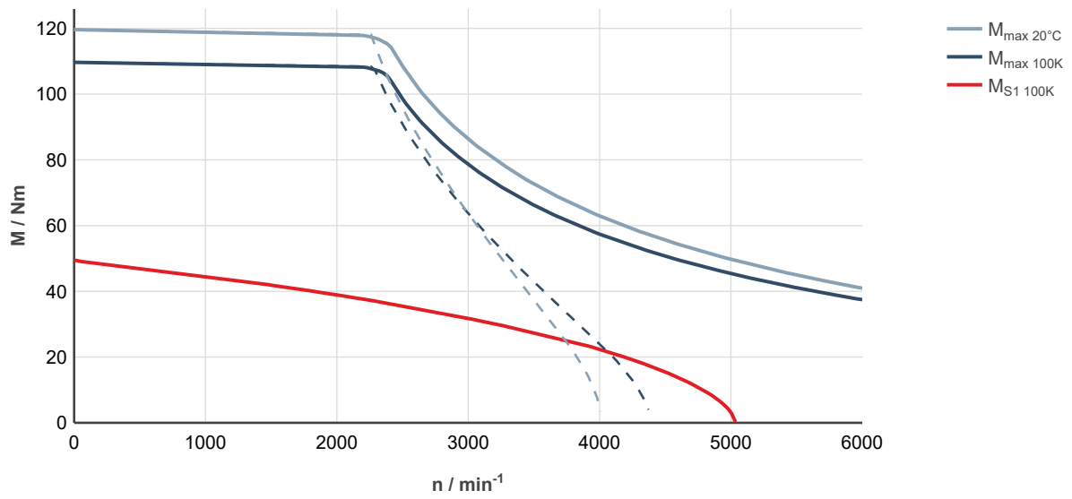
Fig. 156: MS2N07-E0BQA-___0-___-__, ctrlX DRIVE, uncontrolled supply 3 × AC 400 V
