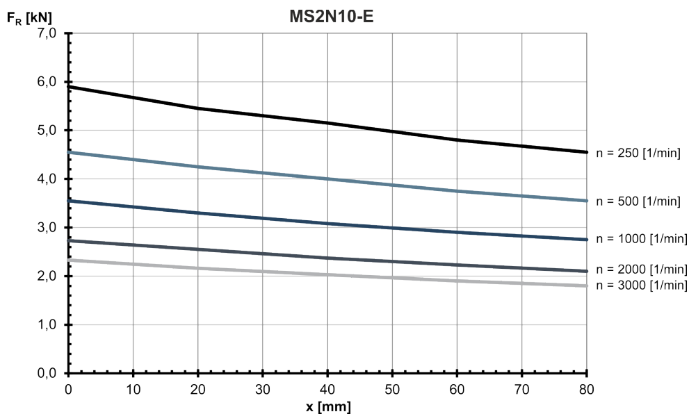
Fig. 300: MS2N10-E: Radial force in distance x from the shaft shoulder at a nominal bearing service life of L_{h10} = 30000 h
