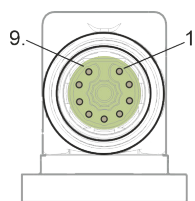
Fig. 367: Connector view of M17 encoder connector
