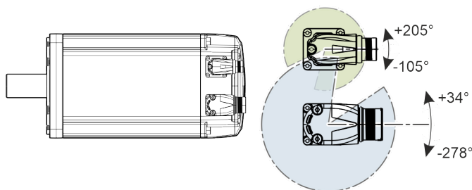
Fig. 382: : Rotating area electrical connection "U"
