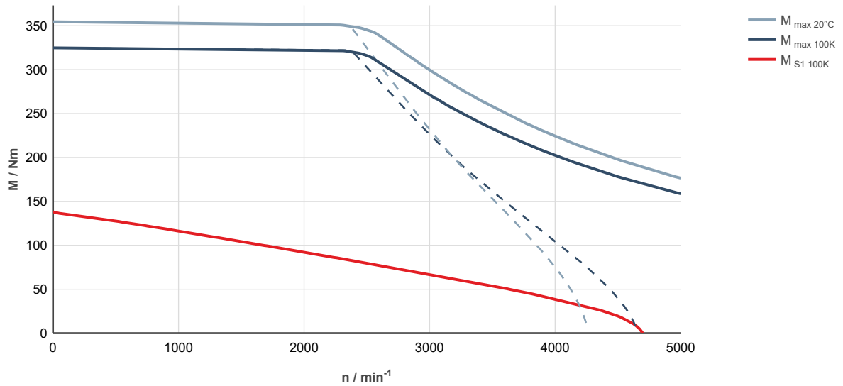
Fig. 262: MS2N10-R0BLA-___-___-___, ctrlX DRIVE, controlled supply 3 x AC 400 ... 480 V
