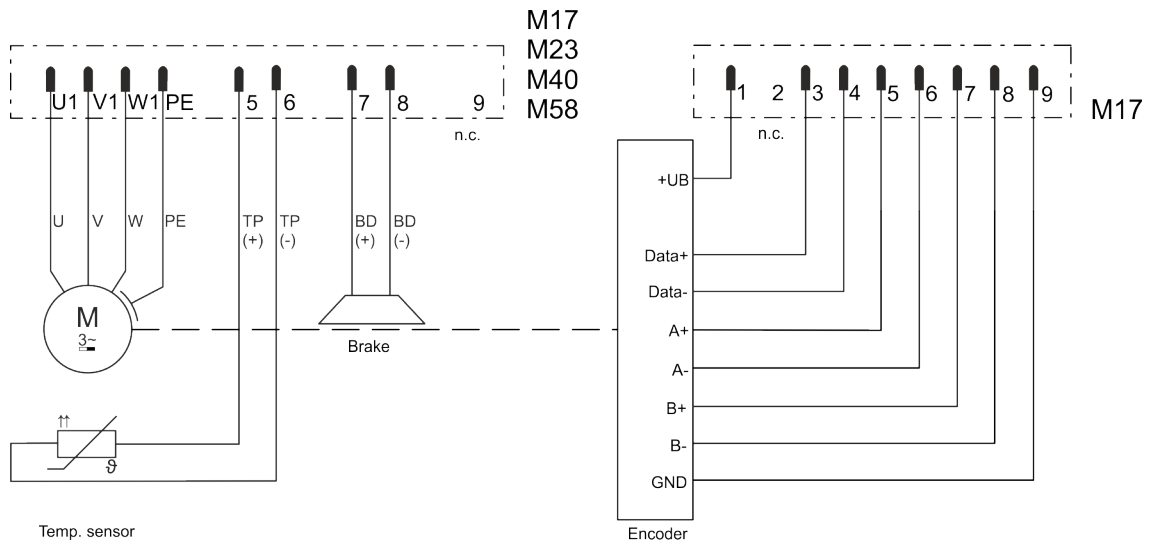
Fig. 360: Double cable connection, analog encoder A, brake optional
