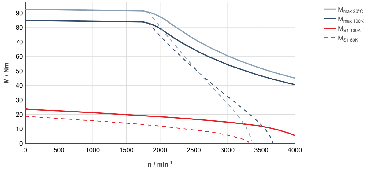
Fig. 111: MS2N07-D1BHN-___0-___-, ctrlX DRIVE, controlled supply 3 × AC 400 ... 480 V
