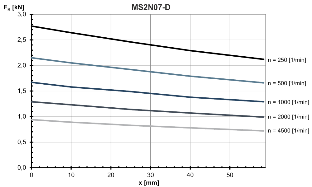
Fig. 191: MS2N07-D: Radial force in distance x from the shaft shoulder at a nominal bearing service life of L_{h10} = 30000 h
