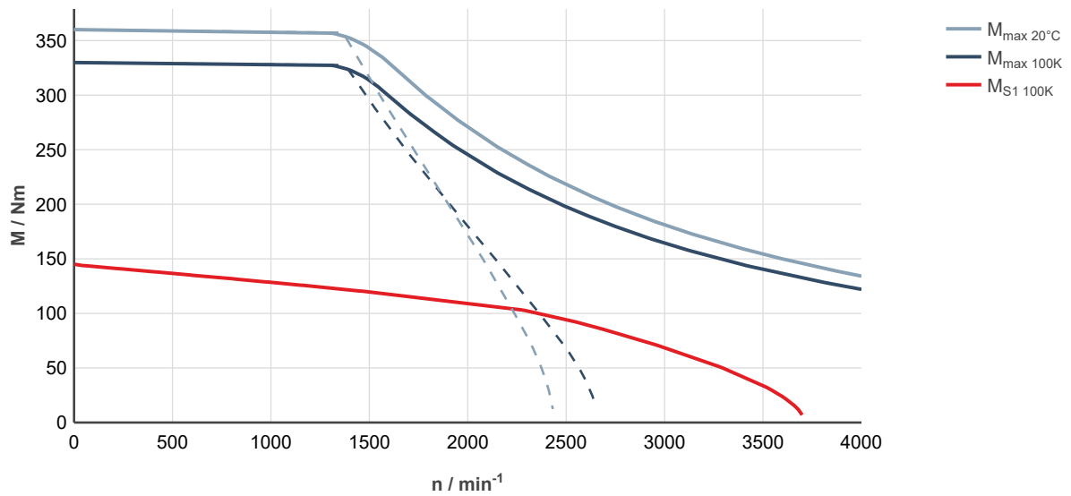
Fig. 259: MS2N10-F1BHA-___0-___-__, ctrlX DRIVE, uncontrolled supply 3 × AC 400 V
