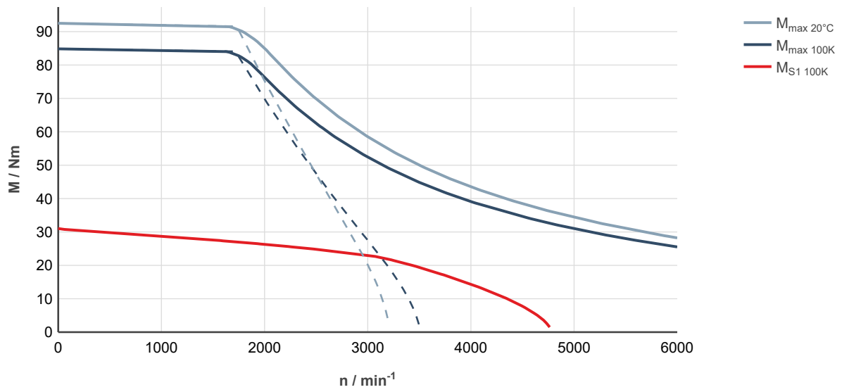
Fig. 148: MS2N07-D1BNA-___0-___- , ctrlX DRIVE, uncontrolled supply 3 × AC 400 V
