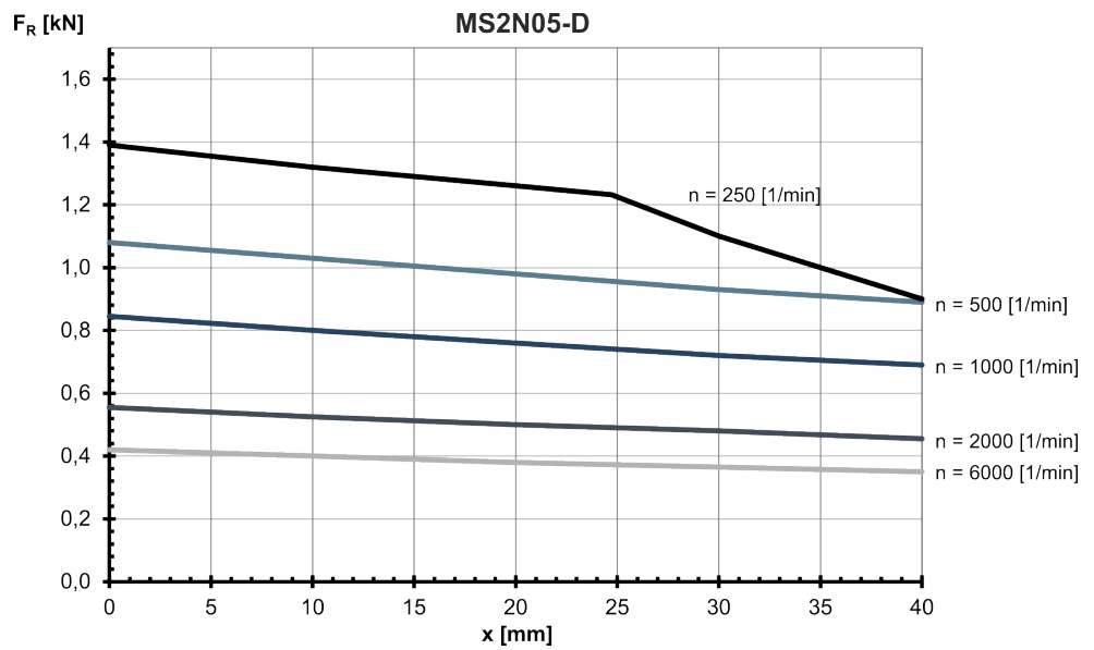
Fig. 68: MS2N05-D: Radial force in distance x from the shaft shoulder at a nominal bearing service life of L_{h10} = 30000 h
