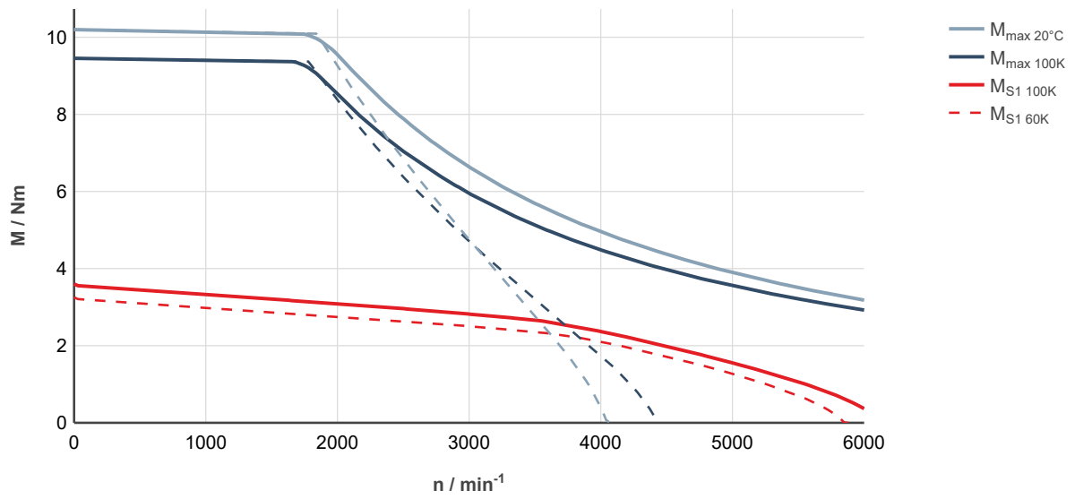
Fig. 69: MS2N06-B1BNN-___0-___-___, ctrlIX DRIVE, uncontrolled supply 3 × AC 400 V
