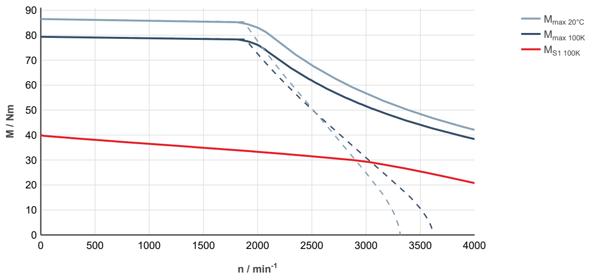
Fig. 234: MS2N10-C1BHA-___0-___-_, ctrlX DRIVE, controlled supply 3 × AC 400 ... 480 V
