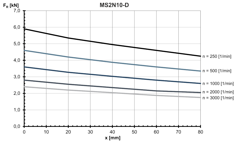
Fig. 299: MS2N10-D: Radial force in distance x from the shaft shoulder at a nominal bearing service life of L_{h10} = 30000 h
