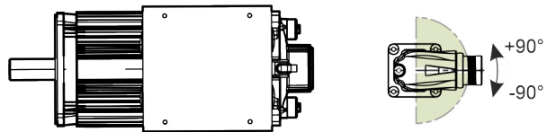
Fig. 373: Rotating area electrical connection "E"
