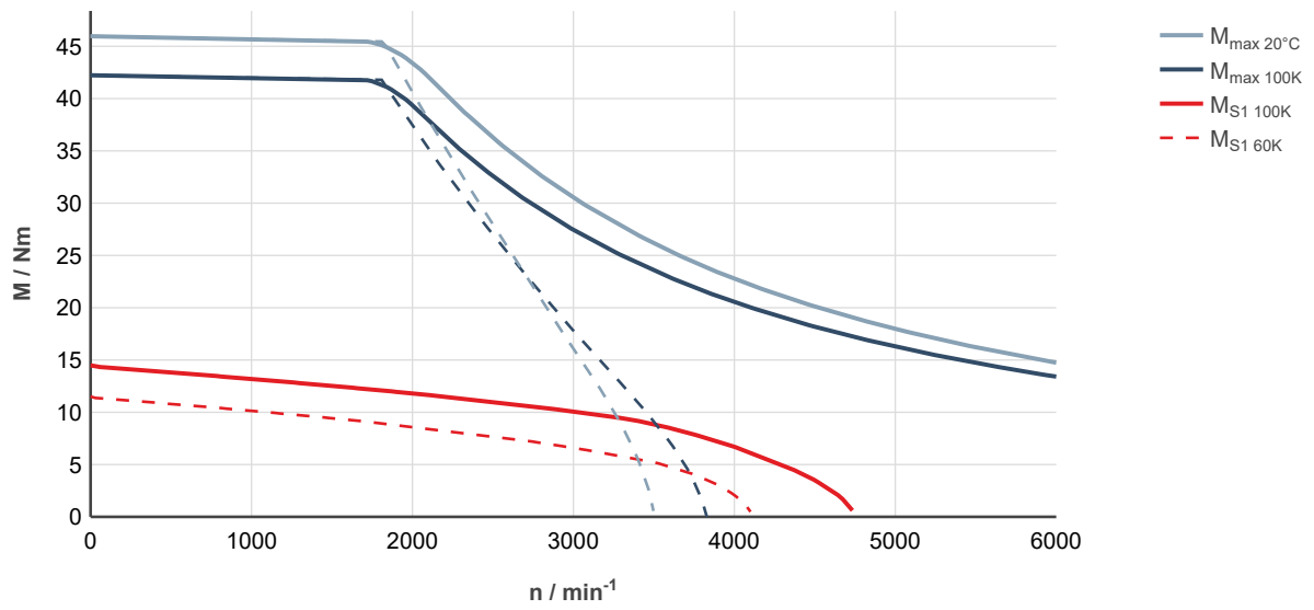
Fig. 96: MS2N07-C1BNN-___0-___-__, ctrlX DRIVE, uncontrolled supply 3 × AC 400 V
