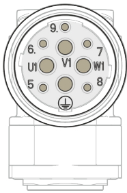
Fig. 383: Connector view of M40 performance connector
