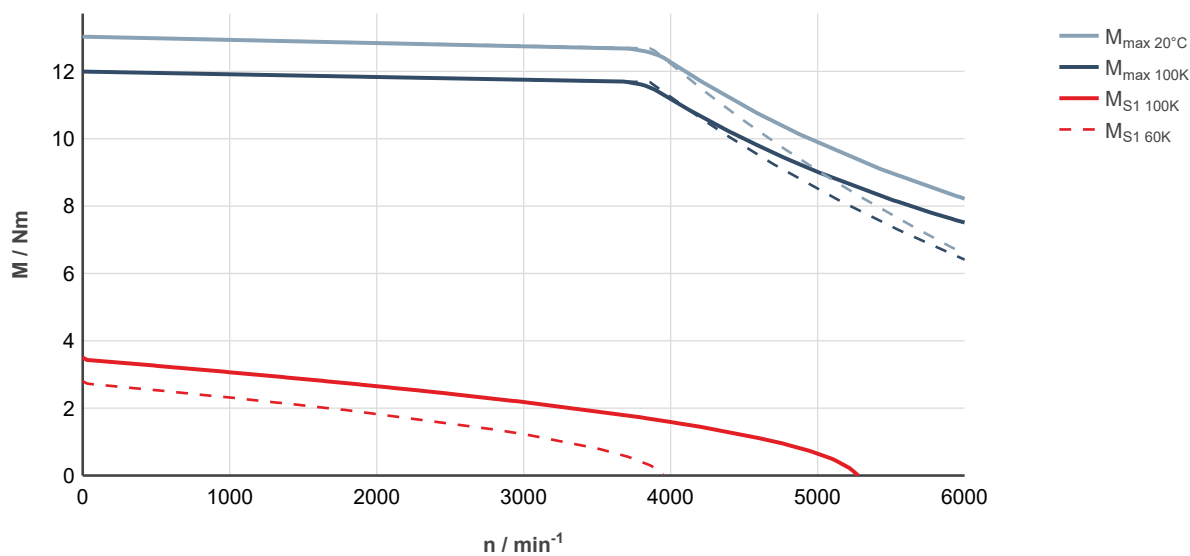
Fig. 42: MS2N04-C0BTN-___0-___-__, ctrlX DRIVE, controlled supply 3 × AC 400 ... 480 V
