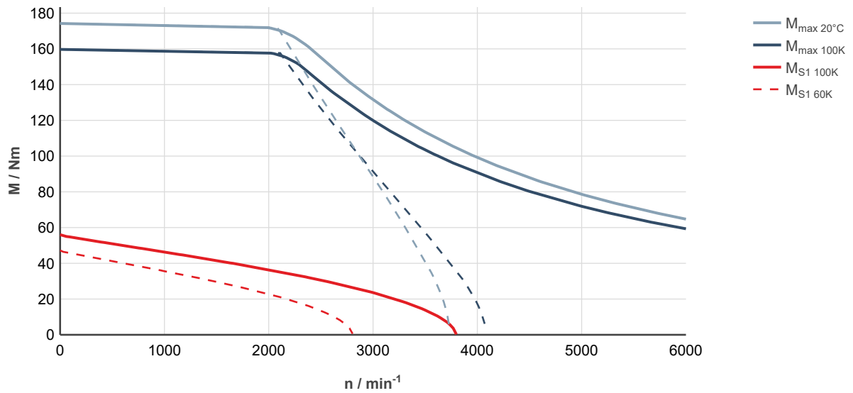
Fig. 209: MS2N10-D1BNN-___0-___-_, ctrlX DRIVE, uncontrolled supply 3 × AC 400 V
