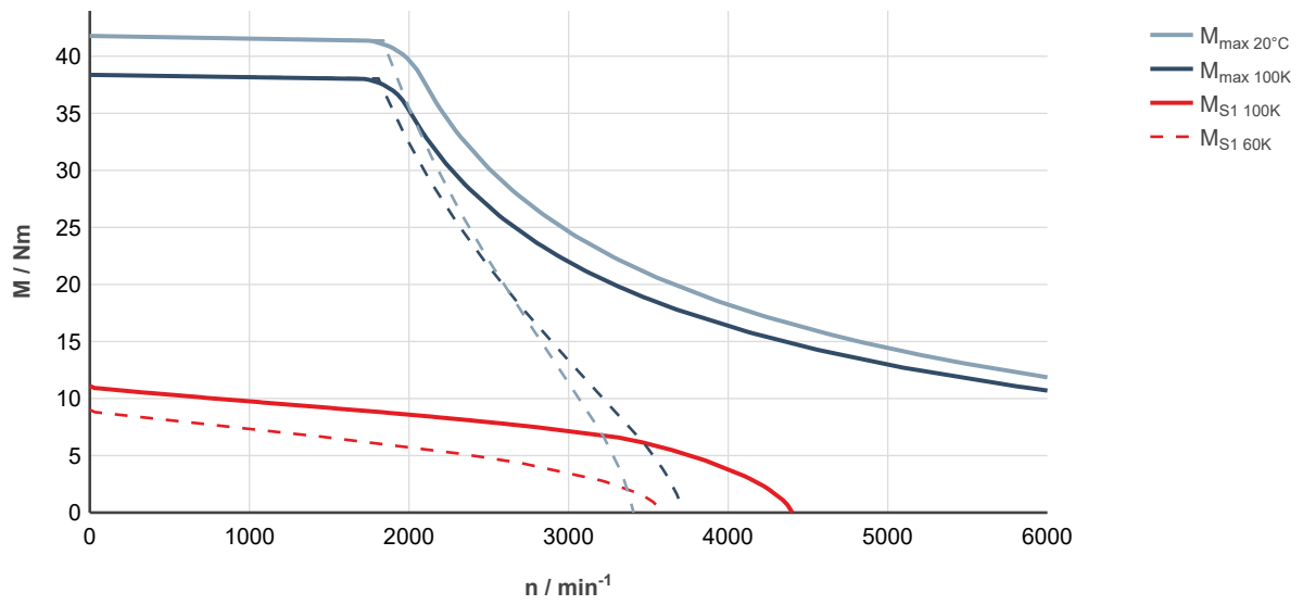
Fig. 79: MS2N06-D1BNN-___0-___-_, ctrlX DRIVE, uncontrolled supply 3 × AC 400 V
