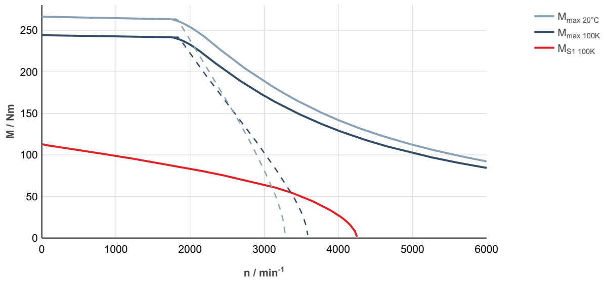
Fig. 251: MS2N10-E1BNA-___0-___-__, ctrlX DRIVE, uncontrolled supply 3 × AC 400 V
