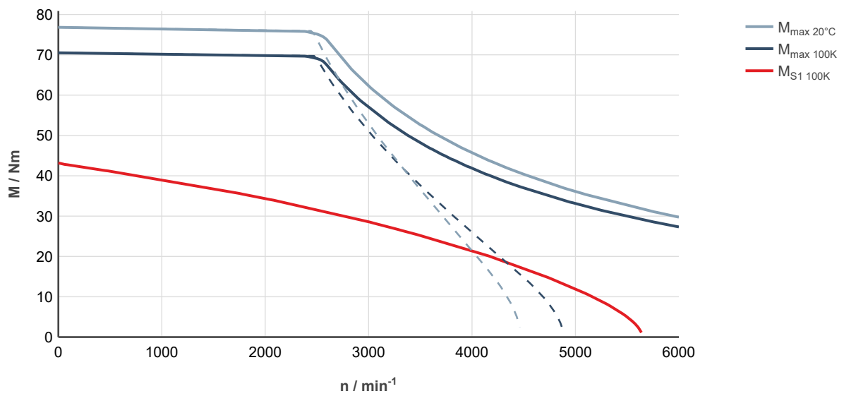
Fig. 232: MS2N10-C0BNA-___0-___-_, ctrlX DRIVE, controlled supply 3 × AC 400 ... 480 V
