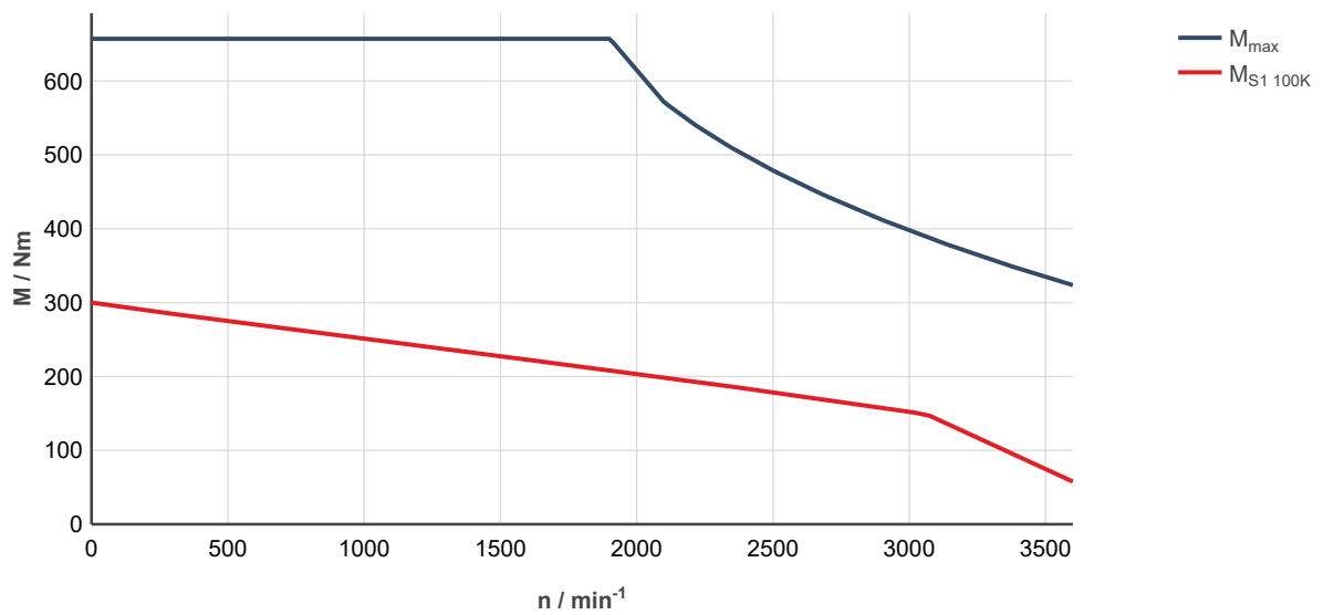
Fig. 333: MS2N13-E1BNC-___0-___-__, ctrlX DRIVE, uncontrolled supply 3 × AC 400 V M_{\text{max}} Characteristic curve applies to maximum torque 20 °C (cold)
