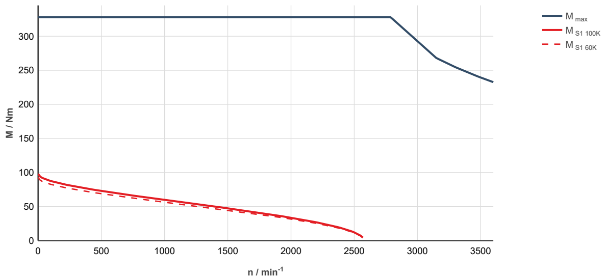
Fig. 306: MS2N13-B1BNN-___0-___-_, ctrIX DRIVE, controlled supply 3 x AC 400 ... 480 V M_{\text{max}} : Characteristic curve applies to maximum torque 20 °C (cold)
