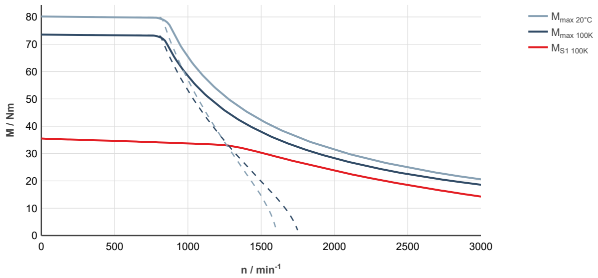
Fig. 136: MS2N07-D0BFA-___0-___-___, ctrlX DRIVE, uncontrolled supply 3 × AC 400 V
