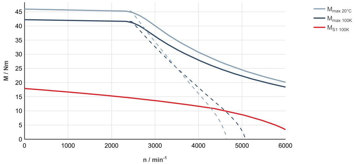
Fig. 133: MS2N07-C1BNA-___0-___-_, ctrlX DRIVE, controlled supply 3 × AC 400 ... 480 V
