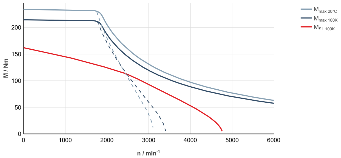
Fig. 277: MS2N10-E0BNL-___0-___-___, ctrlX DRIVE, uncontrolled supply 3 × AC 400 V
