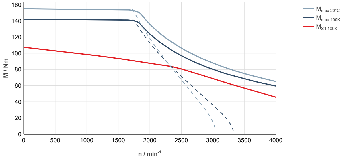
Fig. 270: MS2N10-D0BHL-___0-___-___, ctrIX DRIVE, controlled supply 3 × AC 400 ... 480 V
