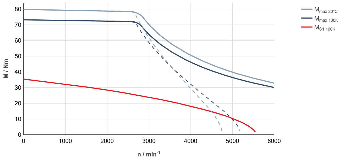
Fig. 142: MS2N07-D0BRA-___0-___-_, ctrlX DRIVE, uncontrolled supply 3 × AC 400 V
