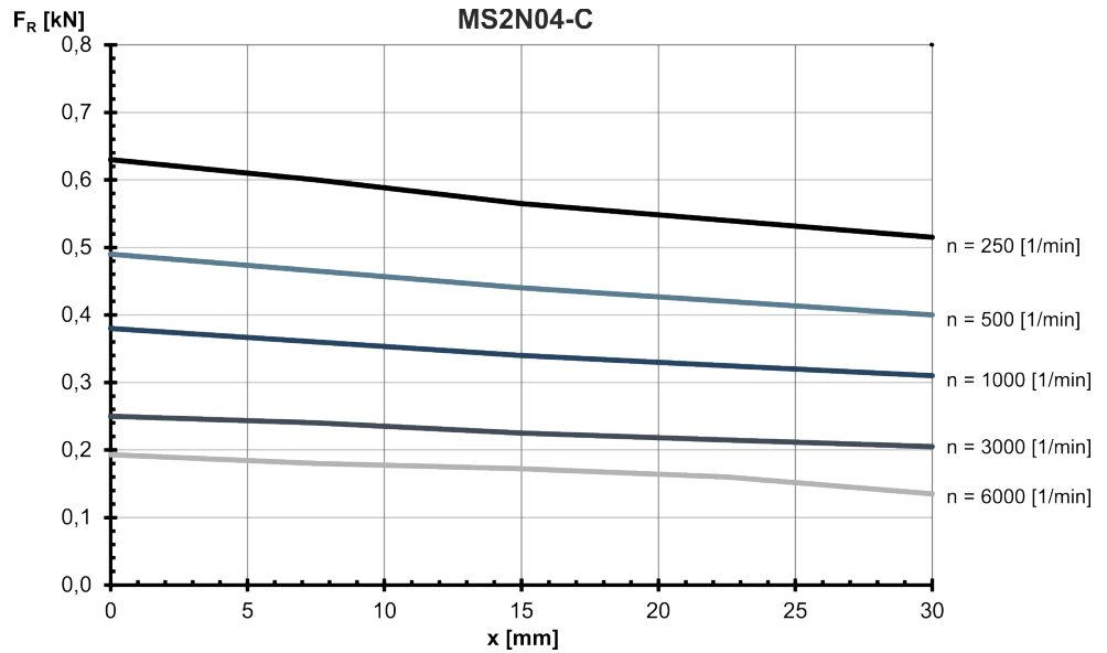
Fig. 50: MS2N04-C: Radial force in distance x from the shaft shoulder at a nominal bearing service life of L_{h10} = 30000 h
