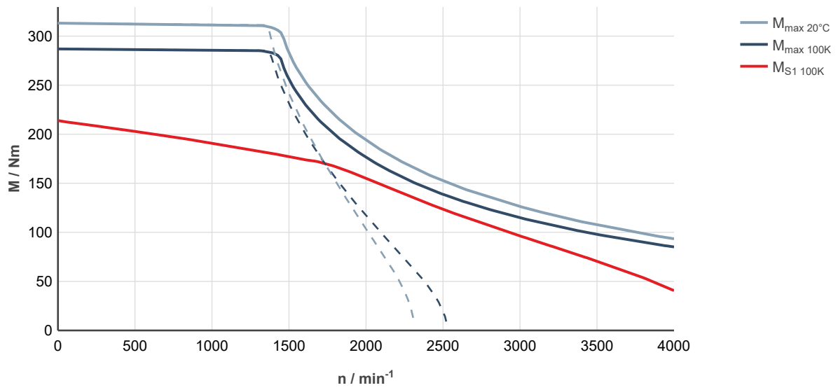
Fig. 281: MS2N10-F0BHL-___0-___-___, ctrlX DRIVE, uncontrolled supply 3 × AC 400 V
