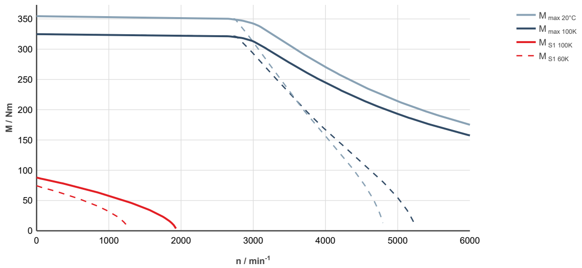
Fig. 227: MS2N10-R0BQN-___0-N___-_, ctrlX DRIVE, uncontrolled supply 3 × AC 400 V
