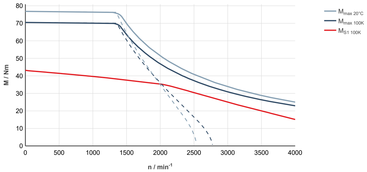
Fig. 229: MS2N10-C0BHA-___0-___-_, ctrlX DRIVE, uncontrolled supply 3 × AC 400 V
