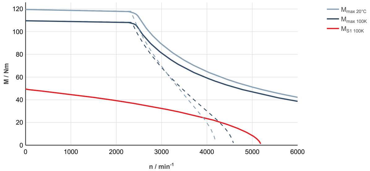
Fig. 155: MS2N07-E0BNA-___0-___-_, ctrlX DRIVE, controlled supply 3 × AC 400 ... 480 V
