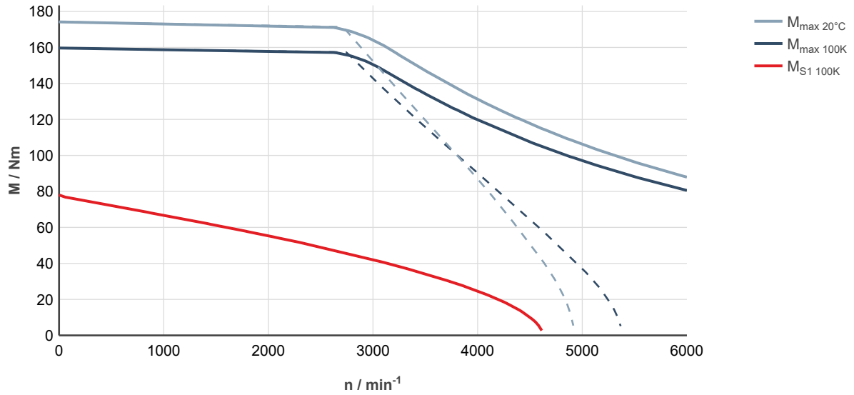
Fig. 244: MS2N10-D1BNA-___0-___-_, ctrlX DRIVE, controlled supply 3 × AC 400 ... 480 V
