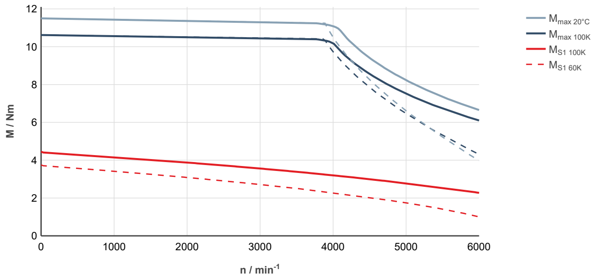
Fig. 54: MS2N05-B0BTN-___0-___-_, ctrlIX DRIVE, uncontrolled supply 3 × AC 400 V
