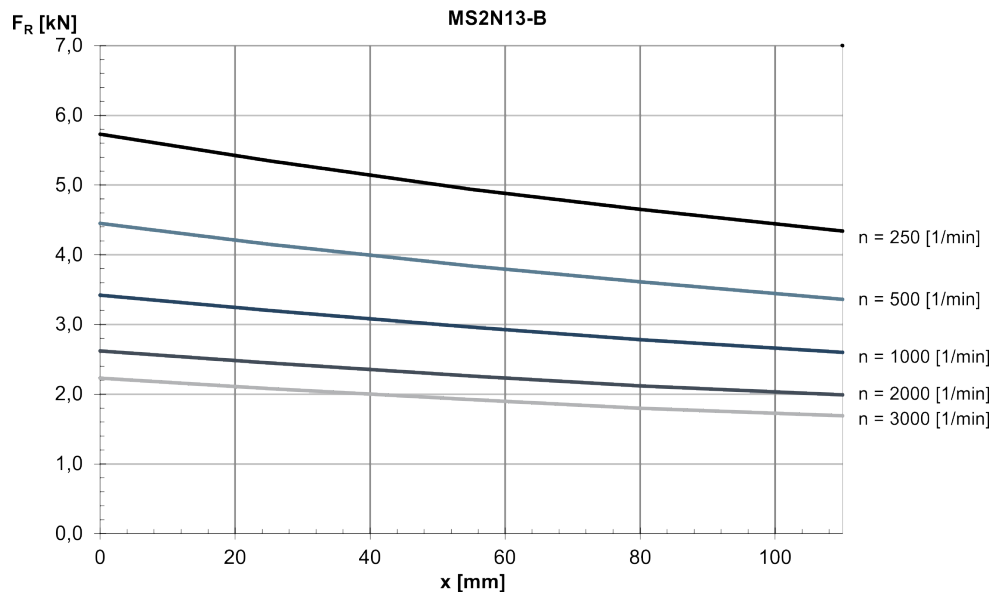
Fig. 354: MS2N13-B: Radial force in distance x from the shaft shoulder at a nominal bearing service life of L_{h10} = 30000 h
