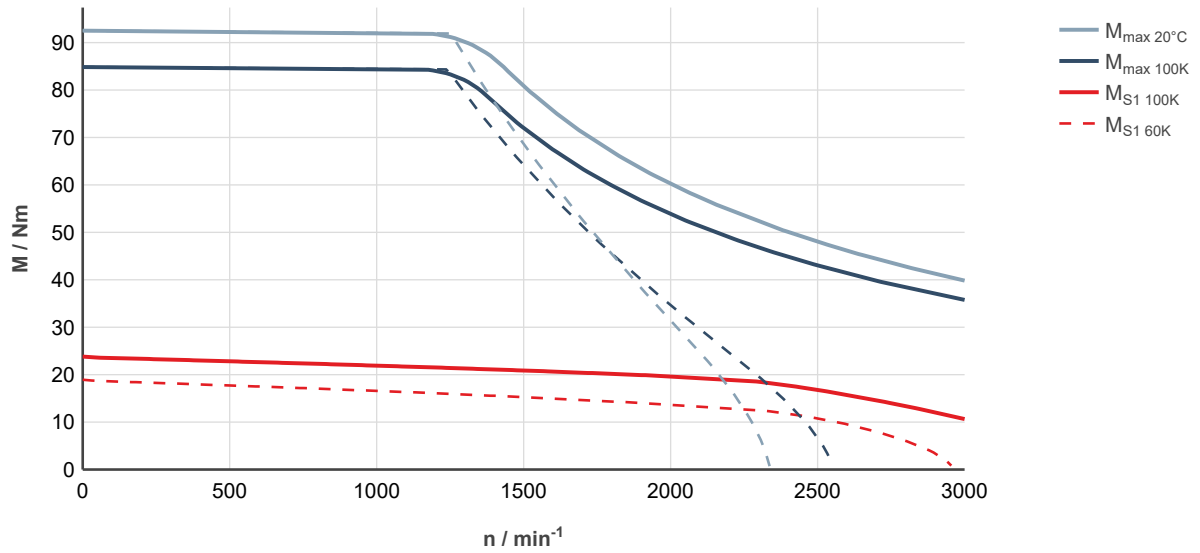
Fig. 109: MS2N07-D1BFN-___0-___-__, ctrlX DRIVE, controlled supply 3 × AC 400 ... 480 V
