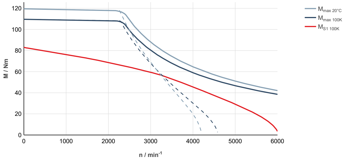
Fig. 181: MS2N07-E0BNL-___0-___-___, ctrlX DRIVE, controlled supply 3 × AC 400 ... 480 V
