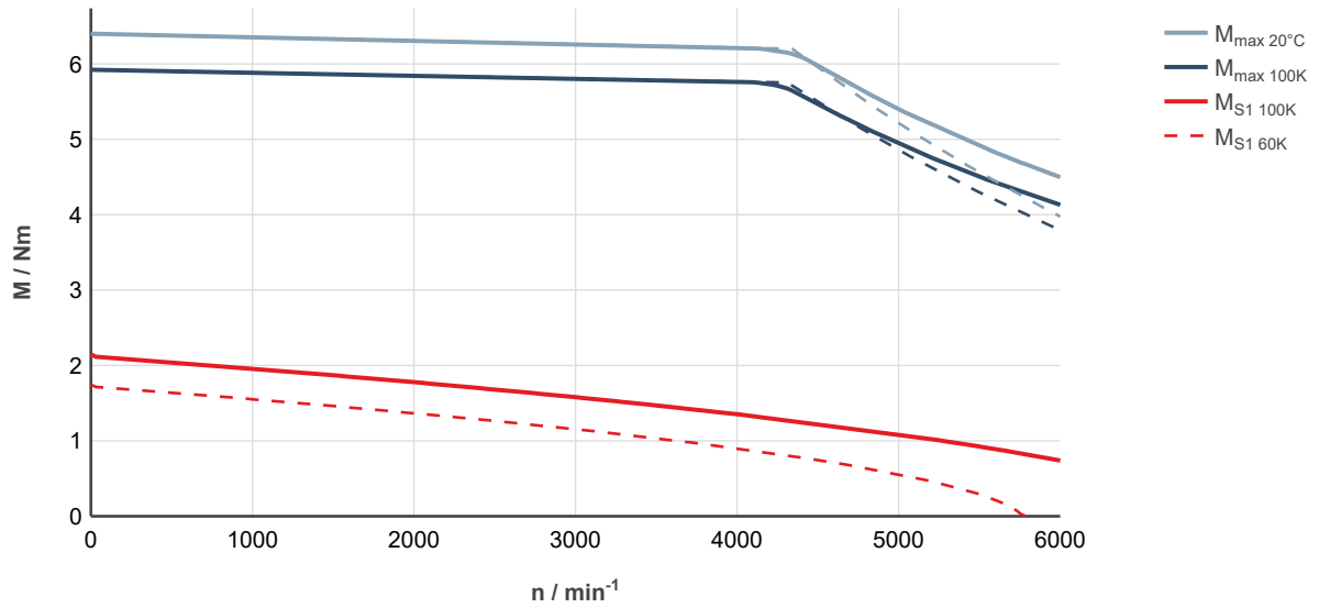
Fig. 38: MS2N04-B0BTN-___0-___-_, ctrlX DRIVE, controlled supply 3 × AC 400 ... 480 V
