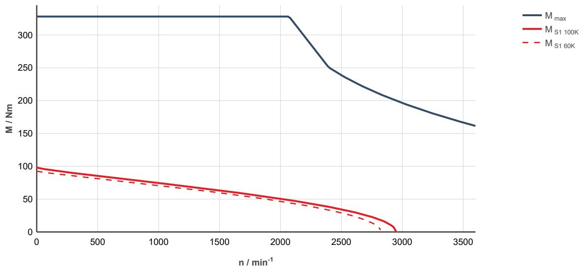
Fig. 304: MS2N13-B1BHN-___0-___-__ (modified), ctrlX DRIVE, controlled supply 3 x AC 400 br ... 480 V M max : Characteristic curve applies to maximum torque 20 °C (cold)
