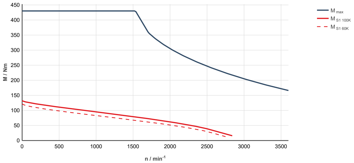
Fig. 307: MS2N13-C1BHN-___0-___-_, ctrIX DRIVE, uncontrolled supply 3 × AC 400 V M_{max} : Characteristic curve applies to maximum torque 20 °C (cold)
