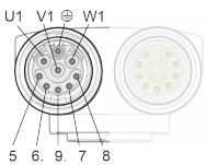
Fig. 375: Connector view double plug M17 power
