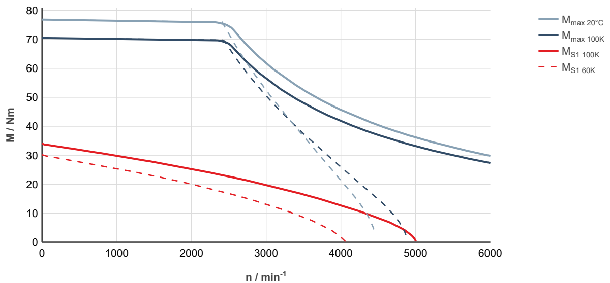
Fig. 198: MS2N10-C0BNN-___0-___-_, ctrlX DRIVE, controlled supply 3 × AC 400 ... 480 V
