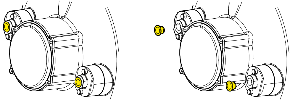
Fig. 397: Protective plug MS2N13 water cooling
