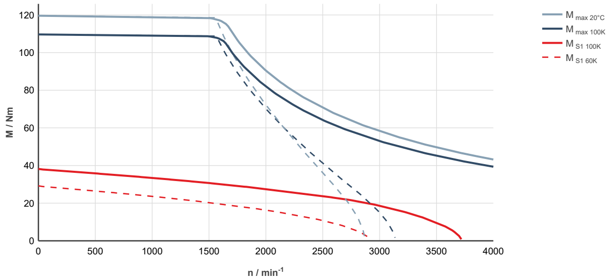
Fig. 117: MS2N07-E0BHN-___0-___-_, ctrlX DRIVE, controlled supply 3 × AC 400 ... 480 V
