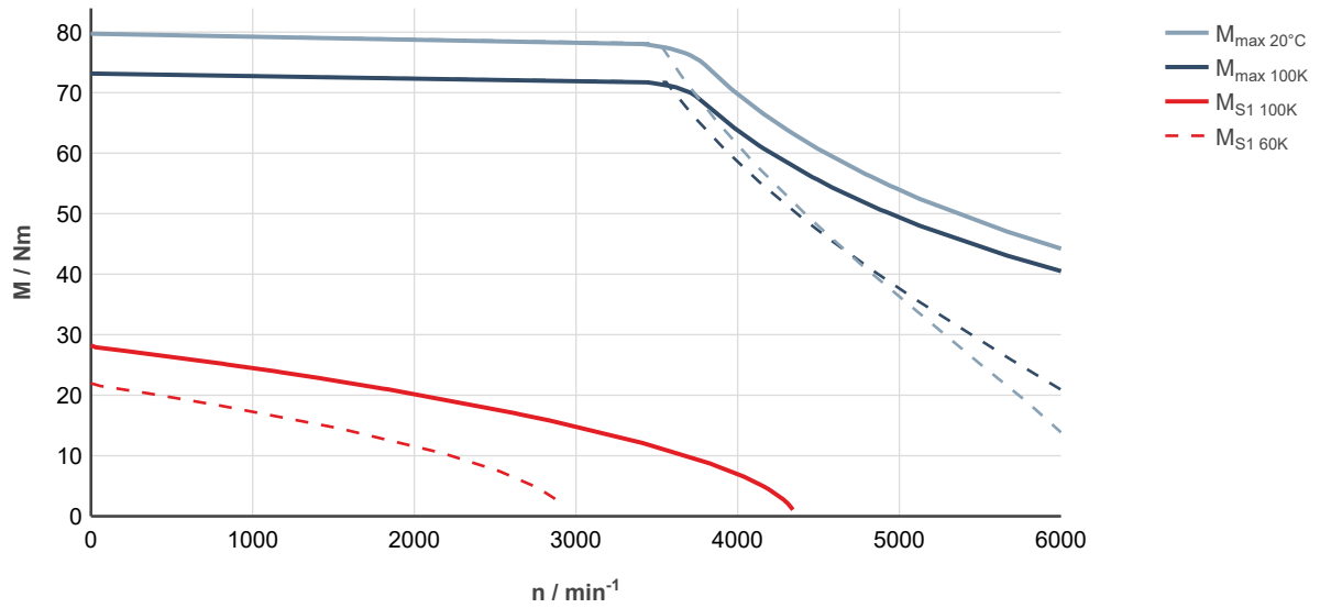
Fig. 107: MS2N07-D0BRN-___0-___-_, ctrlX DRIVE, controlled supply 3 × AC 400 ... 480 V
