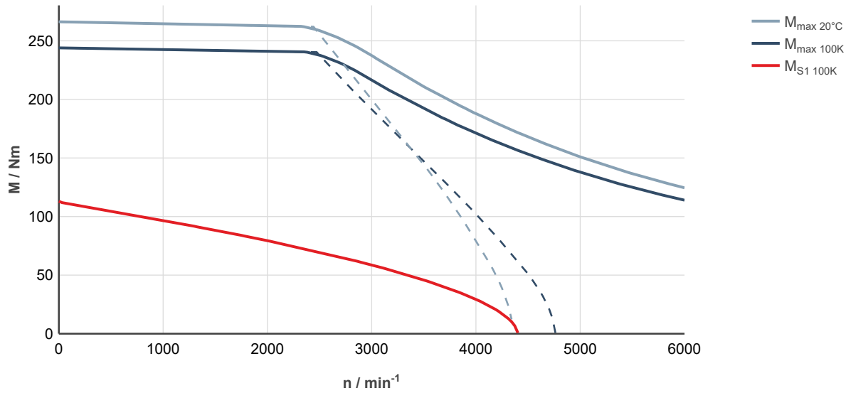
Fig. 252: MS2N10-E1BNA-___0-___-__, ctrlX DRIVE, controlled supply 3 × AC 400 ... 480 V
