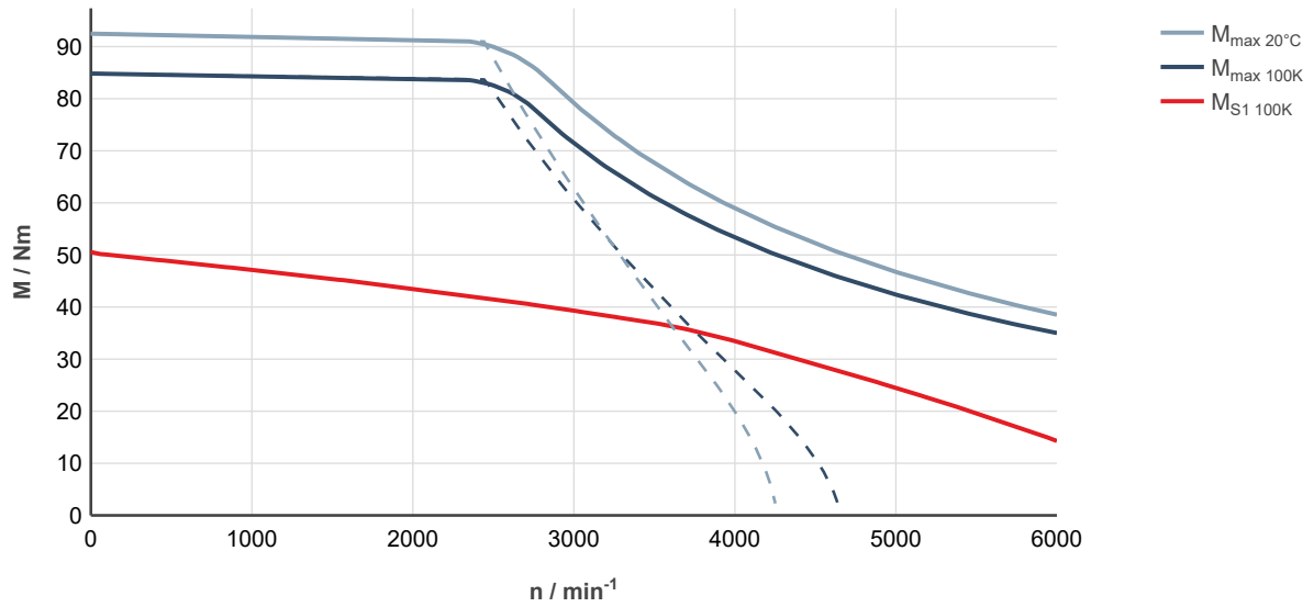
Fig. 177: MS2N07-D1BNL-___0-___-___, ctrlX DRIVE, controlled supply 3 × AC 400 ... 480 V
