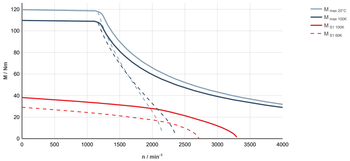
Fig. 116: MS2N07-E0BHN-___0-___-_, ctrlX DRIVE, uncontrolled supply 3 × AC 400 V
