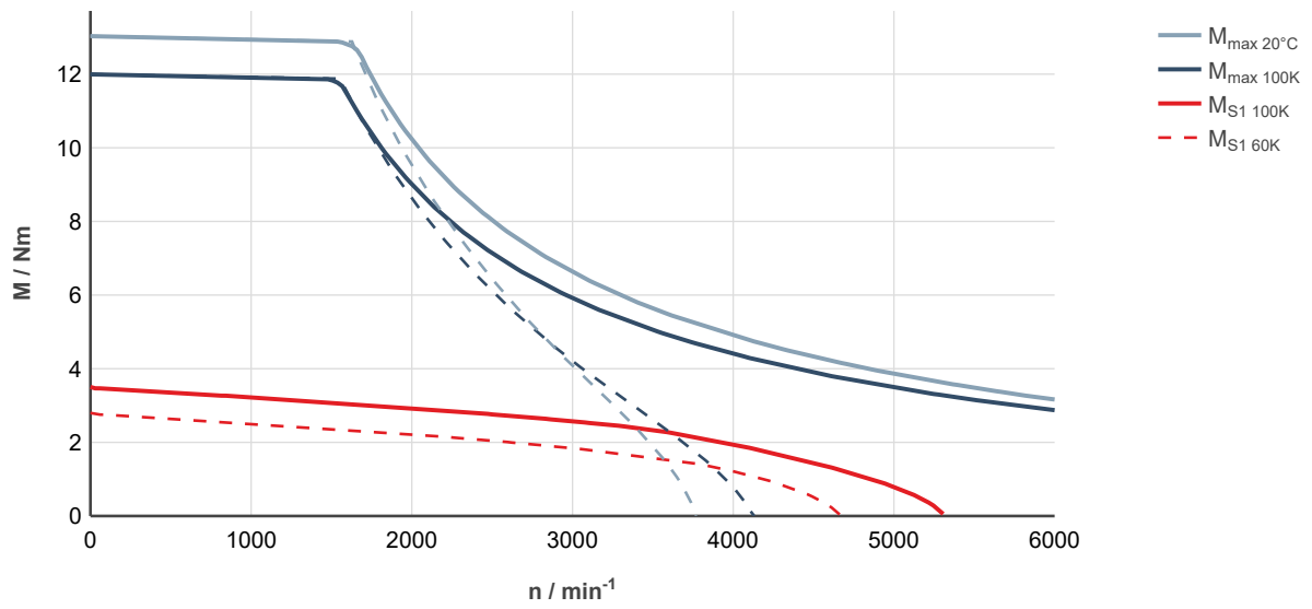
Fig. 39: MS2N04-C0BNN-___0-___-__, ctrlX DRIVE, uncontrolled supply 3 × AC 400 V
