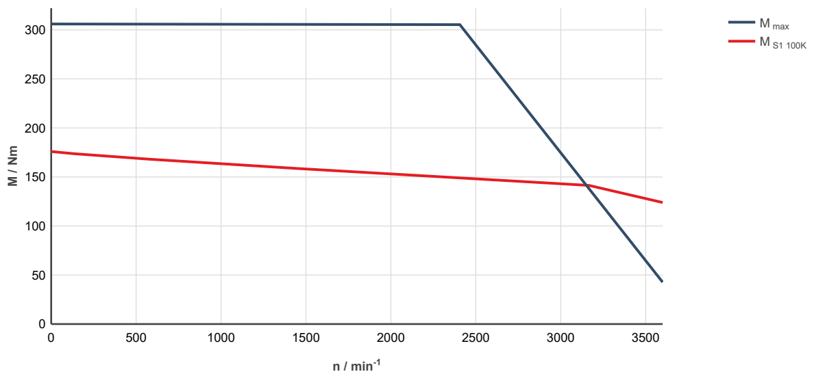
Fig. 337: MS2N13-B1BNL-___0-___-__, ctrlX DRIVE, uncontrolled supply 3 × AC 400 V M_{\text{max}} : Characteristic curve applies to maximum torque 20 °C (cold)
