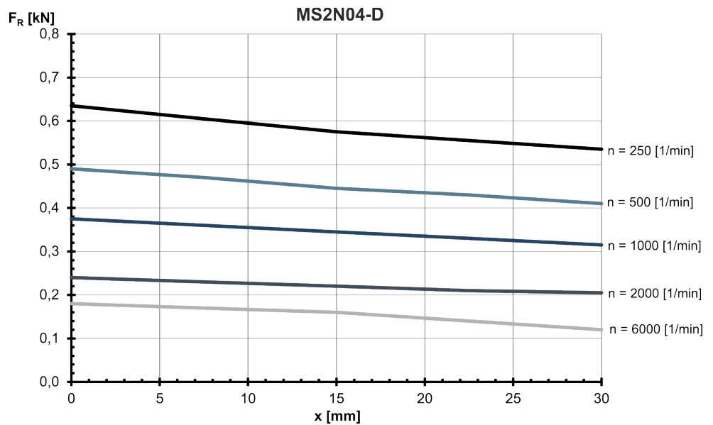
Fig. 51: MS2N04-D: Radial force in distance x from the shaft shoulder at a nominal bearing service life of L_{h10} = 30000 h
