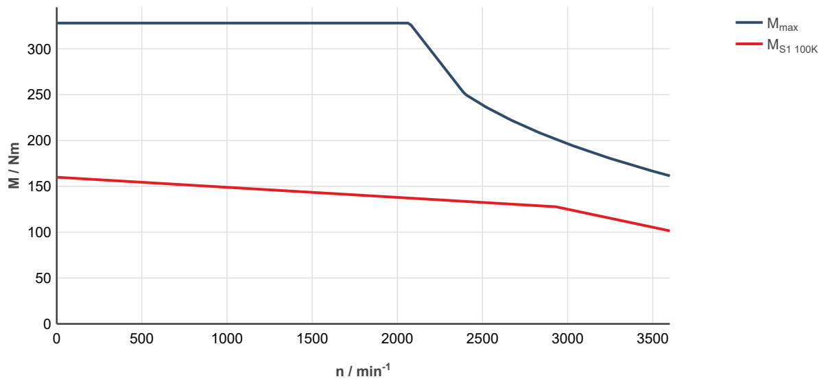
Fig. 320: MS2N13-B1BHC-___0-___-__, ctrlX DRIVE, controlled supply 3 × AC 400 ... 480 V M_max Characteristic curve applies to maximum torque 20 °C (cold)
