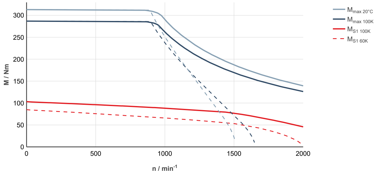
Fig. 220: MS2N10-F0BDN-___0-___-_, ctrlX DRIVE, controlled supply 3 × AC 400 ... 480 V
