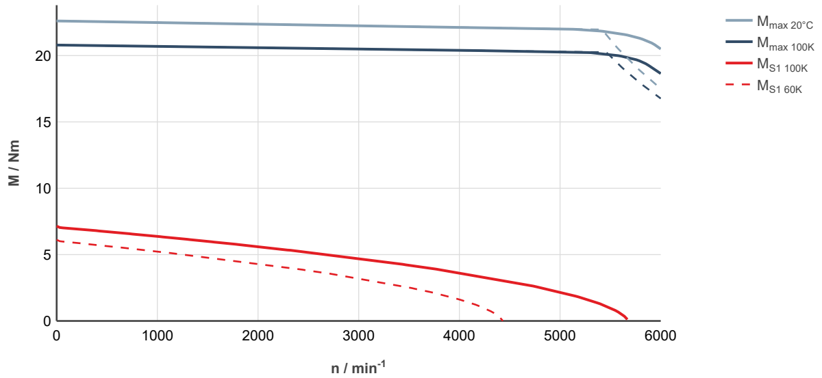
Fig. 59: MS2N05-C0BTN-___0-___-__, ctrlX DRIVE, controlled supply 3 × AC 400 ... 480 V
