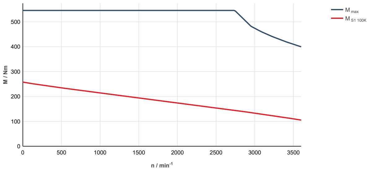
Fig. 330: MS2N13-D1BNC-___0-___-_, ctrlX DRIVE, controlled supply 3 x AC 400 ... 480 V M_{\text{max}} : Characteristic curve applies to maximum torque 20 °C (cold)
