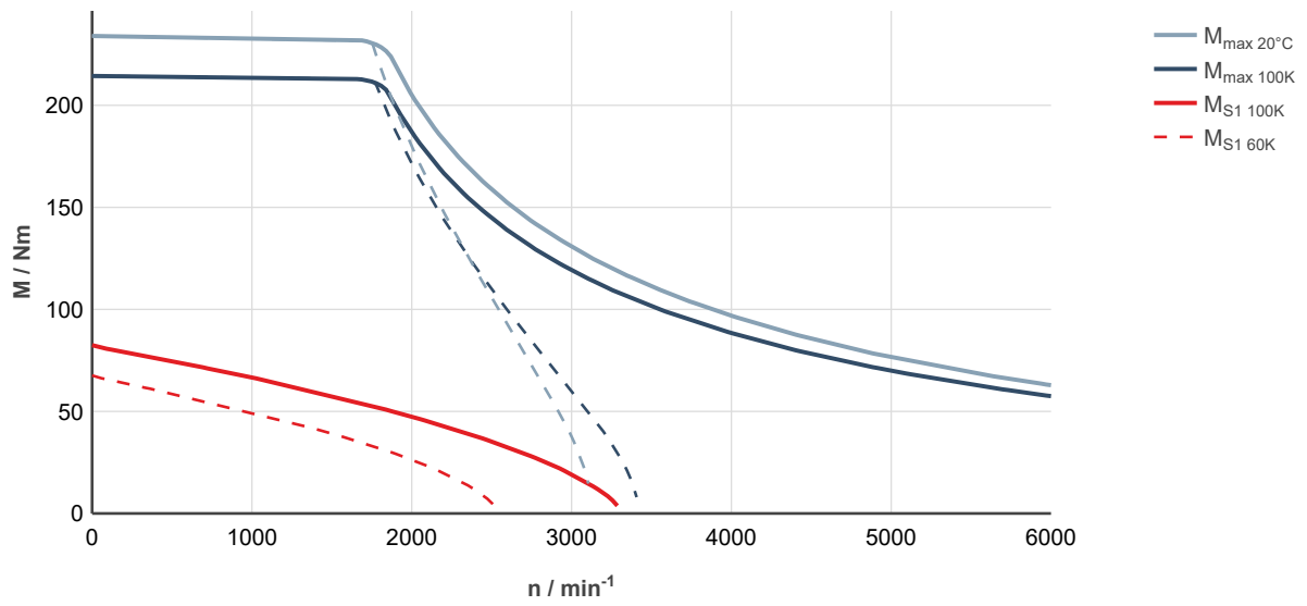
Fig. 213: MS2N10-E0BNN-___0-___-_, ctrlX DRIVE, uncontrolled supply 3 × AC 400 V
