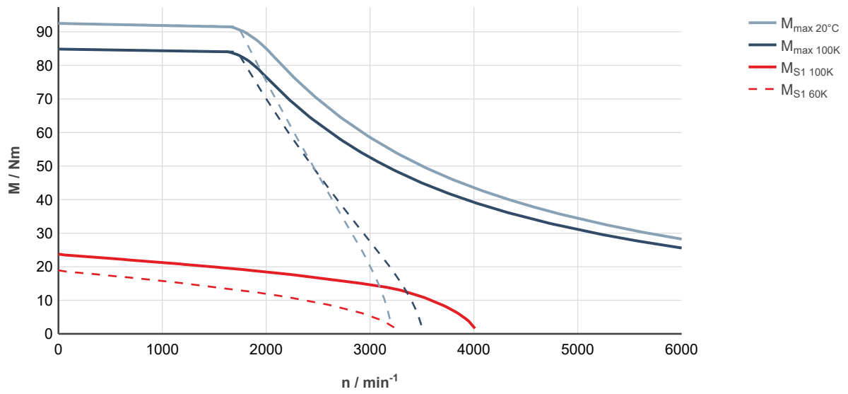
Fig. 112: MS2N07-D1BNN-___0-___-, ctrlX DRIVE, uncontrolled supply 3 × AC 400 V
