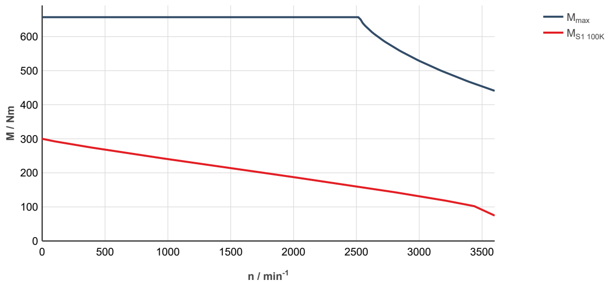
Fig. 334: MS2N13-E1BNC-___0-___-__, ctrlX DRIVE, controlled supply 3 x AC 400 ... 480 V M_{\text{max}} Characteristic curve applies to maximum torque 20 °C (cold)
