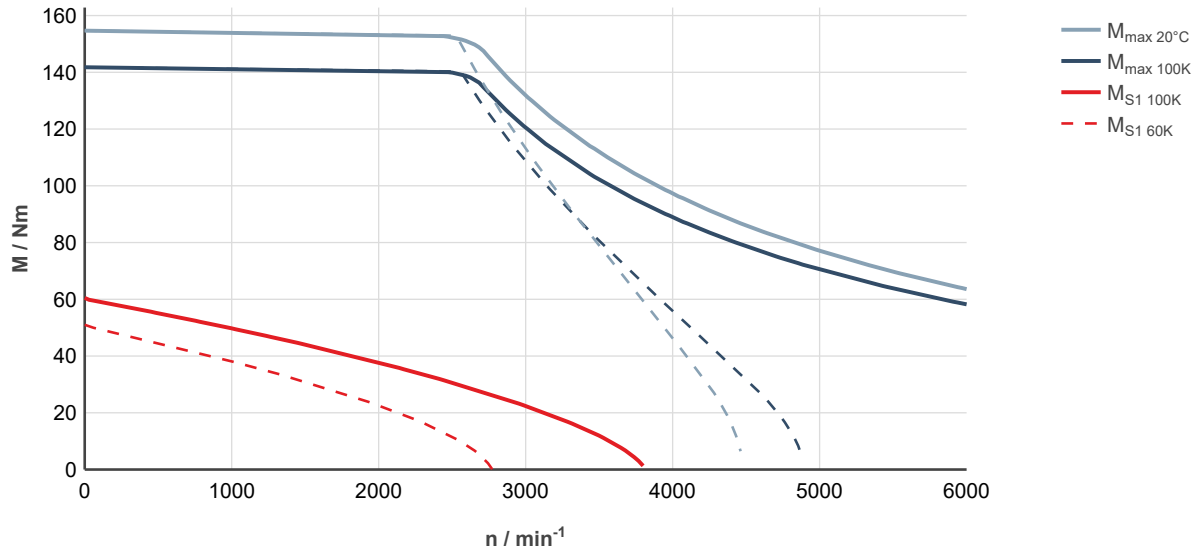
Fig. 206: MS2N10-D0BNN-___0-___-, ctrlX DRIVE, controlled supply 3 × AC 400 ... 480 V
