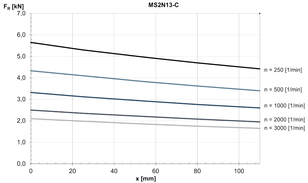
Fig. 355: MS2N13-C: Radial force in distance x from the shaft shoulder at a nominal bearing service life of L_{h10} = 30000 h
