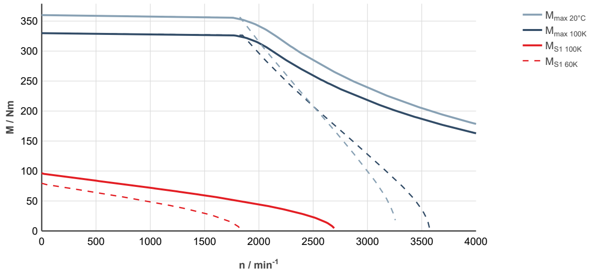
Fig. 226: MS2N10-F1BHN-___0-___-__, ctrlX DRIVE, controlled supply 3 × AC 400 ... 480 V
