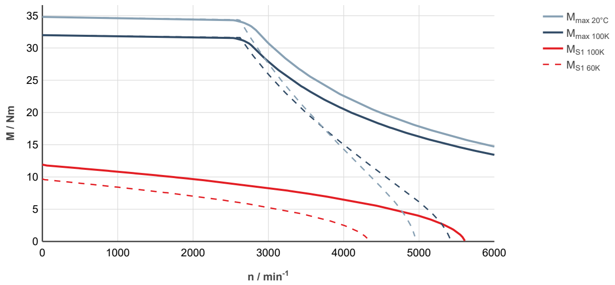
Fig. 77: MS2N06-D0BRN-___0-___-___, ctrlX DRIVE, uncontrolled supply 3 × AC 400 V
