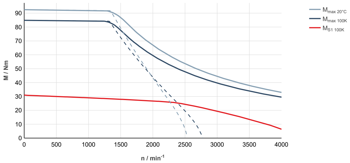
Fig. 146: MS2N07-D1BHA-___0-___-_, ctrlX DRIVE, uncontrolled supply 3 × AC 400 V
