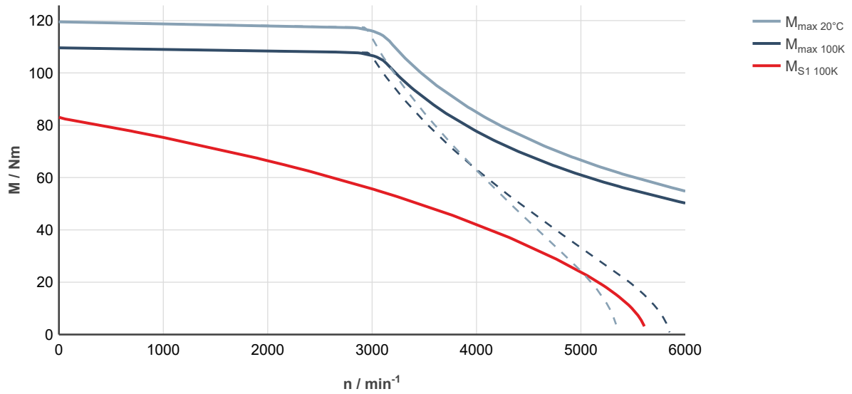
Fig. 183: MS2N07-E0BQL-___0-___-___, ctrIX DRIVE, controlled supply 3 × AC 400 ... 480 V
