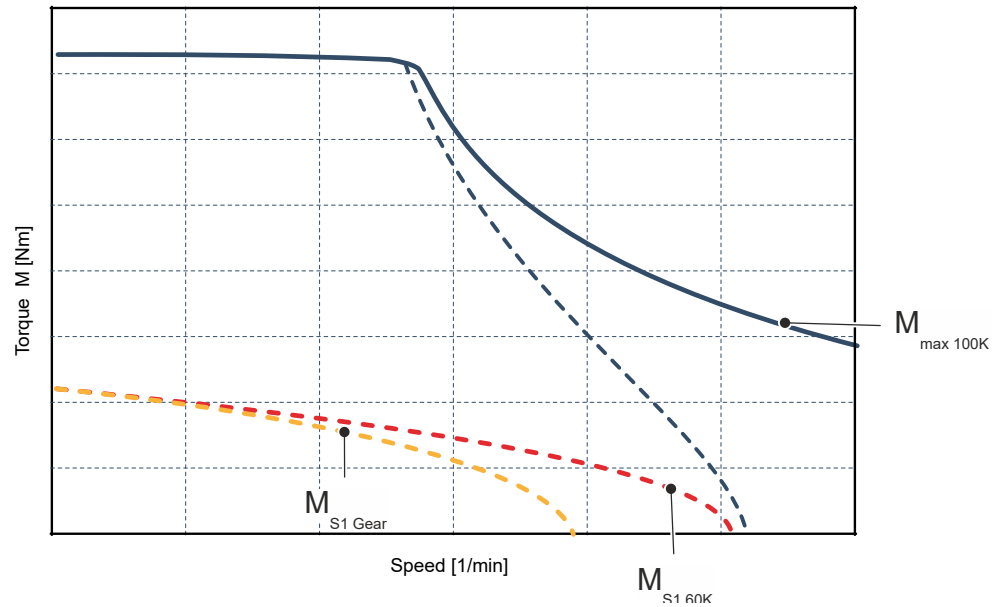
Fig. 23: S1 characteristic curve in gearbox
