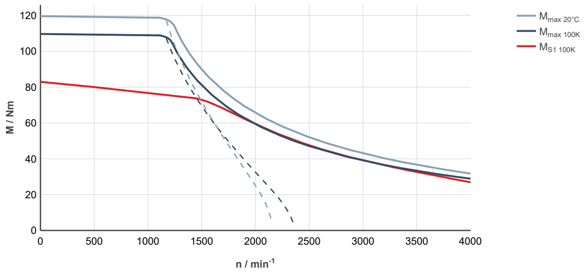
Fig. 178: MS2N07-E0BHL-___0-___-___, ctrIX DRIVE, uncontrolled supply 3 × AC 400 V
