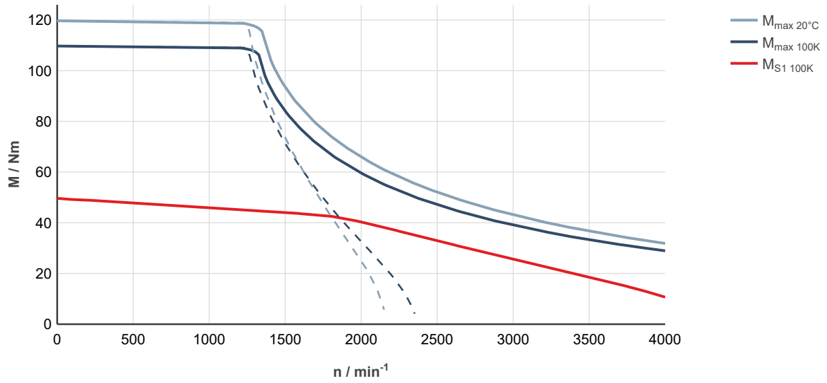
Fig. 152: MS2N07-E0BHA-___0-___-__, ctrlX DRIVE, uncontrolled supply 3 × AC 400 V
