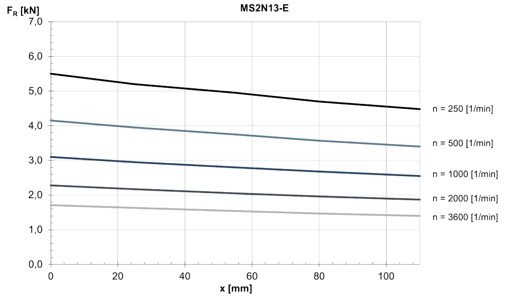
Fig. 357: MS2N13-E: Radial force in distance x from the shaft shoulder at a nominal bearing service life of L_{h10} = 30000 h
