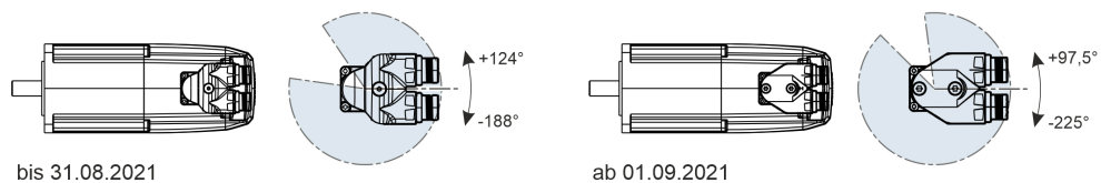
Fig. 376: Rotating area electrical connection "D"
