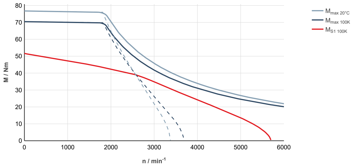
Fig. 265: MS2N10-C0BNL-___0-___-___, ctrlX DRIVE, uncontrolled supply 3 × AC 400 V
