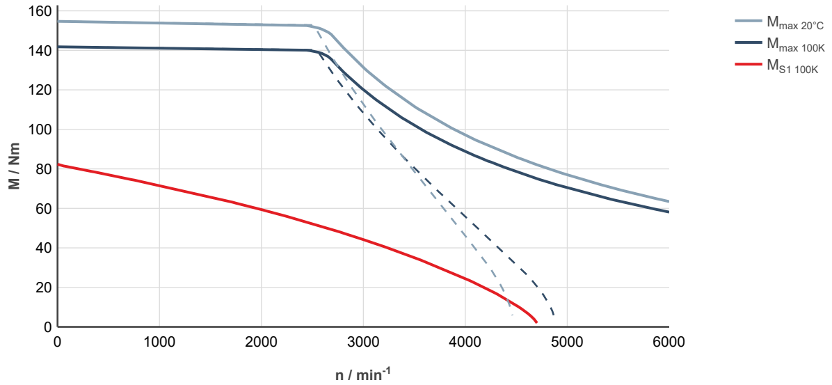
Fig. 240: MS2N10-D0BNA-___0-___-_, ctrlX DRIVE, controlled supply 3 × AC 400 ... 480 V
