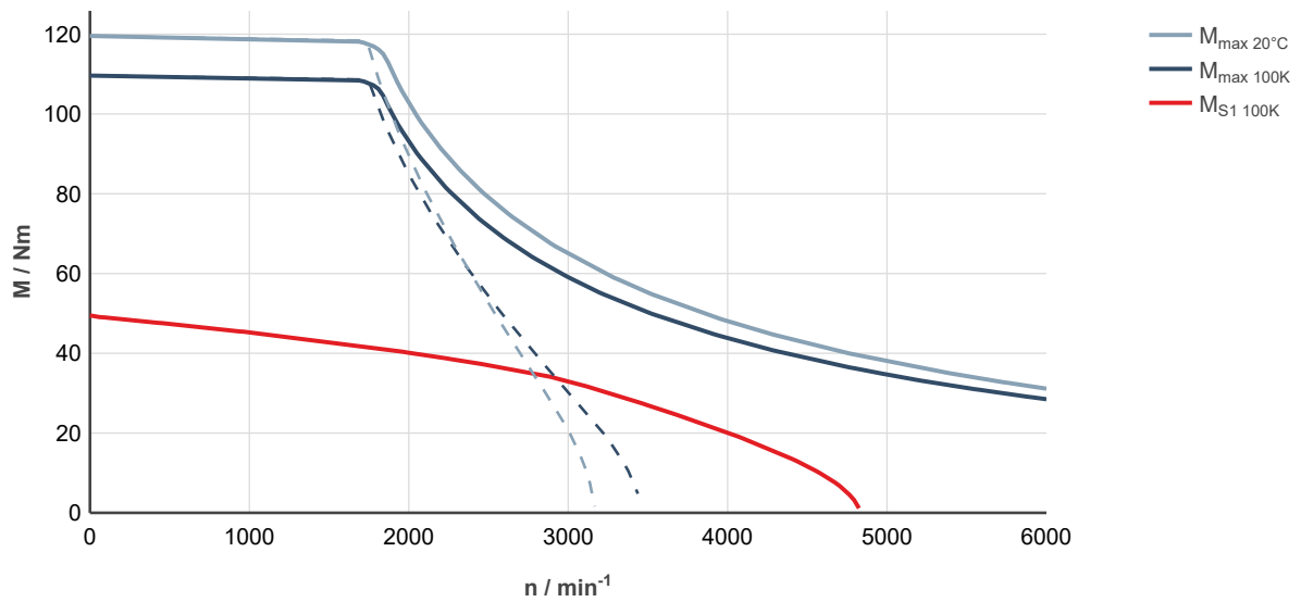
Fig. 154: MS2N07-E0BNA-___0-___-_, ctrlX DRIVE, uncontrolled supply 3 × AC 400 V
