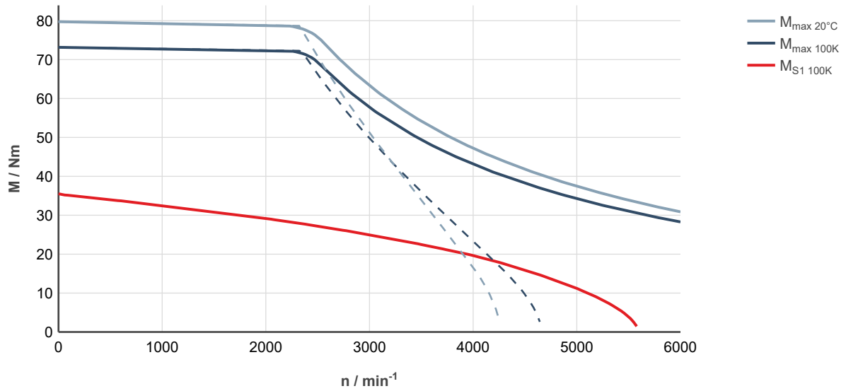
Fig. 141: MS2N07-D0BNA-___0-___-_, ctrlX DRIVE, controlled supply 3 × AC 400 ... 480 V
