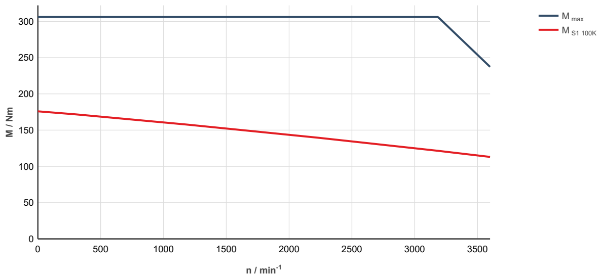
Fig. 338: MS2N13-B1BNL-___0-___-__, ctrlX DRIVE, controlled supply 3 x AC 400 ... 480 V M_{\text{max}} : Characteristic curve applies to maximum torque 20 °C (cold)
