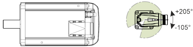
Fig. 370: Rotating area electrical connection "A/B"
