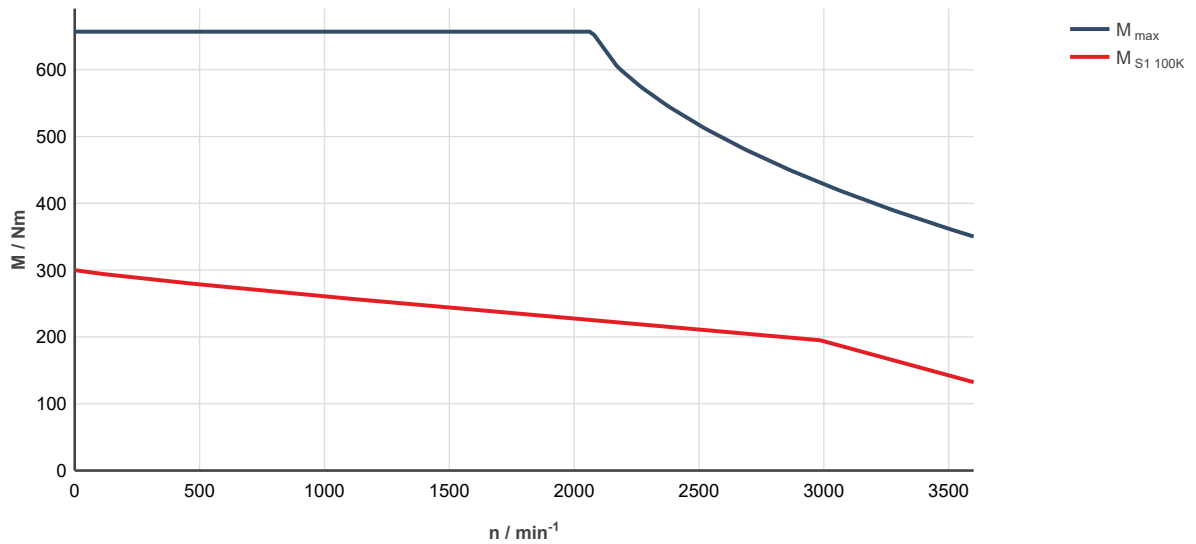
Fig. 332: MS2N13-E1BHC-___0-___-_, ctrIX DRIVE, controlled supply 3 × AC 400 ... 480 V M_{max} Characteristic curve applies to maximum torque 20 °C (cold)
