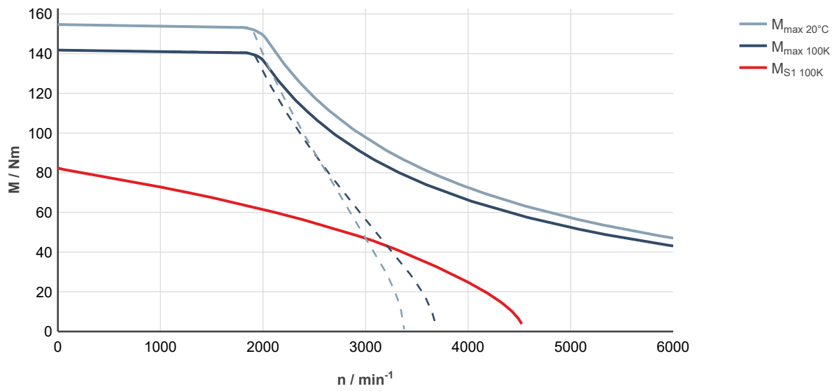
Fig. 239: MS2N10-D0BNA-___0-___-_, ctrlX DRIVE, uncontrolled supply 3 × AC 400 V
