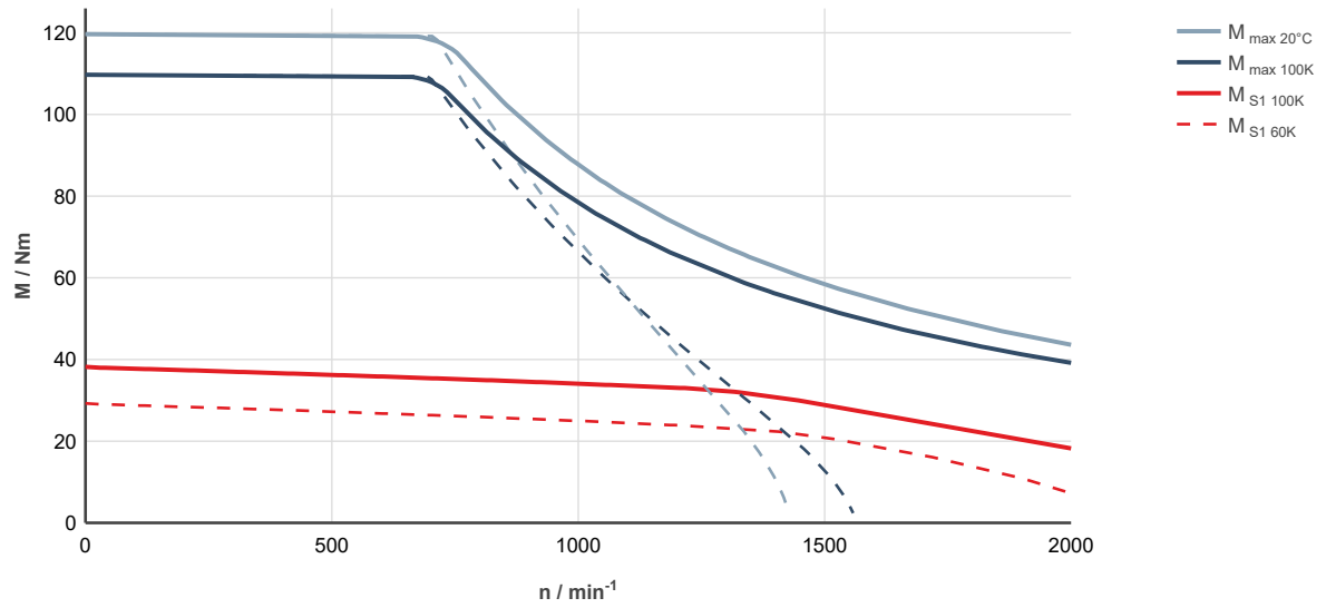
Fig. 115: MS2N07-E0BDN-___0-___-_, ctrlX DRIVE, controlled supply 3 × AC 400 ... 480 V
