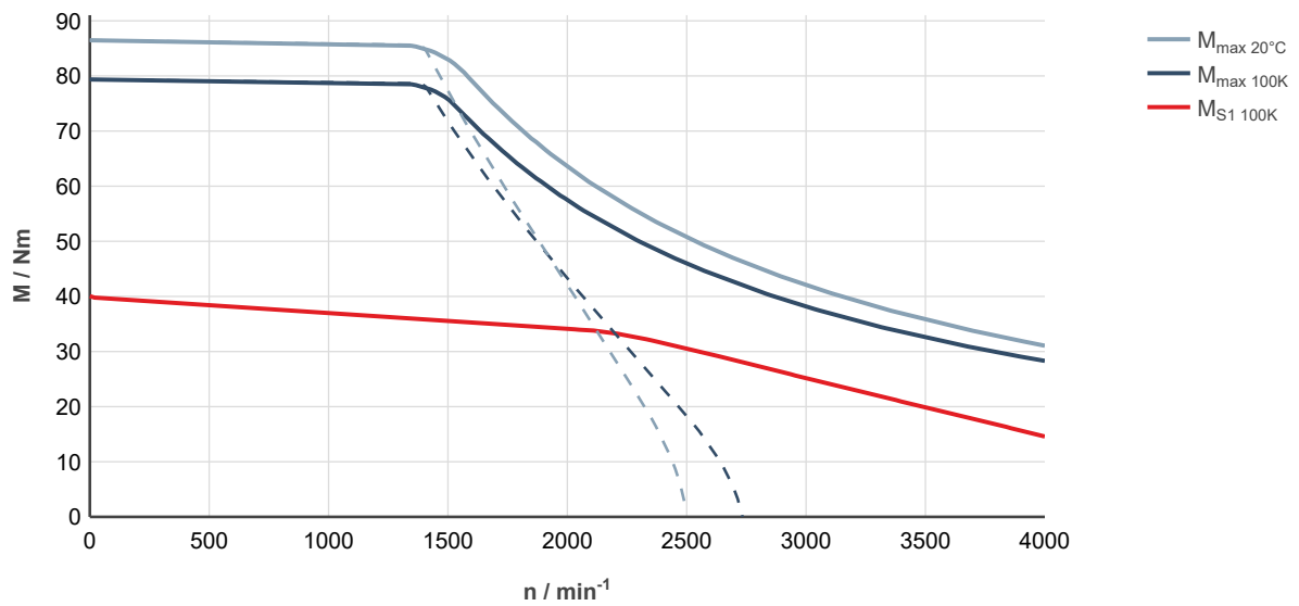
Fig. 233: MS2N10-C1BHA-___0-___-_, ctrlX DRIVE, uncontrolled supply 3 × AC 400 V
