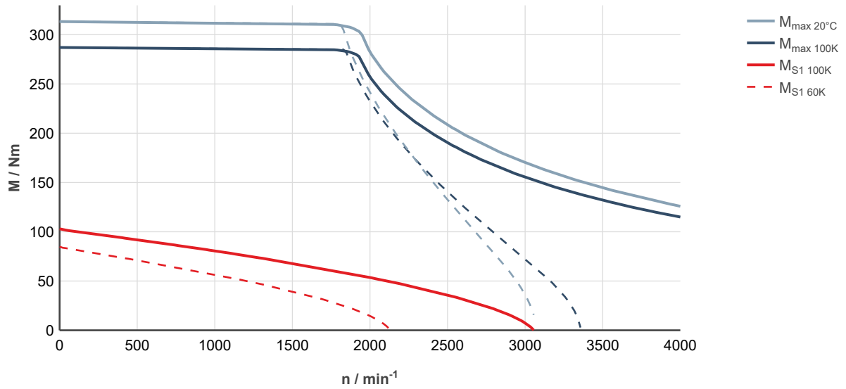
Fig. 222: MS2N10-F0BHN-___0-___-_, ctrlX DRIVE, controlled supply 3 × AC 400 ... 480 V
