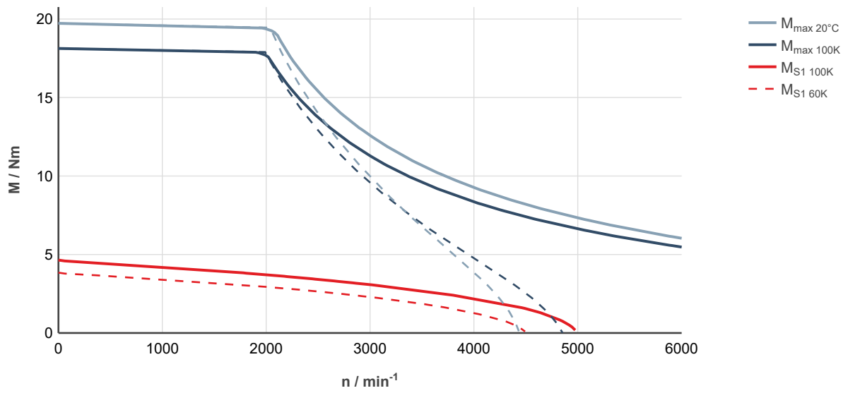
Fig. 45: MS2N04-D0BQN-___0-___-_, ctrlX DRIVE, uncontrolled supply 3 × AC 400 V
