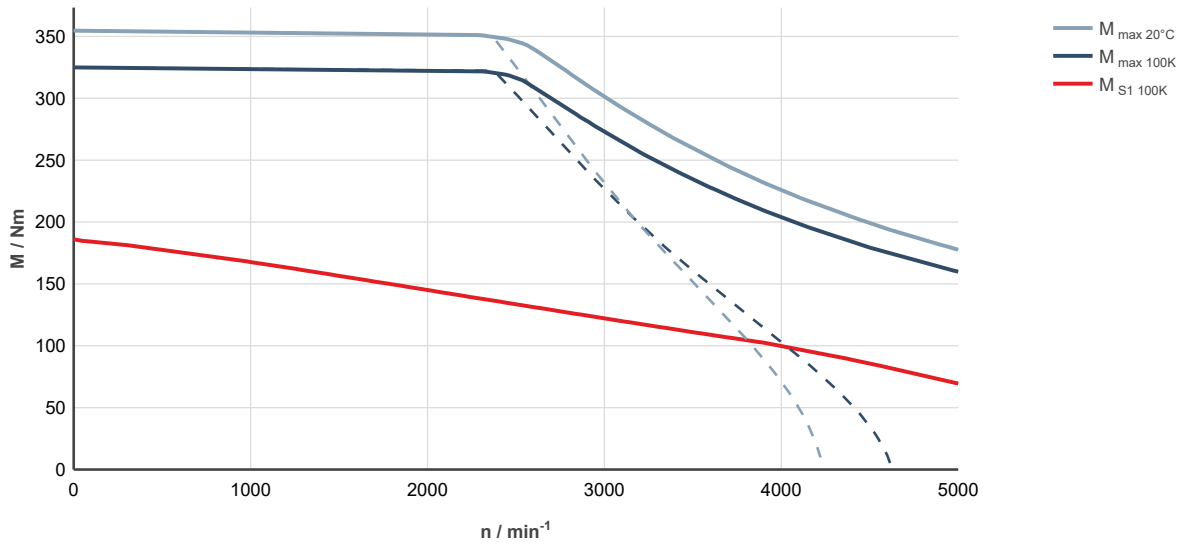
Fig. 288: MS2N10-R0BLL-___0-___-__, ctrlX DRIVE, controlled supply 3 x AC 400 ... 480 V
