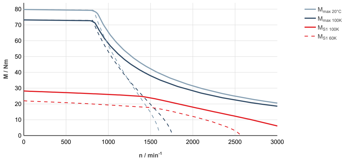
Fig. 100: MS2N07-D0BFN-___0-___-__, ctrlX DRIVE, uncontrolled supply 3 × AC 400 V
