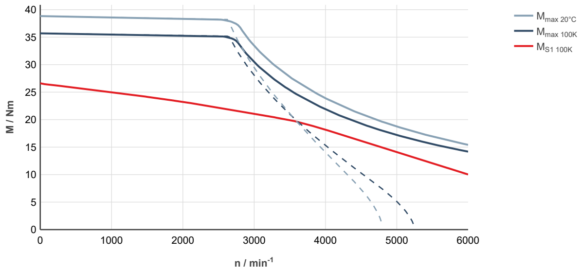
Fig. 166: MS2N07-C0BQL-__0-__-__, ctrlX DRIVE, uncontrolled supply 3 × AC 400 V
