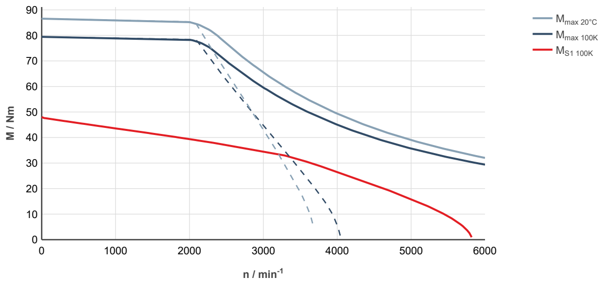
Fig. 267: MS2N10-C1BNL-___0-___-___, ctrIX DRIVE, uncontrolled supply 3 × AC 400 V
