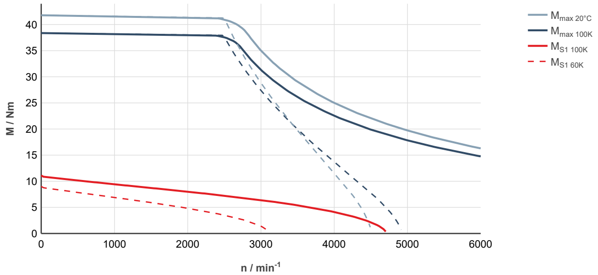
Fig. 80: MS2N06-D1BNN-___0-___-_, ctrlX DRIVE, controlled supply 3 × AC 400 ... 480 V
