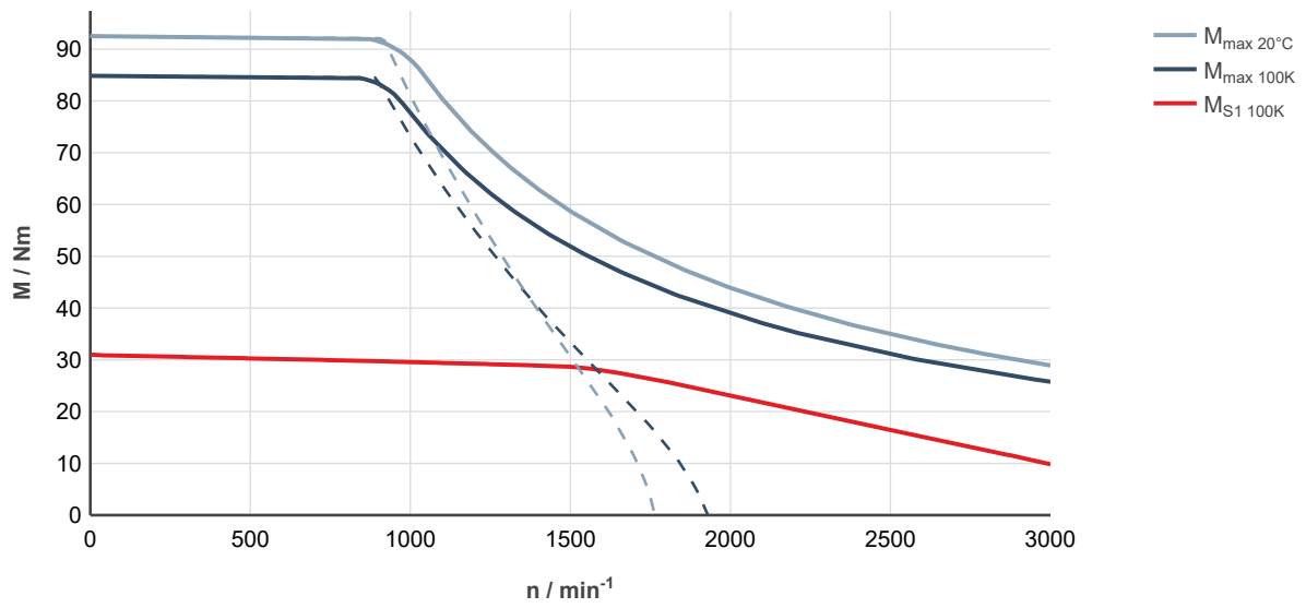
Fig. 144: MS2N07-D1BFA-___0-___-__, ctrlX DRIVE, uncontrolled supply 3 × AC 400 V
