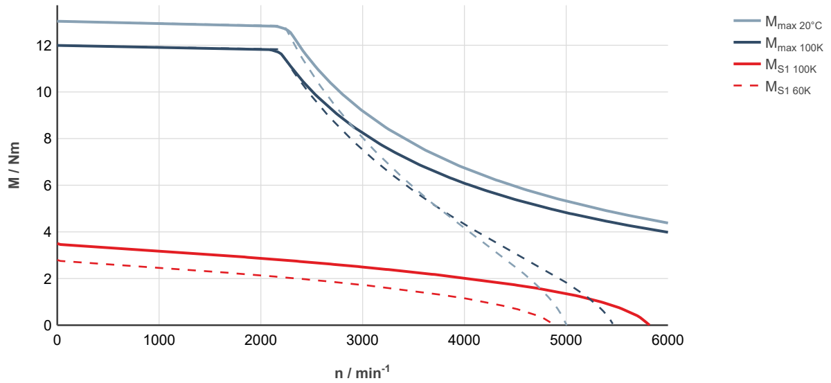
Fig. 40: MS2N04-C0BNN-___0-___-__, ctrlX DRIVE, controlled supply 3 × AC 400 ... 480 V
