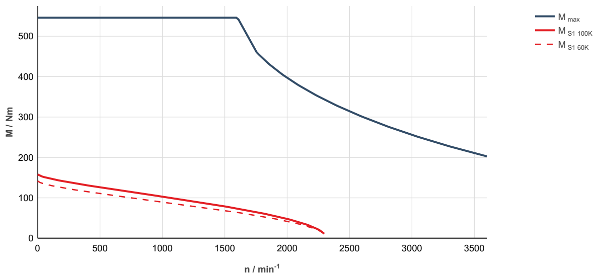
Fig. 311: MS2N13-D1BHN-___0-___-_, ctrIX DRIVE, uncontrolled supply 3 × AC 400 V M_{\max} : Characteristic curve applies to maximum torque 20 °C (cold)
