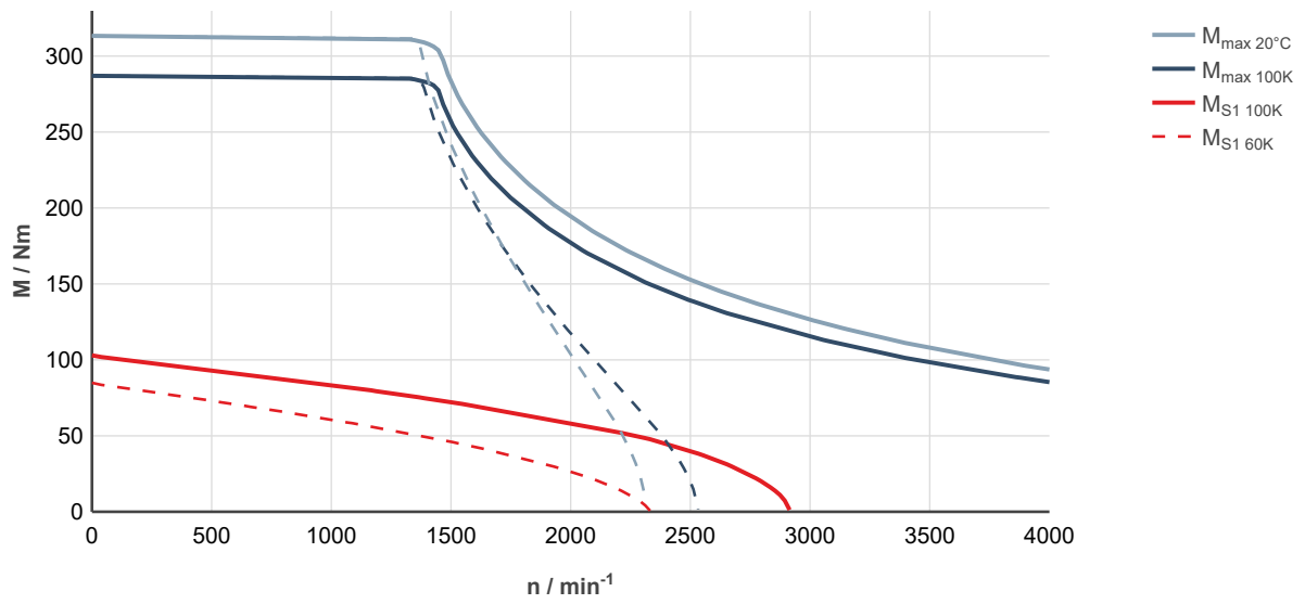
Fig. 221: MS2N10-F0BHN-___0-___-_, ctrlX DRIVE, uncontrolled supply 3 × AC 400 V
