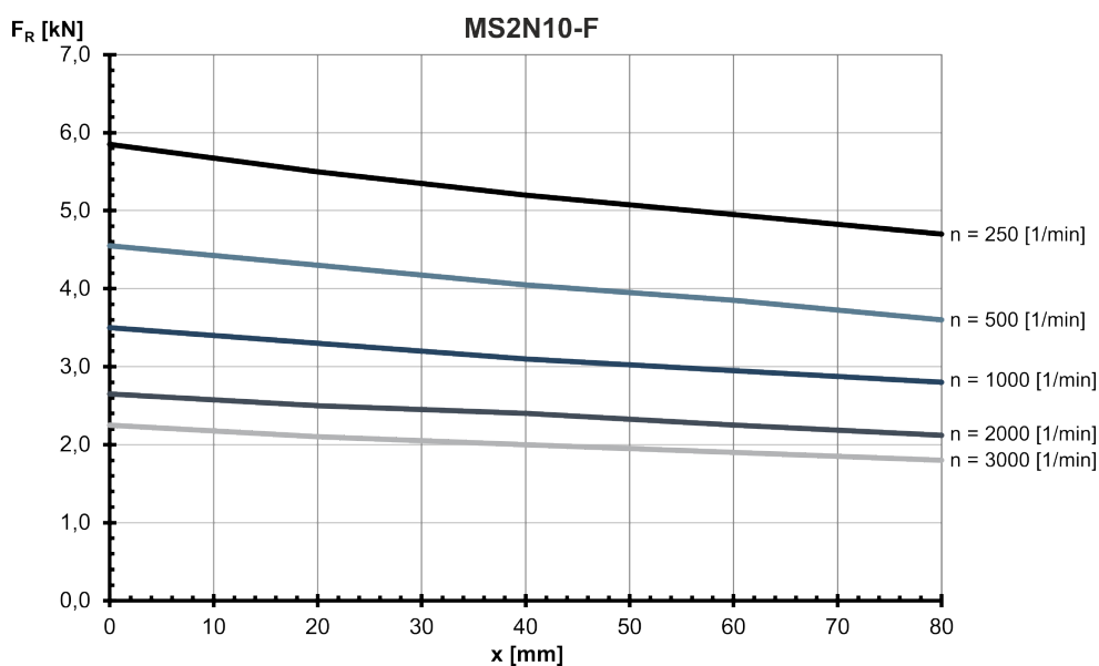
Fig. 301: MS2N10-F: Radial force in distance x from the shaft shoulder at a nominal bearing service life of L_{h10} = 30000 h
