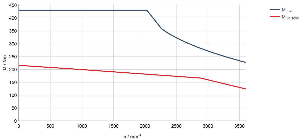
Fig. 324: MS2N13-C1BHC-___0-___-_, ctrIX DRIVE, controlled supply 3 × AC 400 ... 480 V M_{\text{max}} Characteristic curve applies to maximum torque 20 °C (cold)
