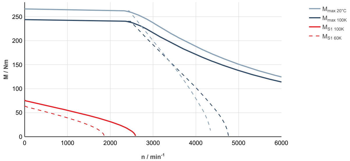
Fig. 218: MS2N10-E1BNN-___0-___-_, ctrlX DRIVE, controlled supply 3 × AC 400 ... 480 V
