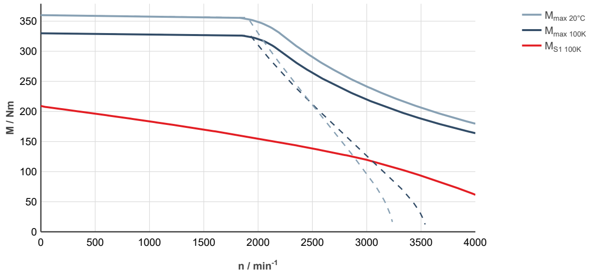
Fig. 286: MS2N10-F1BHL-___0-___-___, ctrlX DRIVE, controlled supply 3 × AC 400 ... 480 V
