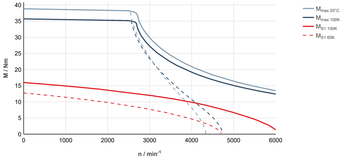
Fig. 93: MS2N07-C0BNN-___0-___-___, ctrlX DRIVE, controlled supply 3 × AC 400 ... 480 V
