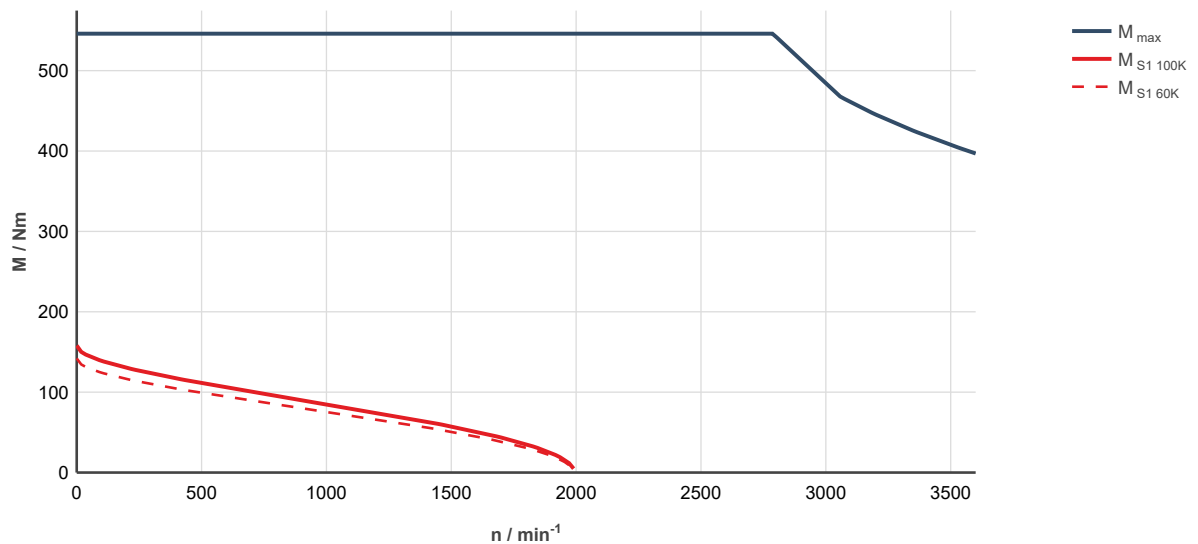
Fig. 314: MS2N13-D1BNN-___0-___-_, ctrlX DRIVE, controlled supply 3 x AC 400 ... 480 V M max : Characteristic curve applies to maximum torque 20 °C (cold)
