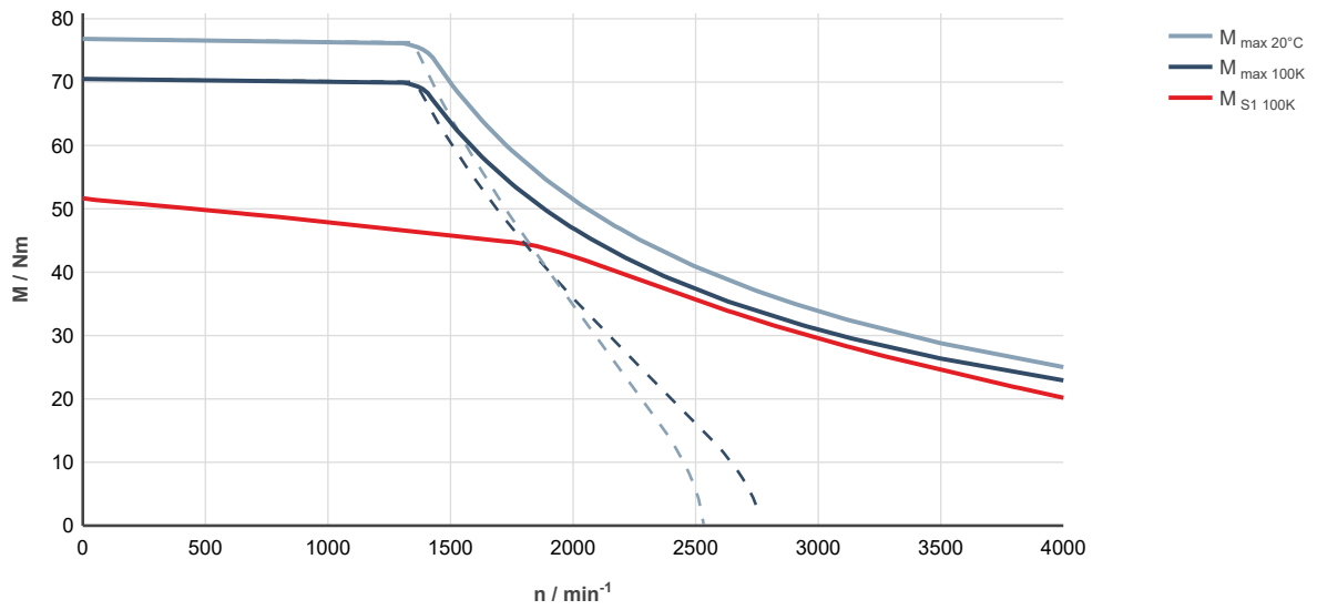
Fig. 263: MS2N10-C0BHL-___0-___-_0, ctrlX DRIVE, uncontrolled supply 3 × AC 400 V
