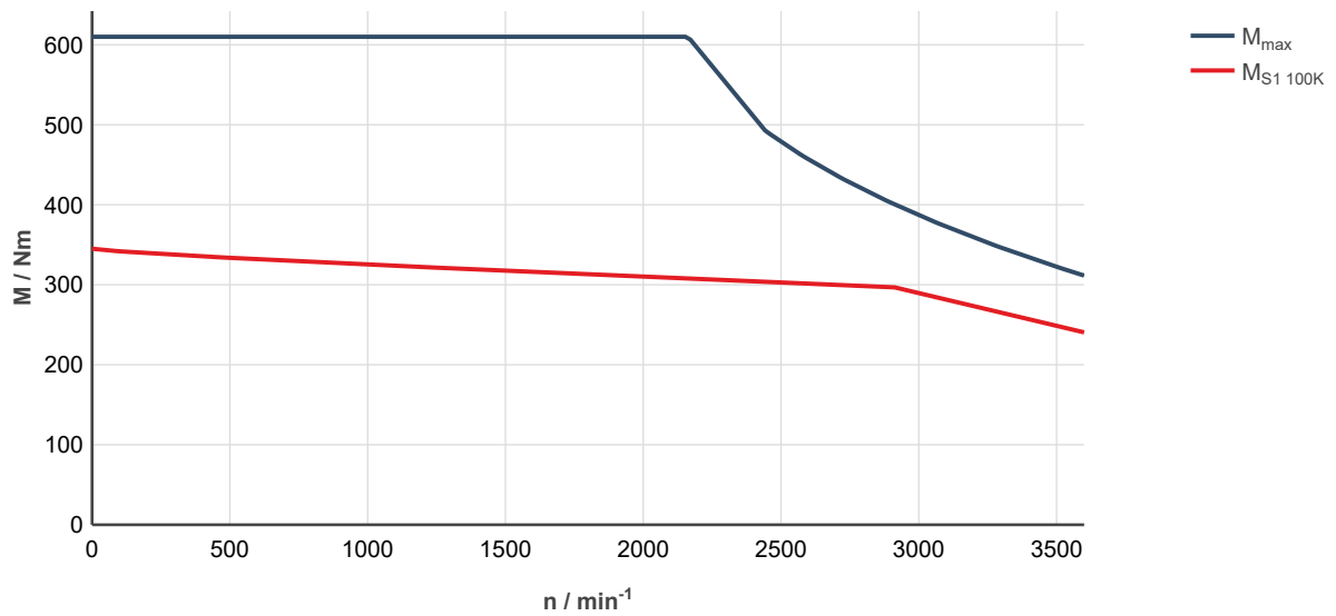
Fig. 349: MS2N13-E1BNL-__0-__-__, ctrlX DRIVE, uncontrolled supply 3 × AC 400 V M_{\text{max}} : Characteristic curve applies to maximum torque 20 °C (cold)
