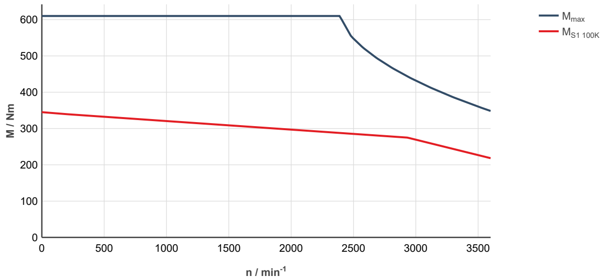
Fig. 348: MS2N13-E1BHL-__0-__-__, ctrlX DRIVE, controlled supply 3 × AC 400 ... 480 V M_{\text{max}} : Characteristic curve applies to maximum torque 20 °C (cold)
