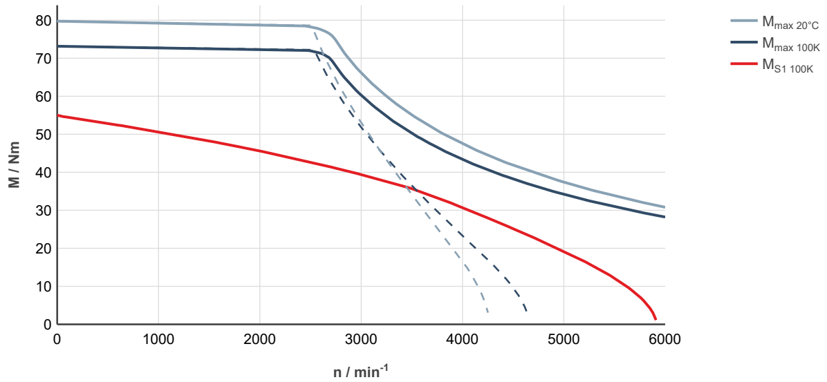
Fig. 173: MS2N07-D0BNL-___0-___-___, ctrIX DRIVE, controlled supply 3 × AC 400 ... 480 V
