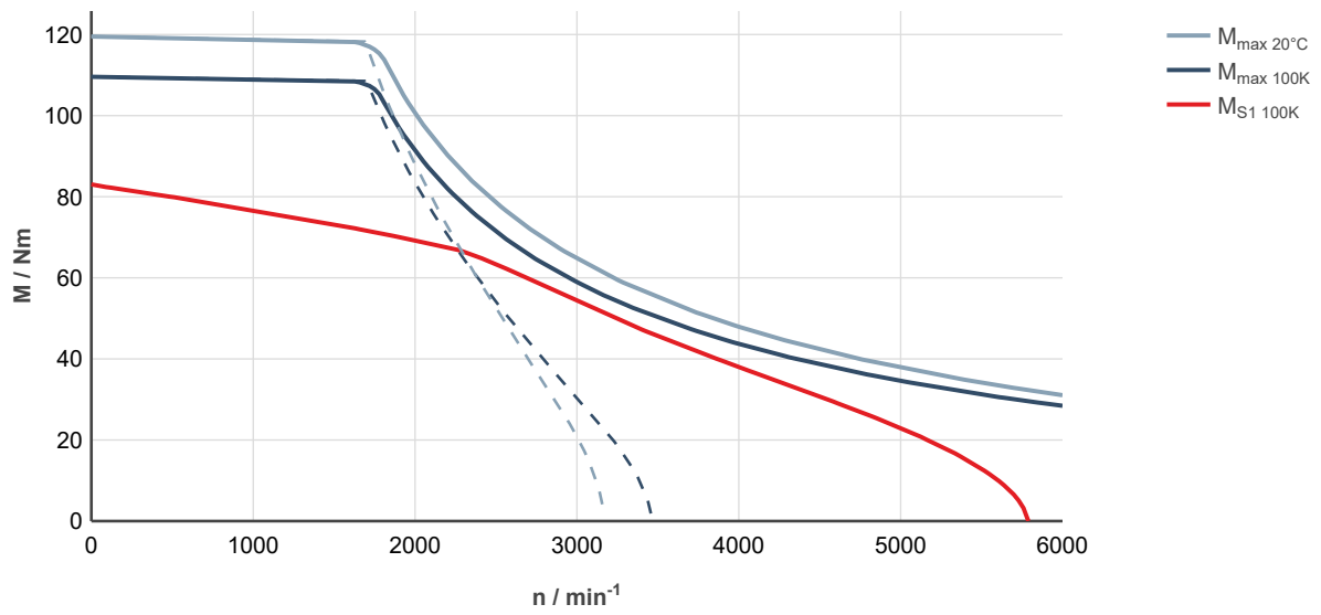
Fig. 180: MS2N07-E0BNL-___0-___-___, ctrlX DRIVE, uncontrolled supply 3 × AC 400 V
