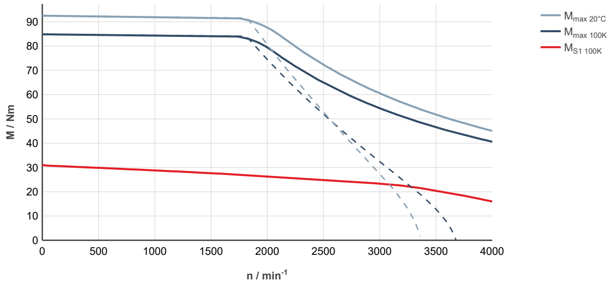
Fig. 147: MS2N07-D1BHA-___0-___-_, ctrlX DRIVE, controlled supply 3 × AC 400 ... 480 V
