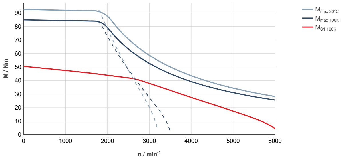
Fig. 176: MS2N07-D1BNL-___0-___-___, ctrlX DRIVE, uncontrolled supply 3 × AC 400 V
