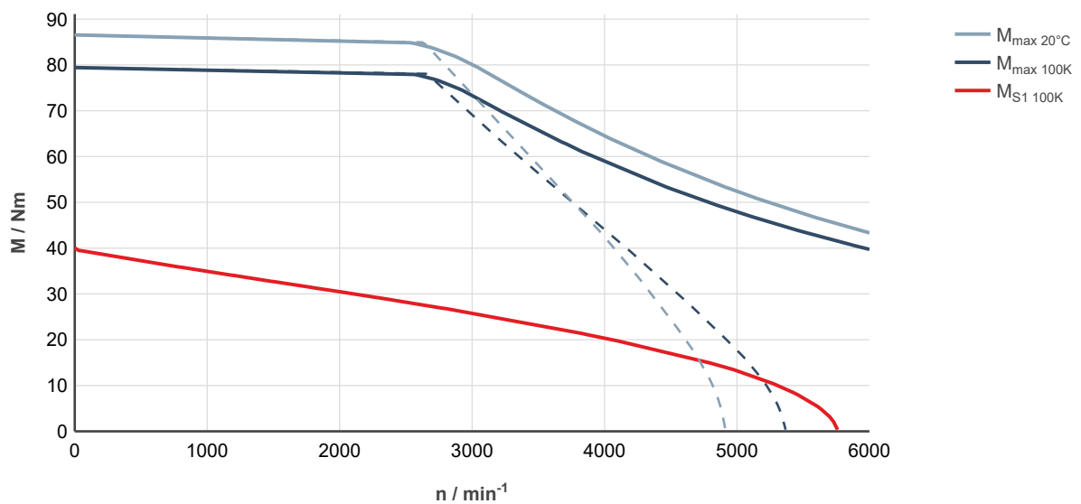
Fig. 236: MS2N10-C1BNA-___0-___-_, ctrlX DRIVE, controlled supply 3 × AC 400 ... 480 V
