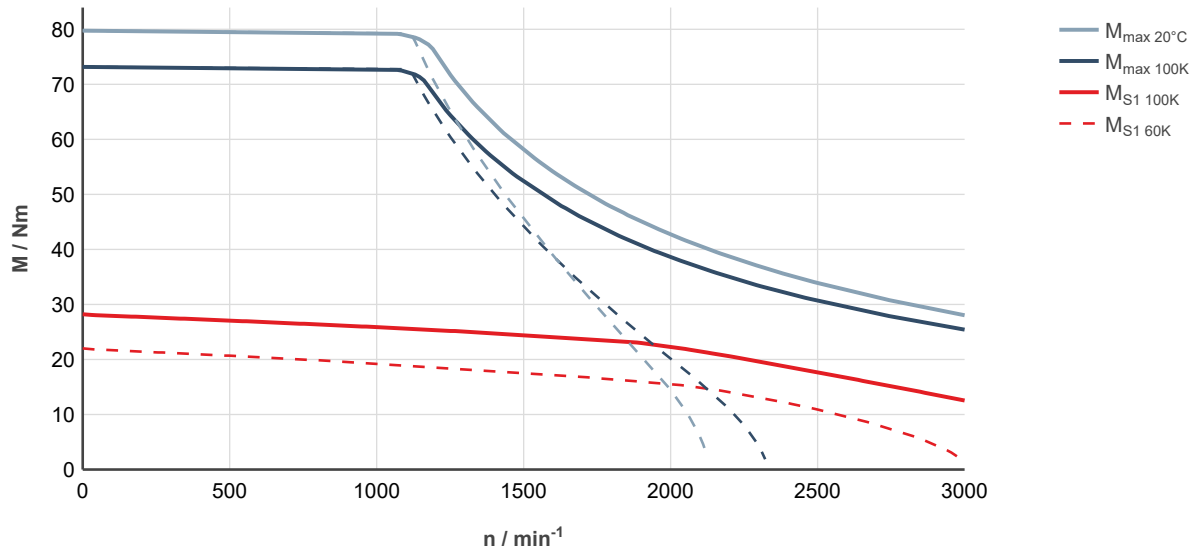
Fig. 101: MS2N07-D0BFN-___0-___-__, ctrlX DRIVE, controlled supply 3 × AC 400 ... 480 V
