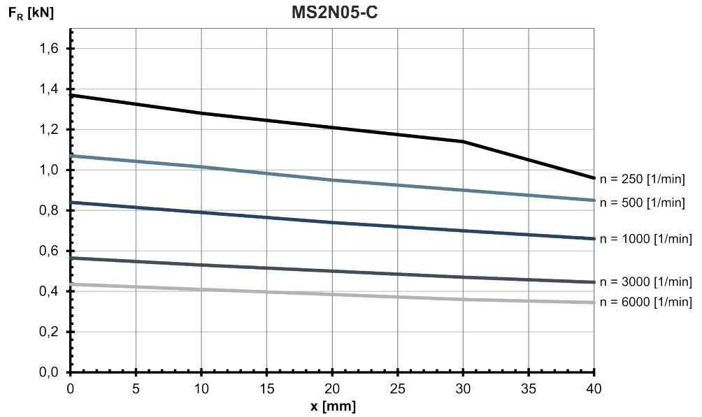
Fig. 67: MS2N05-C: Radial force in distance x from the shaft shoulder at a nominal bearing service life of L_{h10} = 30000 h
