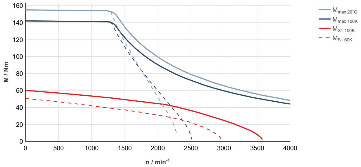
Fig. 203: MS2N10-D0BHN-___0-___-_, ctrlX DRIVE, uncontrolled supply 3 × AC 400 V
