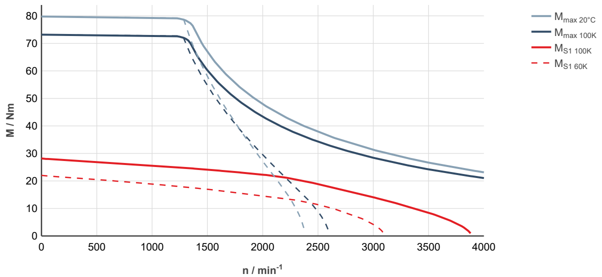
Fig. 102: MS2N07-D0BHN-___0-___-_, ctrlX DRIVE, uncontrolled supply 3 × AC 400 V
