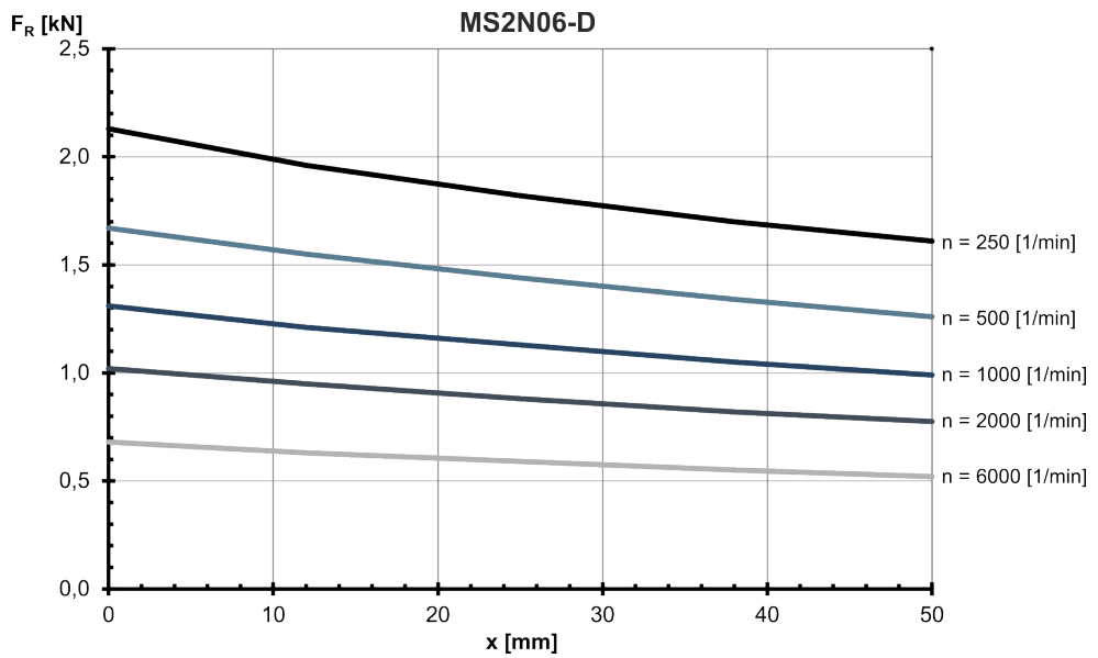
Fig. 88: MS2N06-D: Radial force in distance x from the shaft shoulder at a nominal bearing service life of Lh10 = 30000 h
