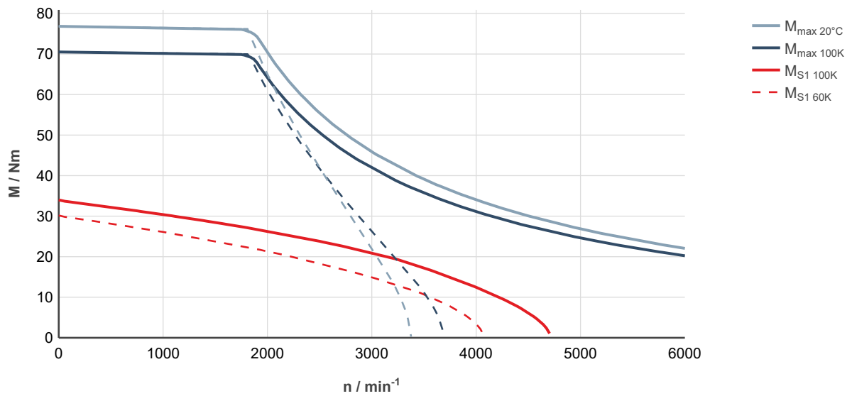
Fig. 197: MS2N10-C0BNN-___0-___-_, ctrlX DRIVE, uncontrolled supply 3 × AC 400 V
