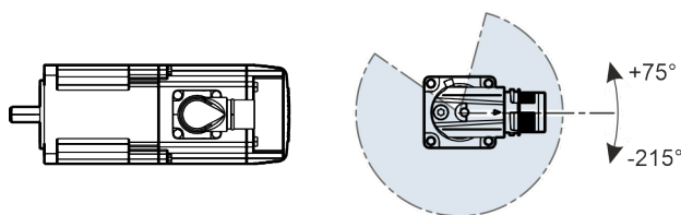
Fig. 378: Rotating area electrical connection "H"
