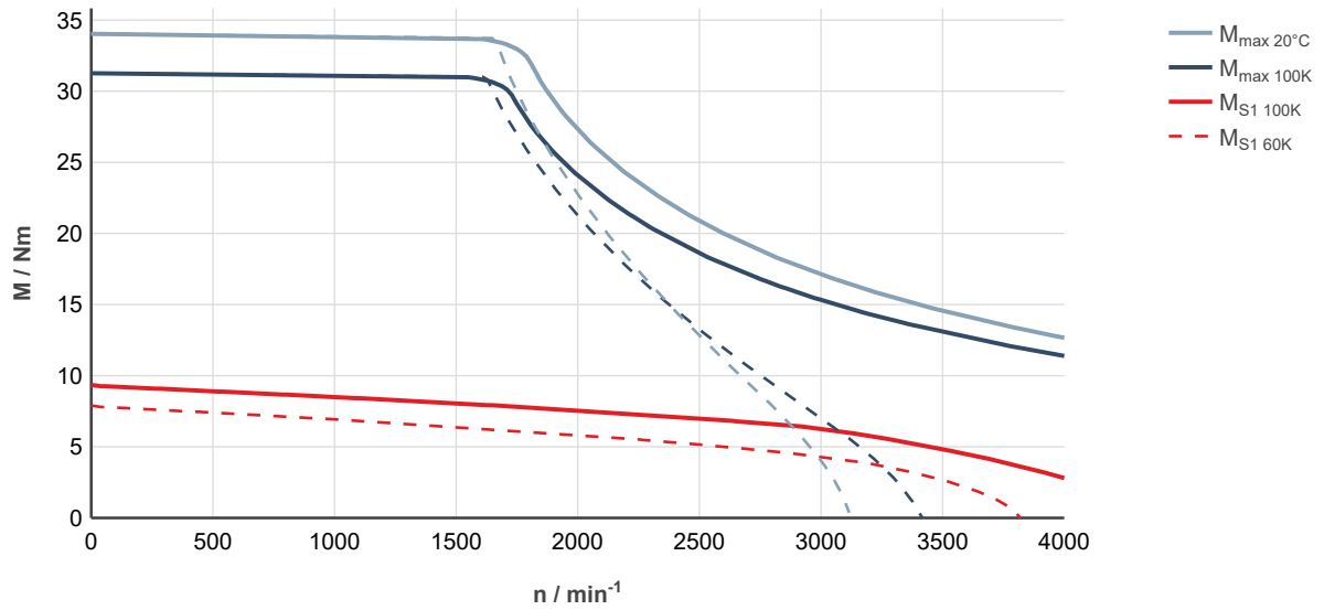
Fig. 61: MS2N05-D0BHN-___0-___-_, ctrIX DRIVE, controlled supply 3 x AC 400 ... 480 V
