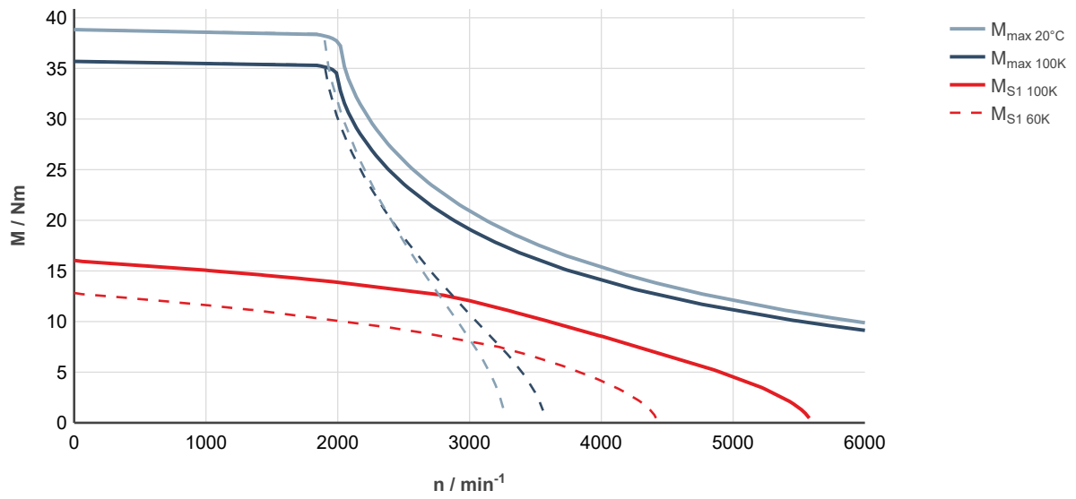
Fig. 92: MS2N07-C0BNN-___0-___-___, ctrlX DRIVE, uncontrolled supply 3 × AC 400 V
