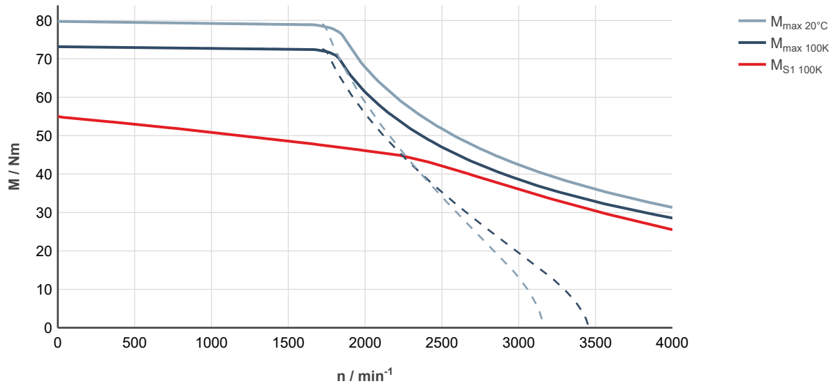
Fig. 171: MS2N07-D0BHL-___0-___-___, ctrIX DRIVE, controlled supply 3 × AC 400 ... 480 V
