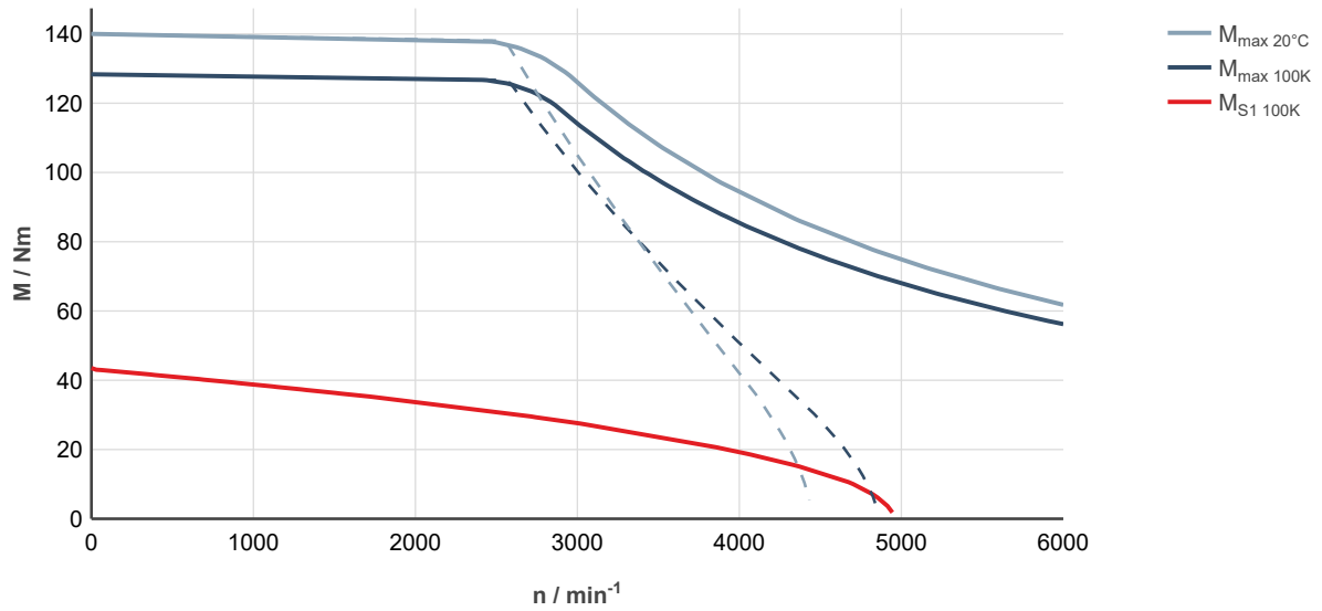
Fig. 163: MS2N07-E1BNA-___0-___-__, ctrlX DRIVE, controlled supply 3 × AC 400 ... 480 V
