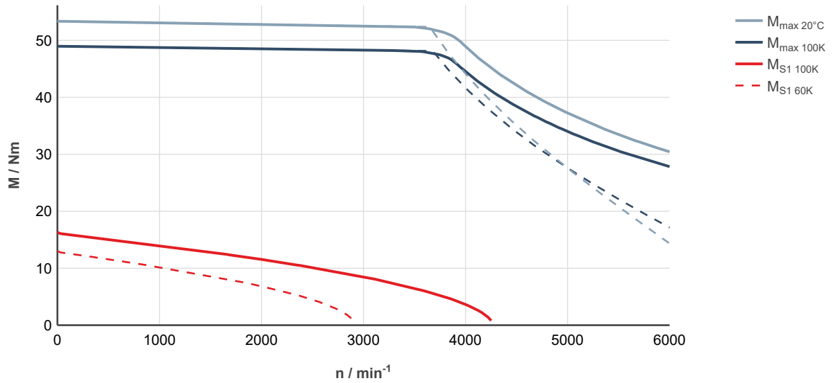
Fig. 84: MS2N06-E0BRN-___0-___-___, ctrlX DRIVE, controlled supply 3 × AC 400 ... 480 V
