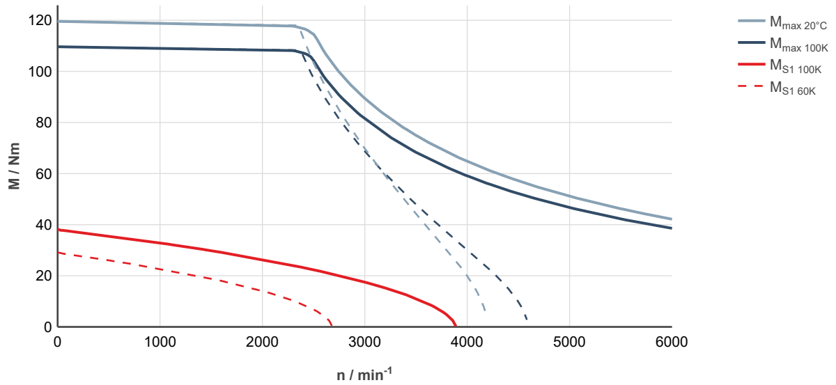
Fig. 119: MS2N07-E0BNN-___0-___-_, ctrlX DRIVE, controlled supply 3 × AC 400 ... 480 V
