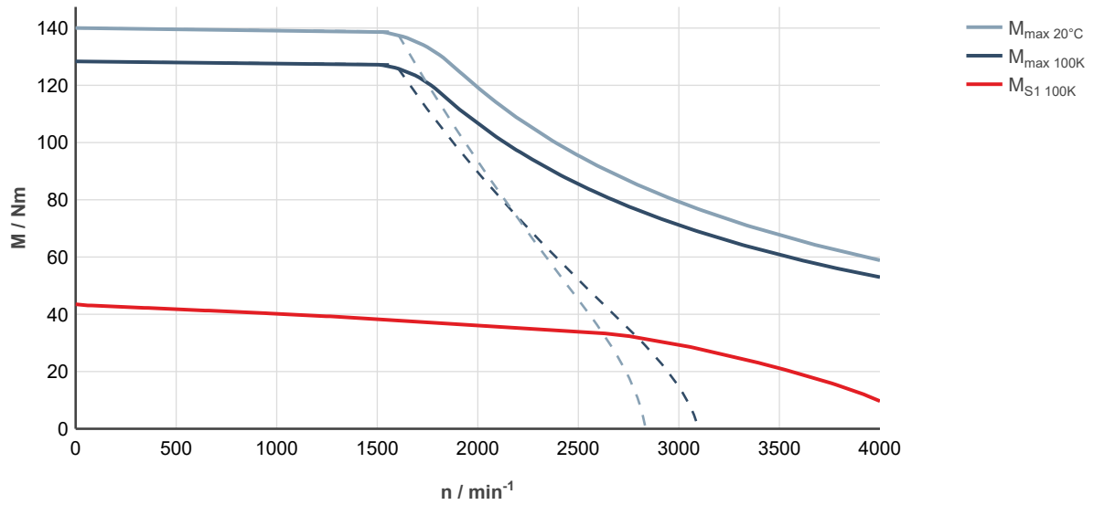
Fig. 161: MS2N07-E1BHA-___0-___-_, ctrIX DRIVE, controlled supply 3 x AC 400 ... 480 V
