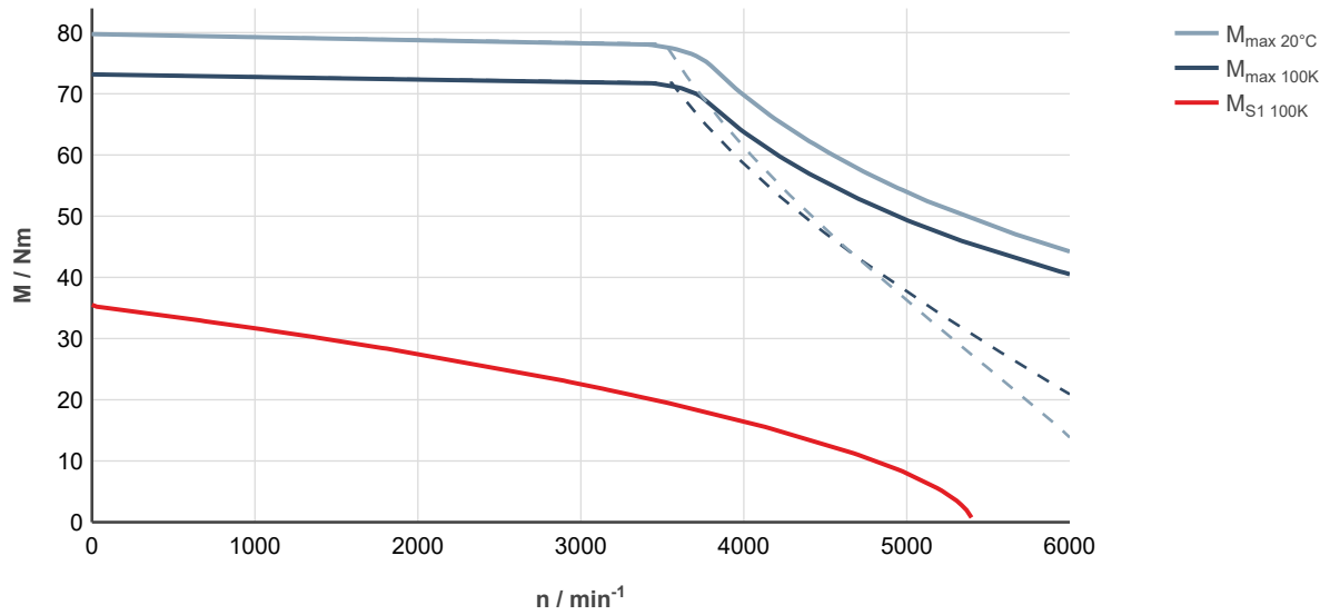
Fig. 143: MS2N07-D0BRA-___0-___-_, ctrlX DRIVE, controlled supply 3 × AC 400 ... 480 V
