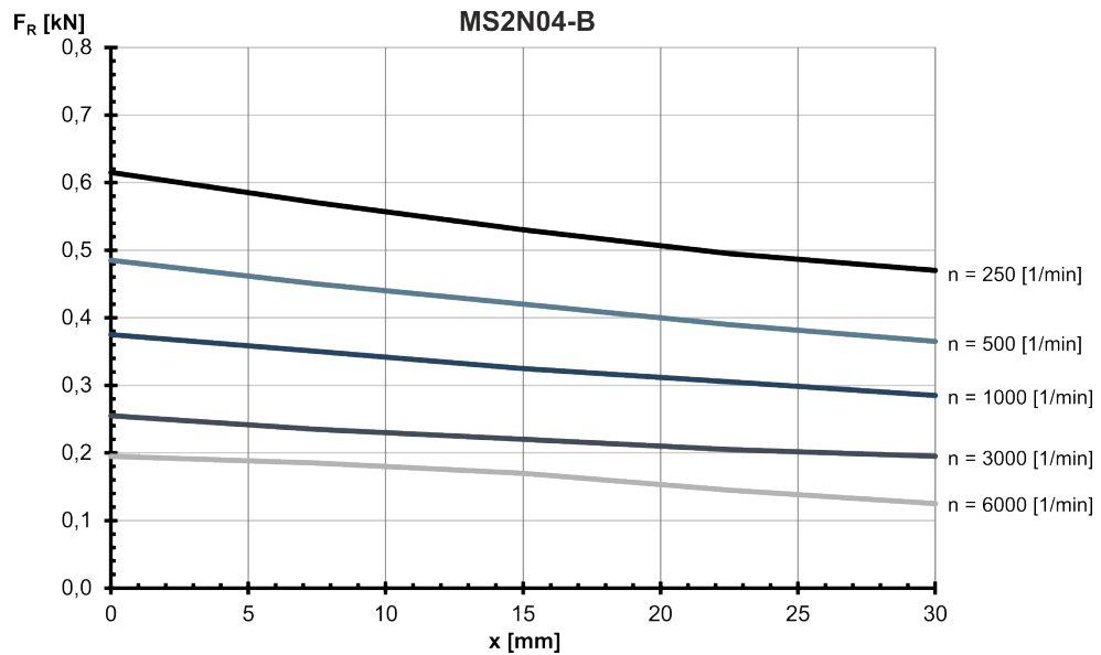
Fig. 49: MS2N04-B: Radial force in distance x from the shaft shoulder at a nominal bearing service life of L_{h10} = 30000 h
