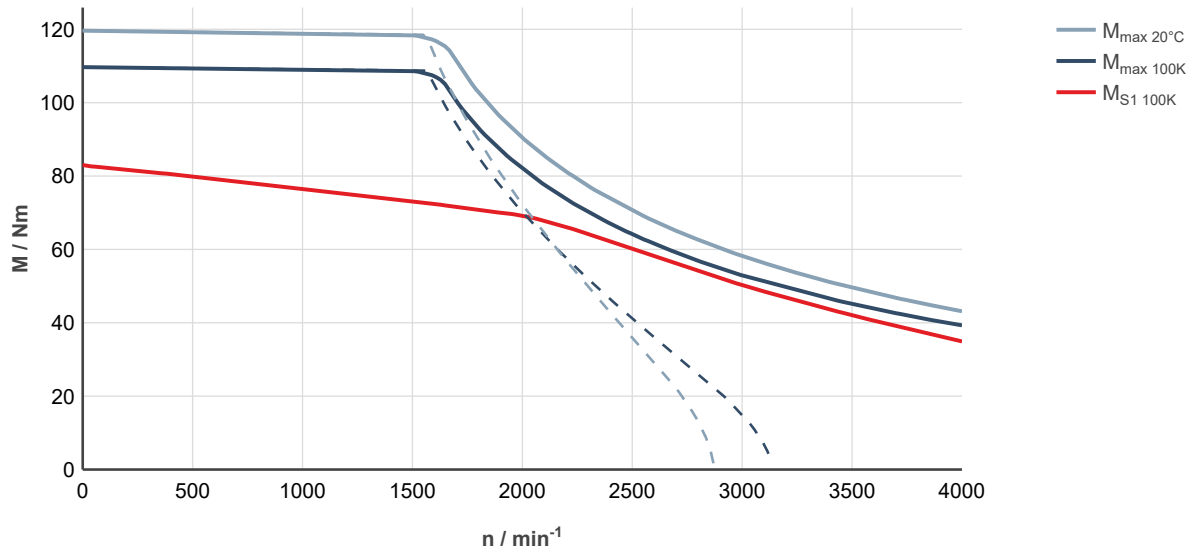
Fig. 179: MS2N07-E0BHL-___0-___-___, ctrIX DRIVE, controlled supply 3 × AC 400 ... 480 V
