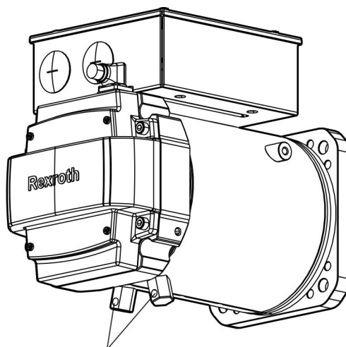
Fig. 394: Coolant connection MS2N10-__L__C__
