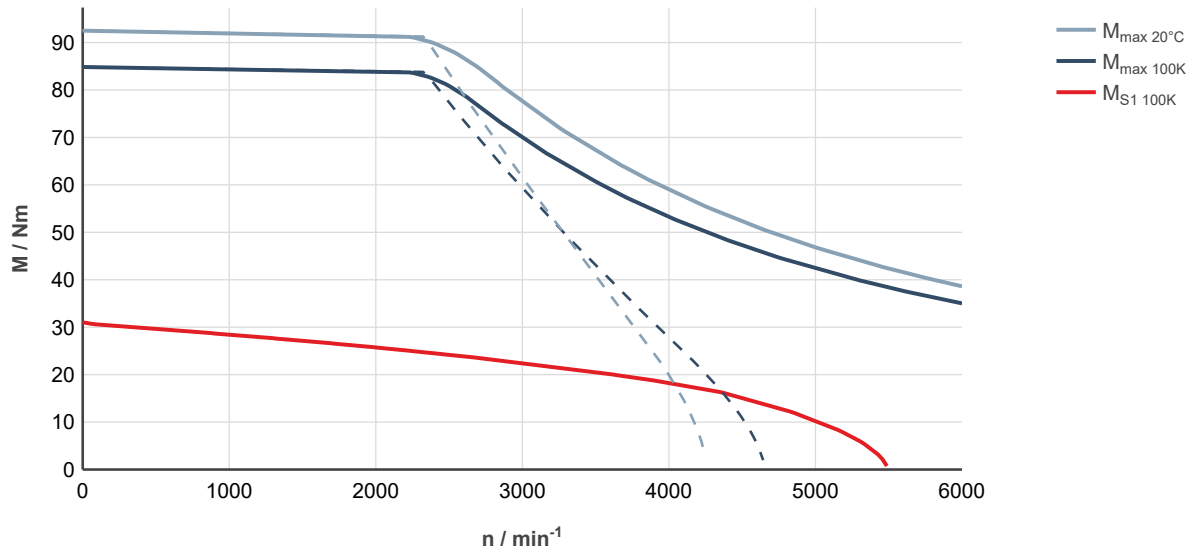
Fig. 149: MS2N07-D1BNA-___0-___- , ctrlX DRIVE, controlled supply 3 × AC 400 ... 480 V
