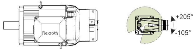
Fig. 371: Rotating area electrical connection "T"
