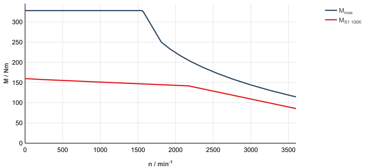
Fig. 319: MS2N13-B1BHC-___0-___-__, ctrlX DRIVE, uncontrolled supply 3 × AC 400 V M_max Characteristic curve applies to maximum torque 20 °C (cold)
