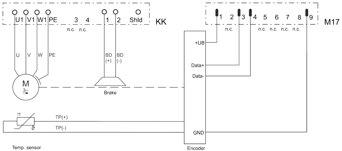
Fig. 361: Double cable connection terminal boxes, digital encoder C and D, brake optional
