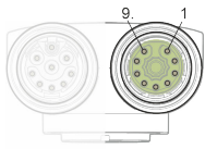
Fig. 374: Connector view double plug M17 encoder
