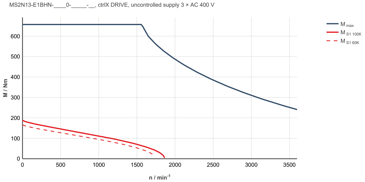
Fig. 315: MS2N13-E1BHN-___0-___-___, ctrlX DRIVE, uncontrolled supply 3 × AC 400 V M max : Characteristic curve applies to maximum torque 20 °C (cold)
