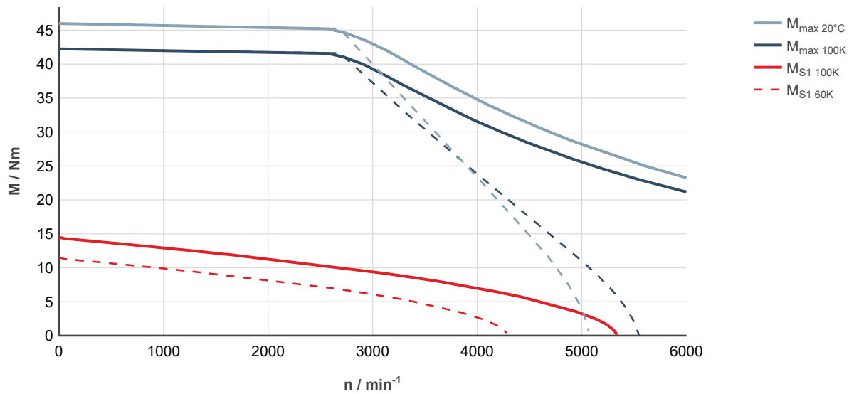
Fig. 98: MS2N07-C1BRN-___0-___-__, ctrlX DRIVE, uncontrolled supply 3 × AC 400 V
