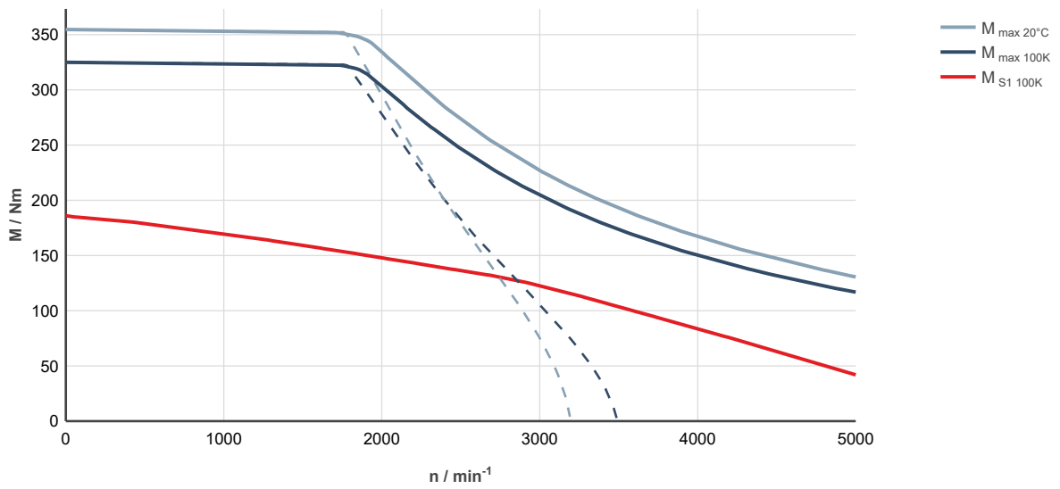
Fig. 287: MS2N10-R0BLL-___0-___-__, ctrlX DRIVE, uncontrolled supply 3 × AC 400 V
