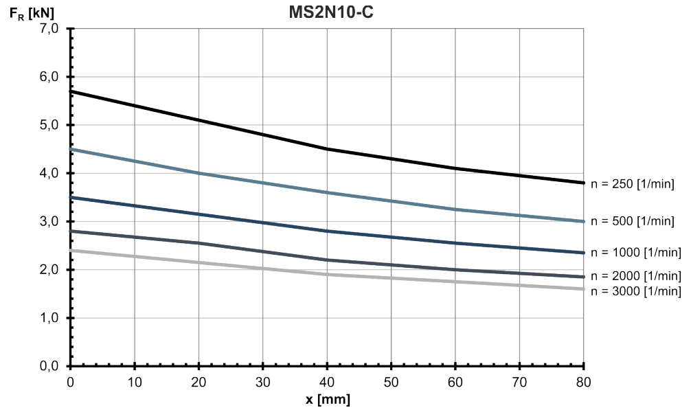
Fig. 298: MS2N10-C: Radial force in distance x from the shaft shoulder at a nominal bearing service life of L_{h10} = 30000 h
