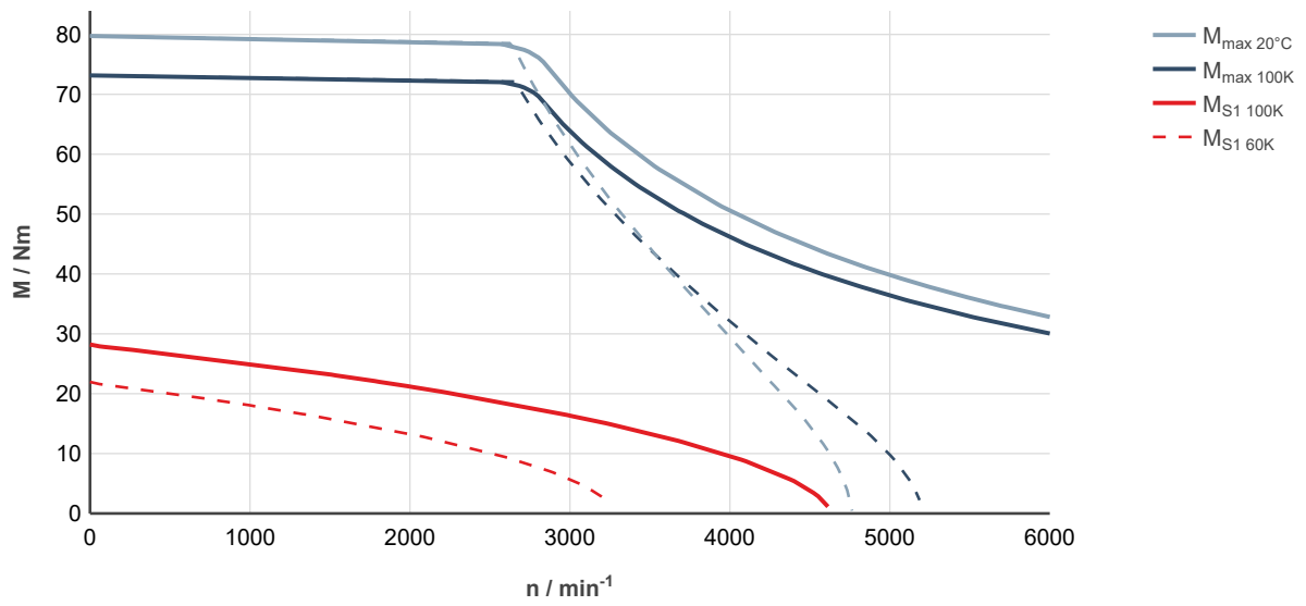
Fig. 106: MS2N07-D0BRN-___0-___-_, ctrlX DRIVE, uncontrolled supply 3 × AC 400 V
