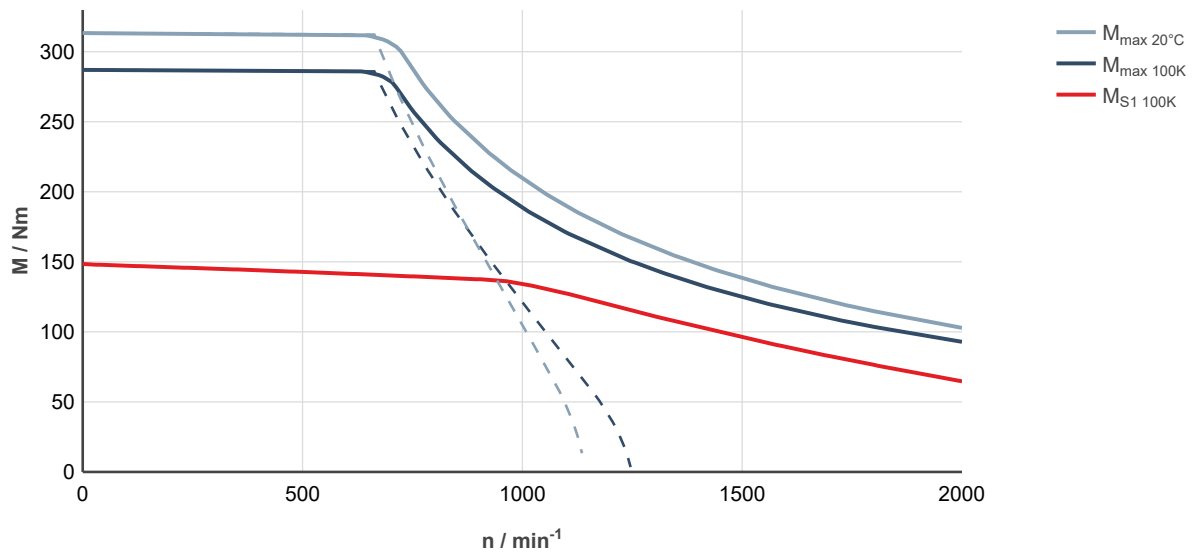
Fig. 253: MS2N10-F0BDA-___0-___-__, ctrlX DRIVE, uncontrolled supply 3 × AC 400 V
