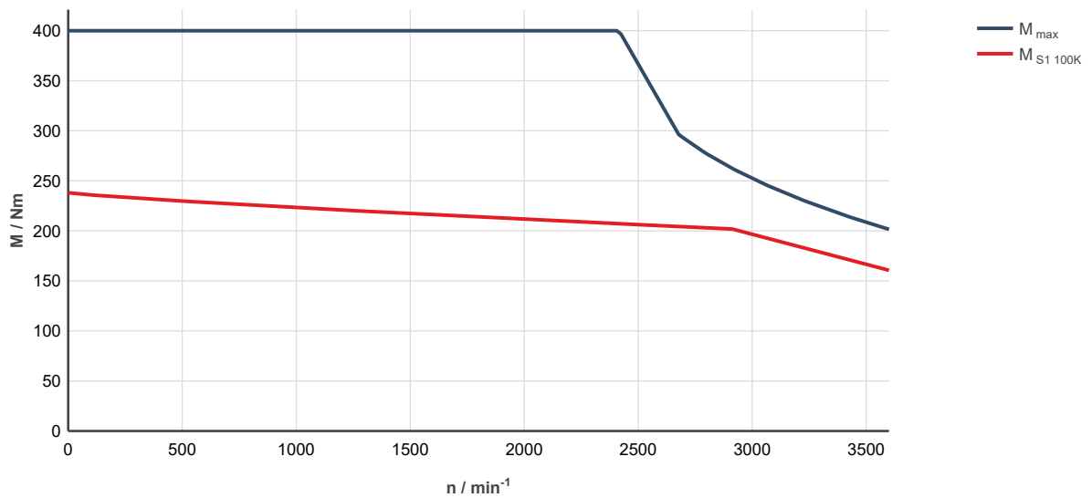
Fig. 340: MS2N13-C1BHL-___0-___-__, ctrlX DRIVE, controlled supply 3 × AC 400 ... 480 V M_{\text{max}} Characteristic curve applies to maximum torque 20 °C (cold)
