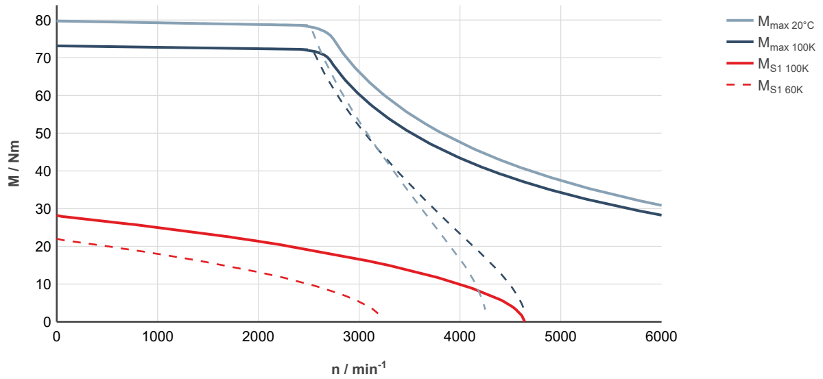
Fig. 105: MS2N07-D0BNN-___0-___-, ctrlX DRIVE, controlled supply 3 × AC 400 ... 480 V
