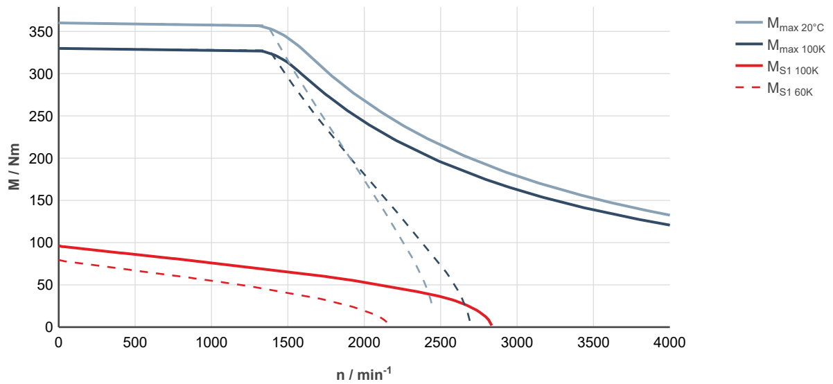
Fig. 225: MS2N10-F1BHN-___0-___-__, ctrlX DRIVE, uncontrolled supply 3 × AC 400 V
