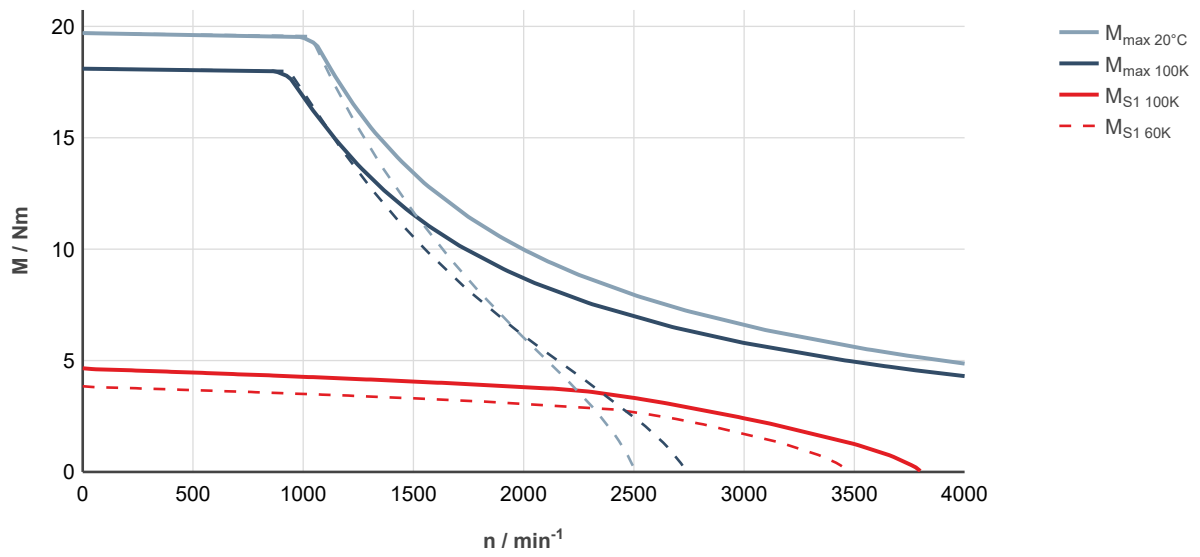
Fig. 43: MS2N04-D0BHN-___0-___-_, ctrlX DRIVE, uncontrolled supply 3 × AC 400 V
