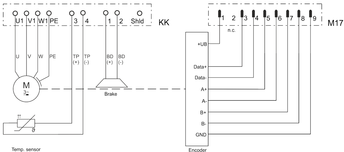
Fig. 362: Double cable connection terminal boxes, analog encoder A, brake optional
