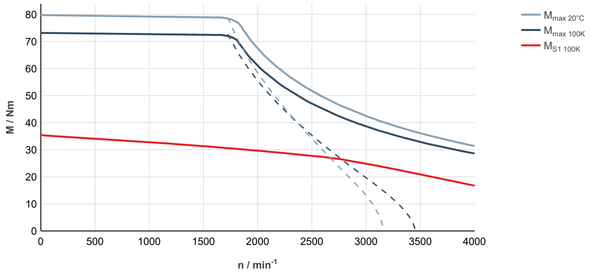
Fig. 139: MS2N07-D0BHA-___0-___-_, ctrlX DRIVE, controlled supply 3 × AC 400 ... 480 V
