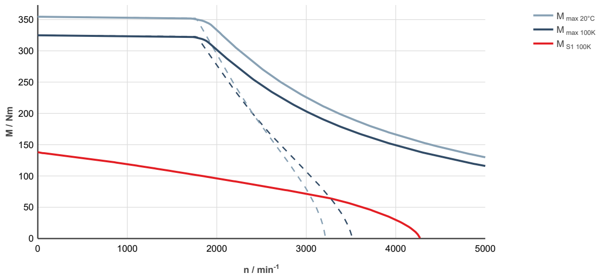
Fig. 261: MS2N10-R0BLA-___0-___-___, ctrlX DRIVE, uncontrolled supply 3 × AC 400 V
