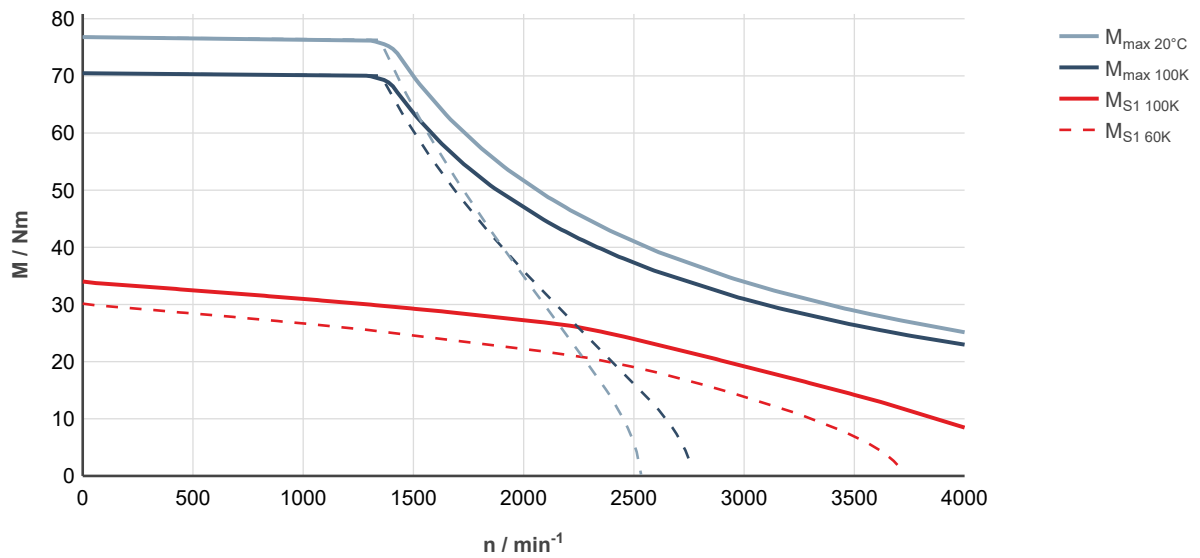
Fig. 195: MS2N10-C0BHN-___0-___-_, ctrlX DRIVE, uncontrolled supply 3 × AC 400 V
