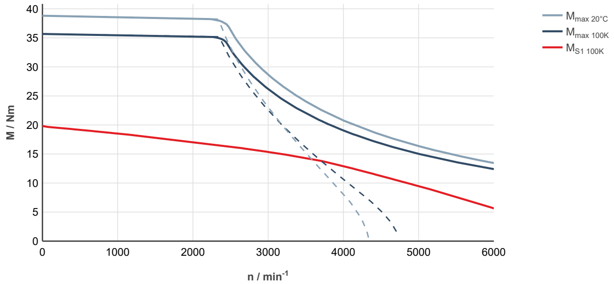
Fig. 129: MS2N07-C0BNA-___0-___-_, ctrlX DRIVE, controlled supply 3 × AC 400 ... 480 V
