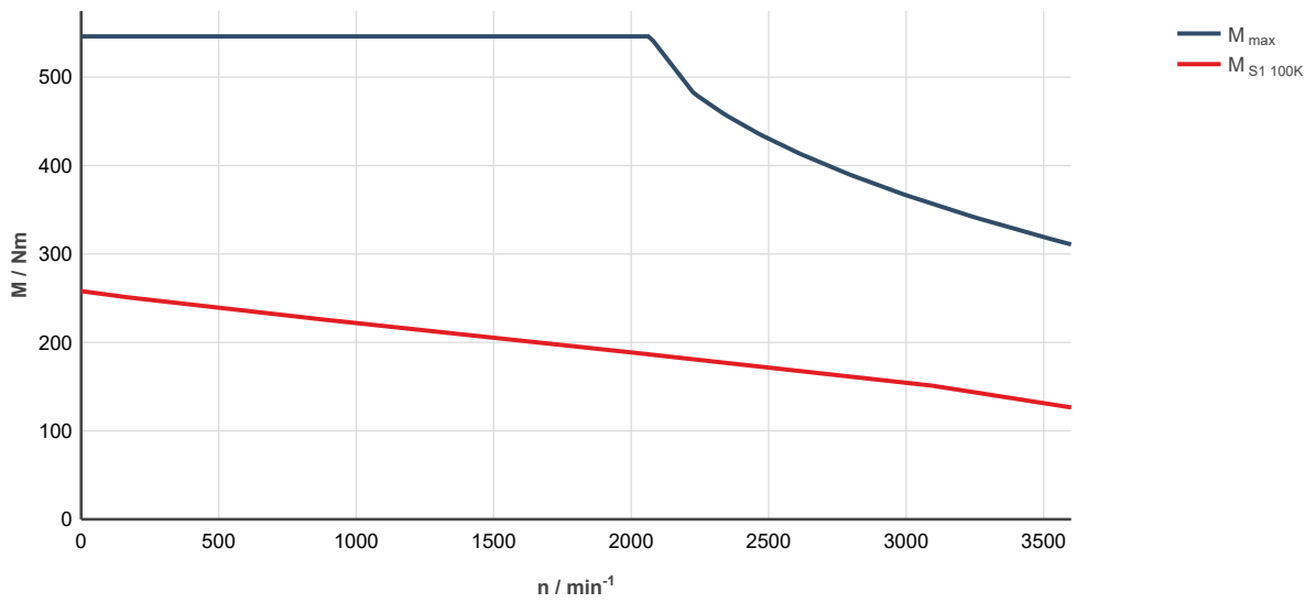
Fig. 329: MS2N13-D1BNC-___0-___-_, ctrlX DRIVE, uncontrolled supply 3 × AC 400 V M_{\text{max}} : Characteristic curve applies to maximum torque 20 °C (cold)
