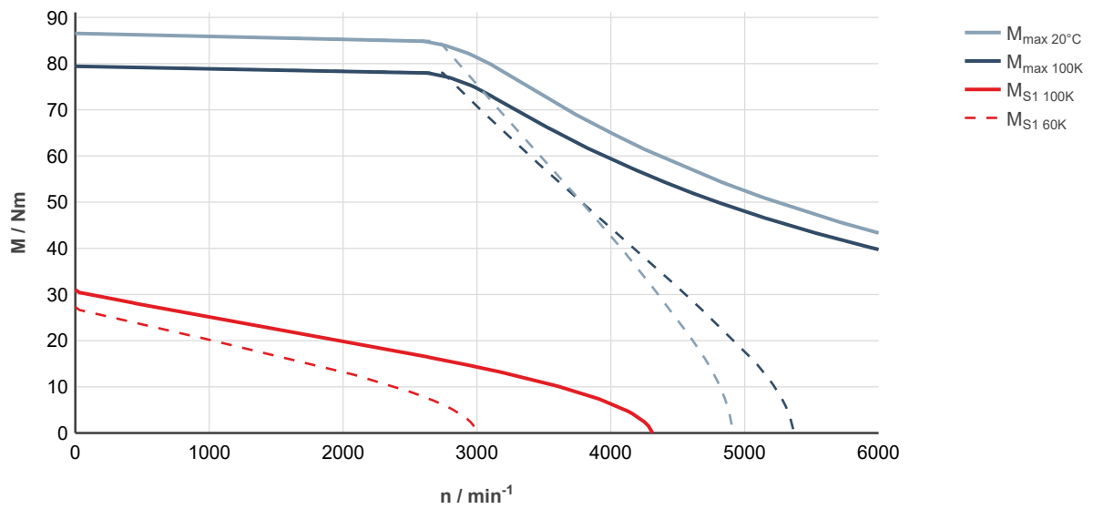
Fig. 202: MS2N10-C1BNN-___0-___-_, ctrlX DRIVE, controlled supply 3 × AC 400 ... 480 V
