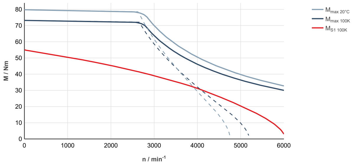
Fig. 174: MS2N07-D0BRL-___0-___-___, ctrlX DRIVE, uncontrolled supply 3 × AC 400 V
