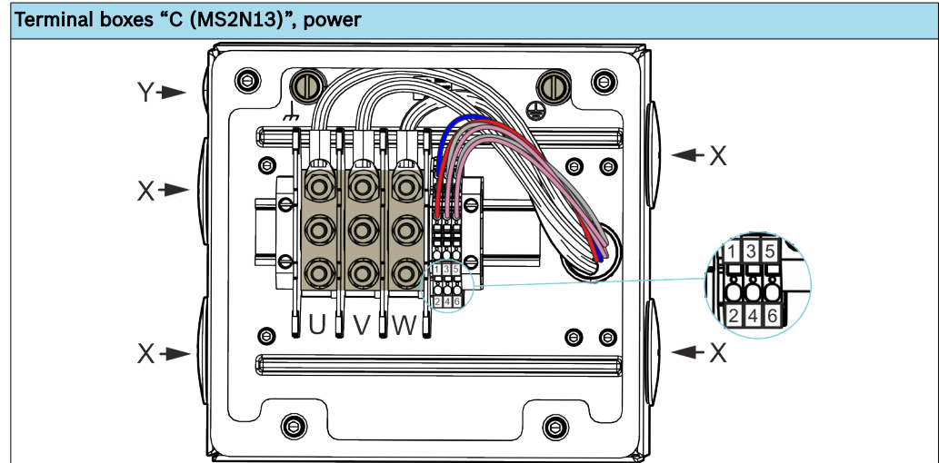
Pin assignment, terminal boxes "C (MS2N13)", power
