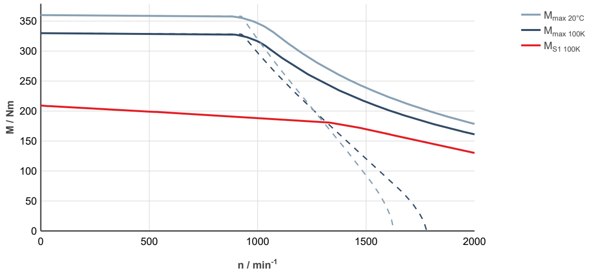
Fig. 284: MS2N10-F1BDL-___0-___-___, ctrlX DRIVE, controlled supply 3 × AC 400 ... 480 V
