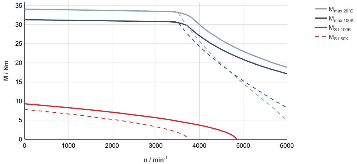
Fig. 63: MS2N05-D0BRN-___0-___-___, ctrlX DRIVE, controlled supply 3 × AC 400 ... 480 V
