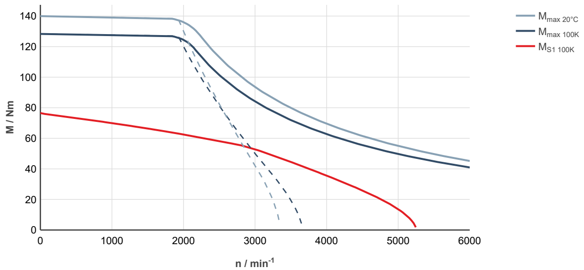
Fig. 184: MS2N07-E1BNL-__0-__-__, ctrlX DRIVE, uncontrolled supply 3 × AC 400 V
