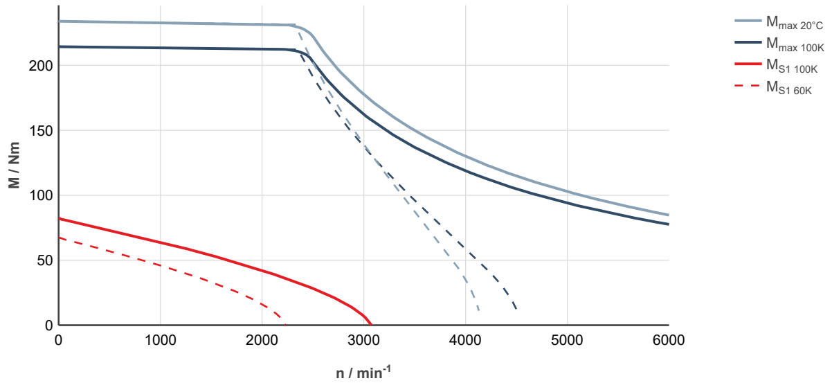
Fig. 214: MS2N10-E0BNN-___0-___-_, ctrlX DRIVE, controlled supply 3 × AC 400 ... 480 V
