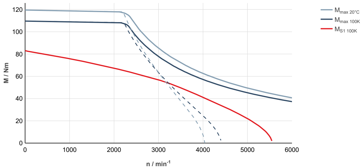
Fig. 182: MS2N07-E0BQL-___0-___-___, ctrIX DRIVE, uncontrolled supply 3 × AC 400 V
