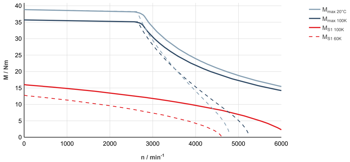
Fig. 94: MS2N07-C0BQN-___0-___-_, ctrlX DRIVE, uncontrolled supply 3 × AC 400 V
