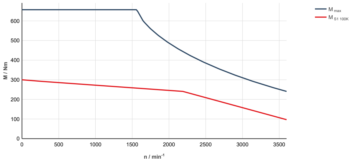
Fig. 331: MS2N13-E1BHC-___0-___-_, ctrIX DRIVE, uncontrolled supply 3 × AC 400 V M_{max} Characteristic curve applies to maximum torque 20 °C (cold)
