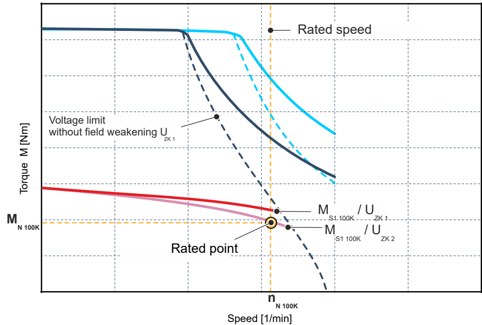
Fig. 21: Rated point
