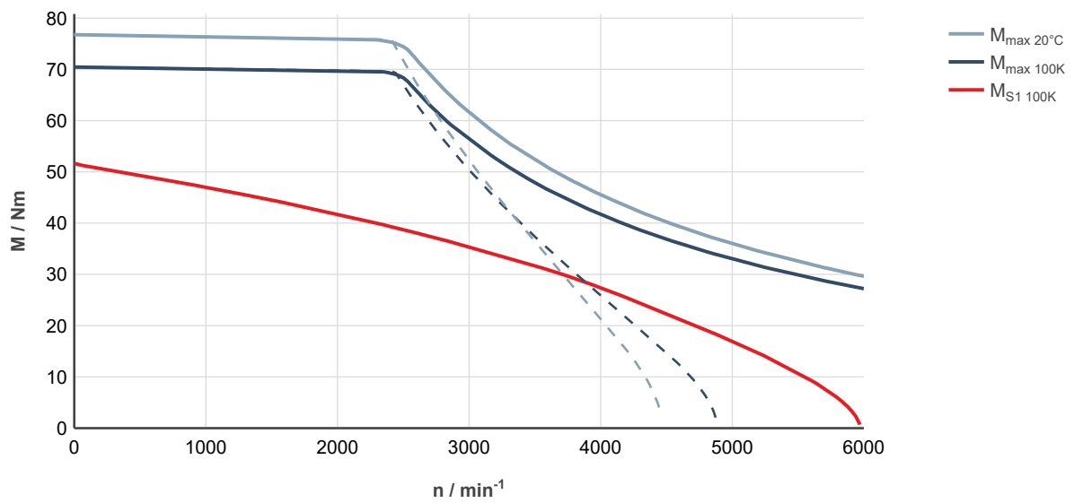
Fig. 266: MS2N10-C0BNL-___0-___-___, ctrlX DRIVE, controlled supply 3 × AC 400 ... 480 V
