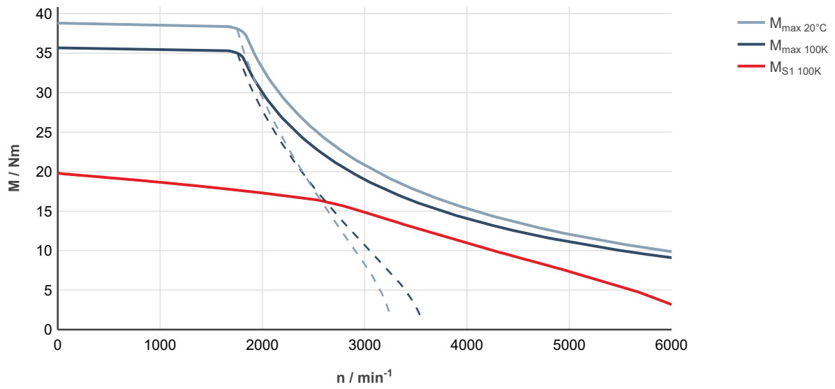
Fig. 128: MS2N07-C0BNA-___0-___-_, ctrlX DRIVE, uncontrolled supply 3 × AC 400 V
