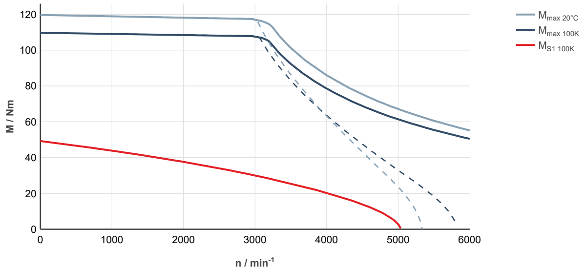
Fig. 157: MS2N07-E0BQA-___0-___-__, ctrlX DRIVE, controlled supply 3 × AC 400 ... 480 V
