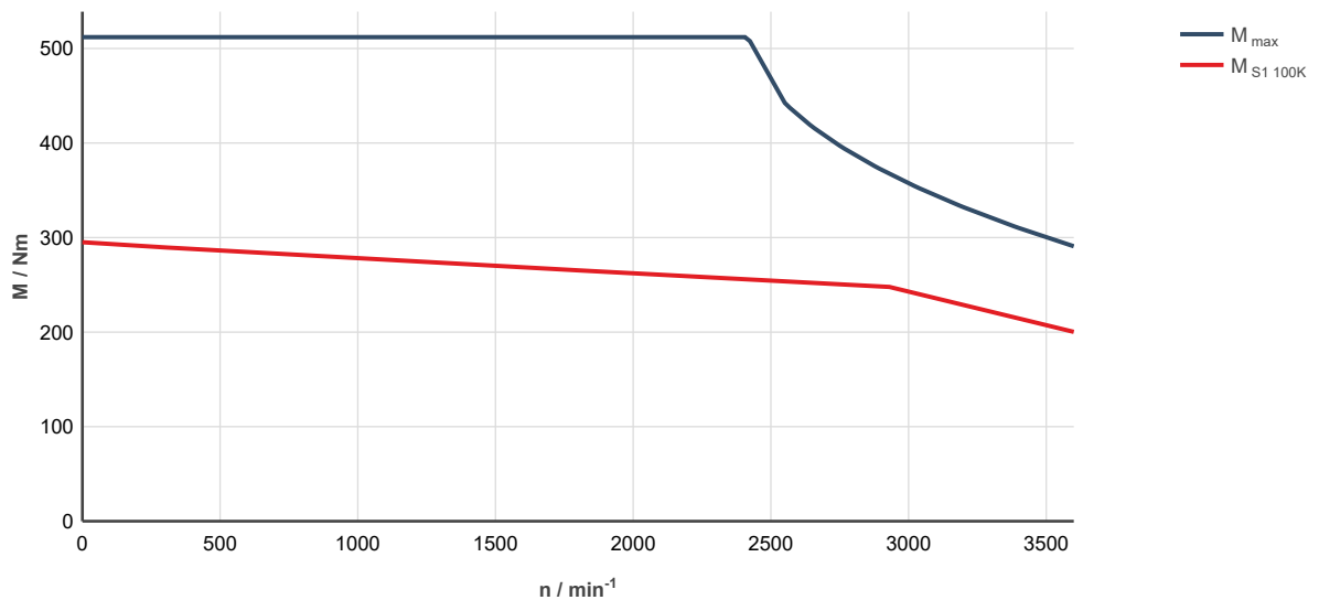
Fig. 344: MS2N13-D1BHL-___0-___-__, ctrlX DRIVE, controlled supply 3 x AC 400 ... 480 V M_{\text{max}} : Characteristic curve applies to maximum torque 20 °C (cold)
