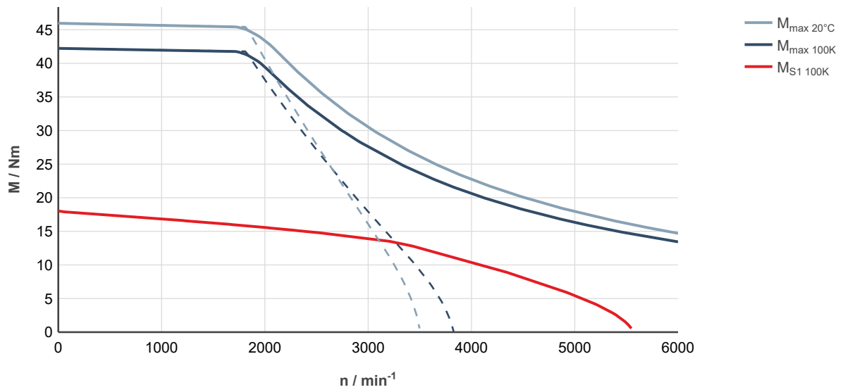
Fig. 132: MS2N07-C1BNA-___0-___-_, ctrlX DRIVE, uncontrolled supply 3 × AC 400 V
