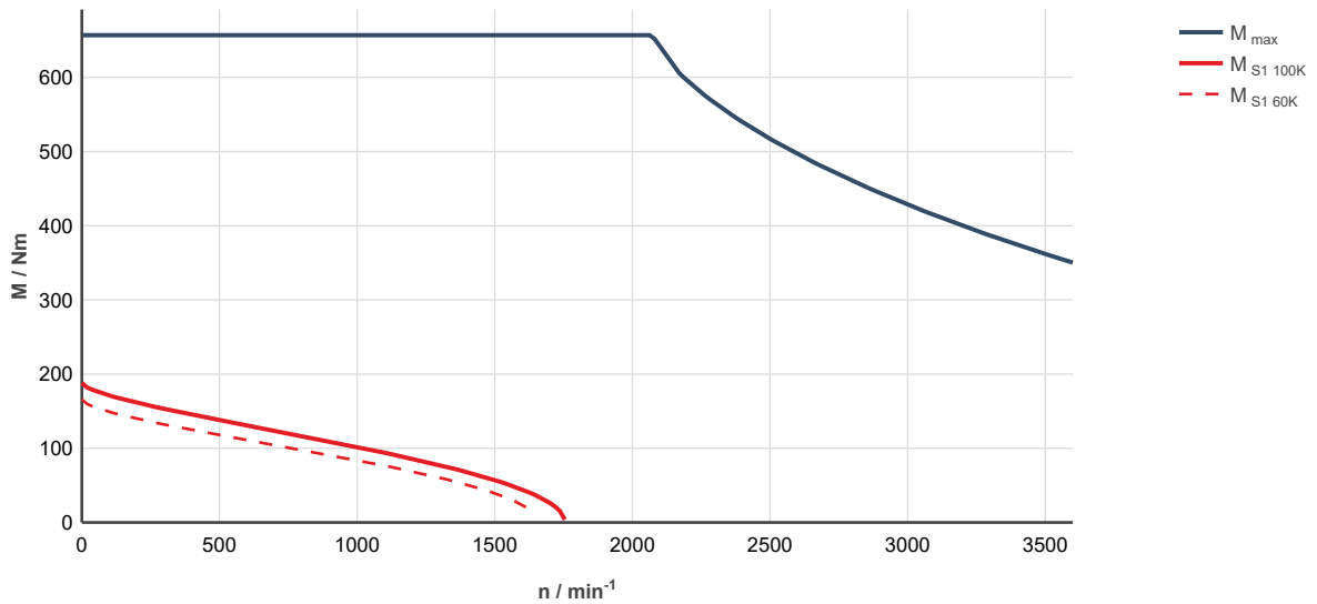
Fig. 316: MS2N13-E1BHN-___0-___-___, ctrlX DRIVE, controlled supply 3 x AC 400 ... 480 V M max : Characteristic curve applies to maximum torque 20 °C (cold)
